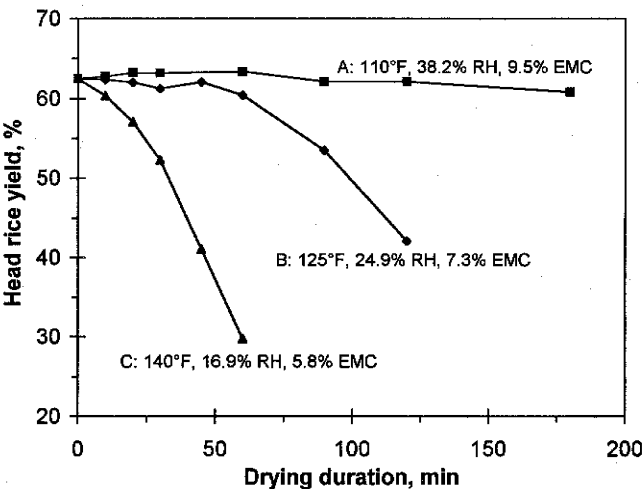
Fig. 1. Changes in head rice yield of Bengal (harvested at 22.5% MC) with drying duration under the three indicated drying air conditions.
