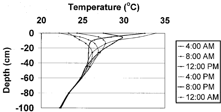
Fig. 3b. Daily soil temperature distribution after flooding on 15 June 1998.
