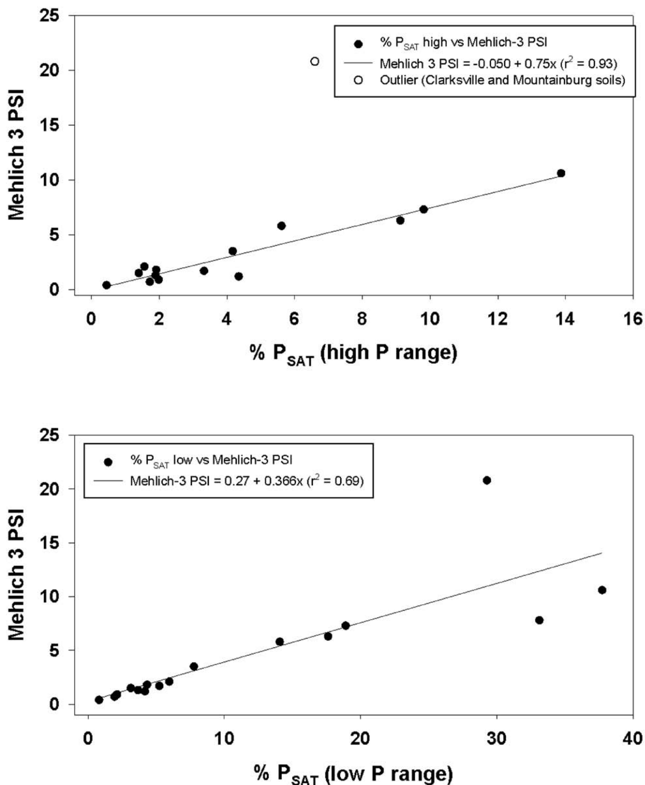
Figure 3. Relationship between percentage soil P saturation [ \% P_{SAT} = \text{Mehlich-3 P (ppm)} / S_{MAX} ] with high ( n=14 ) and low ( n=16 ) P solution ranges and Mehlich-3 P saturation index [ PSI_{M3} = (((\text{Mehlich-3 P}) / (\text{Mehlich-3 Fe} + \text{Al})) \times 100 ; with concentrations expressed as mmol/kg]. Note the different range for x-axis between low and high range.
