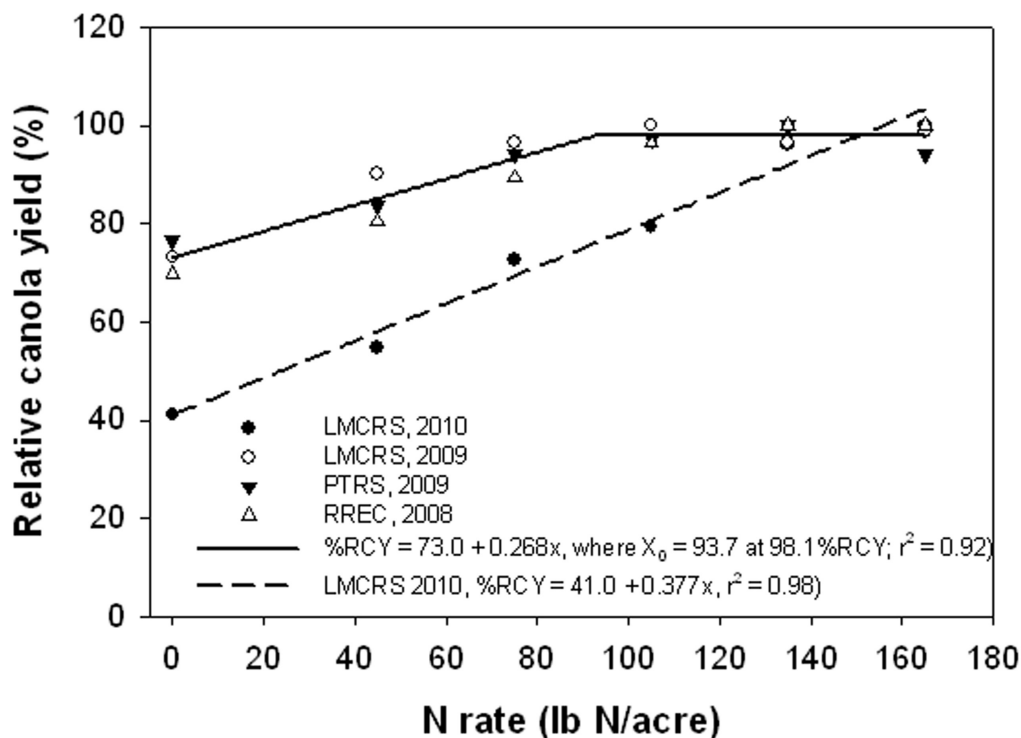
Fig. 1. Nitrogen calibration curves for the 2010 site at Lon Mann Cotton Research Station (LMCRS) and three other sites at the LMCRS, Rice Research Extension Center (RREC), and Pine Tree Research Station (PTRS) as defined using linear and liner-plateau models, respectively.
