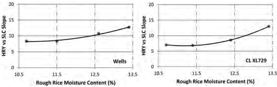
Fig. 5. Head rice yield (HRY) vs. surface lipid content (SLC) regression line slopes of Wells and CL XL729 cultivars milled at rough rice moisture contents of approximately 10.5%, 11.5%, 12.5%, and 13.5% (w.b.) for 10, 20, 30, and 40 s using a laboratory mill. Each data point represents the average slope calculated from each of three milling replications.
