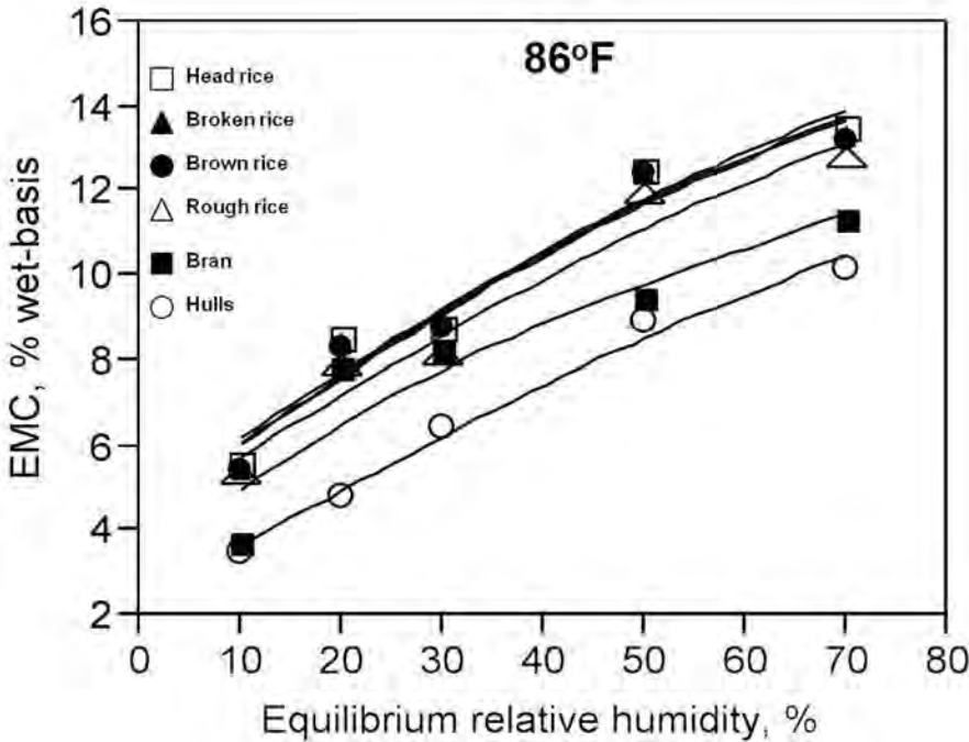
Fig. 2. Equilibrium moisture contents of Wells rice kernel components after exposure to 86 °F and 10% to 70% relative humidity. Each value is an average of four measurements, i.e., two EMC replications with each replicate moisture content measured in duplicate.
