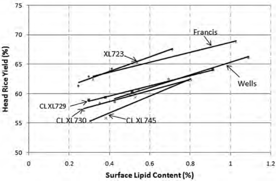
Fig. 2. Head rice yield vs. head rice surface lipid content of Wells, Francis, XL723, CL XL729, CL XL730, and CL XL745 cultivars milled at a rough rice moisture content of approximately 12.5% (w.b.) for 10, 20, 30, and 40 s using a laboratory mill. Each data point represents the average of three milling replications.
