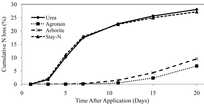
Fig. 2. Cumulative NH 3 volatilization loss from urea, urea + Agrotain, urea + Stay-N, and urea+Arborite applied to a silt loam soil using static diffusion jars (2011).
