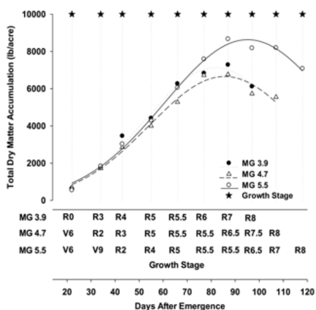
Fig. 2. Dry matter accumulation across time of three soybean cultivars belonging to different maturity groups (MG) as predicted with a Gaussian peak model. Coefficient and estimated parameter values are listed in Table 1.
