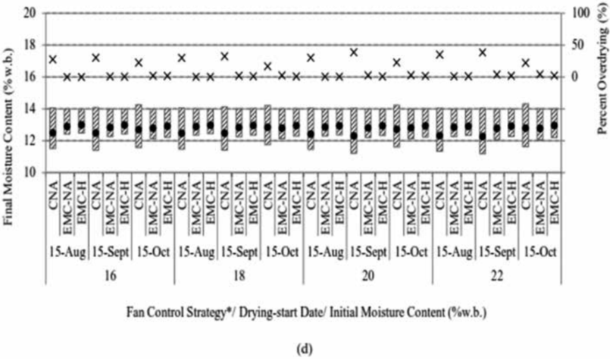
Fig. 3. Effects of initial moisture content (% wet basis, w.b.), fan control strategy, drying-start date, and airflow rate [(a) 0.69 m³/min/ton (0.5 cfm/bu), (b) 1.39 m³/min/ton (1 cfm/bu), (c) 2.08 m³/min/ton (1.5 cfm/bu), and (d) 2.77 m³/min/ton (2 cfm/bu)] on percent overdrying (right y-axis) and minimum, maximum, and average final moisture content of rough rice (left y-axis); The cross (x) and circular solid (●) marks represent the percent overdrying and the average final MC of the rice bed, respectively. The upper and lower limits of the solid box (▨) represent the average of the maximum and minimum final MCs attainable in the rice bed. CNA = continuous natural-air fan control strategy; EMC-NA = equilibrium moisture content controlled natural-air fan control strategy; EMC-H = equilibrium moisture content controlled air with supplemental heat fan control strategy.
