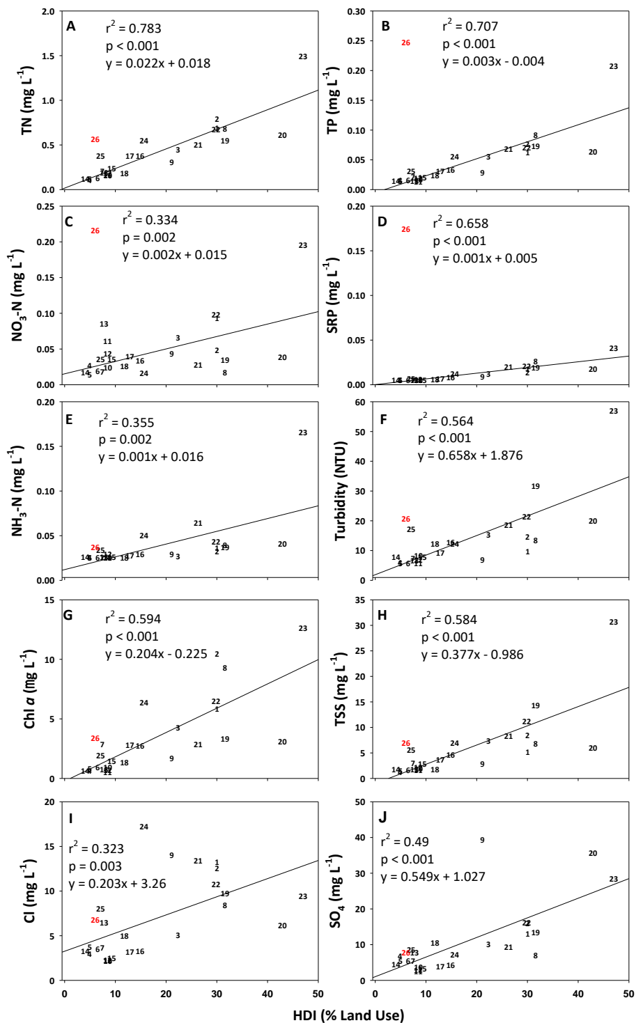
Figure 3: Simple linear regression of geomean constituent concentrations verse human disturbance index (HDI) values for the Oklahoma portion of the Lake Wister Watershed. The site number in red is Shawnee Creek at highway 59 downstream of effluent discharge, thus it was not used in the statistical analysis.
