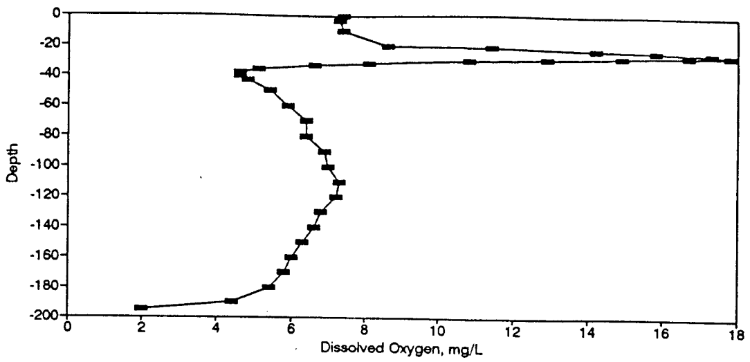
Figure BD175. Dissolved Oxygen Profile for the Eureka Springs Site-August 9, 1988.
