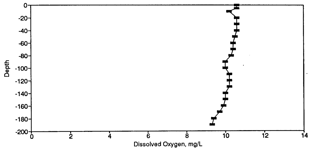
Figure BD27. Dissolved Oxygen Profile for the Eureka Springs Site-March 23, 1976.
