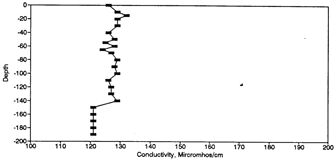
Figure BC29. Conductivity Profile for the Eureka Springs Site-May 25, 1976.
