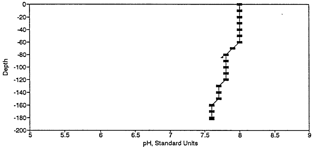
Figure BP110. pH Profile for the Eureka Springs Site-March 23, 1983.
