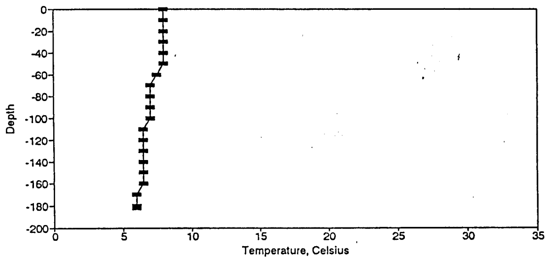
Figure BT110. Temperature Profile for the Eureka Springs Site, March 23, 1983.
