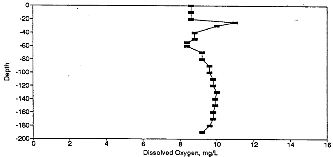
Figure BD54. Dissolved Oxygen Profile for the Eureka Springs Site-June 15, 1978.
