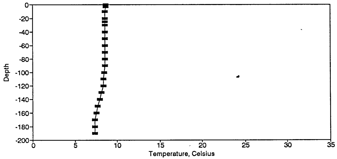
Figure BT179. Temperature Profile for the Eureka Springs Site-January 4, 1989.
