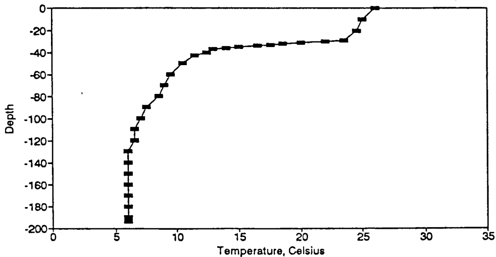
Figure BT78. Temperature Profile for the Eureka Springs Site-June 19, 1980.
