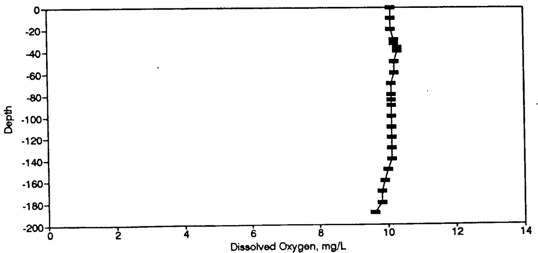
Figure BD99. Dissolved Oxygen Profile for the Eureka Springs Site-April 20, 1982.
