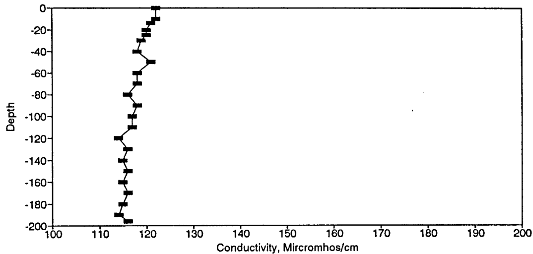
Figure BC147. Conductivity Profile for the Eureka Springs Site-April 9, 1986.
