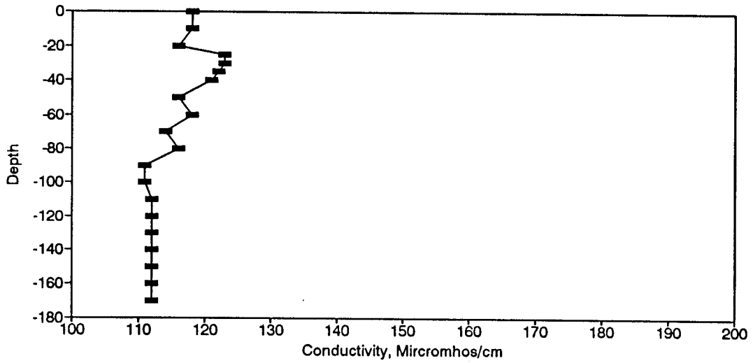
Figure BC19. Conductivity Profile for the Eureka Springs Site-July 8, 1975.
