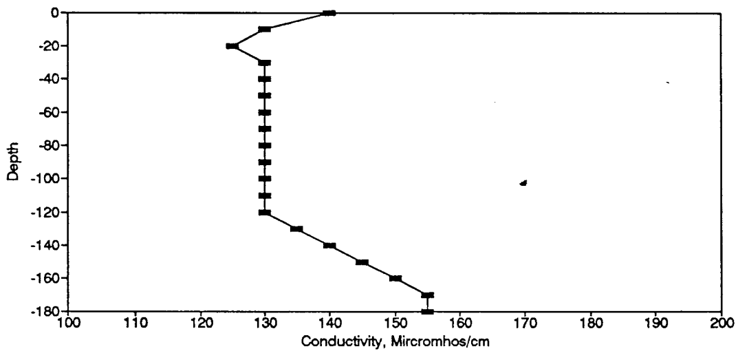
Figure BC35. Conductivity Profile for the Eureka Springs Site-November 16, 1976.
