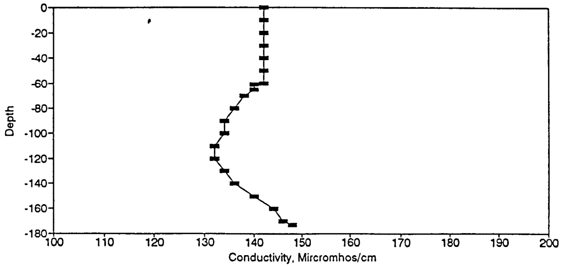
Figure BC118. Conductivity Profile for the Eureka Springs Site-November 14, 1983.
