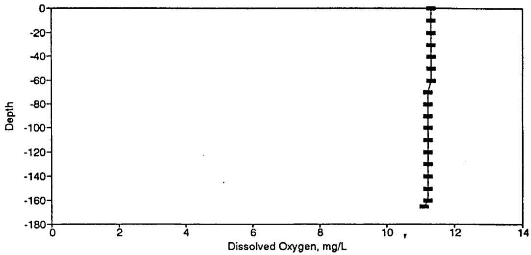
Figure BD121. Dissolved Oxygen Profile for the Eureka Springs Site-February 29, 1984.
