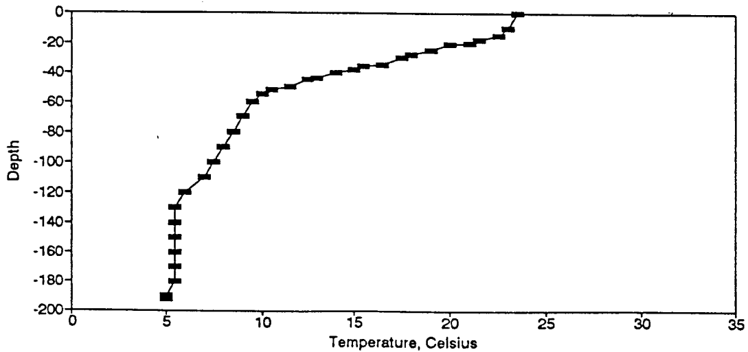
Figure BT66. Temperature Profile for the Eureka Springs Site-June 6, 1979.
