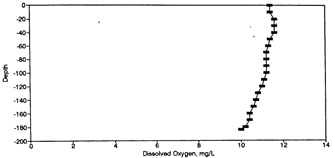
Figure BD98. Dissolved Oxygen Profile for the Eureka Springs Site-March 23, 1982.
