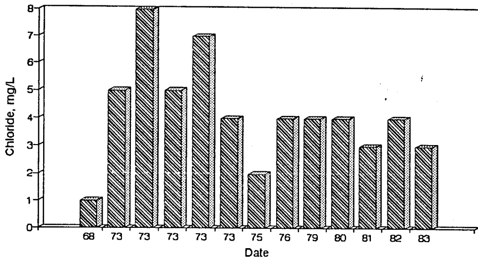
Figure A8. Graph of Chloride vs. Time for the White River Site-Aug.
