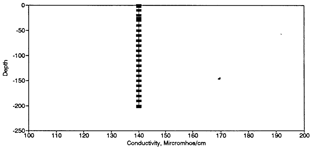
Figure BC131. Conductivity Profile for the Eureka Springs Site-December 13, 1984.
