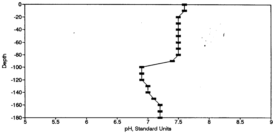
Figure BP35. pH Profile for the Eureka Springs Site-November 16, 1976.
