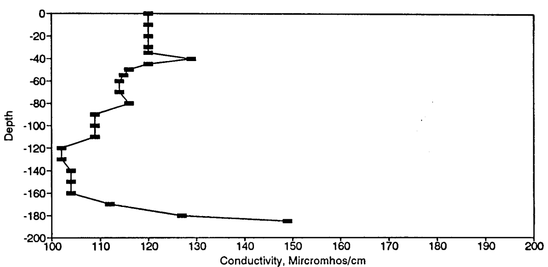
Figure BC21. Conductivity Profile for the Eureka Springs Site-September 17, 1975.
