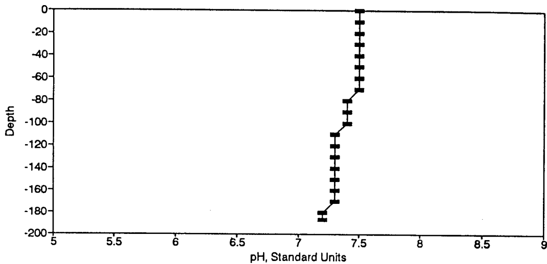
Figure BP64. pH Profile for the Eureka Springs Site-April 9, 1979.
