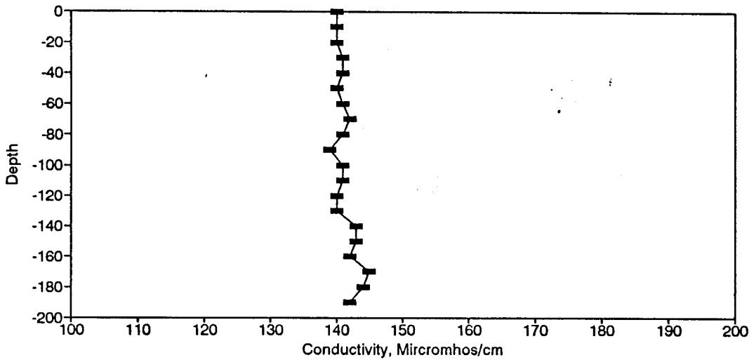
Figure BC170. Conductivity Profile for the Eureka Springs Site-March 16, 1988.
