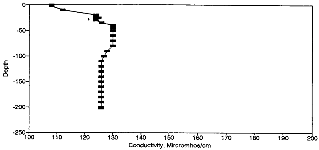
Figure BC136. Conductivity Profile for the Eureka Springs Site-May 8, 1985.
