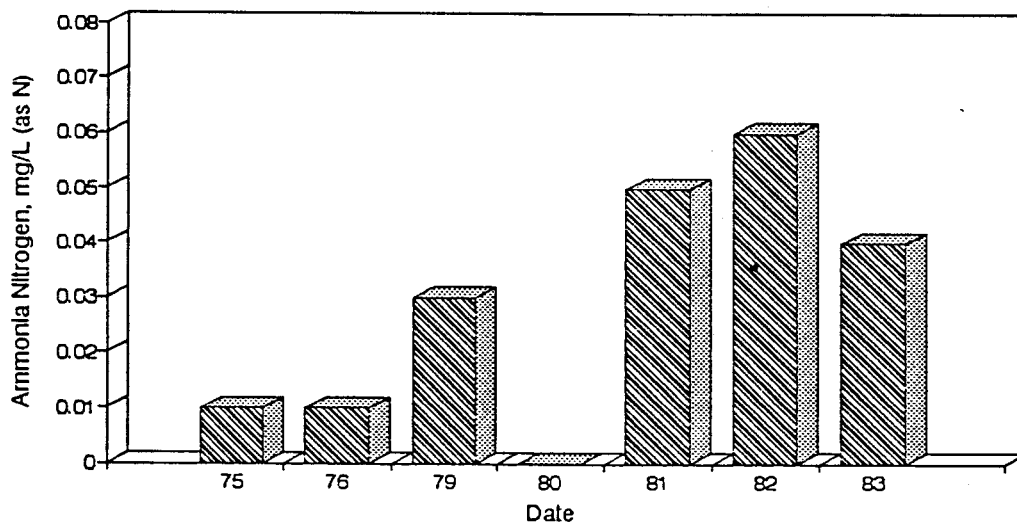
Figure A77. Graph of Ammonia Nitrogen vs. Time for the White River Site-Aug.
