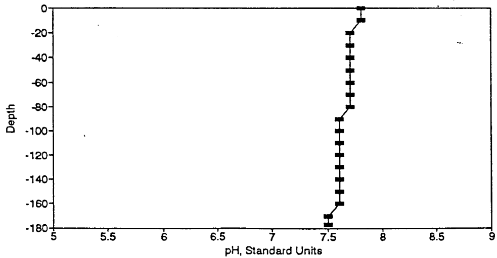
Figure BP75. pH Profile for the Eureka Springs Site-March 12, 1980.
