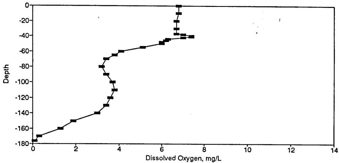
Figure BD116. Dissolved Oxygen Profile for the Eureka Springs Site-September 19, 1983.
