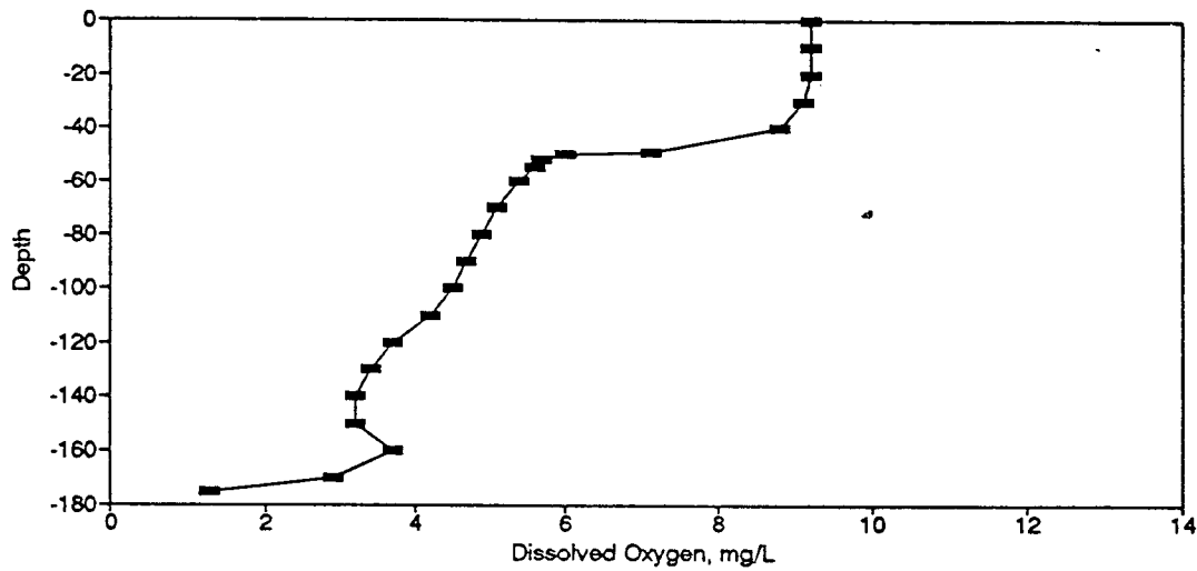
Figure BD83. Dissolved Oxygen Profile for the Eureka Springs Site-November 5, 1980.
