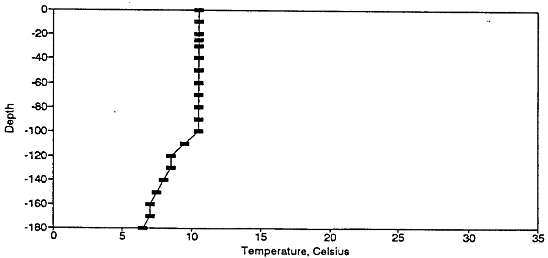
Figure BT72. Temperature Profile for the Eureka Springs Site-December 5, 1979.
