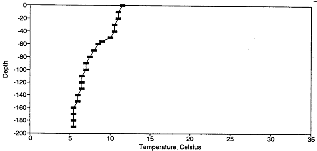
Figure BT123. Temperature Profile for the Eureka Springs Site-April 24, 1984.
