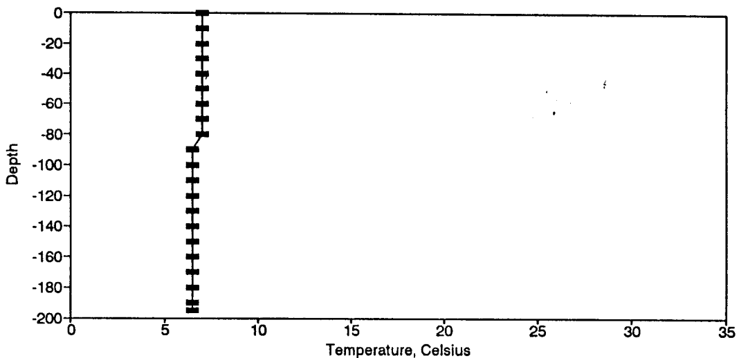
Figure BT14. Temperature Profile for the Eureka Springs Site-February 18, 1975.
