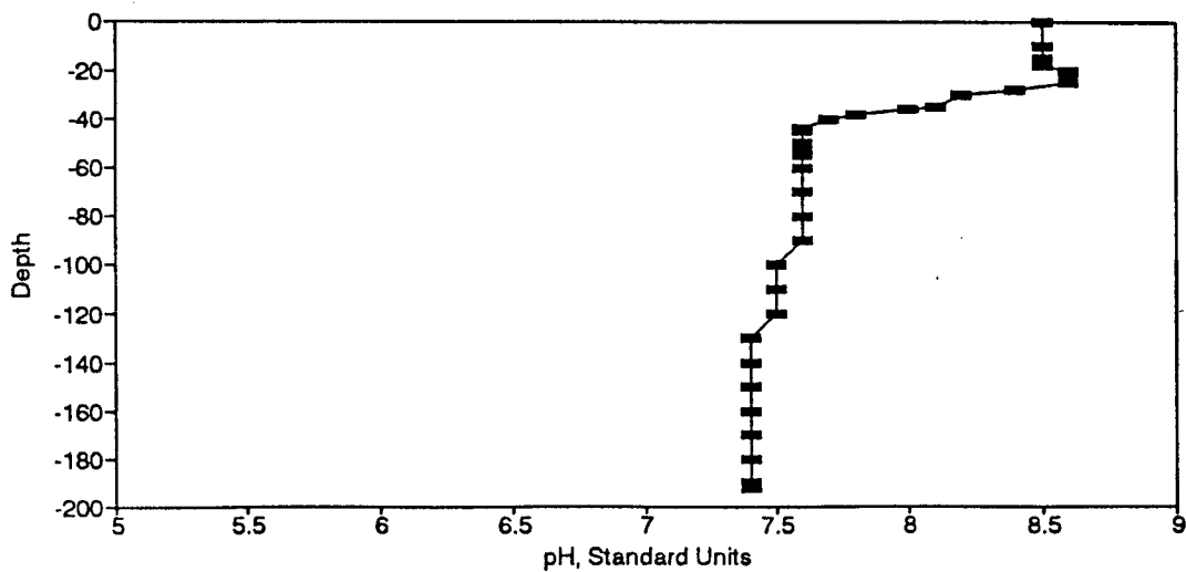
Figure BP66. pH Profile for the Eureka Springs Site-June 6, 1979.
