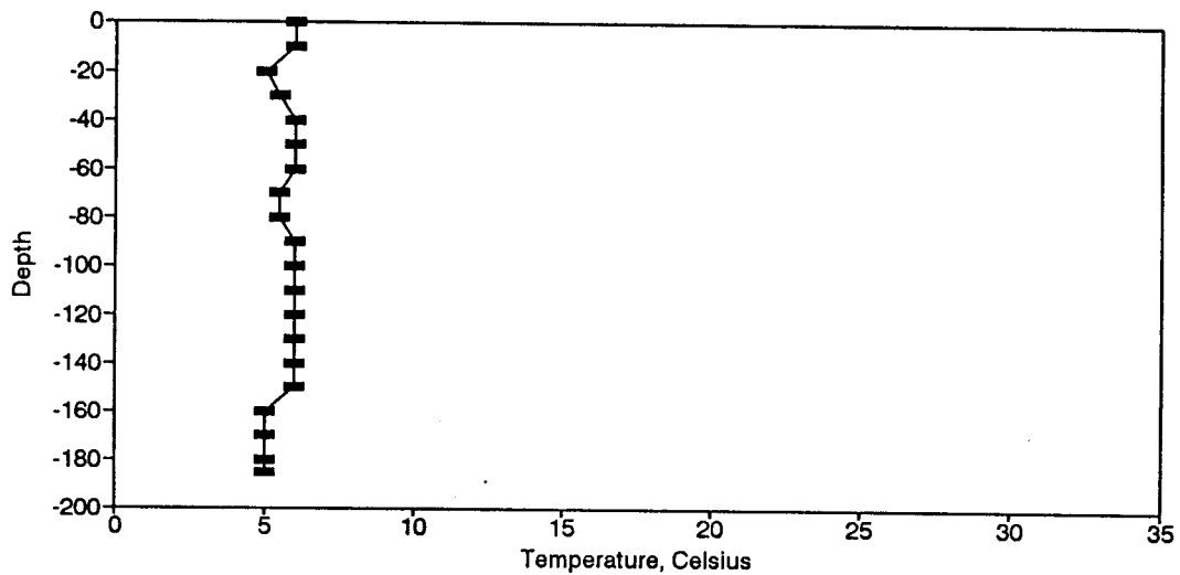
Figure BT25. Temperature Profile for the Eureka Springs Site-January 20, 1976.
