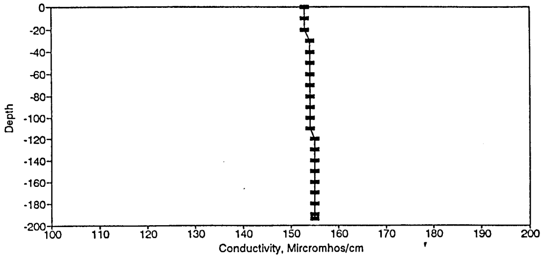
Figure BC97. Conductivity Profile for the Eureka Springs Site-February 16, 1982.
