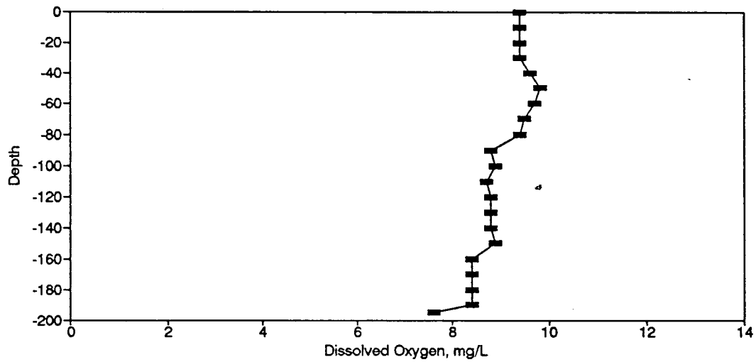
Figure BD5. Dissolved Oxygen Profile for the Eureka Springs Site-April 16, 1974.
