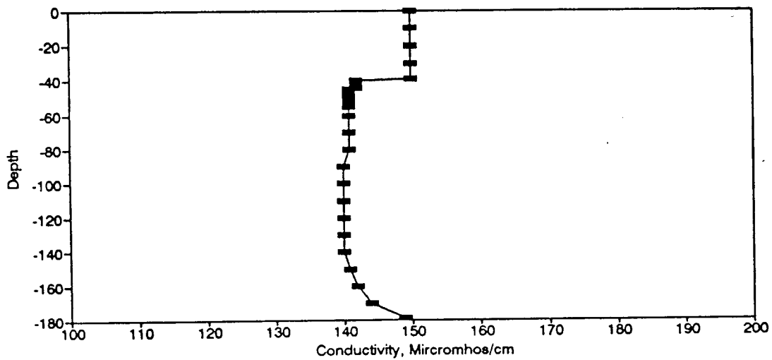
Figure BC81. Conductivity Profile for the Eureka Springs Site - September 16, 1980.
