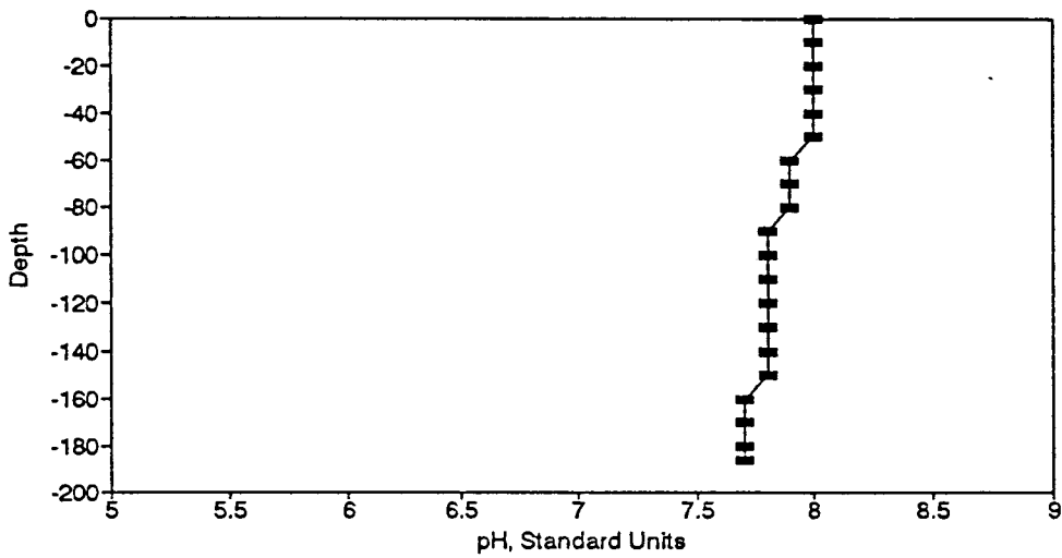
Figure BP86. pH Profile for the Eureka Springs Site-March 3, 1981.
