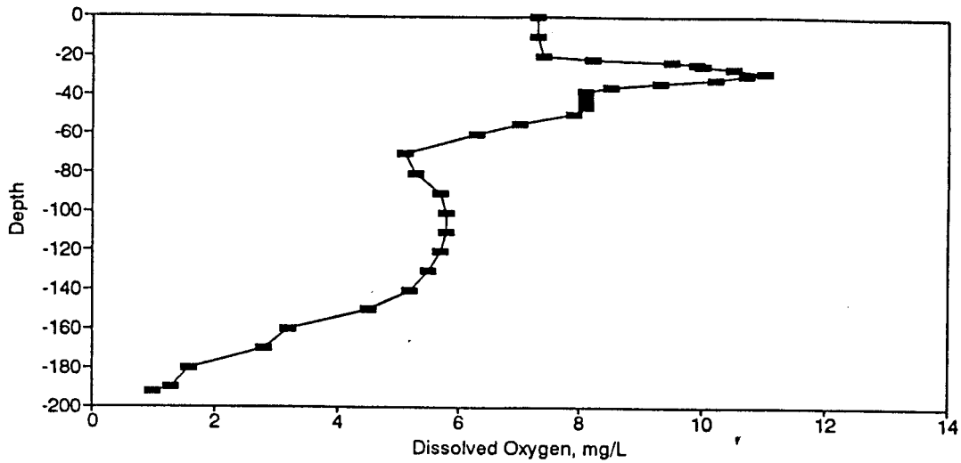
Figure BD115. Dissolved Oxygen Profile for the Eureka Springs Site-August 17, 1983.
