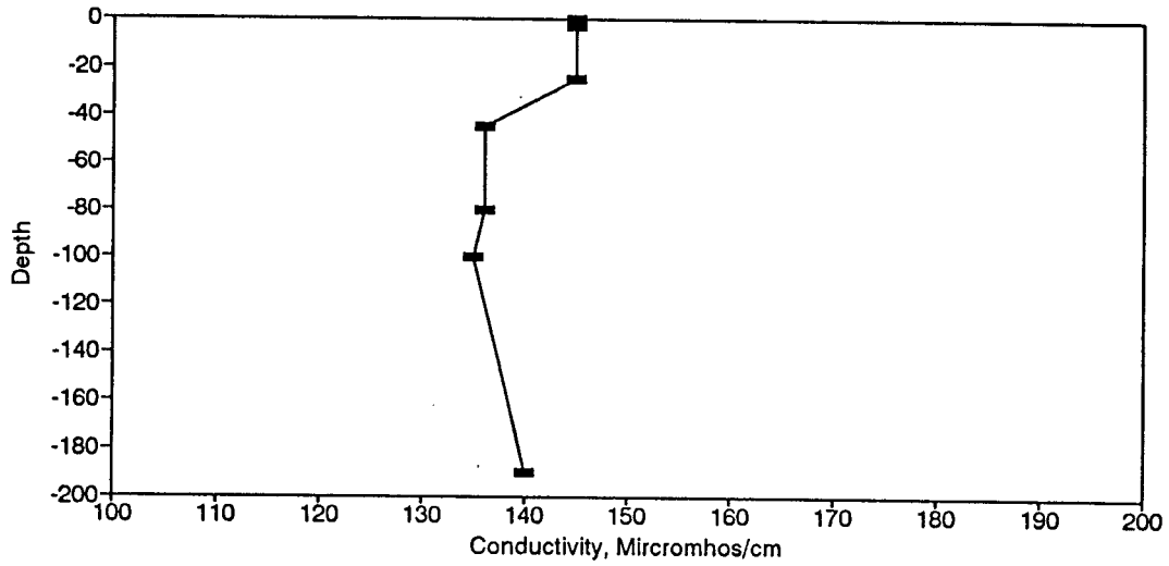
Figure BC163. Conductivity Profile for the Eureka Springs Site-August 19, 1987.
