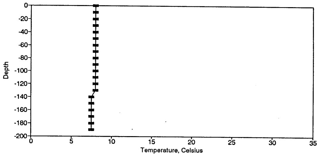
Figure BT13. Temperature Profile for the Eureka Springs Site-January 21, 1975.
