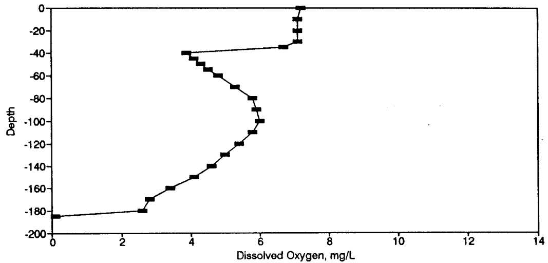
Figure BD21. Dissolved Oxygen Profile for the Eureka Springs Site-September 17, 1975.
