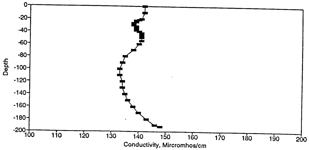
Figure BC115. Conductivity Profile for the Eureka Springs Site-August 17, 1983.
