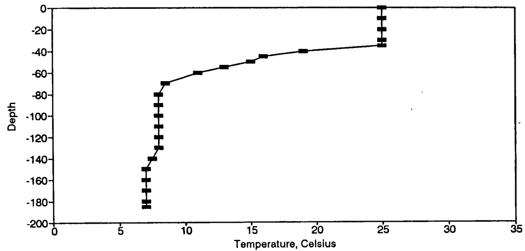
Figure BT21. Temperature Profile for the Eureka Springs Site-September 17, 1975.
