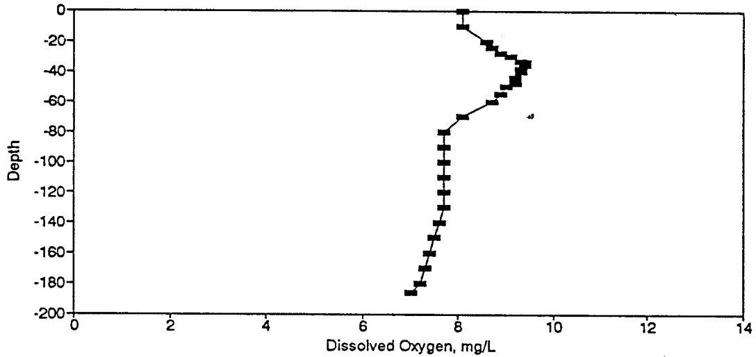
Figure BD101. Dissolved Oxygen Profile for the Eureka Springs Site-June 22, 1982.
