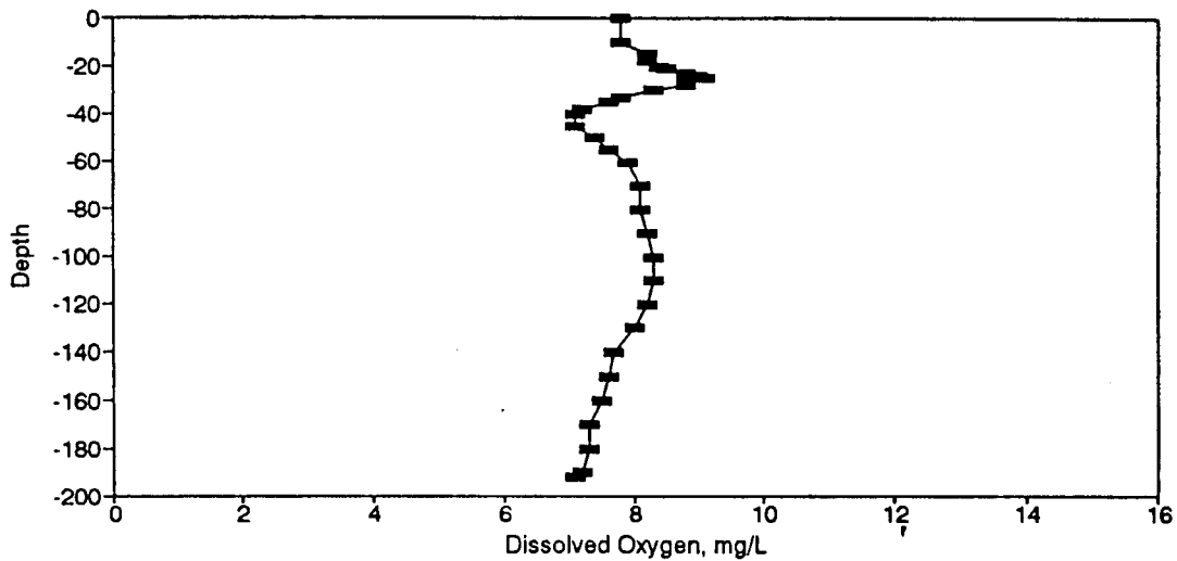
Figure BD67. Dissolved Oxygen Profile for the Eureka Springs Site-July 17, 1979.
