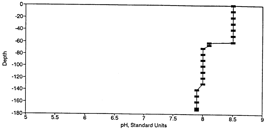
Figure BP118. pH Profile for the Eureka Springs Site-November 14, 1983.
