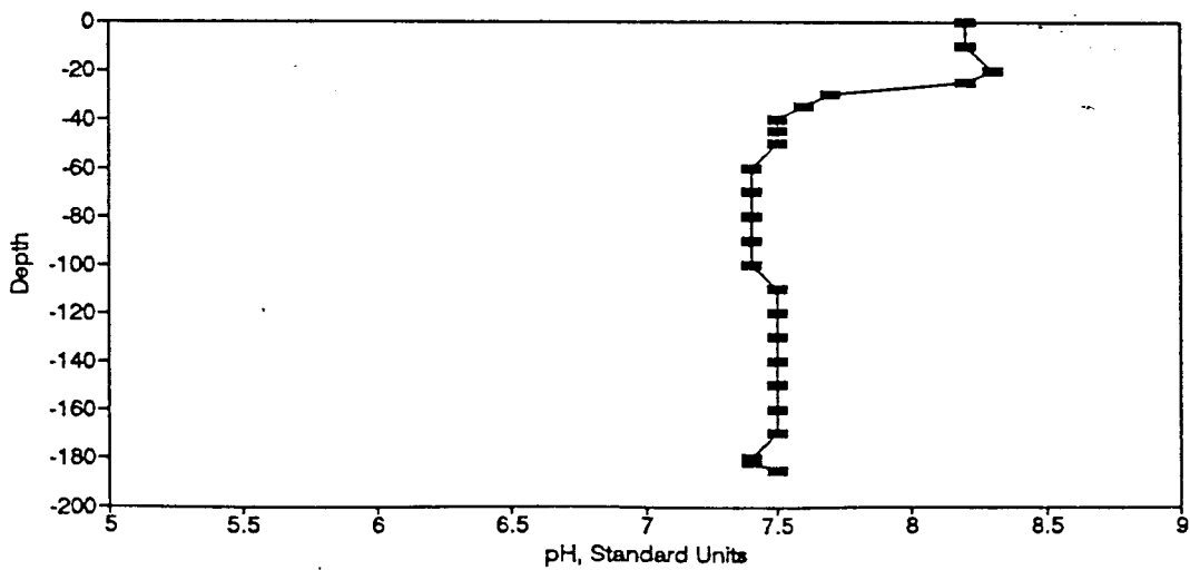
Figure BP45. pH Profile for the Eureka Springs Site-August 22, 1977.
