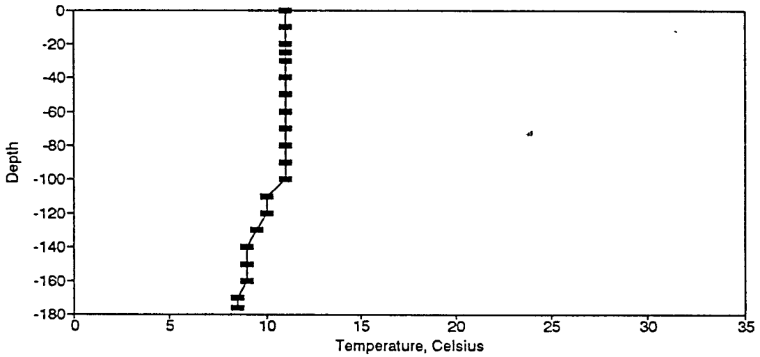
Figure BT119. Temperature Profile for the Eureka Springs Site-December 7, 1983.
