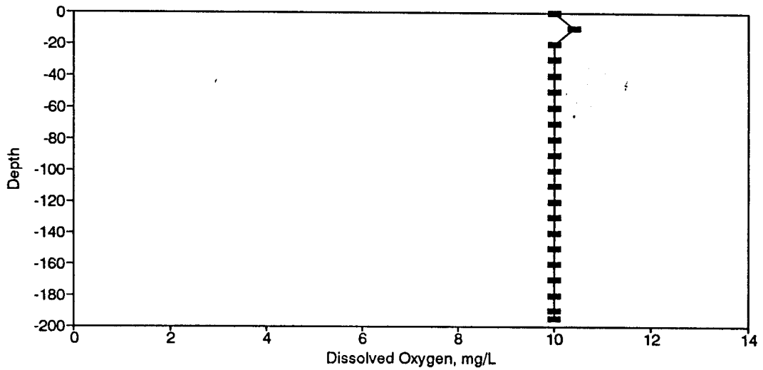
Figure BD14. Dissolved Oxygen Profile for the Eureka Springs Site-February 18, 1975.
