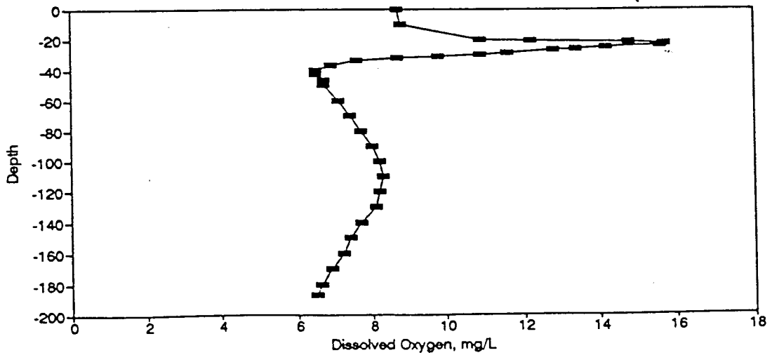
Figure BD174. Dissolved Oxygen Profile for the Eureka Springs Site-July 12, 1988.
