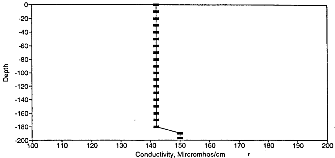
Figure BC109. Conductivity Profile for the Eureka Springs Site-February 11, 1983.
