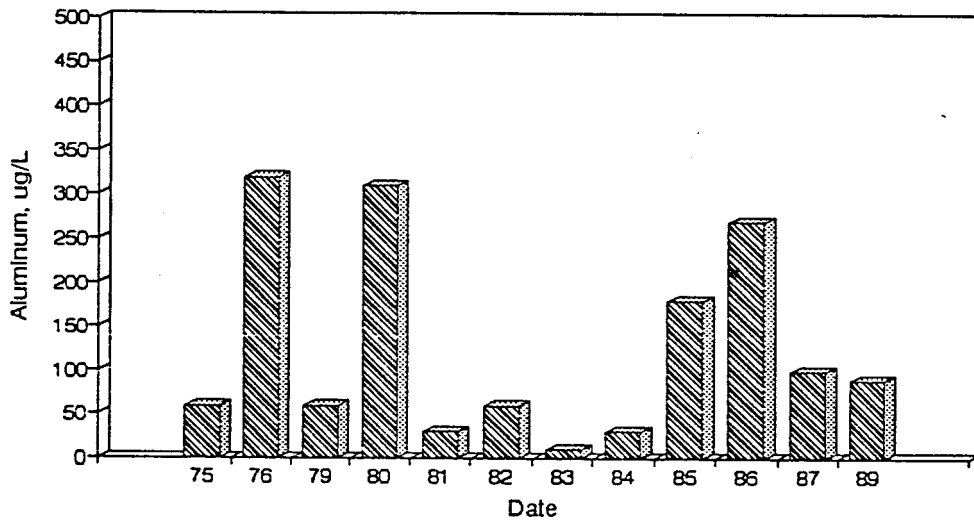
Figure A41. Graph of Aluminum vs. Time for the White River Site-Aug.
