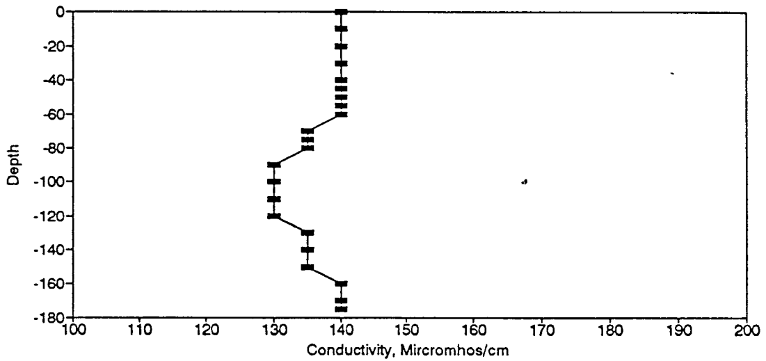
Figure BC59. Conductivity Profile for the Eureka Springs Site-November 7, 1978.
