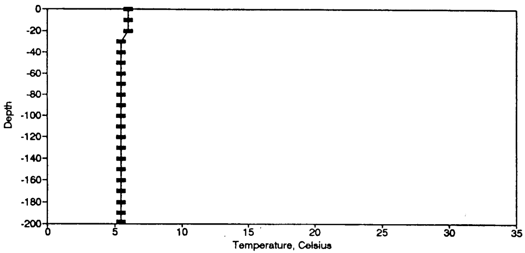
Figure BT169. Temperature Profile for the Eureka Springs Site-February 24, 1988.
