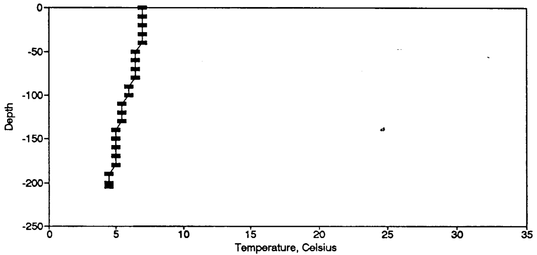
Figure BT134. Temperature Profile for the Eureka Springs Site-March 7, 1985.
