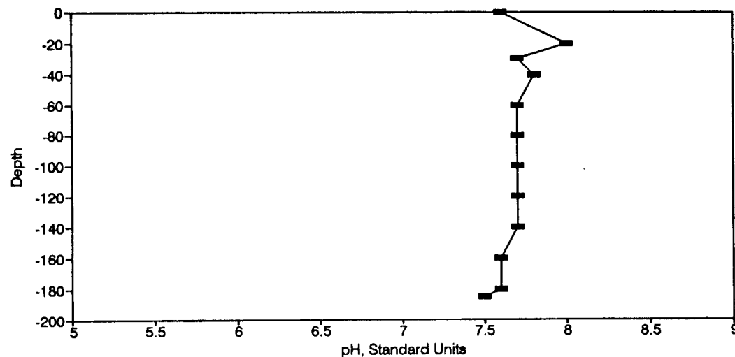
Figure BP18. pH Profile for the Eureka Springs Site-June 11, 1975.
