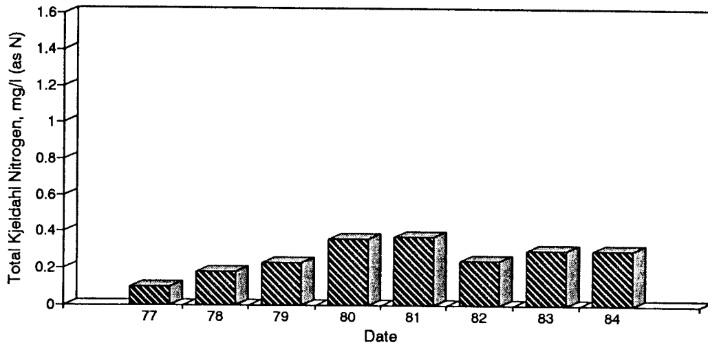
Figure A85. Graph of Total Kjeldahl Nitrogen vs. Time for the White River Site-May.
