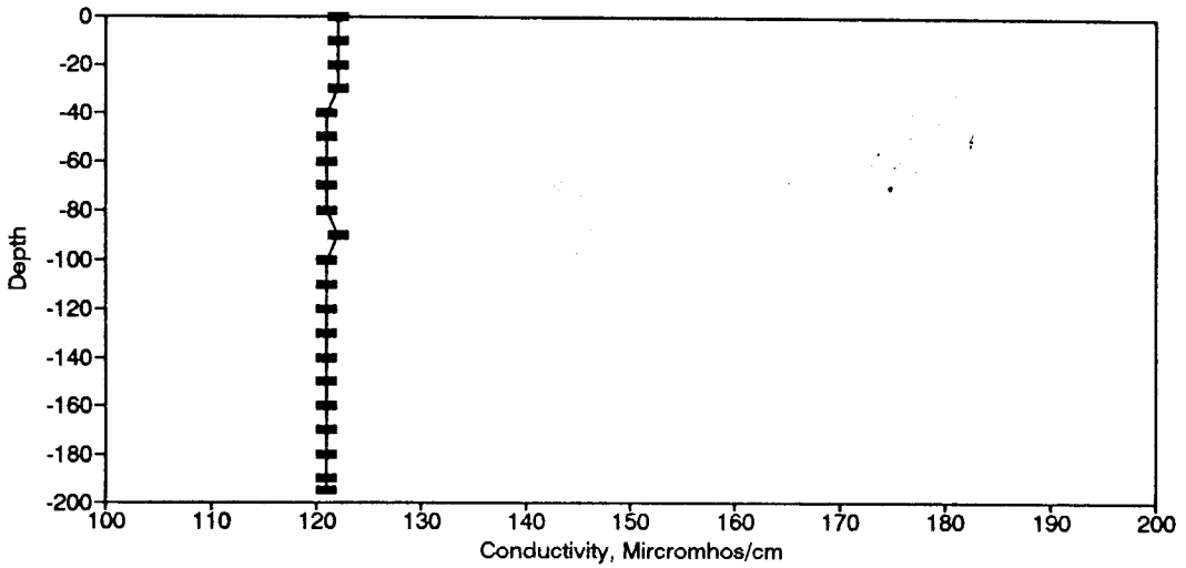
Figure BC14. Conductivity Profile for the Eureka Springs Site - February 18, 1975.
