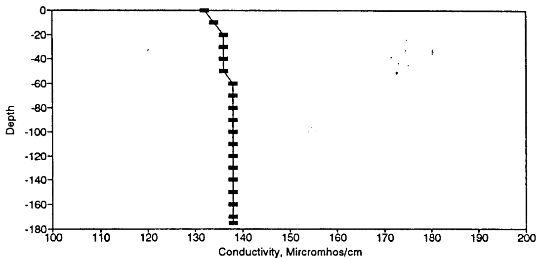
Figure BC62. Conductivity Profile for the Eureka Springs Site-February 14, 1979.
