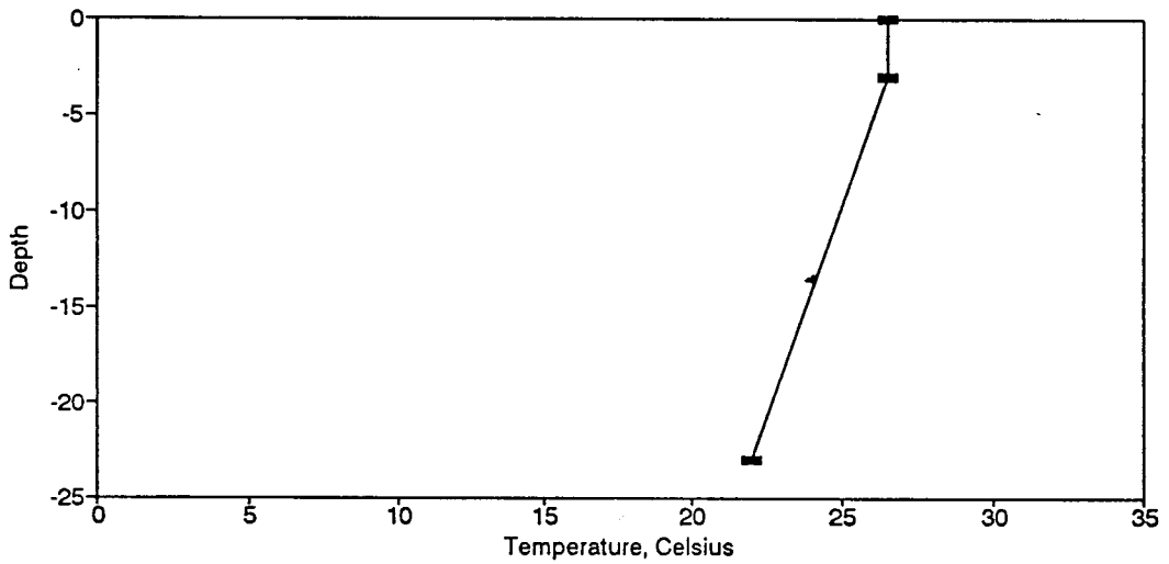
Figure BT161. Temperature Profile for the Eureka Springs Site-June 10, 1987.
