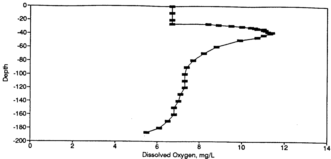
Figure BD79. Dissolved Oxygen Profile for the Eureka Springs Site-July 16, 1980.
