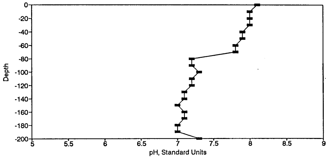
Figure BP3. pH Profile for the Eureka Springs Site-February 20, 1974.
