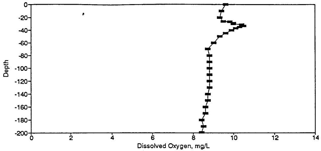
Figure BD184. Dissolved Oxygen Profile for the Eureka Springs Site-June 7, 1989.
