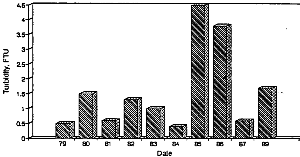
Figure A107. Graph of Turbidity vs. Time for the White River Site-Aug.
