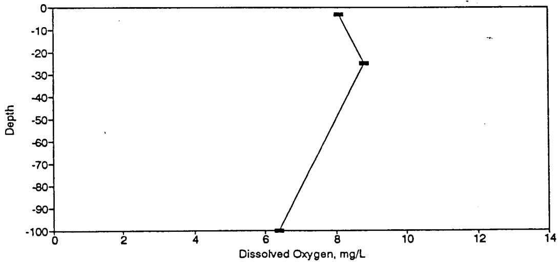
Figure BD186. Dissolved Oxygen Profile for the Eureka Springs Site-August 8, 1989.
