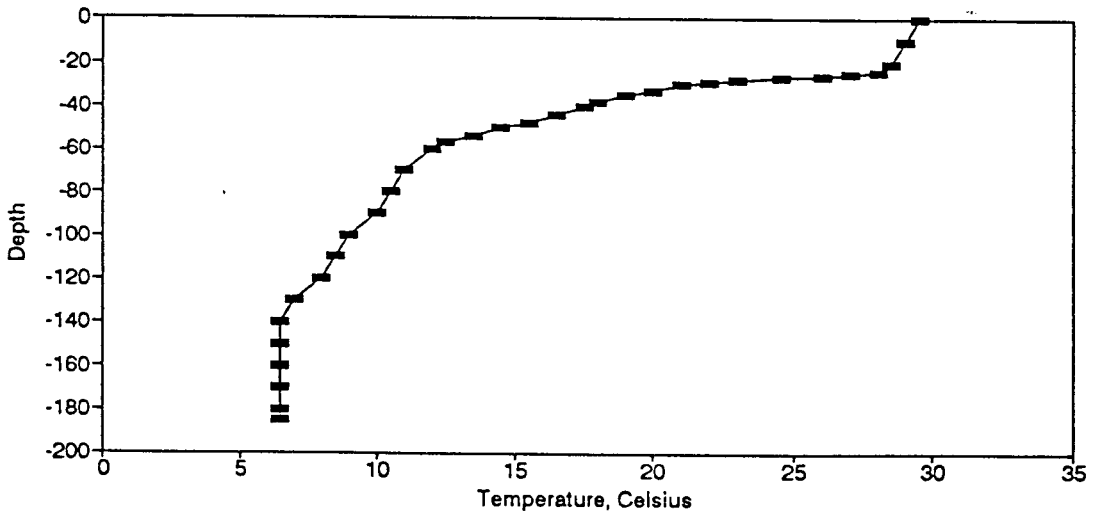
Figure BT102. Temperature Profile for the Eureka Springs Site-July 20, 1982.
