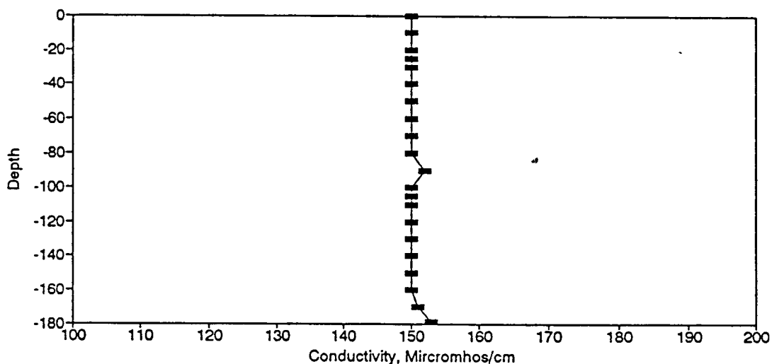
Figure BC95. Conductivity Profile for the Eureka Springs Site-December 9, 1981.
