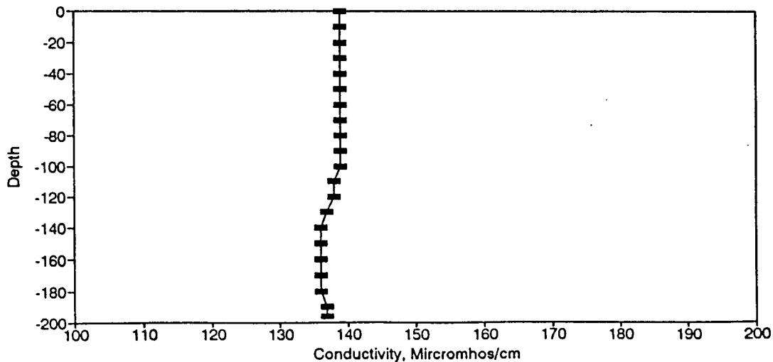
Figure BC111. Conductivity Profile for the Eureka Springs Site-April 21, 1983.
