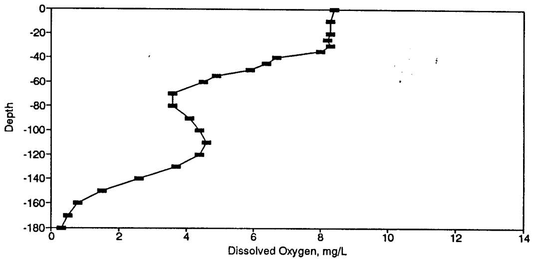
Figure BD32. Dissolved Oxygen Profile for the Eureka Springs Site-August 24, 1976.
