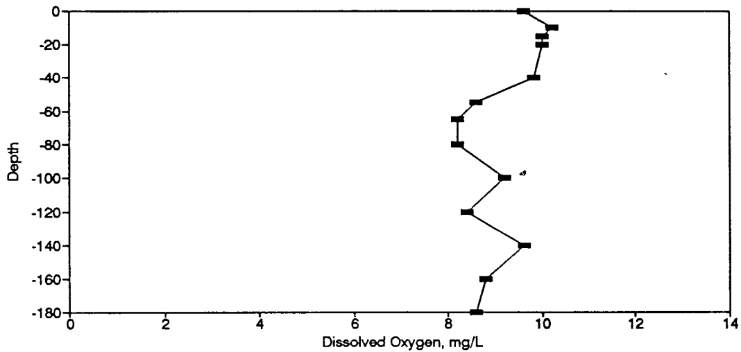
Figure BD29. Dissolved Oxygen Profile for the Eureka Springs Site-May 25, 1976.
