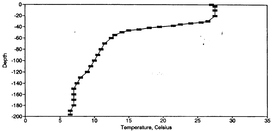
Figure BT140. Temperature Profile for the Eureka Springs Site-September 6, 1985.
