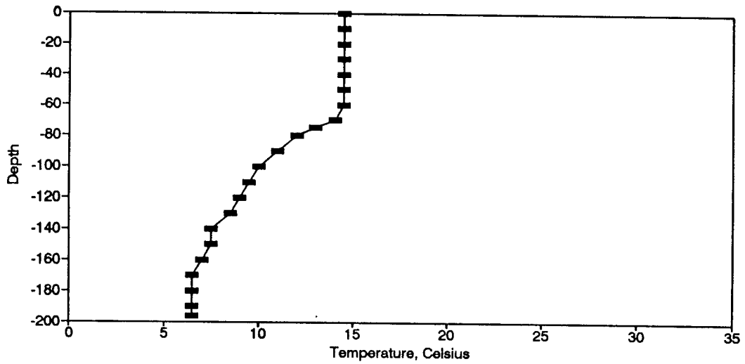
Figure BT130. Temperature Profile for the Eureka Springs Site-November 8, 1984.
