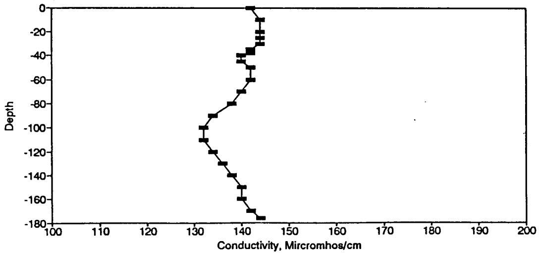
Figure BC57. Conductivity Profile for the Eureka Springs Site-September 28, 1978.
