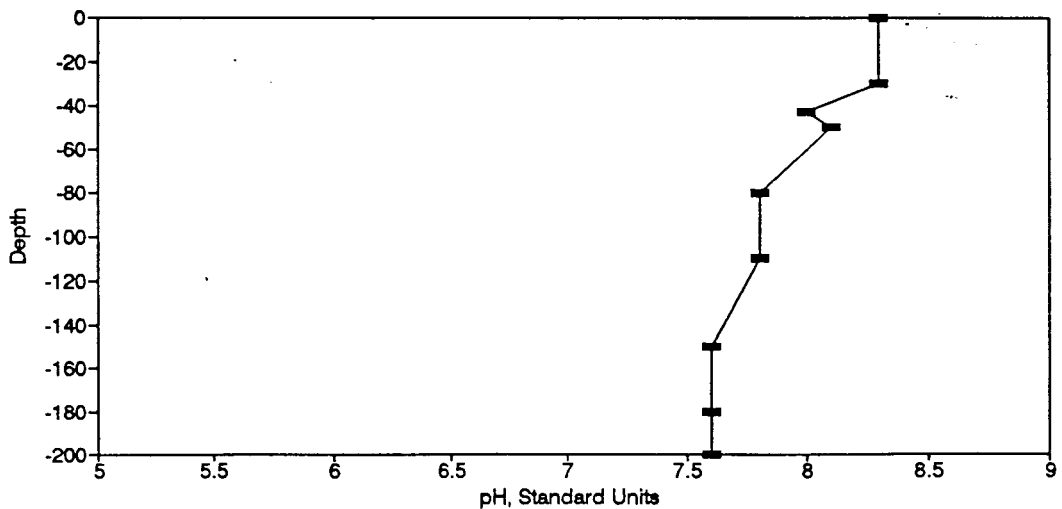
Figure BP6. pH Profile for the Eureka Springs Site-May 14, 1974.
