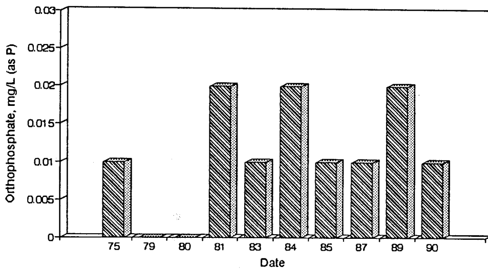
Figure A99. Graph of Orthophosphate vs. Time for the White River Site-Dec.
