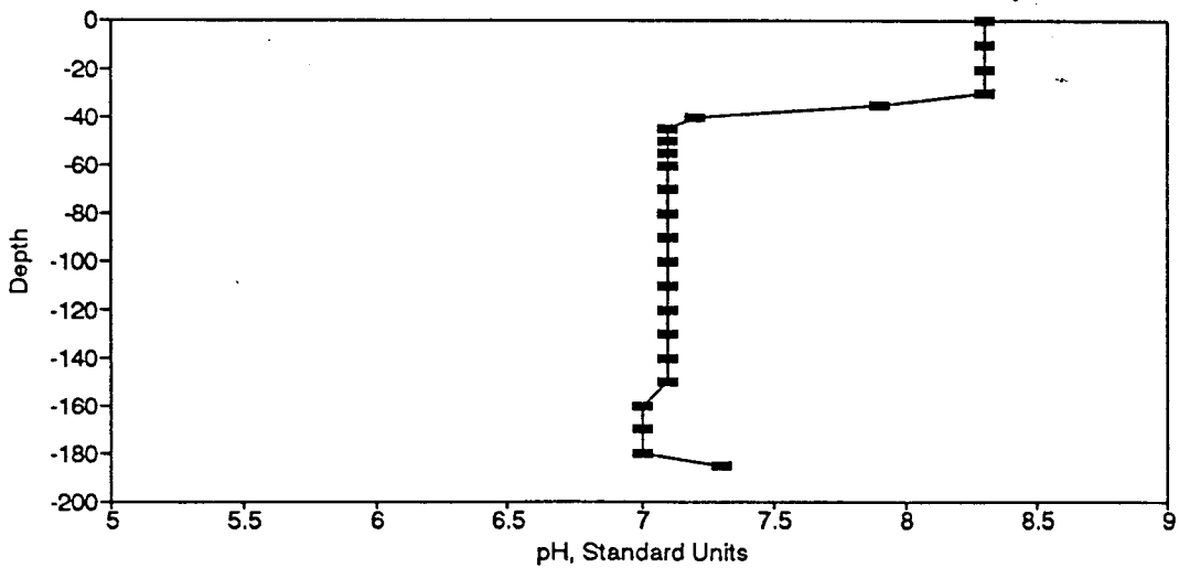
Figure BP21. pH Profile for the Eureka Springs Site-September 17, 1975.
