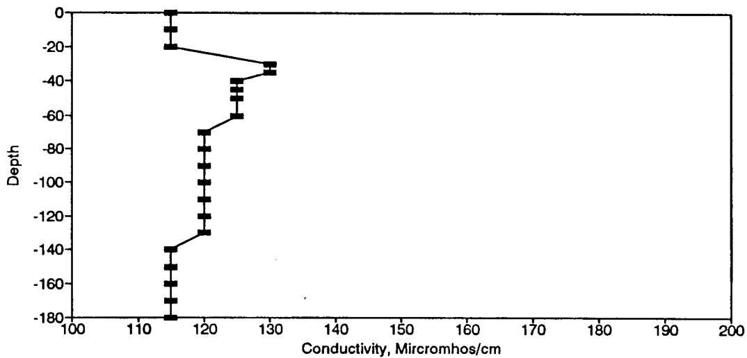
Figure BC31. Conductivity Profile for the Eureka Springs Site-July 23, 1976.
