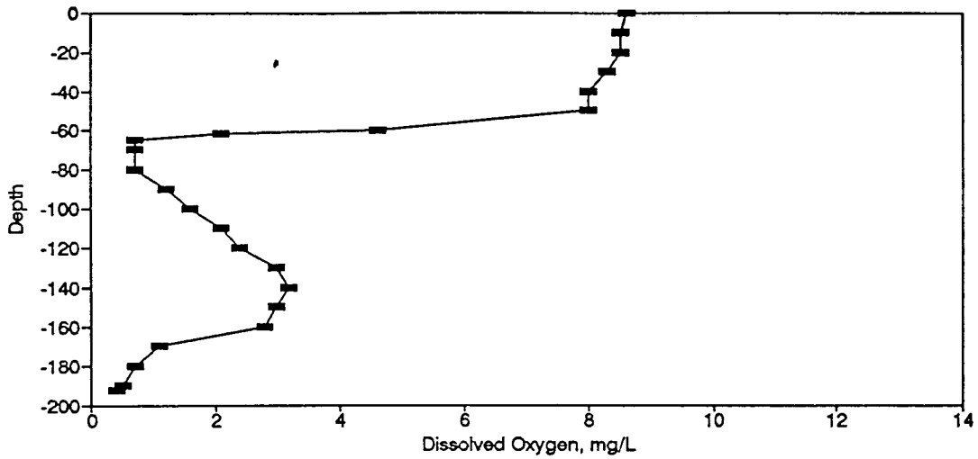
Figure BD142. Dissolved Oxygen Profile for the Eureka Springs Site-November 6, 1985.
