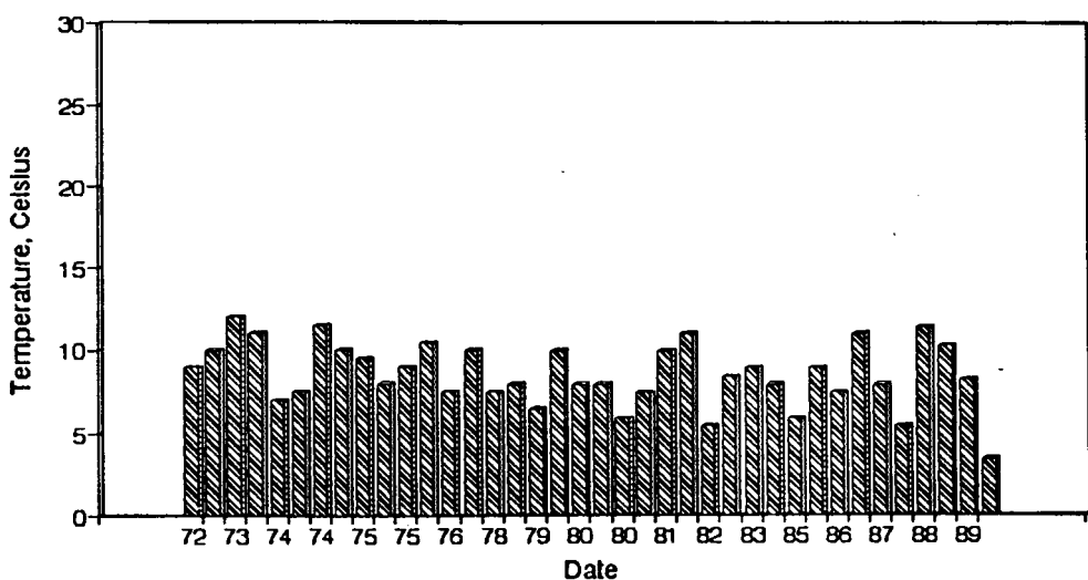
Figure A105. Graph of Temperature vs. Time for the White River Site-Dec.
