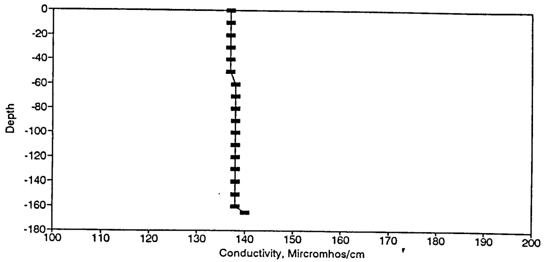
Figure BC121. Conductivity Profile for the Eureka Springs Site-February 29, 1984.
