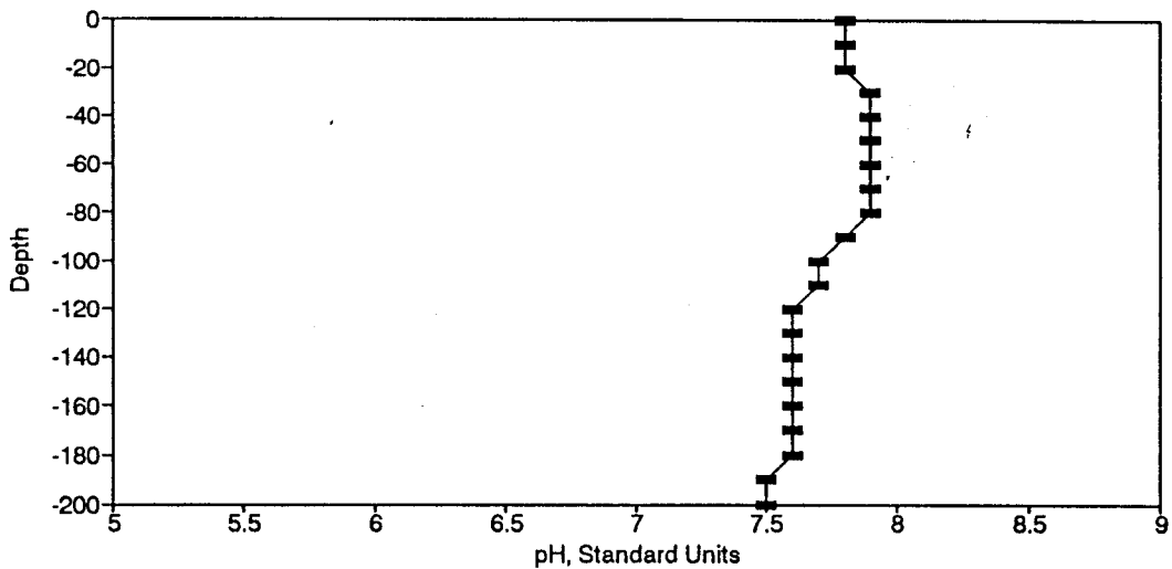
Figure BP2. pH Profile for the Eureka Springs Site-January 15, 1974.
