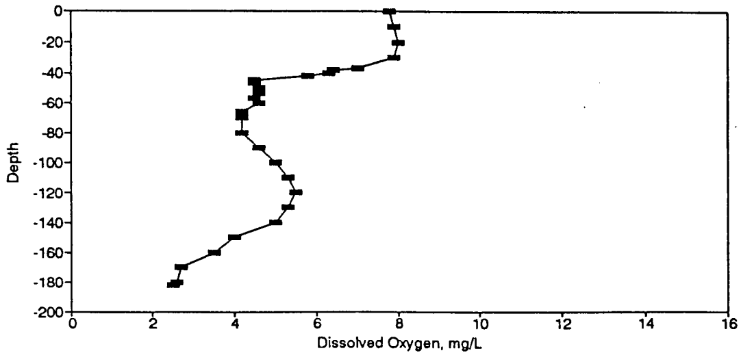
Figure BD69. Dissolved Oxygen Profile for the Eureka Springs Site-September 17, 1979.
