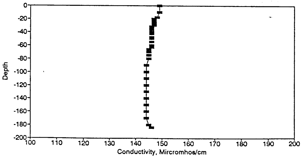
Figure BC90. Conductivity Profile for the Eureka Springs Site-July 14, 1981.
