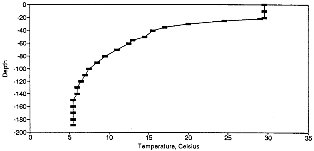
Figure BT55. Temperature Profile for the Eureka Springs Site - July 18, 1978.
