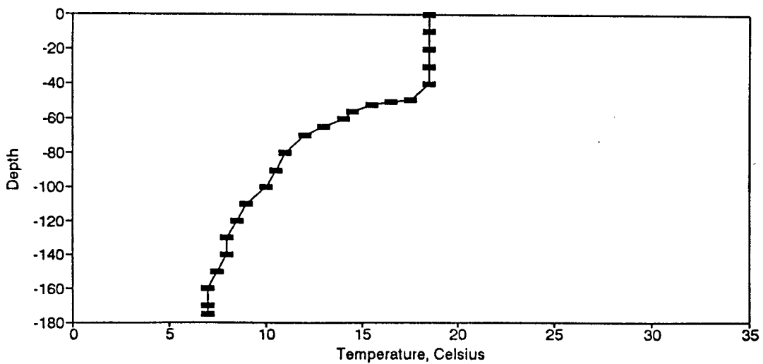
Figure BT105. Temperature Profile for the Eureka Springs Site-October 22, 1982.
