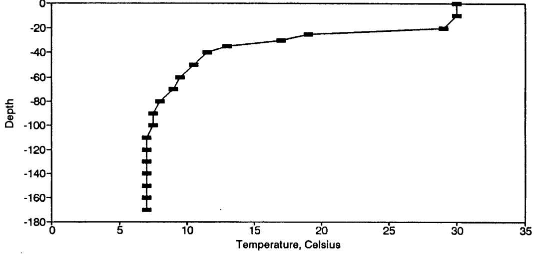
Figure BT19. Temperature Profile for the Eureka Springs Site-July 8, 1975.
