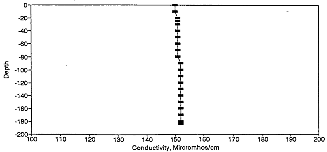
Figure BC108. Conductivity Profile for the Eureka Springs Site-January 25, 1983.
