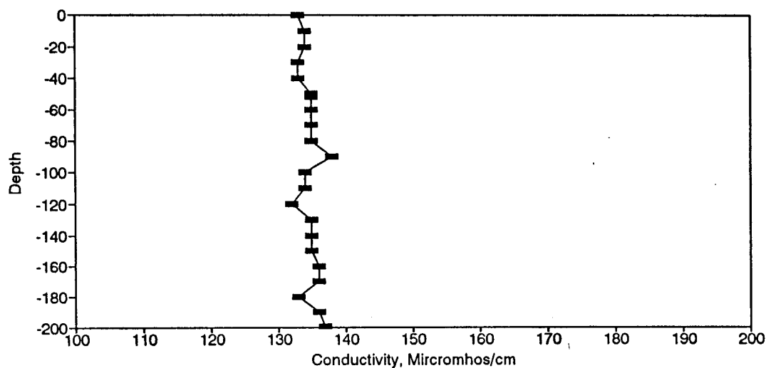
Figure BC159. Conductivity Profile for the Eureka Springs Site-April 15, 1987.
