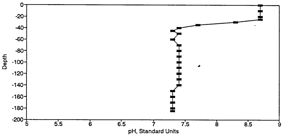
Figure BP20. pH Profile for the Eureka Springs Site-August 13, 1975.
