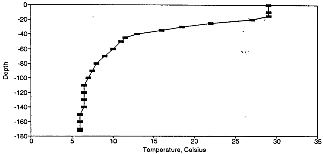
Figure BT44. Temperature Profile for the Eureka Springs Site-July 26, 1977.
