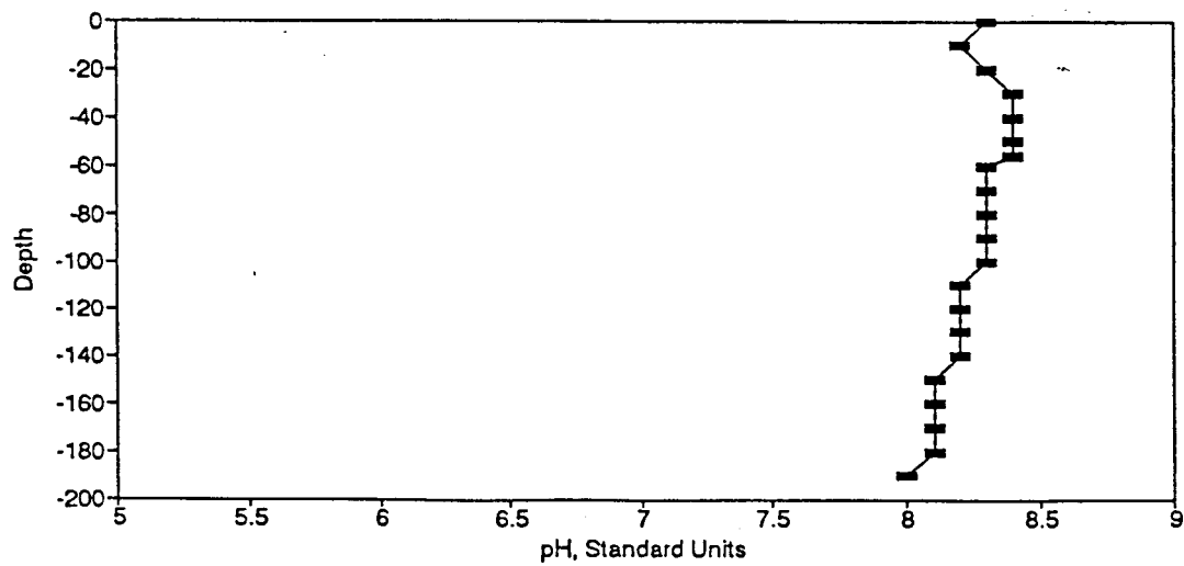
Figure BP123. pH Profile for the Eureka Springs Site-April 24, 1984.
