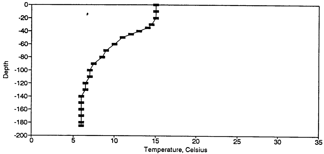
Figure BT28. Temperature Profile for the Eureka Springs Site-April 20, 1976.
