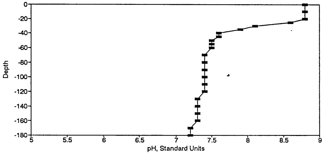
Figure BP32. pH Profile for the Eureka Springs Site-August 24, 1976.
