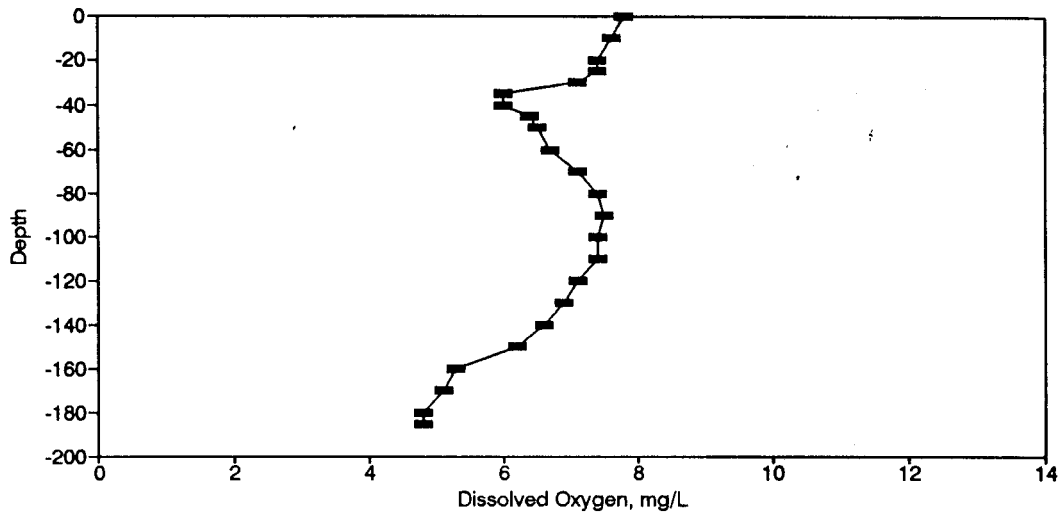
Figure BD20. Dissolved Oxygen Profile for the Eureka Springs Site-August 13, 1975.
