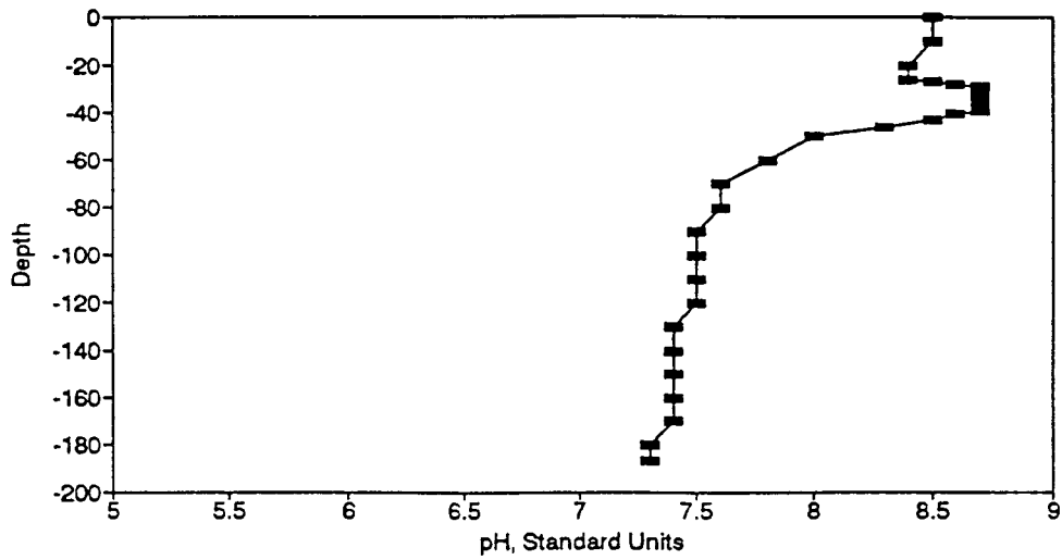
Figure BP79. pH Profile for the Eureka Springs Site-July 16, 1980.
