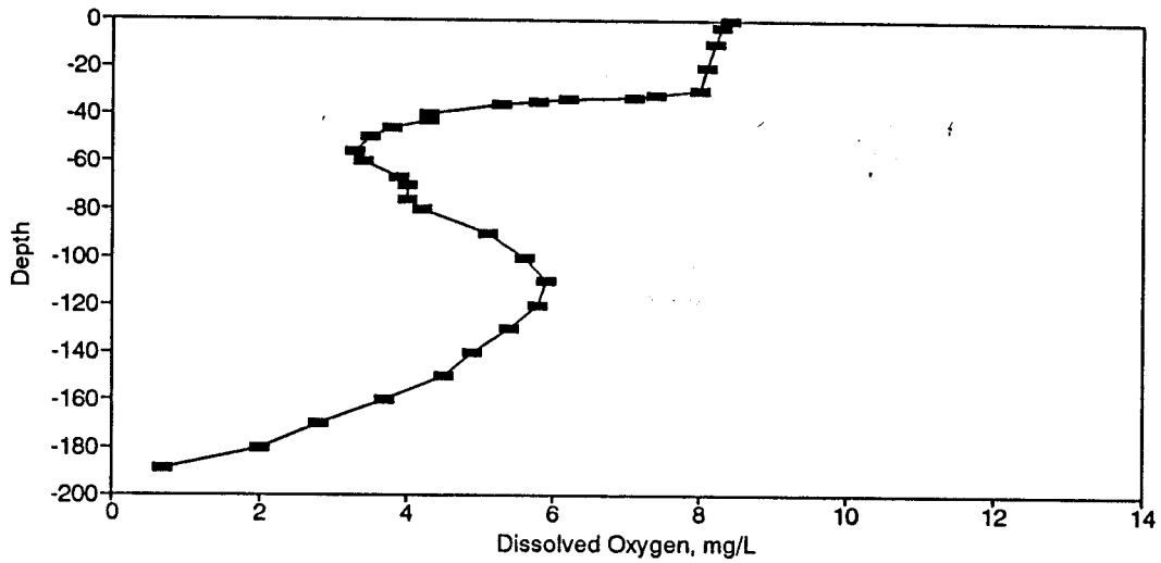
Figure BD152. Dissolved Oxygen Profile for the Eureka Springs Site-September 4, 1986.
