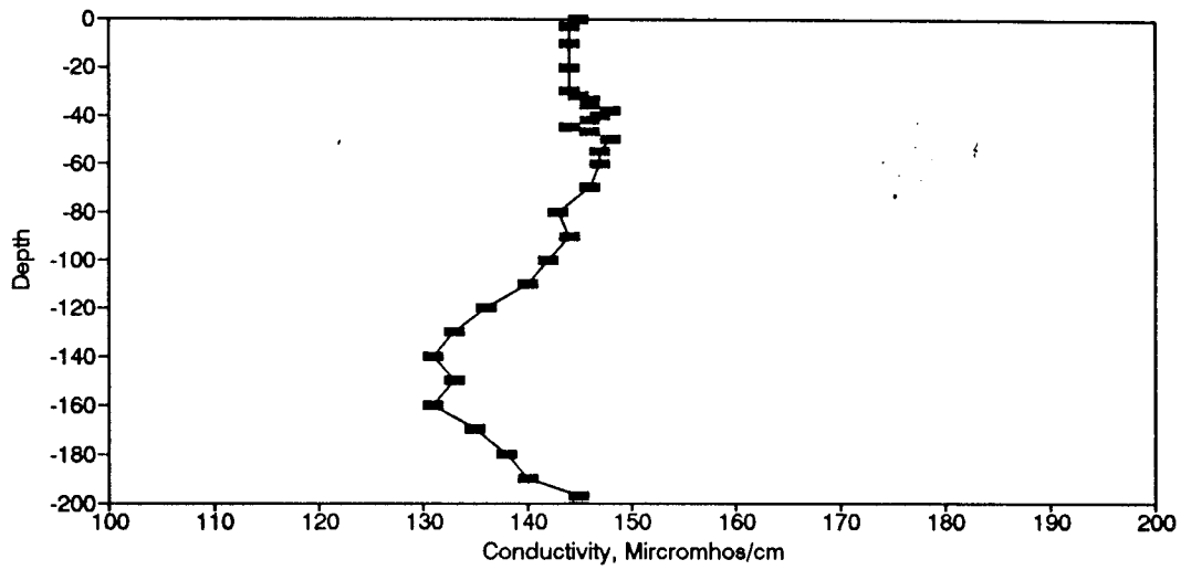
Figure BC140. Conductivity Profile for the Eureka Springs Site-September 6, 1985.
