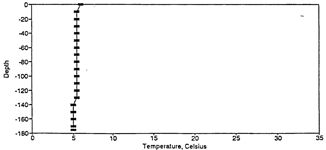
Figure BT96. Temperature Profile for the Eureka Springs Site-January 26, 1982.
