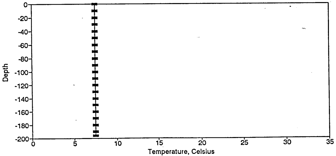
Figure BT144. Temperature Profile for the Eureka Springs Site-Januaray 8, 1986.
