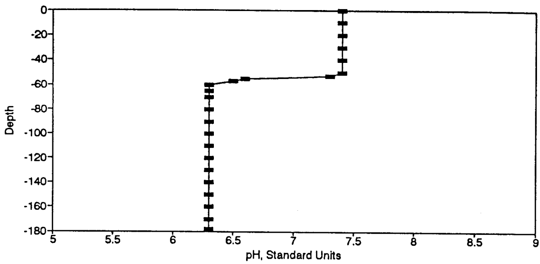
Figure BP58. pH Profile for the Eureka Springs Site-October 10, 1978.
