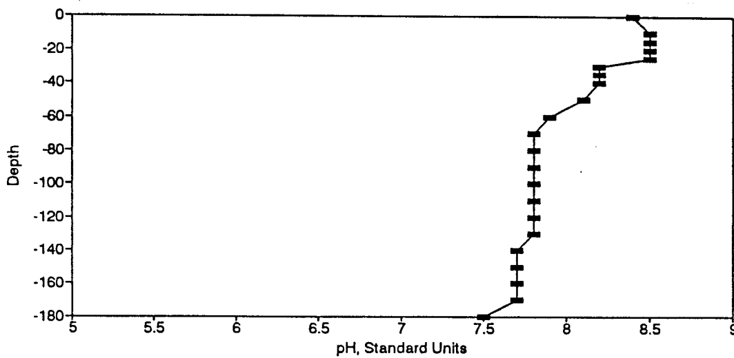
Figure BP42. pH Profile for the Eureka Springs Site-May 31, 1977.
