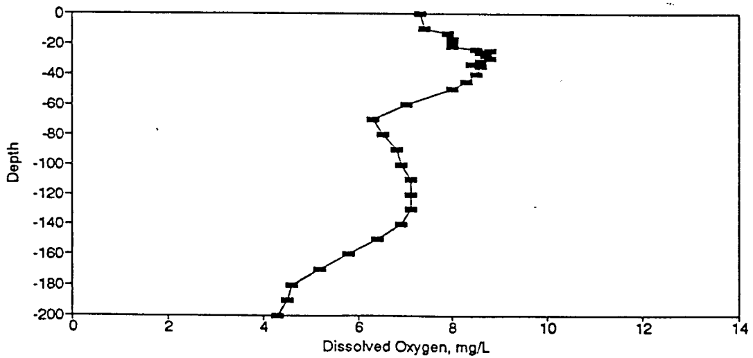
Figure BD114. Dissolved Oxygen Profile for the Eureka Springs Site-July 12, 1983.
