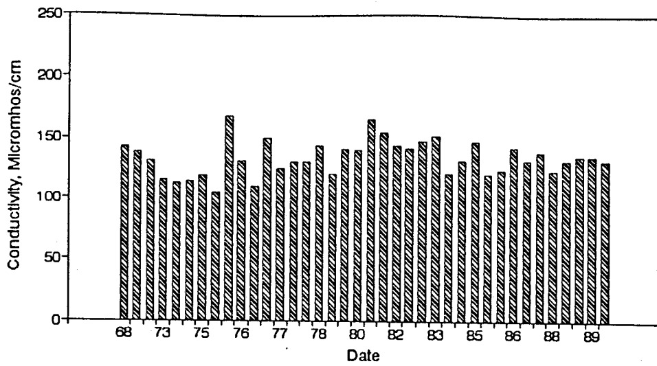
Figure A13. Graph of Conductivity vs. Time for the White River Site-May.
