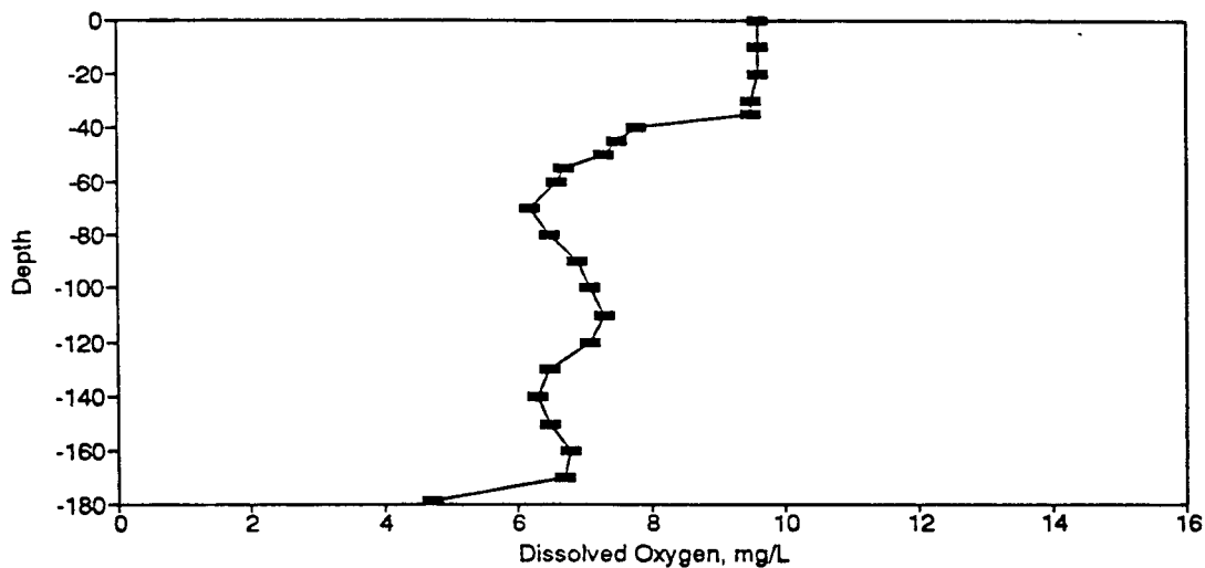
Figure BD47. Dissolved Oxygen Profile for the Eureka Springs Site-October 12, 1977.
