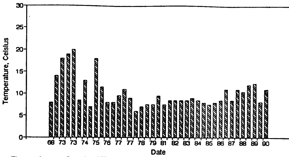
Figure A103. Graph of Temperature vs. Time for the White River Site-May.
