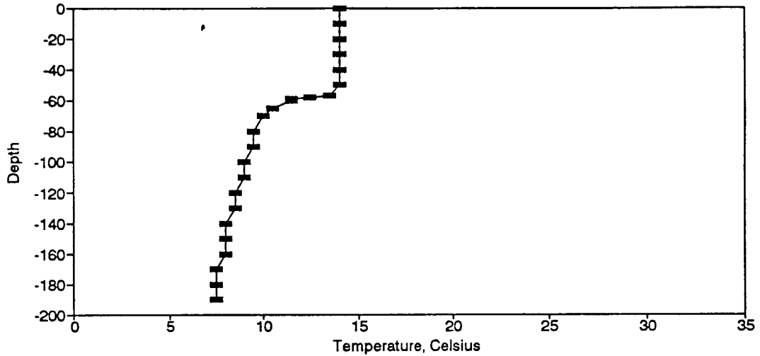
Figure BT166. Temperature Profile for the Eureka Springs Site-November 12, 1987.
