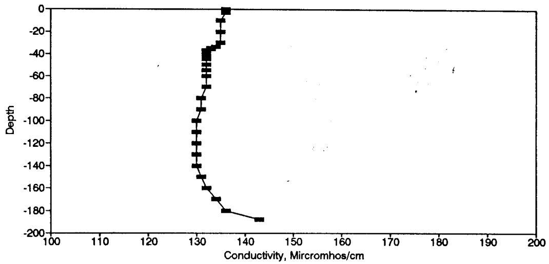
Figure BC128. Conductivity Profile for the Eureka Springs Site-September 18, 1984.
