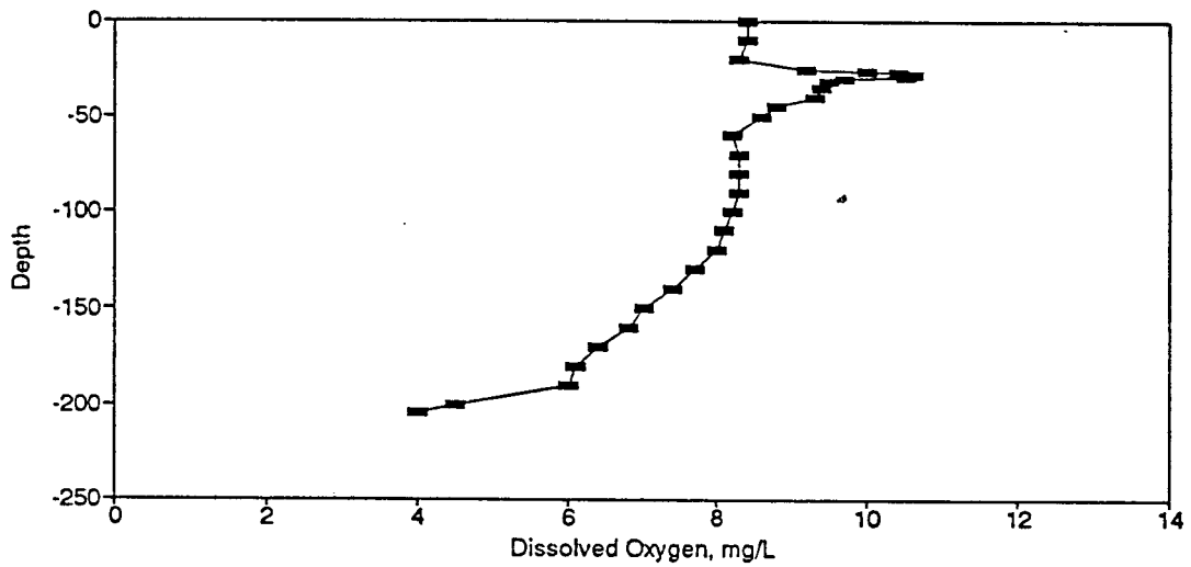
Figure BD113. Dissolved Oxygen Profile for the Eureka Springs Site-June 14, 1983.
