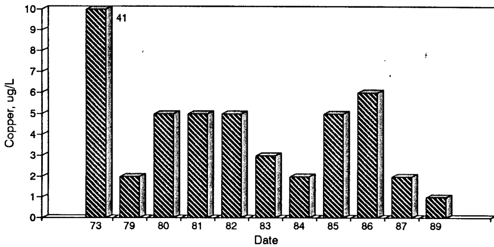
Figure A50. Graph of Copper vs. time for the White River Site-Aug.
