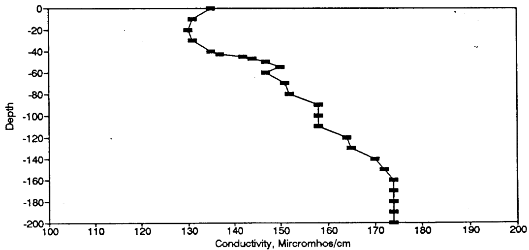
Figure BC6. Conductivity Profile for the Eureka Springs Site-May 14, 1974.
