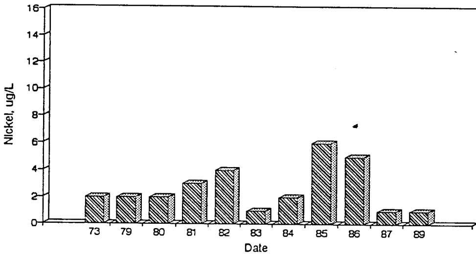
Figure A65. Graph of Nickel vs. Time for the White River Site-Aug.
