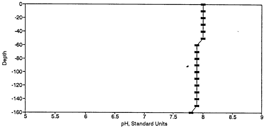
Figure BP38. pH Profile for the Eureka Springs Site-February 7, 1977.
