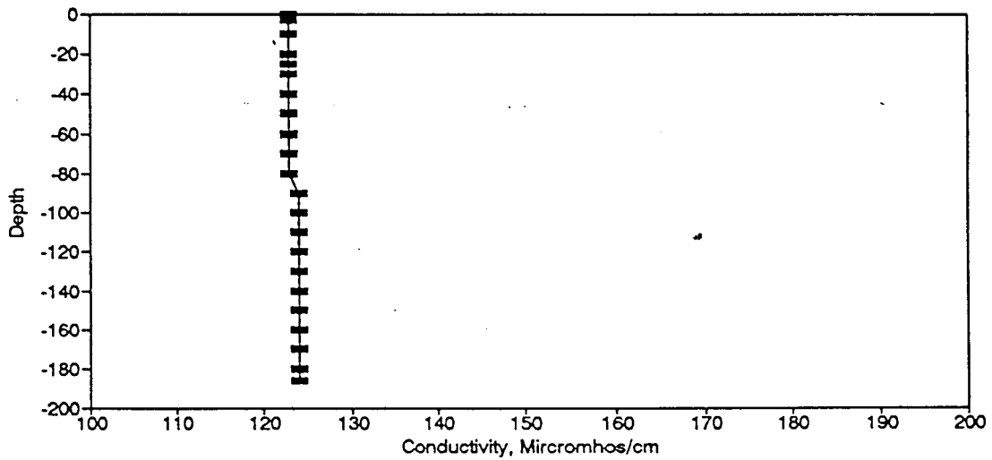
Figure BC143. Conductivity Profile for the Eureka Springs Site-December 19, 1985.
