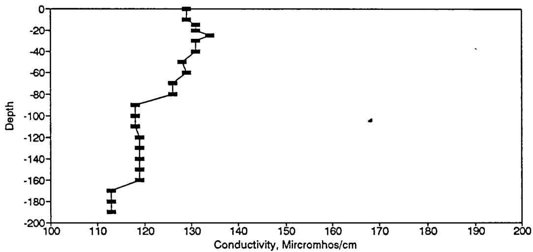
Figure BC17. Conductivity Profile for the Eureka Springs Site-May 14, 1975.
