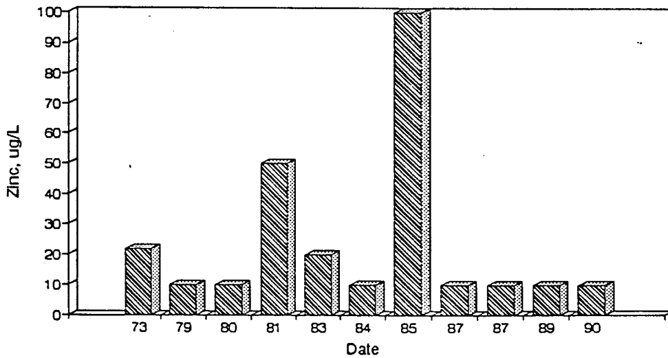
Figure A72. Graph of Zinc vs. Time for the White River Site-Dec.
