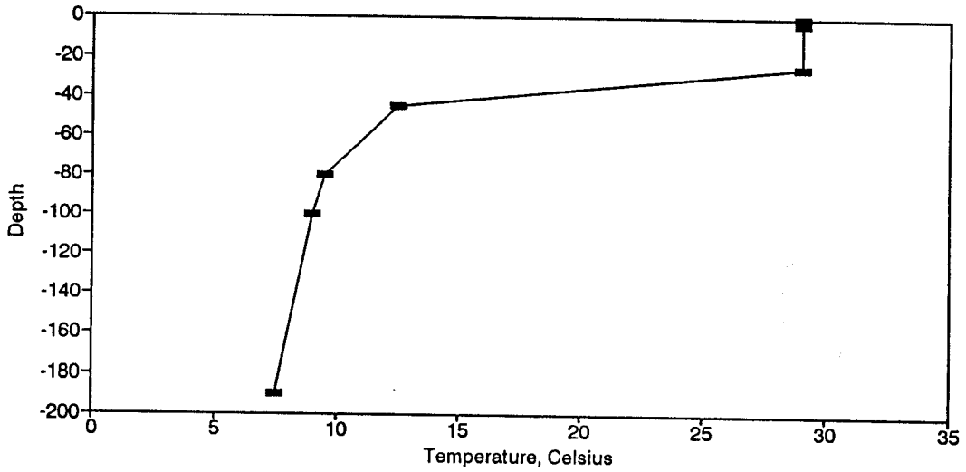
Figure BT163. Temperature Profile for the Eureka Springs Site-August 19, 1987.
