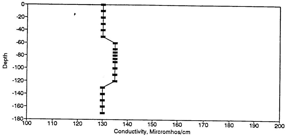
Figure BC40. Conductivity Profile for the Eureka Springs Site-April 5, 1977.
