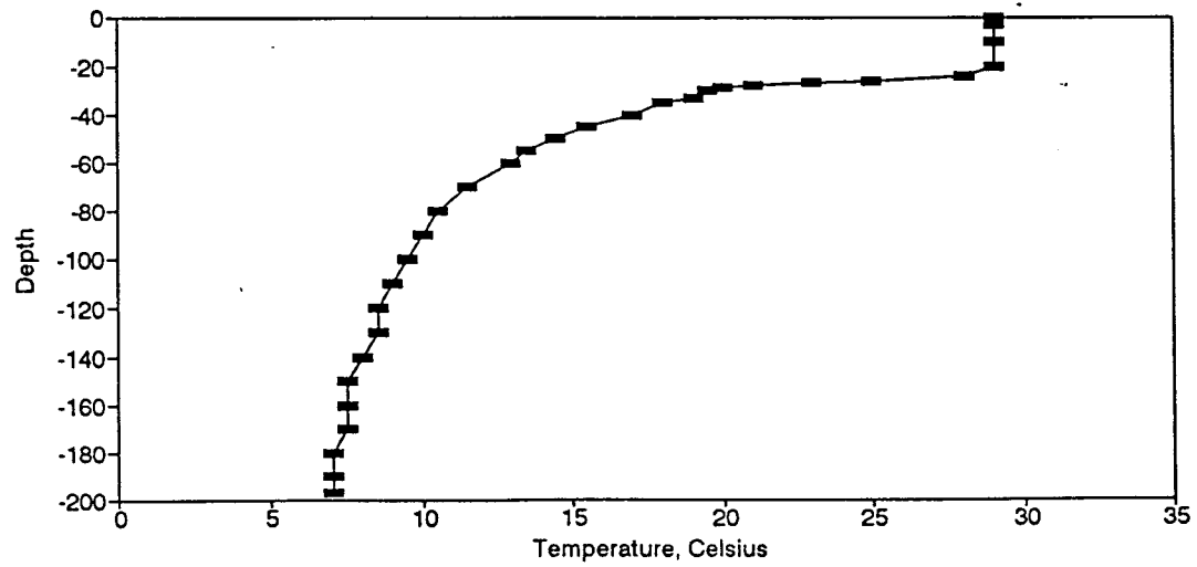
Figure BT150. Temperature Profile for the Eureka Springs Site-July 9, 1986.
