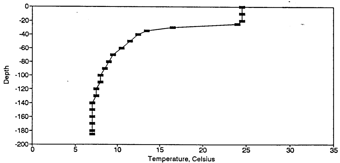
Figure BT18. Temperature Profile for the Eureka Springs Site-June 11, 1975.
