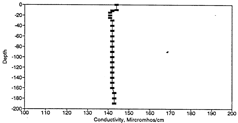
Figure BC77. Conductivity Profile for the Eureka Springs Site-May 7, 1980.
