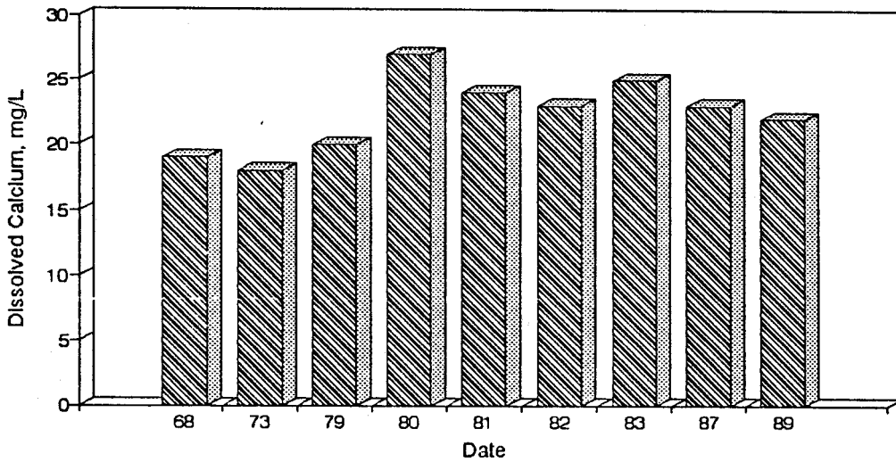
Figure A32. Graph of Dissolved Calcium vs. Time for the White River Site-Aug.
