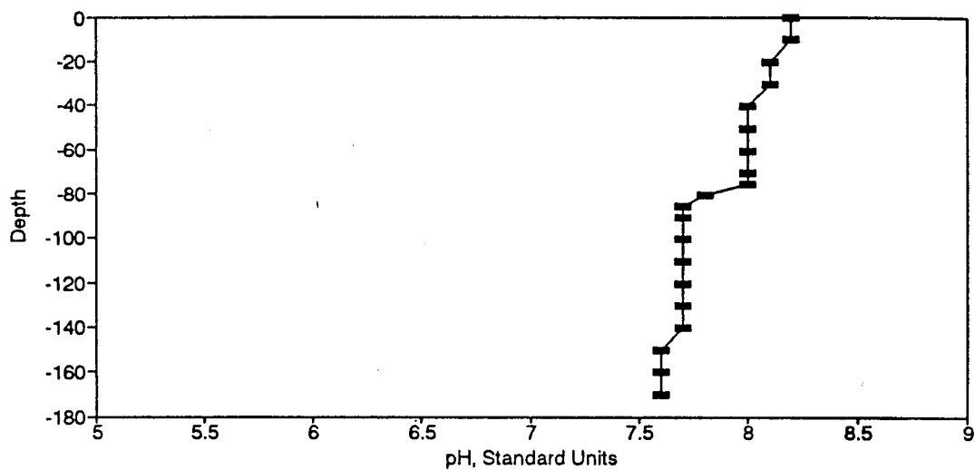
Figure BP40. pH Profile for the Eureka Springs Site-April 5, 1977.
