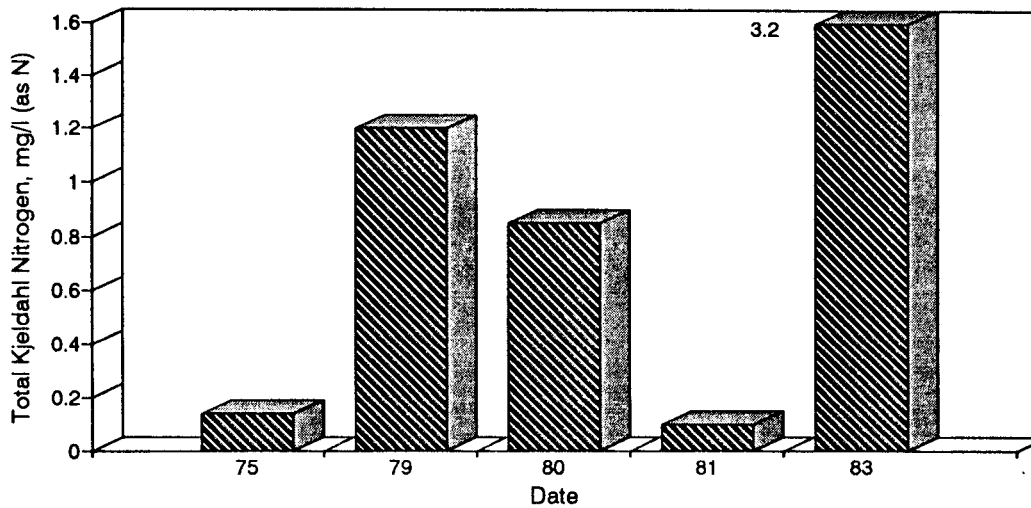
Figure A87. Graph of Total Kjeldahl Nitrogen vs. Time for the White River Site-Dec.
