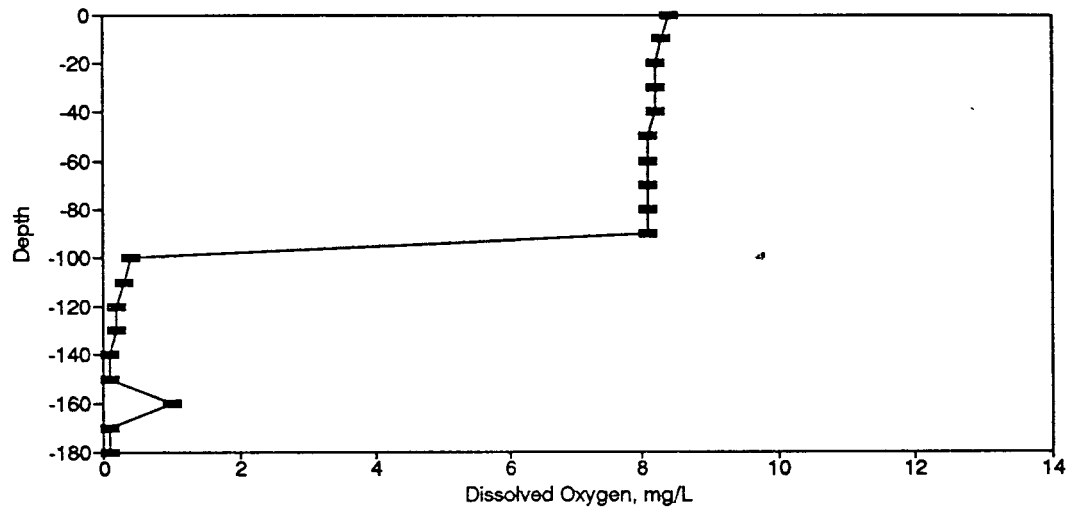
Figure BD35. Dissolved Oxygen Profile for the Eureka Springs Site-November 16, 1976.
