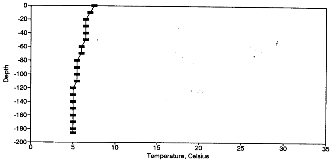
Figure BT86. Temperature Profile for the Eureka Springs Site-March 3, 1981.
