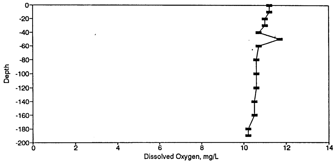
Figure BD26. Dissolved Oxygen Profile for the Eureka Springs Site-February 24, 1976.
