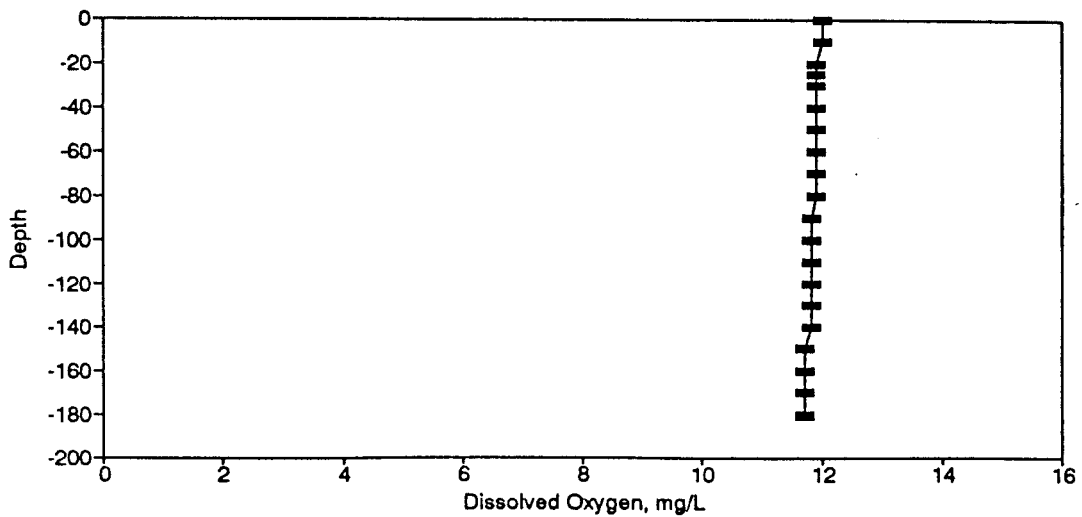
Figure BD63. Dissolved Oxygen Profile for the Eureka Springs Site-March 8, 1979.
