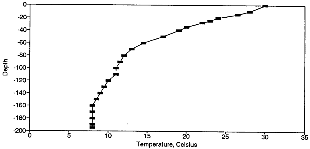
Figure BT7. Temperature Profile for the Eureka Springs Site July 8, 1974.
