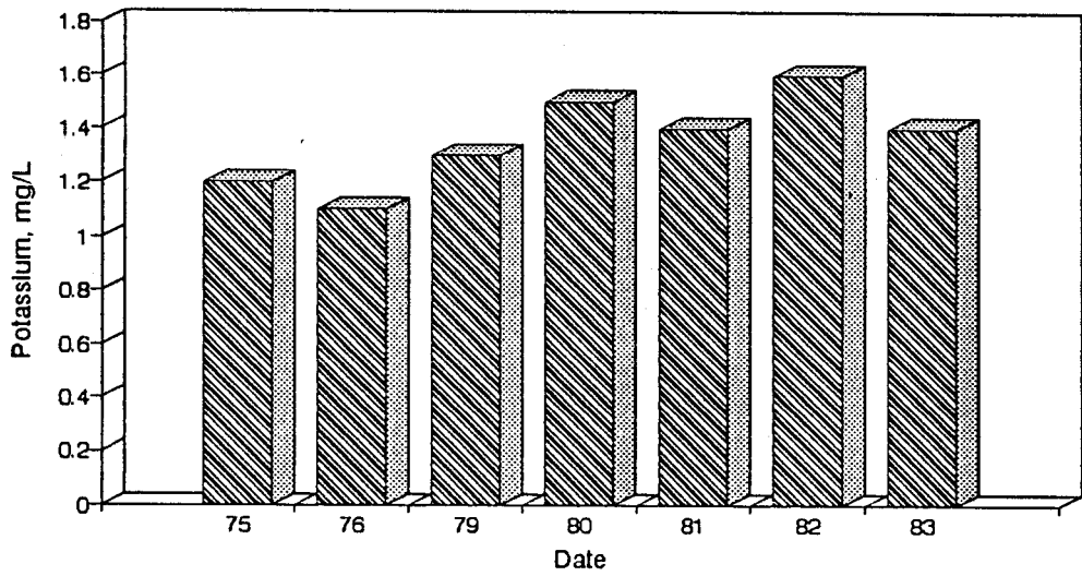
Figure A68. Graph of Potassium vs. Time for the White River Site-Aug.
