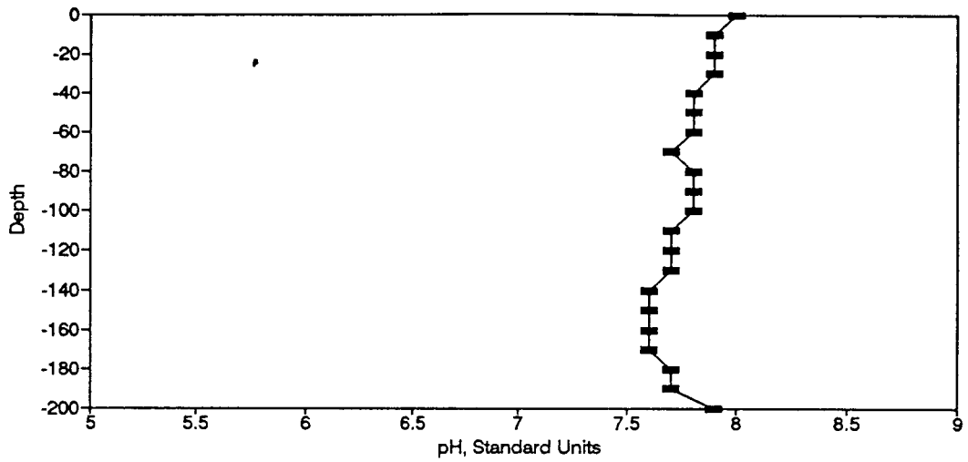
Figure BP4. pH Profile for the Eureka Springs Site-March 19, 1974.
