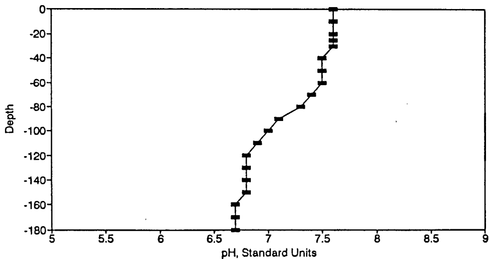
Figure BP84. pH Profile for the Eureka Springs Site-December 10, 1980.
