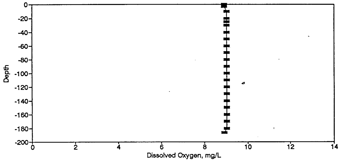
Figure BD143. Dissolved Oxygen Profile for the Eureka Springs Site-December 19, 1985.
