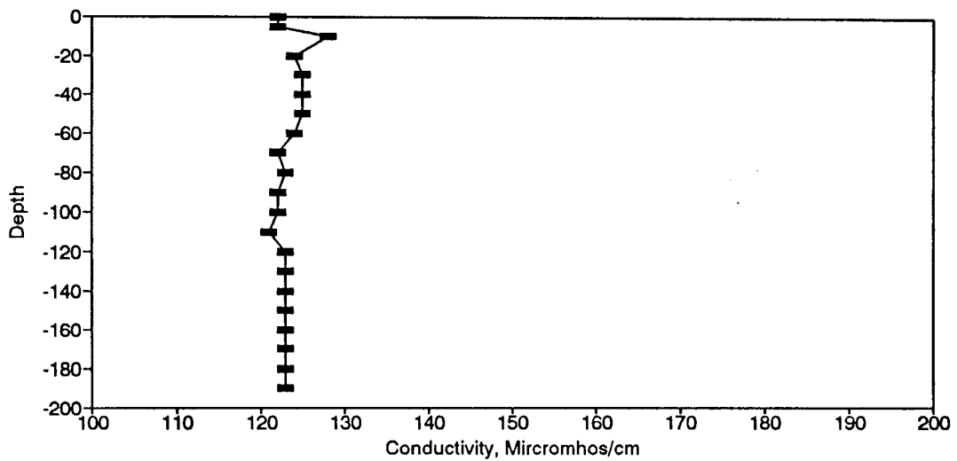
Figure BC27. Conductivity Profile for the Eureka Springs Site-March 23, 1976.
