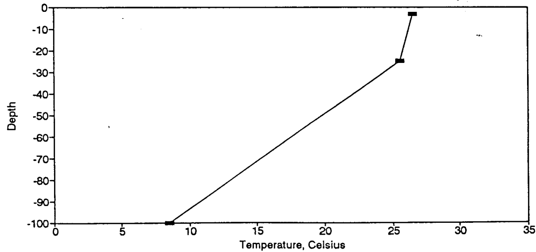
Figure BT186. Temperature Profile for the Eureka Springs Site-August 8, 1989.
