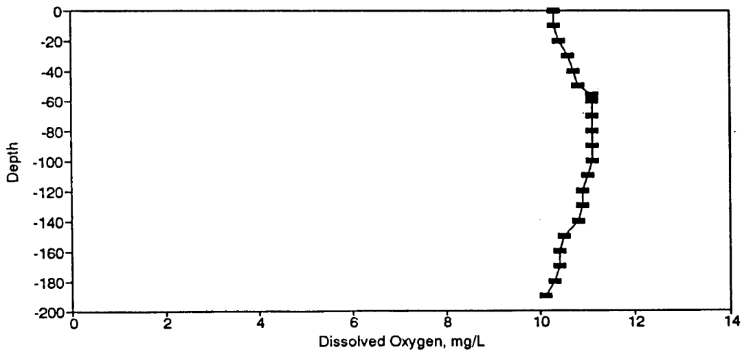
Figure BD123. Dissolved Oxygen Profile for the Eureka Springs Site-April 24, 1984.
