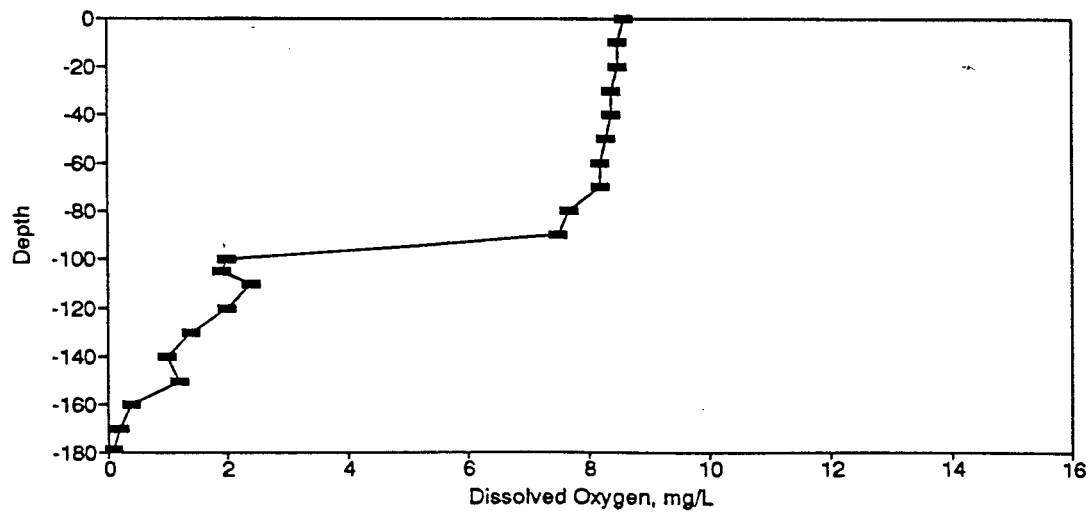
Figure BD60. Dissolved Oxygen Profile for the Eureka Springs Site-December 5, 1978.
