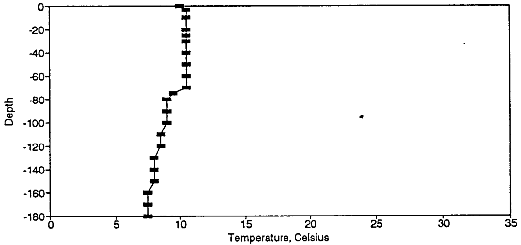
Figure BT167. Temperature Profile for the Eureka Springs Site-December 2, 1987.
