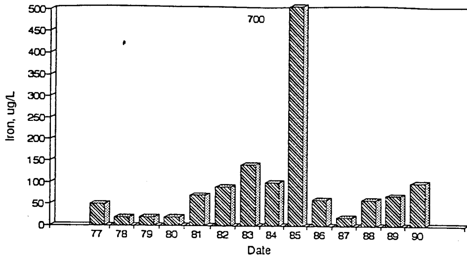
Figure A52. Graph of Iron vs. Time for the White River Site-May.
