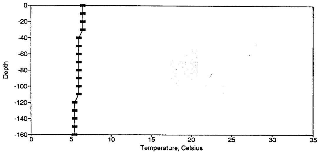
Figure BT39. Temperature Profile for the Eureka Springs Site-March 8, 1977.
