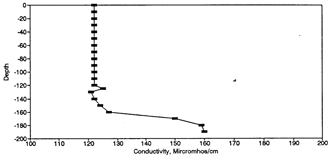
Figure BC11. Conductivity Profile for the Eureka Springs Site-November 20, 1974.
