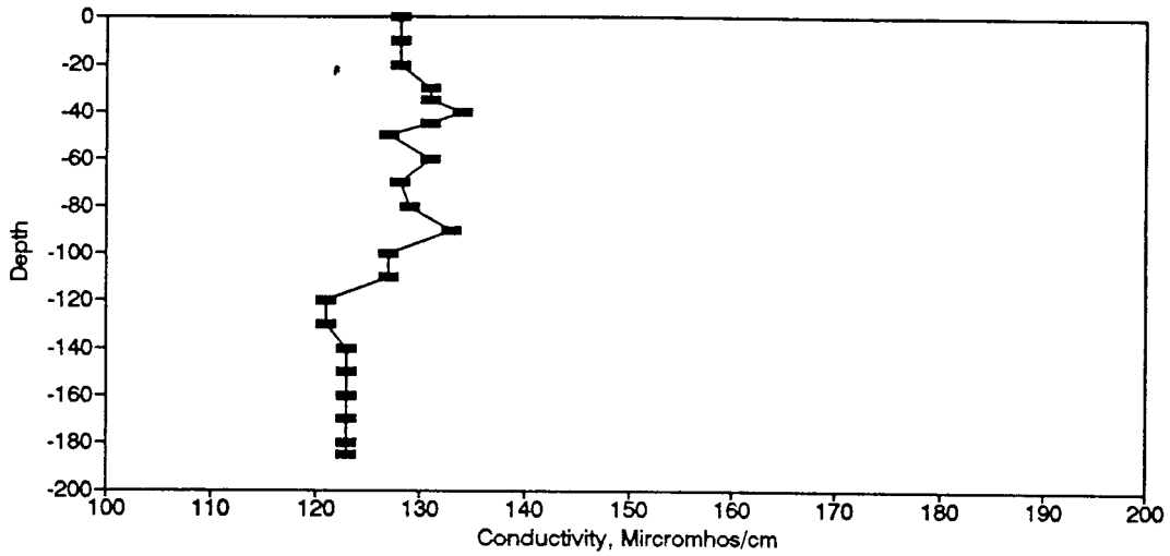
Figure BC28. Conductivity Profile for the Eureka Springs Site-April 20, 1976.
