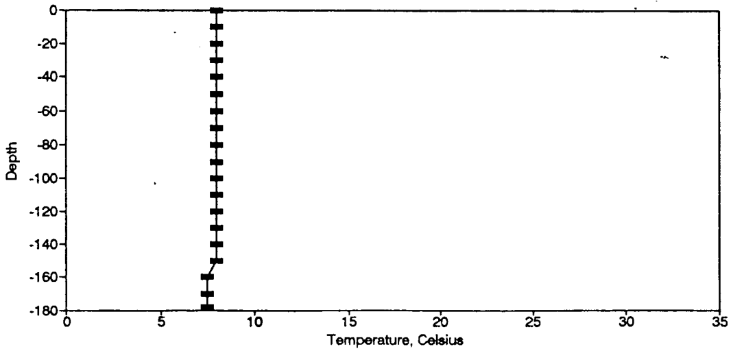
Figure BT36. Temperature Profile for the Eureka Springs Site-December 14, 1976.
