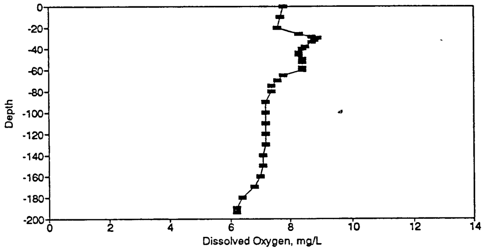
Figure BD89. Dissolved Oxygen Profile for the Eureka Springs Site-June 16, 1981.
