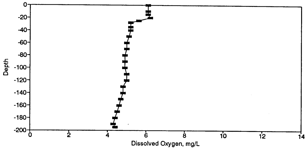
Figure BD7. Dissolved Oxygen Profile for the Eureka Springs Site-July 8, 1974.
