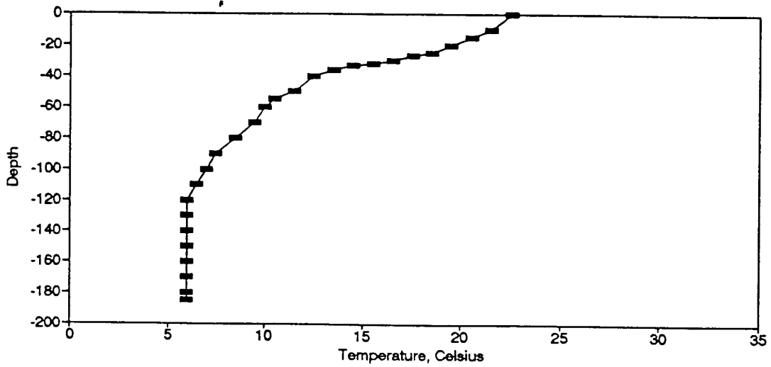
Figure BT100. Temperature Profile for the Eureka Springs Site-May 19, 1982.
