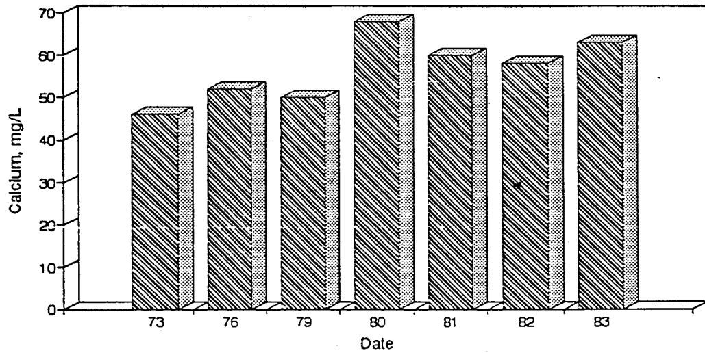
Figure A29. Graph of Calcium vs. Time for the White River Site-Aug.
