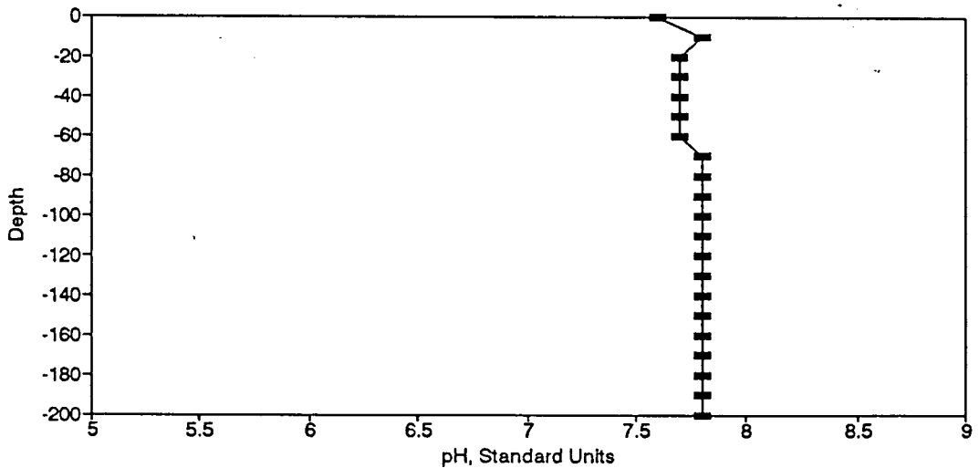
Figure BP15. pH Profile for the Eureka Springs Site-March 17, 1975.
