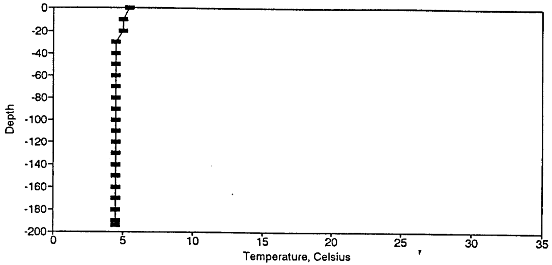
Figure BT97. Temperature Profile for the Eureka Springs Site-February 16, 1982.
