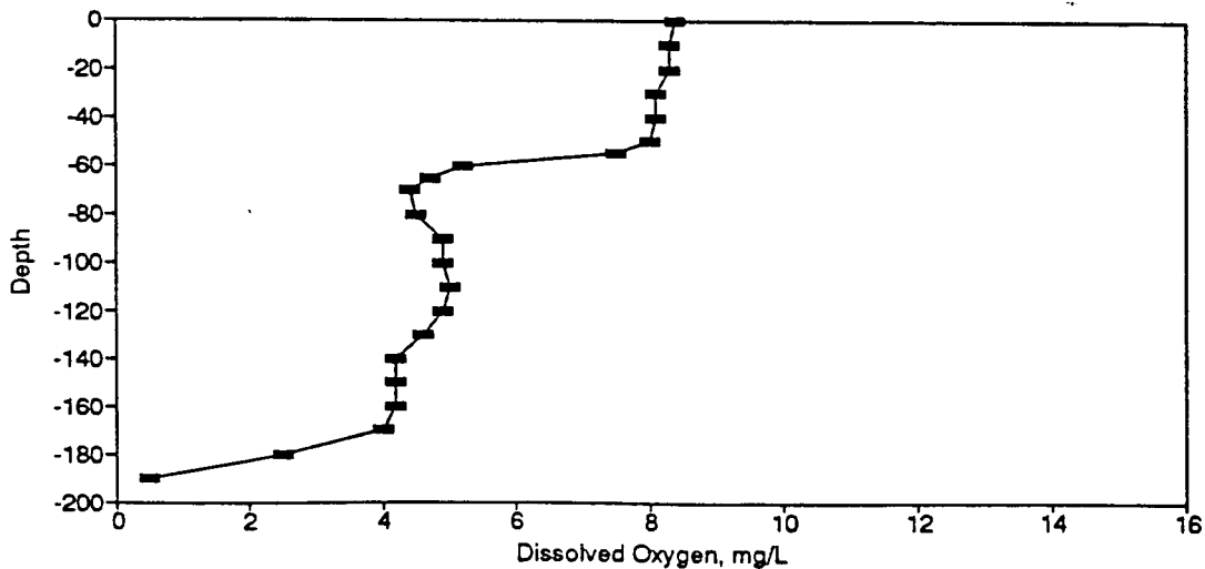
Figure BD48. Dissolved Oxygen Profile for the Eureka Springs Site-November 9, 1977.
