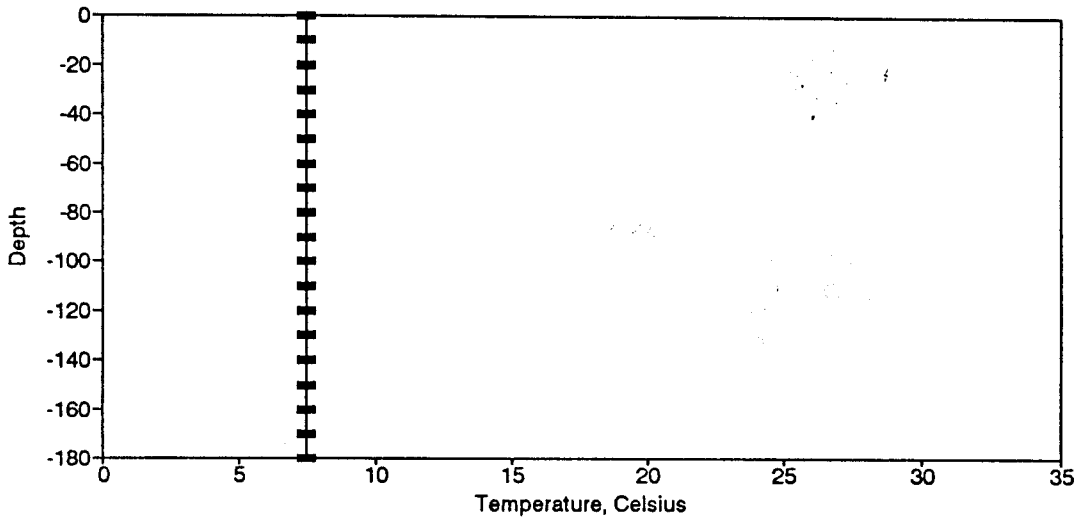
Figure BT50. Temperature Profile for the Eureka Springs Site-January 4, 1978.
