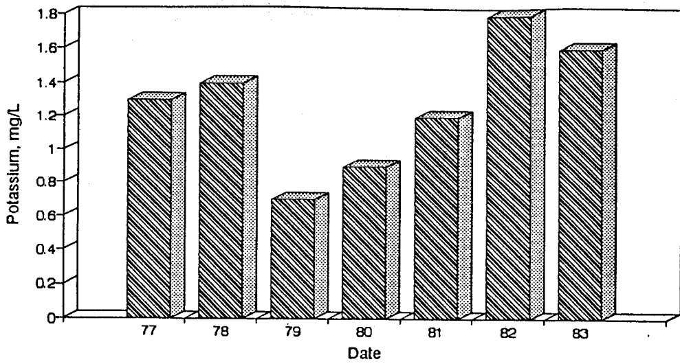
Figure A67. Graph of Potassium vs. Time for the White River Site-May.
