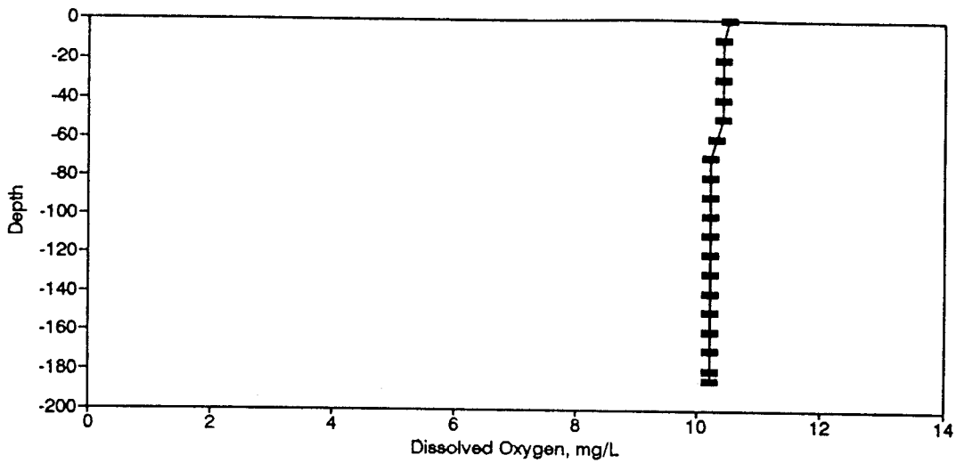
Figure BD85. Dissolved Oxygen Profile for the Eureka Springs Site-February 3, 1981.
