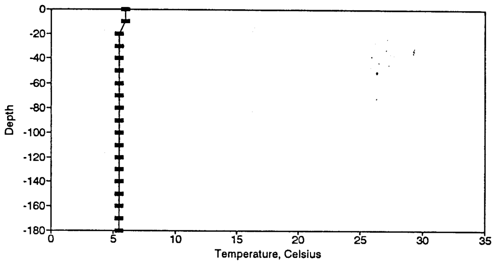
Figure BT74. Temperature Profile for the Eureka Springs Site-February 14, 1980.
