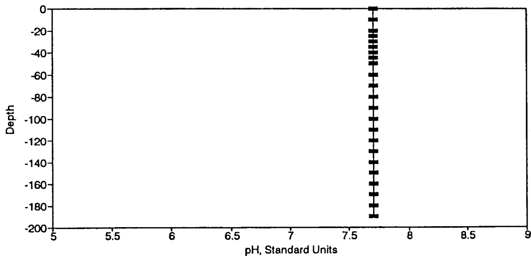
Figure BP30. pH Profile for the Eureka Springs Site-June 23, 1976.
