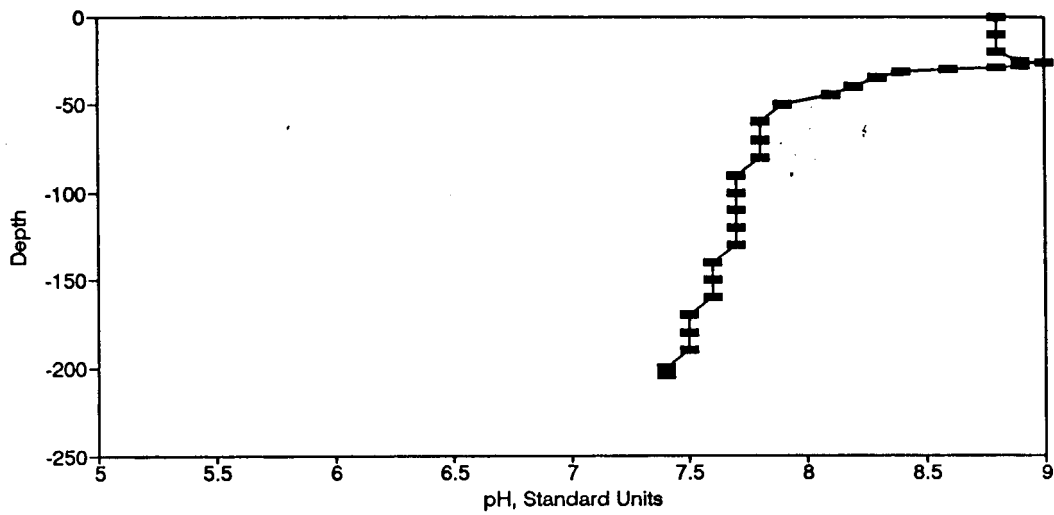
Figure BP113. pH Profile for the Eureka Springs Site-June 14, 1983.
