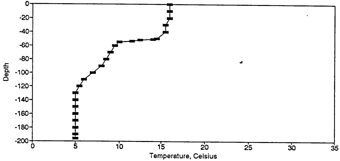
Figure BT65. Temperature Profile for the Eureka Springs Site-May 7, 1979.
