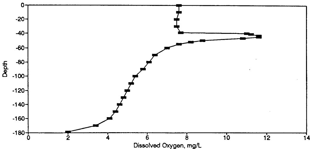
Figure BD81. Dissolved Oxygen Profile for the Eureka Springs Site-September 16, 1980.
