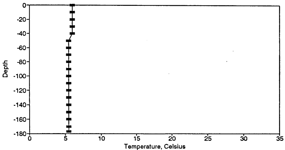
Figure BT75. Temperature Profile for the Eureka Springs Site-March 12, 1980.
