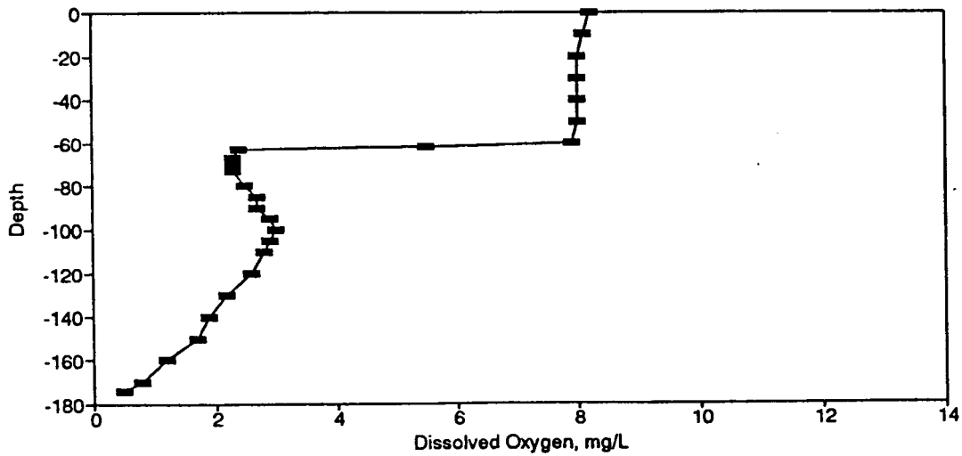
Figure BD93. Dissolved Oxygen Profile for the Eureka Springs Site-October 20, 1981.
