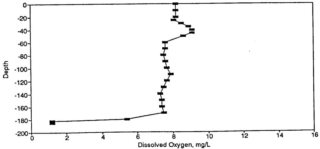
Figure BD45. Dissolved Oxygen Profile for the Eureka Springs Site-August 22, 1977.
