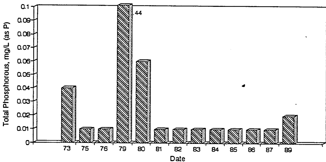
Figure A95. Graph of Total Phosphorous vs. Time for the White River Site-Aug.
