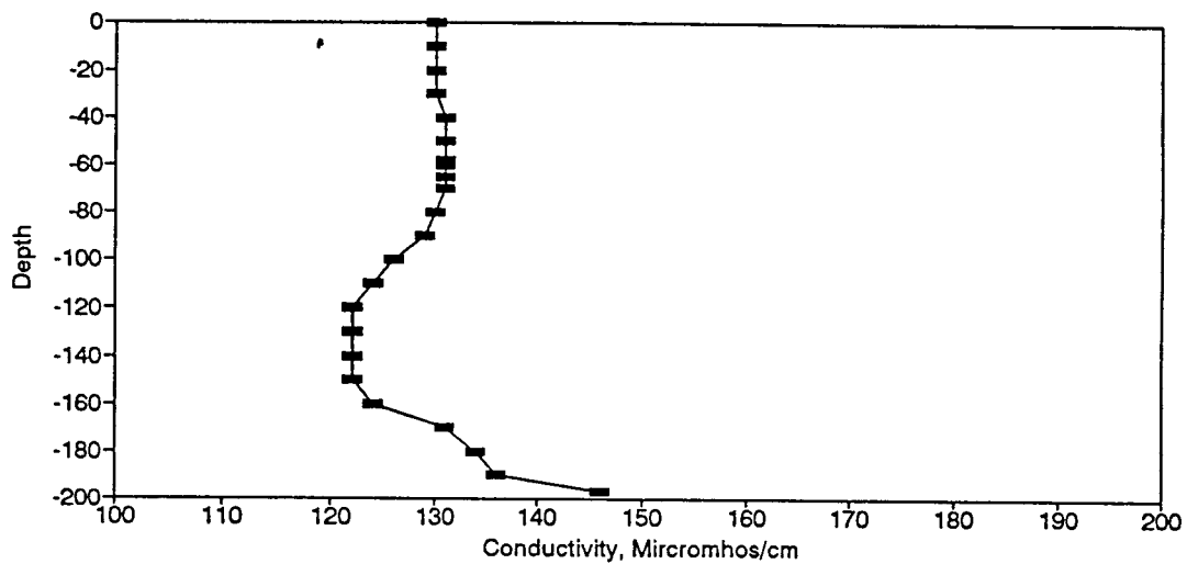
Figure BC154. Conductivity Profile for the Eureka Springs Site-November 5, 1986.
