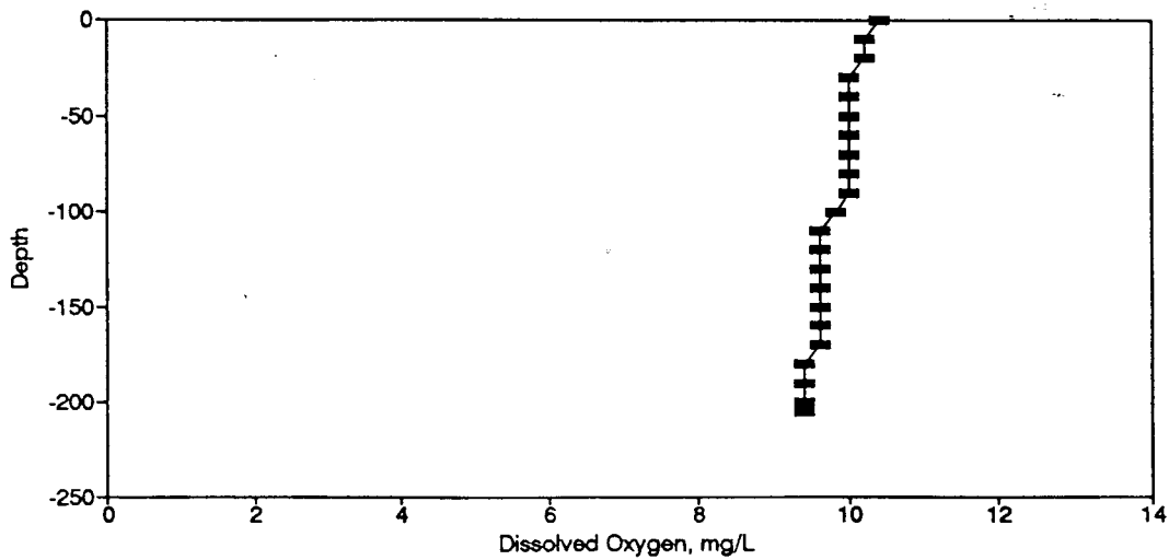
Figure BD132. Dissolved Oxygen Profile for the Eureka Springs Site-January 11, 1985.
