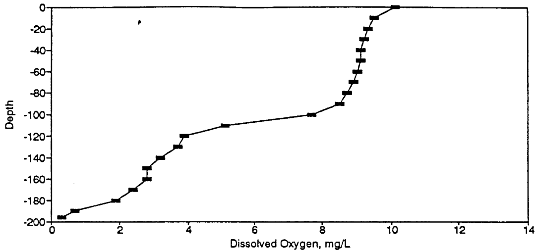
Figure BD178. Dissolved Oxygen Profile for the Eureka Springs Site-December 14, 1988.
