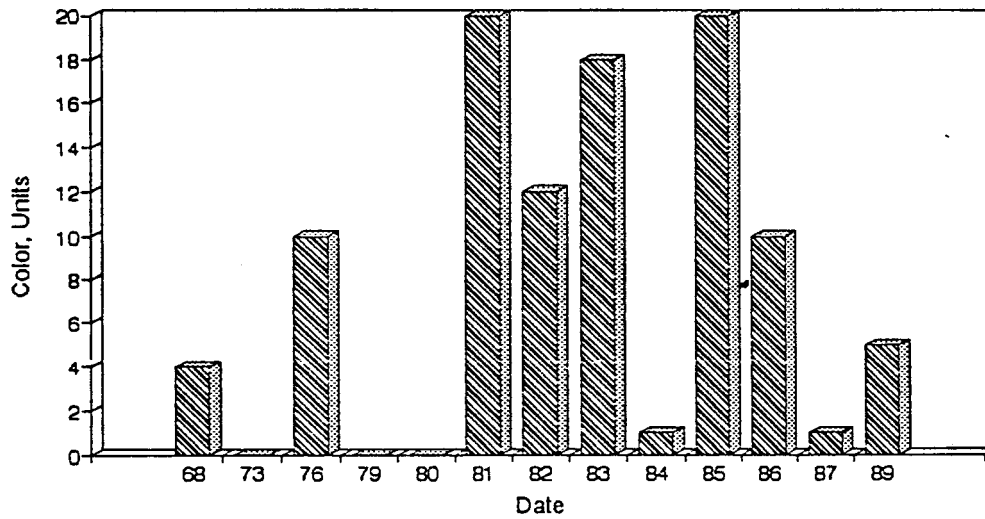
Figure A11. Graph of Color vs. Time for the White River Site-Aug.
