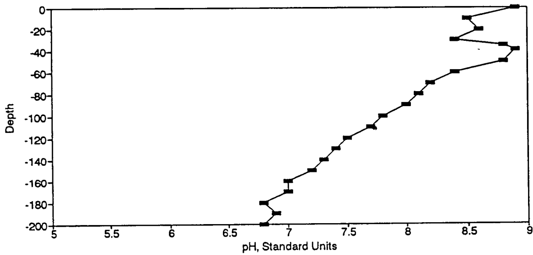
Figure BP8. pH Profile for the Eureka Springs Site-August 13, 1974.
