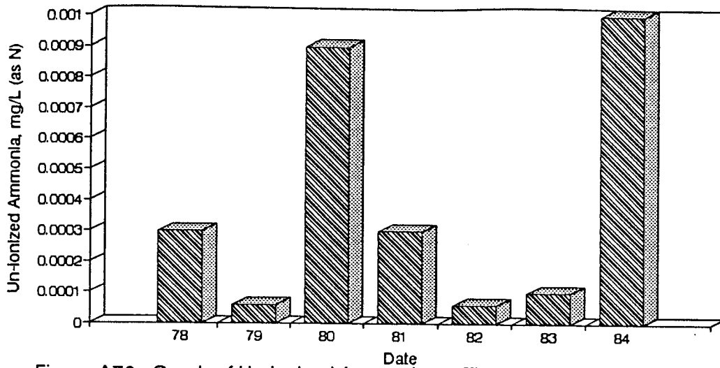
Figure A73. Graph of Un-ionized Ammonia vs. Time for the White River Site-May.
