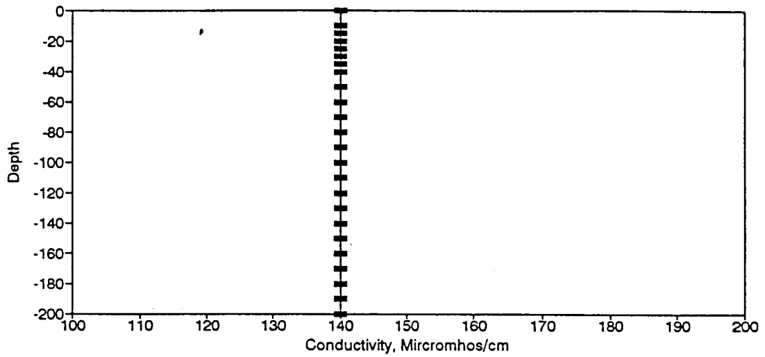
Figure BC52. Conductivity Profile for the Eureka Springs Site-April 11, 1978.
