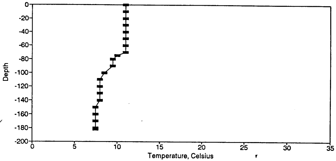
Figure BT49. Temperature Profile for the Eureka Springs Site-December 7, 1977.
