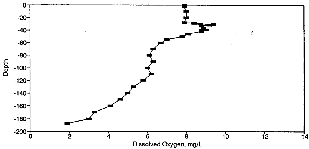
Figure BD164. Dissolved Oxygen Profile for the Eureka Springs Site-September 3, 1987.
