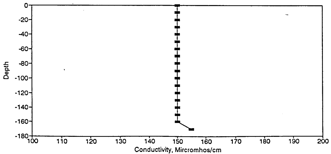
Figure BC120. Conductivity Profile for the Eureka Springs Site-January 25, 1984.
