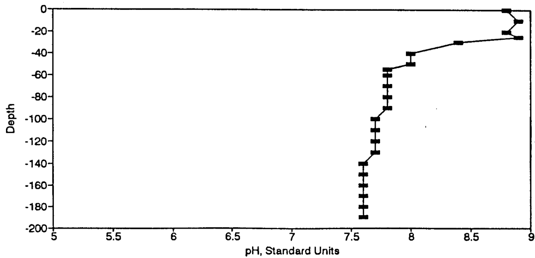
Figure BP54. pH Profile for the Eureka Springs Site-June 15, 1978.
