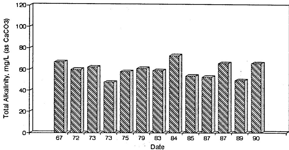
Figure A3. Graph of Total Alkalinity vs. Time for the White River Site-Dec.
