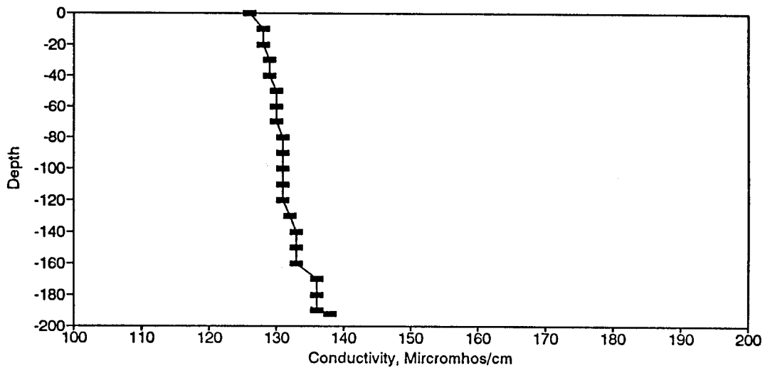
Figure BC157. Conductivity Profile for the Eureka Springs Site-February 4, 1987.
