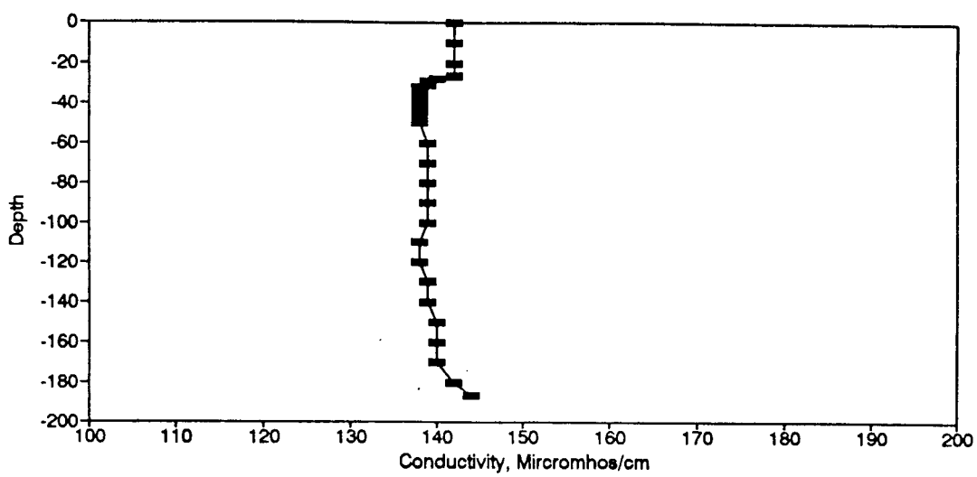
Figure BC79. Conductivity Profile for the Eureka Springs Site - July 16, 1980.
