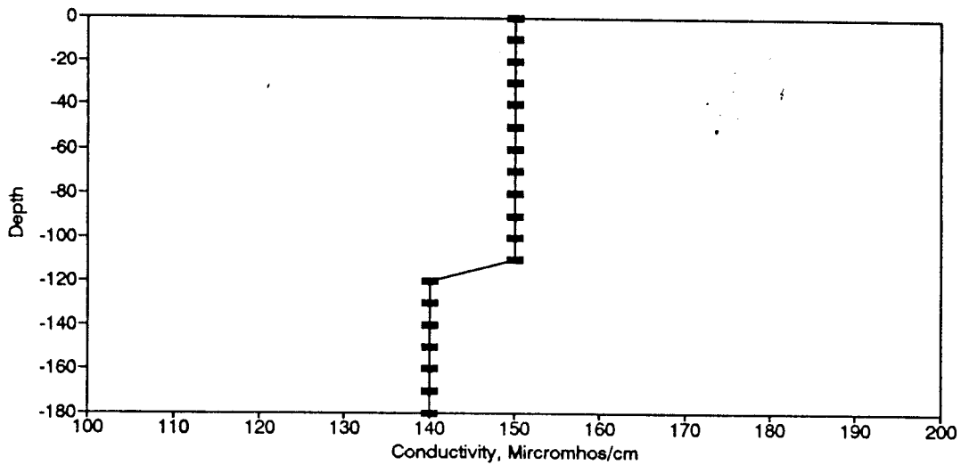
Figure BC50. Conductivity Profile for the Eureka Springs Site-January 4, 1978.
