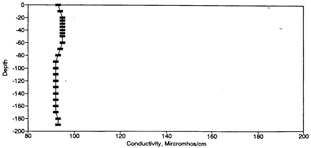
Figure BC30. Conductivity Profile for the Eureka Springs Site-June 23, 1976.
