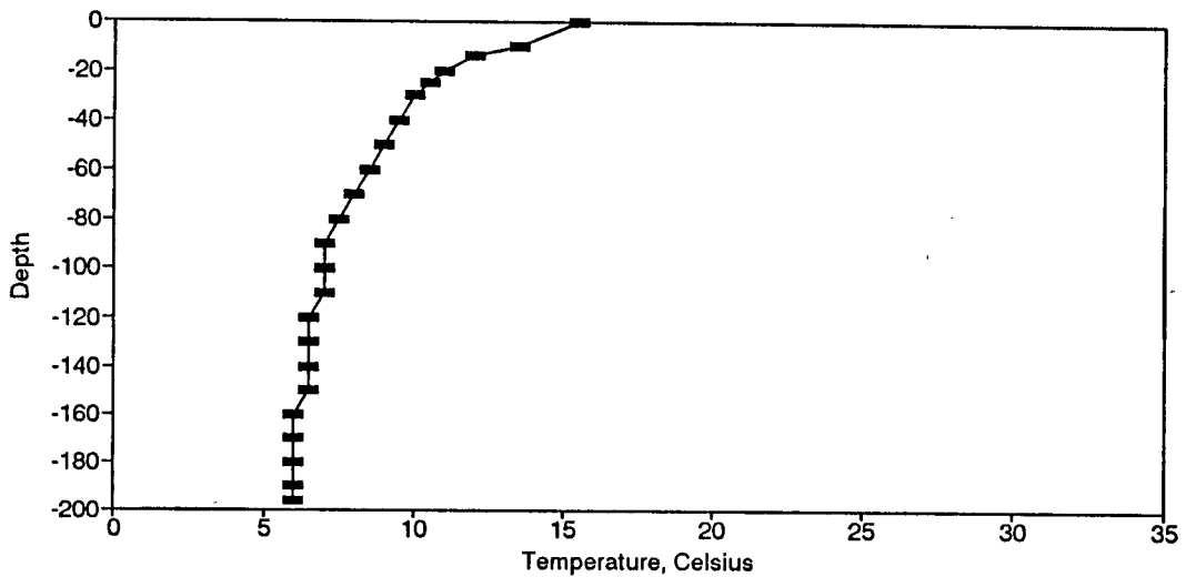
Figure BT147. Temperature Profile for the Eureka Springs Site-April 9, 1986.
