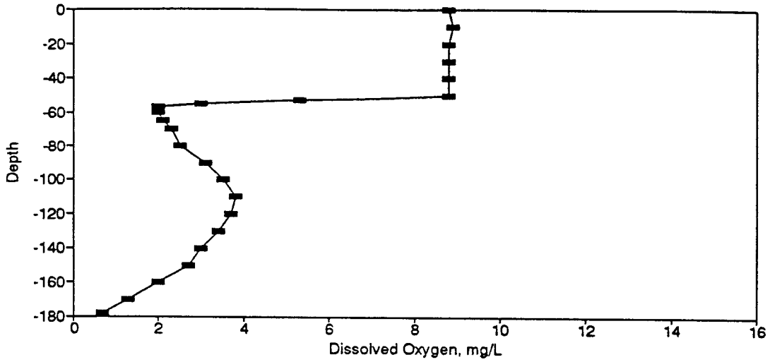
Figure BD58. Dissolved Oxygen Profile for the Eureka Springs Site-October 10, 1978.
