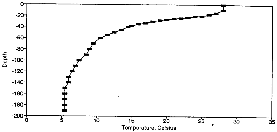
Figure BT67. Temperature Profile for the Eureka Springs Site-July 17, 1979.
