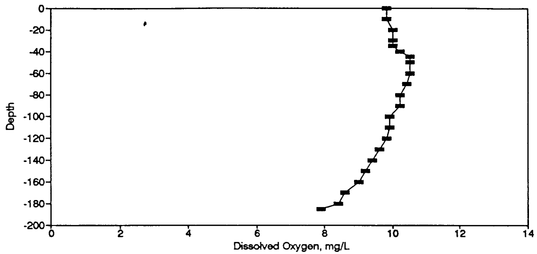
Figure BD28. Dissolved Oxygen Profile for the Eureka Springs Site-April 20, 1976.
