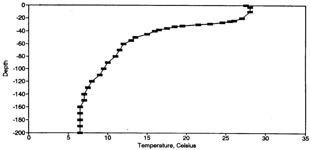
Figure BT139. Temperature Profile for the Eureka Springs Site-August 7, 1985.
