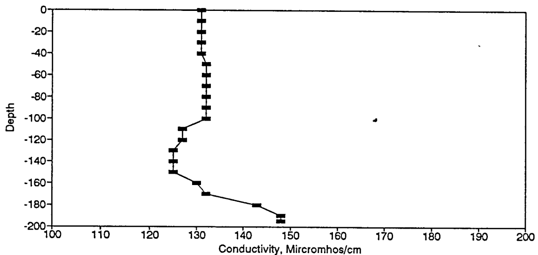
Figure BC155. Conductivity Profile for the Eureka Springs Site-December 4, 1986.
