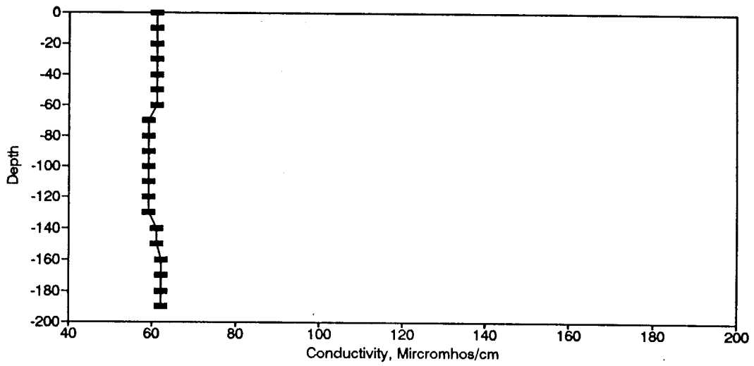
Figure BC13. Conductivity Profile for the Eureka Springs Site - January 21, 1975.
