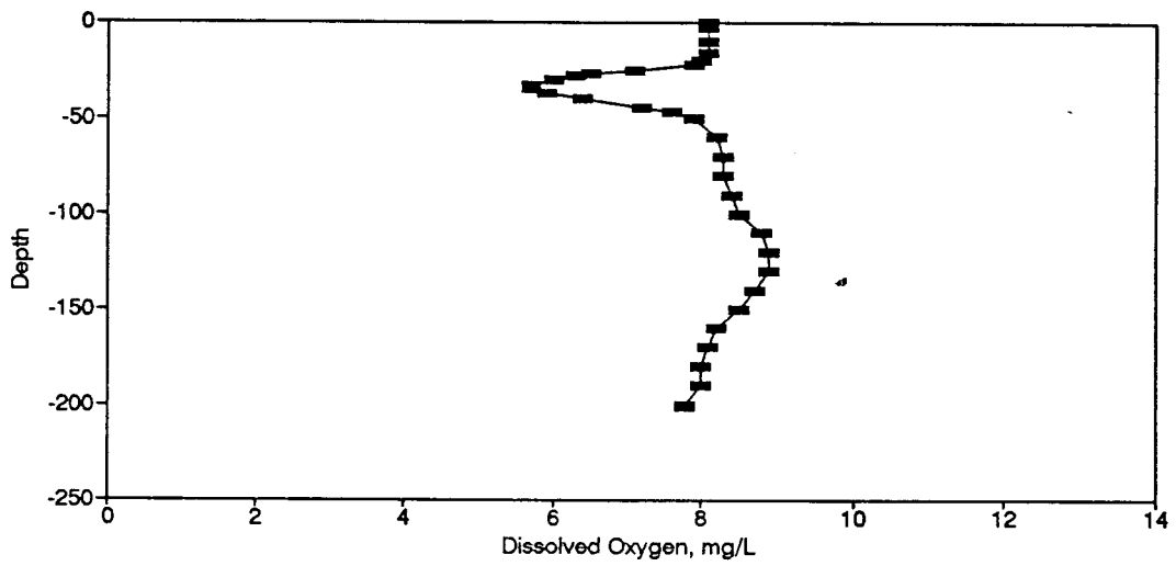
Figure BD137. Dissolved Oxygen Profile for the Eureka Springs Site-June 5, 1985.
