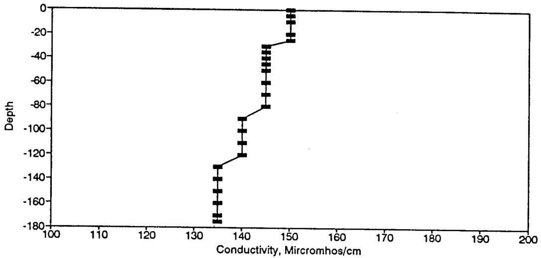
Figure BC43. Conductivity Profile for the Eureka Springs Site-June 27, 1977.
