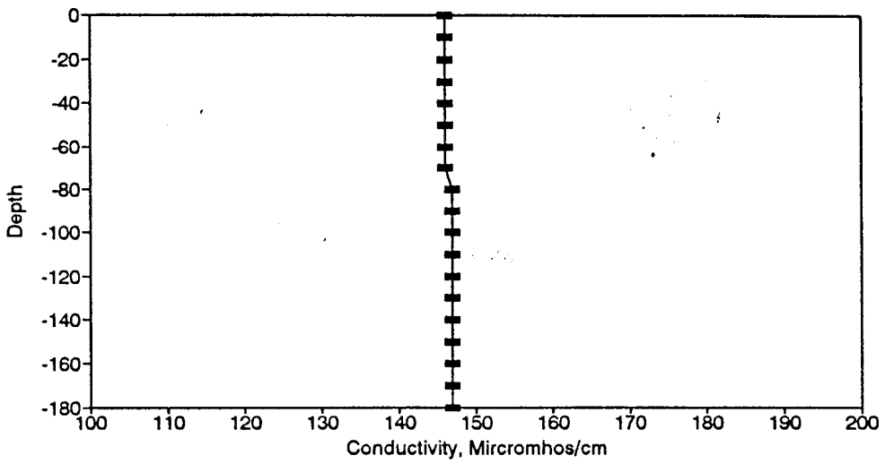
Figure BC74. Conductivity Profile for the Eureka Springs Site-February 14, 1980.
