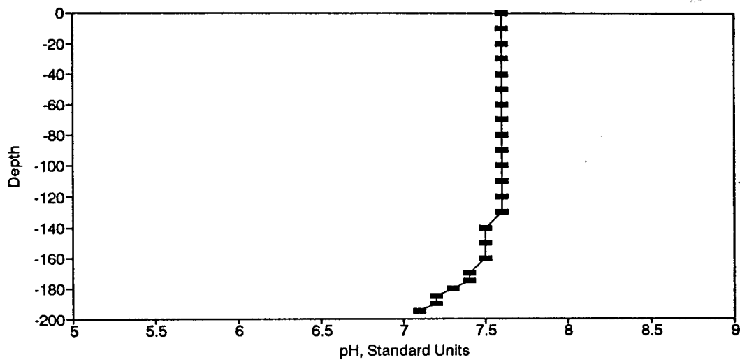
Figure BP12. pH Profile for the Eureka Springs Site-December 16, 1974.
