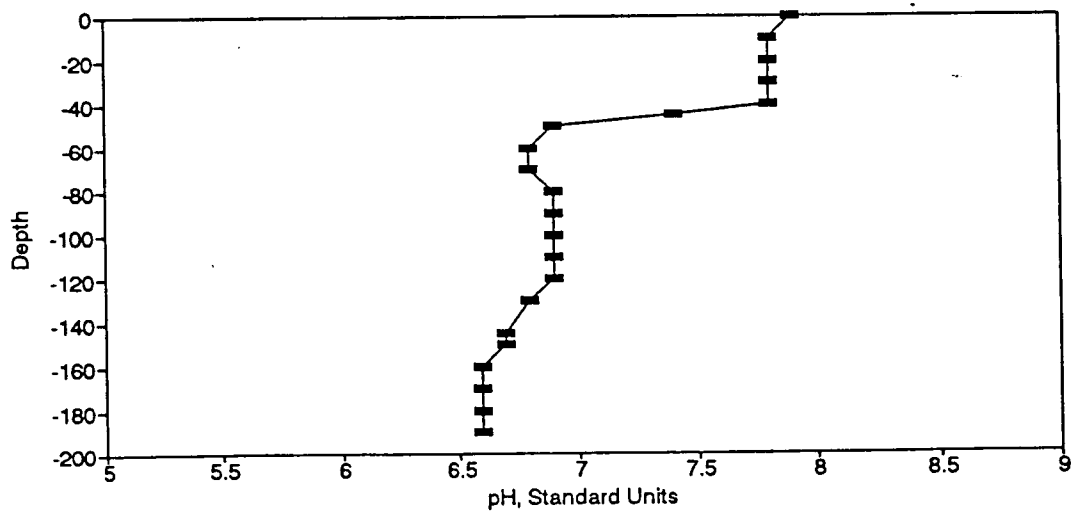
Figure BP9. pH Profile for the Eureka Springs Site-September 24, 1974.
