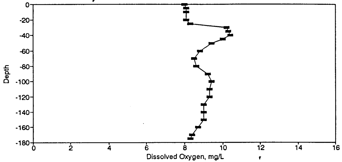
Figure BD43. Dissolved Oxygen Profile for the Eureka Springs Site-June 27, 1977.
