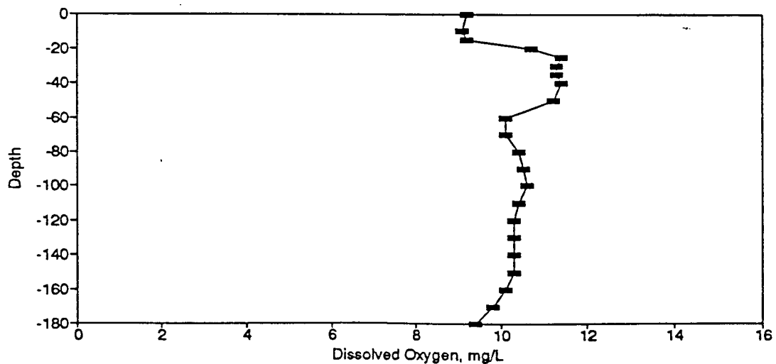
Figure BD42. Dissolved Oxygen Profile for the Eureka Springs Site-May 31, 1977.
