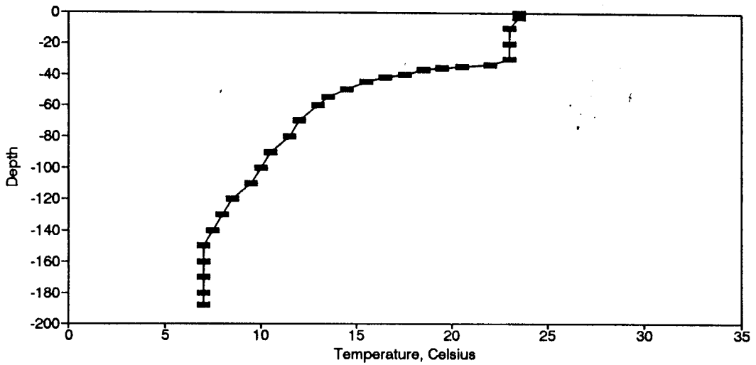
Figure BT128. Temperature Profile for the Eureka Springs Site-September 18, 1984.
