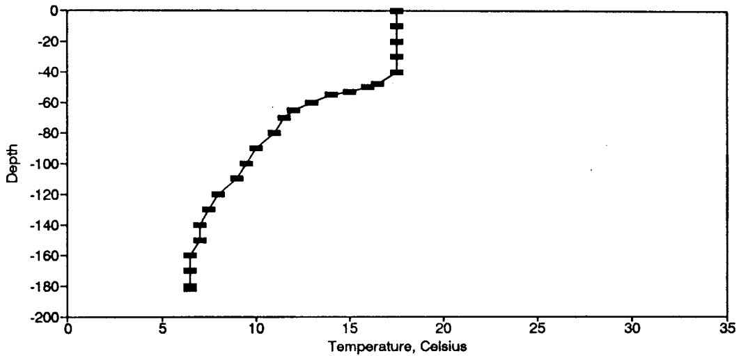
Figure BT129. Temperature Profile for the Eureka Springs Site-October 18, 1984.
