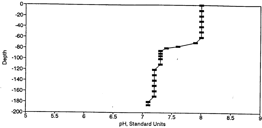
Figure BP94. pH Profile for the Eureka Springs Site-November 16, 1981.
