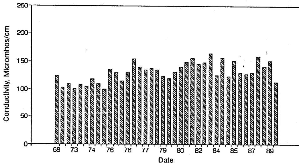
Figure A14. Graph of Conductivity vs. Time for the White River Site-Aug.
