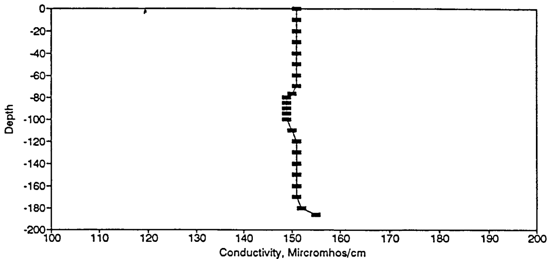
Figure BC94. Conductivity Profile for the Eureka Springs Site-November 16, 1981.
