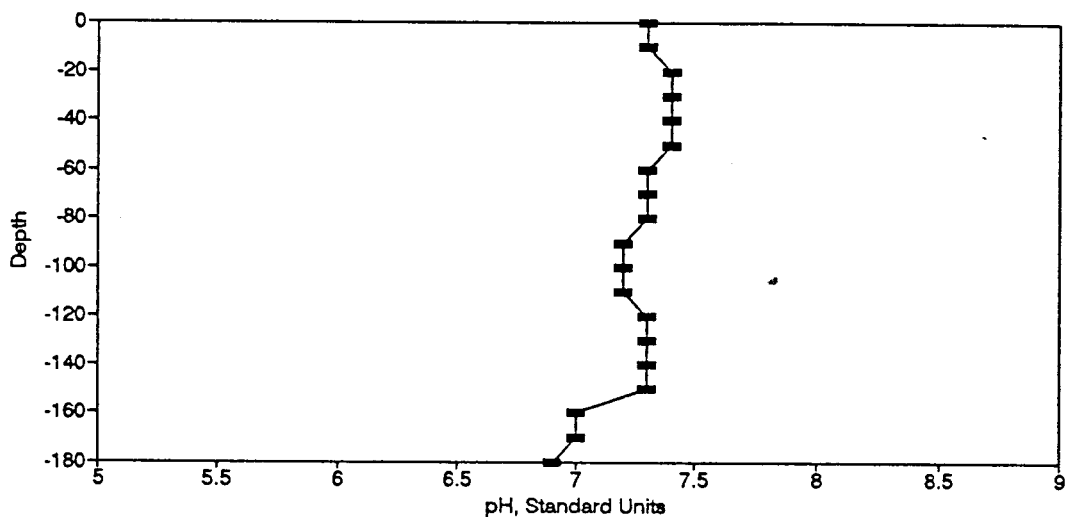
Figure BP50. pH Profile for the Eureka Springs Site-January 4, 1978.
