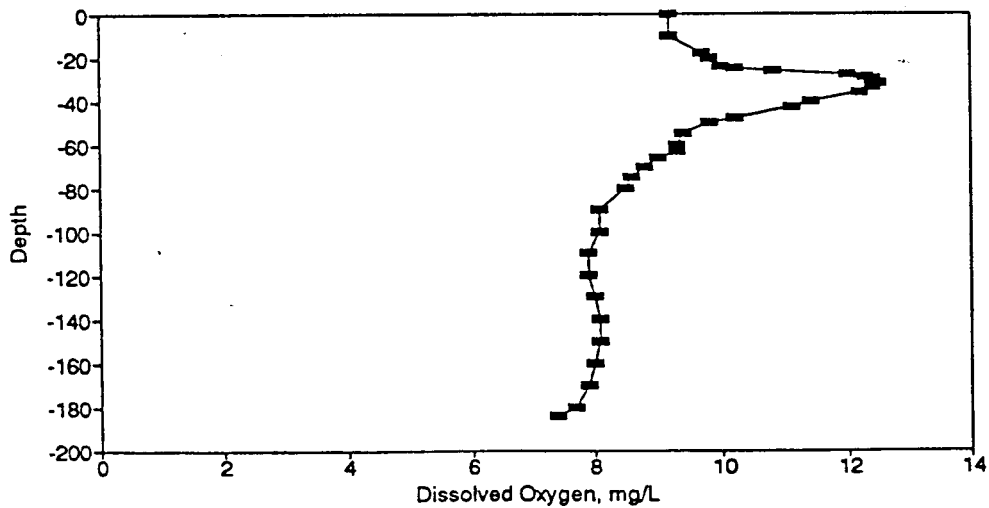
Figure BD90. Dissolved Oxygen Profile for the Eureka Springs Site-July 14, 1981.
