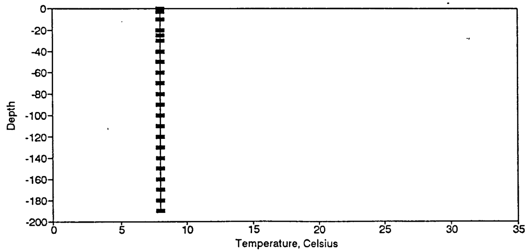
Figure BT156. Temperature Profile for the Eureka Springs Site-January 13, 1987.
