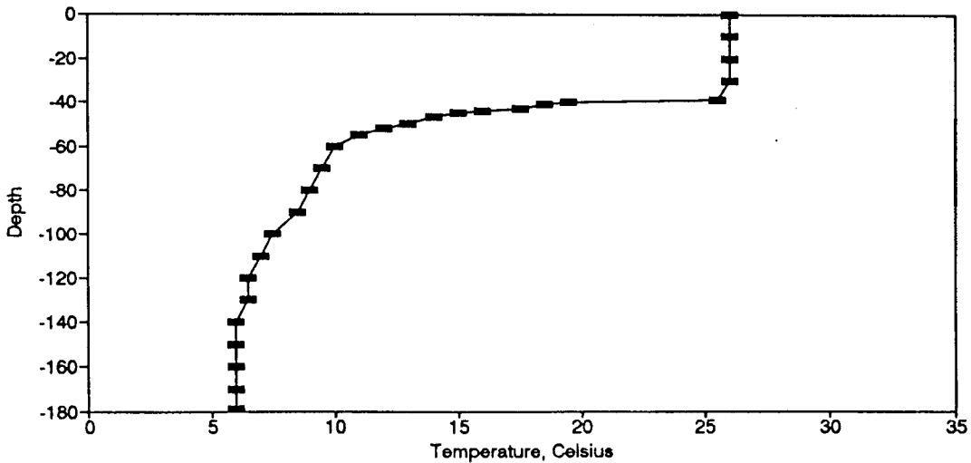
Figure BT81. Temperature Profile for the Eureka Springs Site-September 16, 1980.
