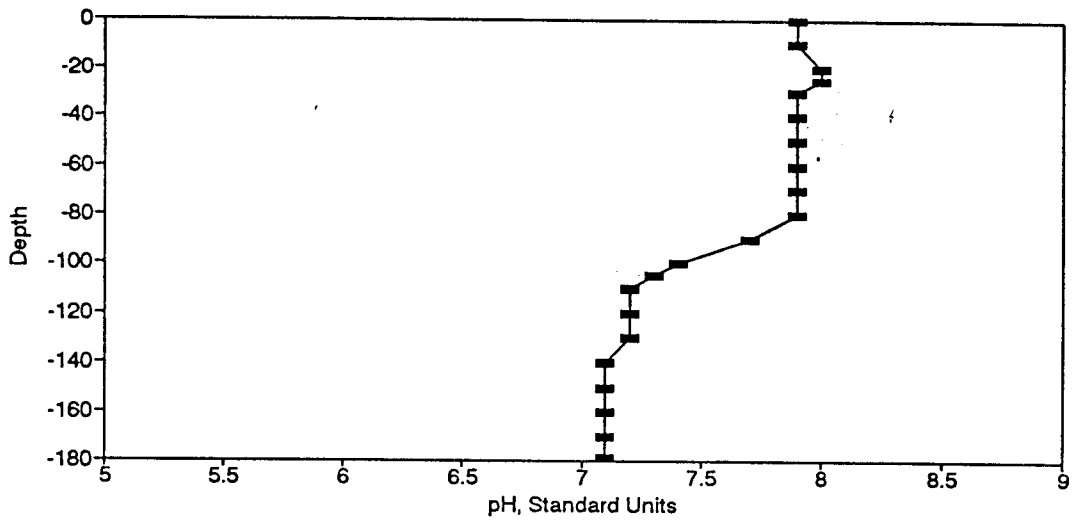
Figure BP95. pH Profile for the Eureka Springs Site-December 9, 1981.
