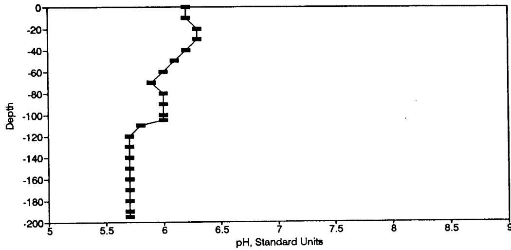
Figure BP24. pH Profile for the Eureka Springs Site-December 16, 1975.
