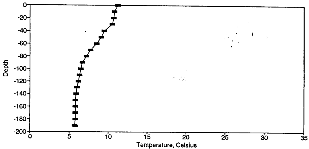
Figure BT182. Temperature Profile for the Eureka Springs Site-April 11, 1989.
