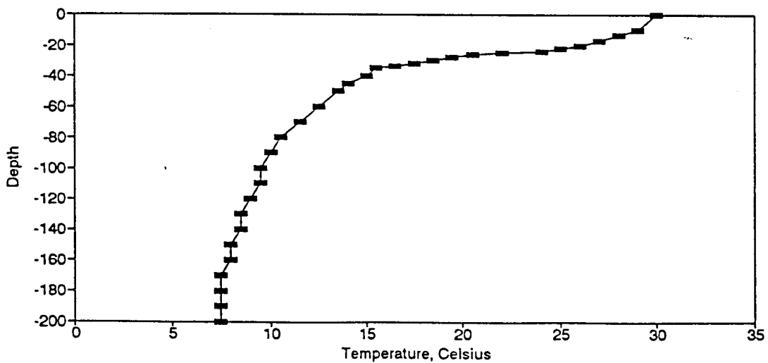
Figure BT114. Temperature Profile for the Eureka Springs Site-July 12, 1983.
