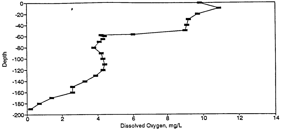
Figure BD166. Dissolved Oxygen Profile for the Eureka Springs Site-November 12, 1987.
