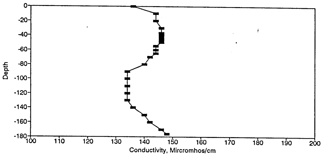
Figure BC116. Conductivity Profile for the Eureka Springs Site-September 19, 1983.
