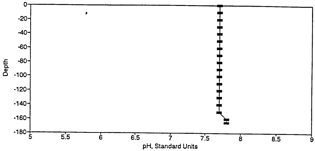
Figure BP121. pH Profile for the Eureka Springs Site-February 29, 1984.
