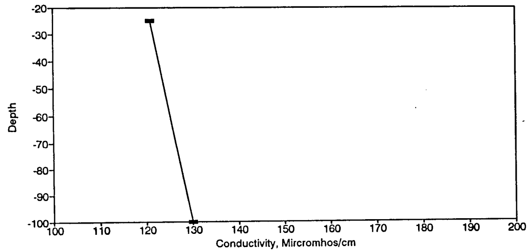
Figure BC189. Conductivity Profile for the Eureka Springs Site-May 15, 1990.
