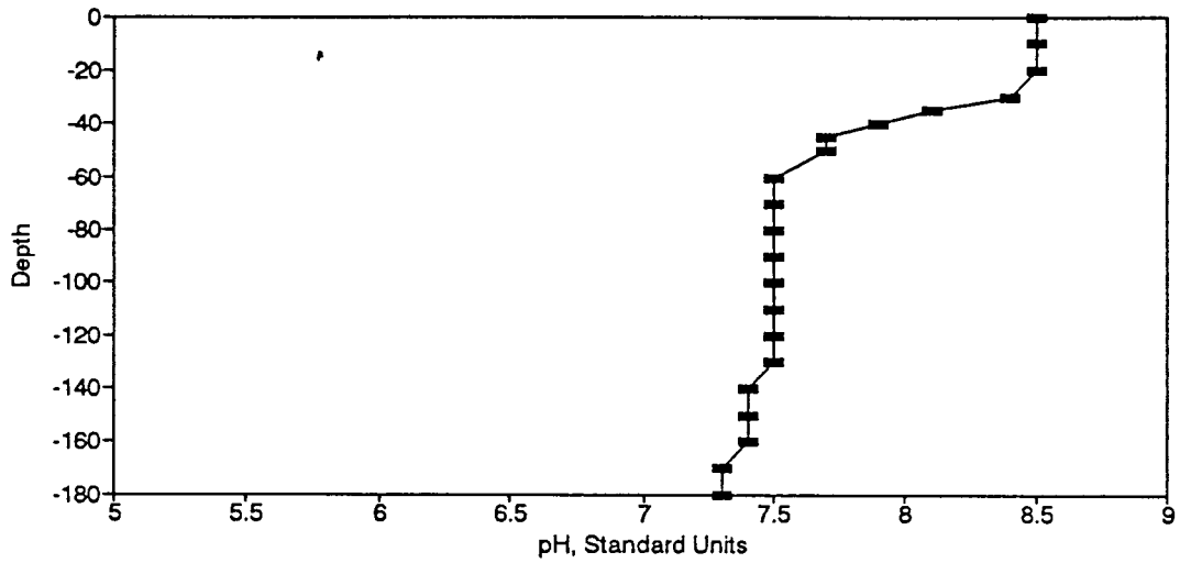
Figure BP31. pH Profile for the Eureka Springs Site-July 23, 1976.
