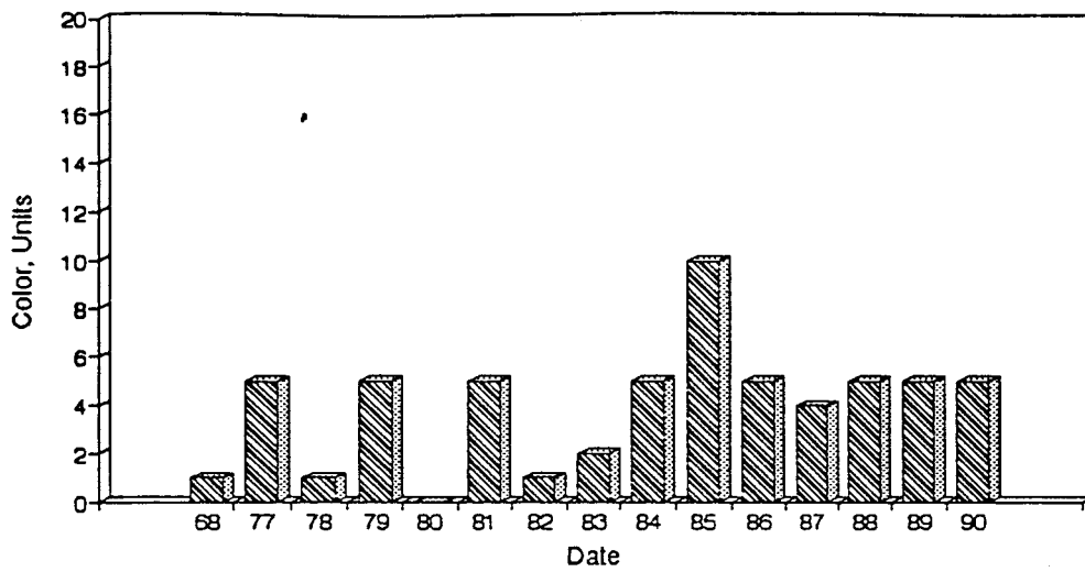
Figure A10. Graph of Color vs. Time for the White River Site-May.
