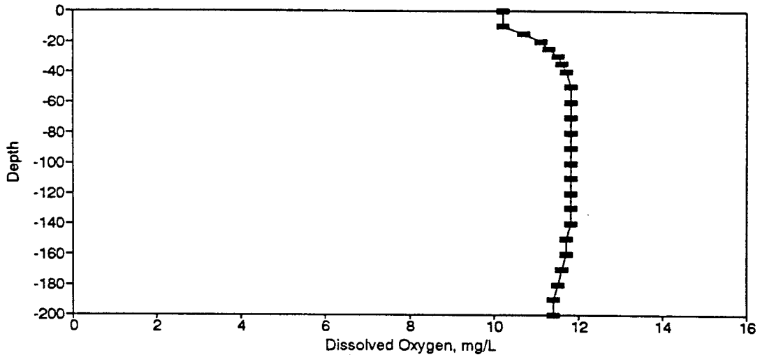
Figure BD52. Dissolved Oxygen Profile for the Eureka Springs Site-April 11, 1978.
