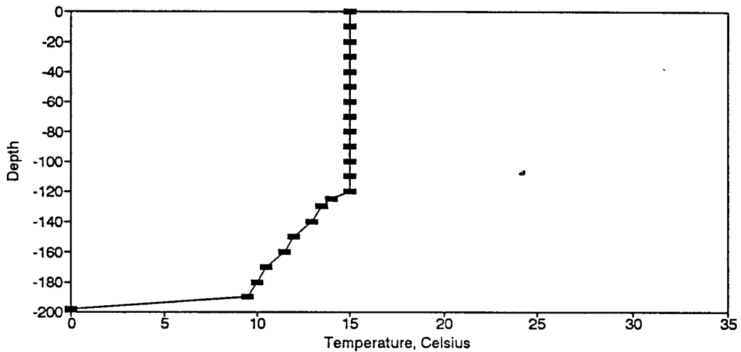
Figure BT11. Temperature Profile for the Eureka Springs Site-November 20, 1974.
