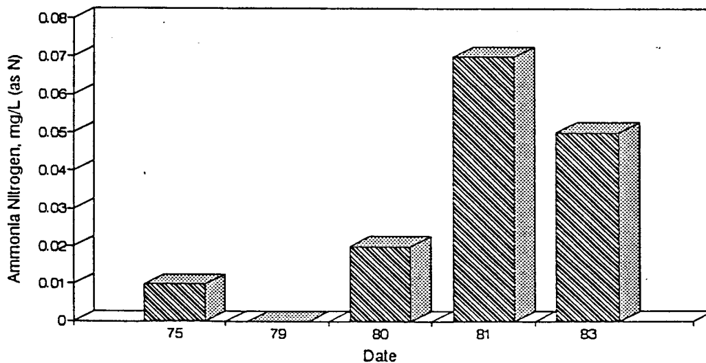
Figure A78. Graph of Ammonia Nitrogen vs. Time for the White River Site-Dec.
