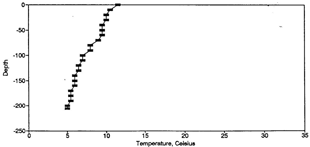
Figure BT135. Temperature Profile for the Eureka Springs Site-April 3, 1985.
