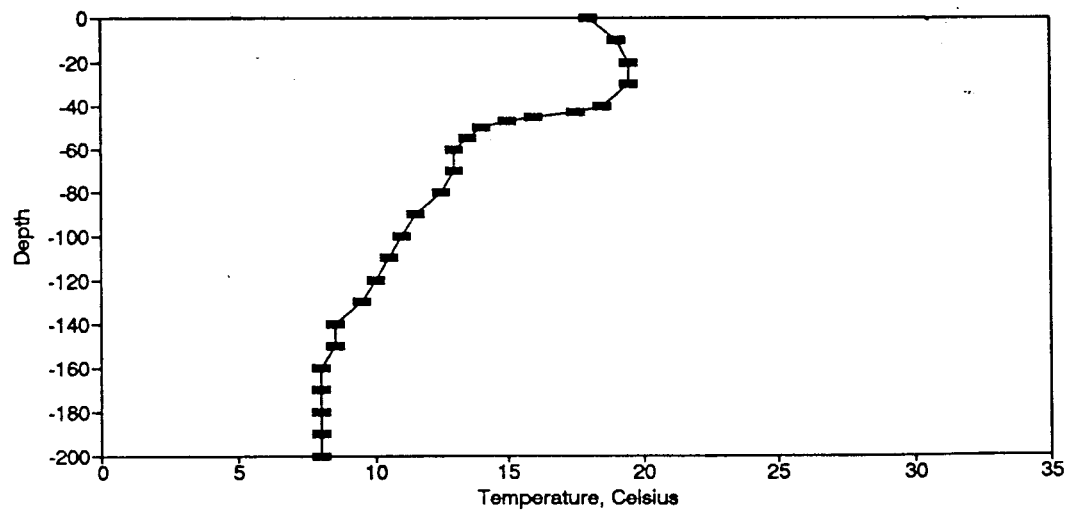
Figure BT6. Temperature Profile for the Eureka Springs Site-May 14, 1974.
