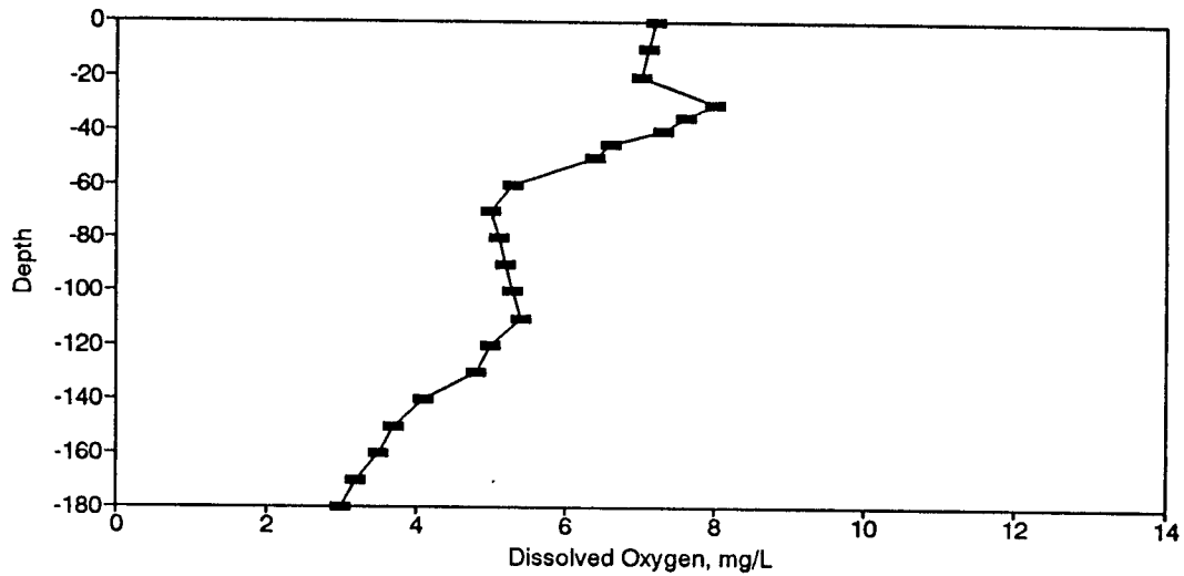
Figure BD31. Dissolved Oxygen Profile for the Eureka Springs Site-July 23, 1976.
