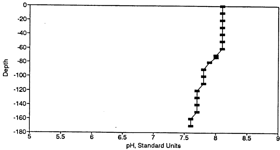
Figure BP76. pH Profile for the Eureka Springs Site-April 8, 1980.
