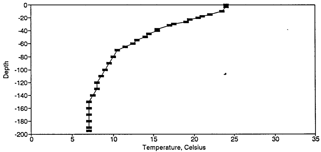
Figure BT149. Temperature Profile for the Eureka Springs Site-June 4, 1986.
