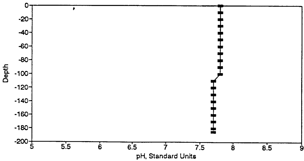
Figure BP85. pH Profile for the Eureka Springs Site-February 3, 1981.
