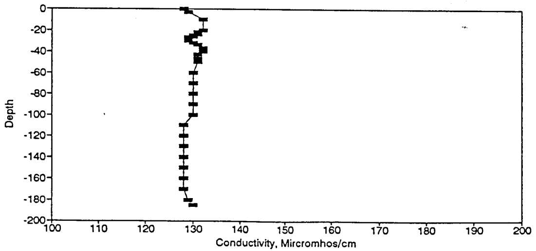
Figure BC126. Conductivity Profile for the Eureka Springs Site-July 17, 1984.
