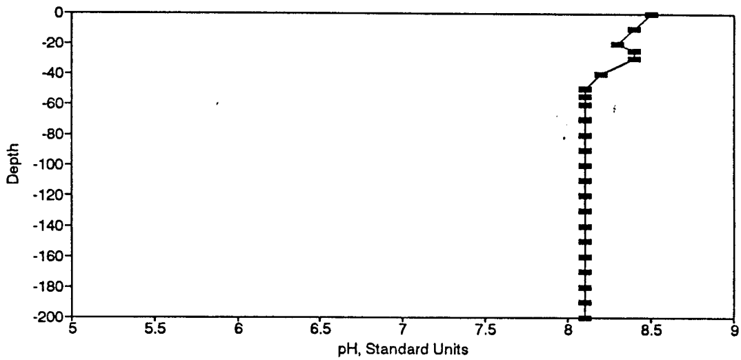
Figure BP53. pH Profile for the Eureka Springs Site-May 9, 1978.
