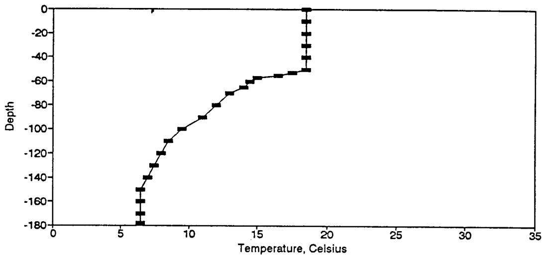
Figure BT58. Temperature Profile for the Eureka Springs Site-October 10, 1978.
