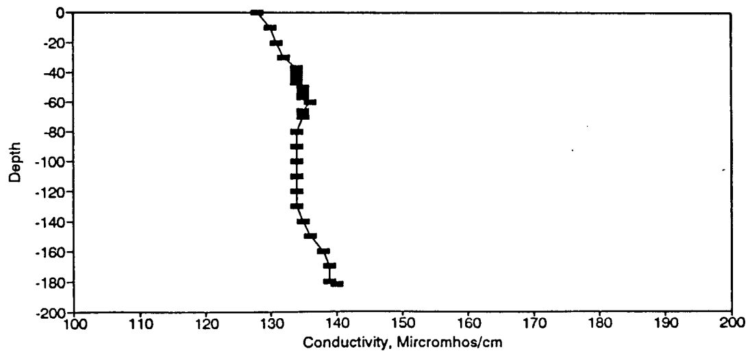
Figure BC69. Conductivity Profile for the Eureka Springs Site-September 17, 1979.
