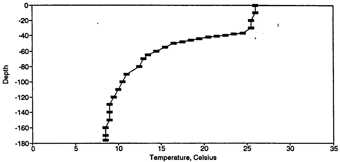
Figure BT116. Temperature Profile for the Eureka Springs Site-September 19, 1983.
