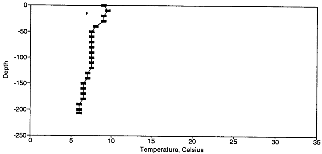
Figure BT16. Temperature Profile for the Eureka Springs Site-April 15, 1975.
