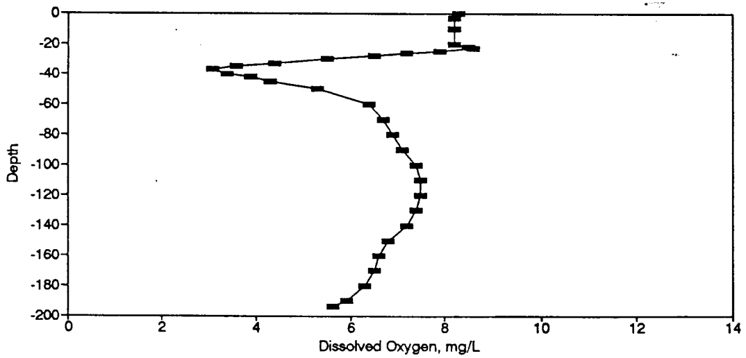
Figure BD138. Dissolved Oxygen Profile for the Eureka Springs Site-July 11, 1985.
