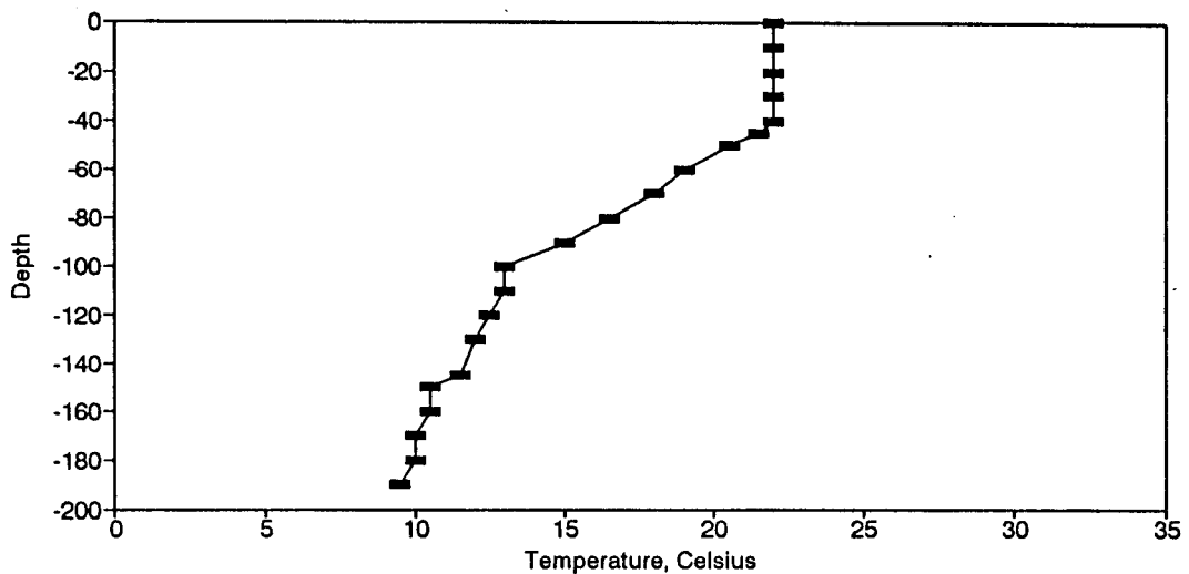
Figure BT9. Temperature Profile for the Eureka Springs Site September 24, 1974.
