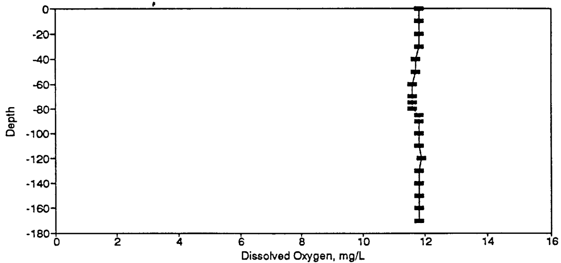
Figure BD40. Dissolved Oxygen Profile for the Eureka Springs Site-April 5, 1977.
