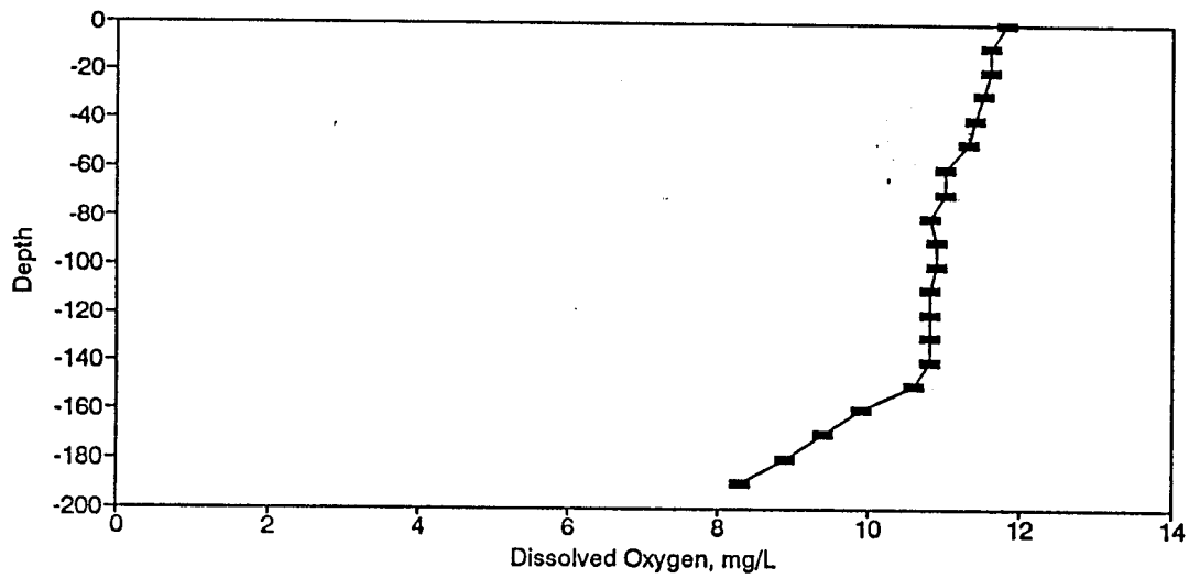
Figure BD158. Dissolved Oxygen Profile for the Eureka Springs Site-March 11, 1987.
