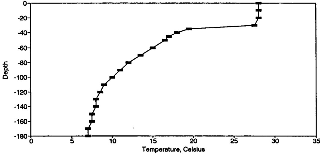
Figure BT31. Temperature Profile for the Eureka Springs Site-July 23, 1976.
