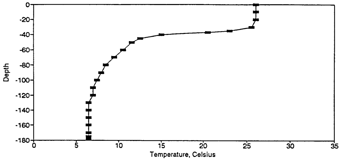
Figure BT46. Temperature Profile for the Eureka Springs Site-September 12, 1977.
