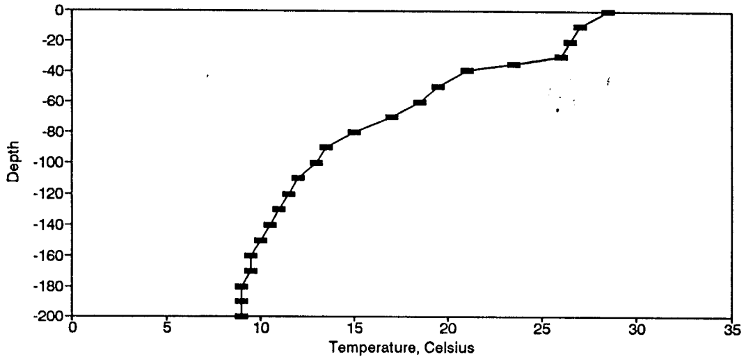
Figure BT8. Temperature Profile for the Eureka Springs Site August 13, 1974.
