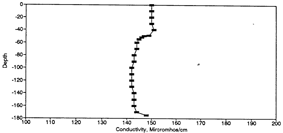
Figure BC83. Conductivity Profile for the Eureka Springs Site-November 5, 1980.
