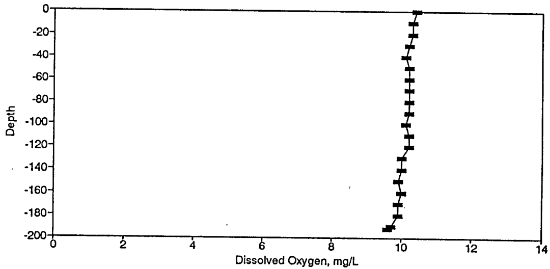
Figure BD157. Dissolved Oxygen Profile for the Eureka Springs Site-February 4, 1987.
