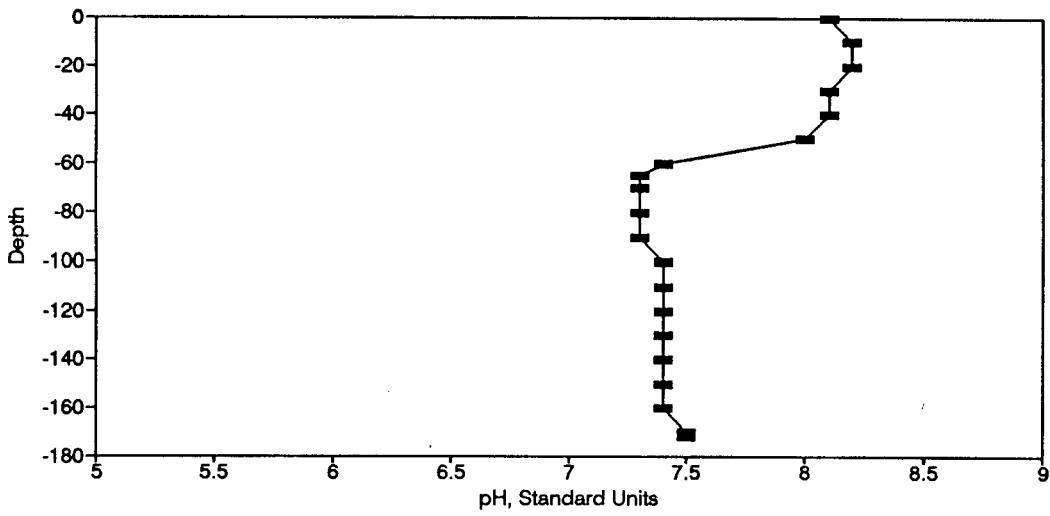
Figure BP34. pH Profile for the Eureka Springs Site-October 18, 1976.
