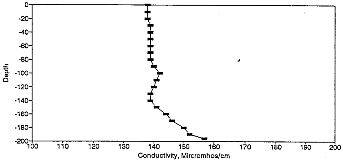
Figure BC107. Conductivity Profile for the Eureka Springs Site-December 8, 1982.
