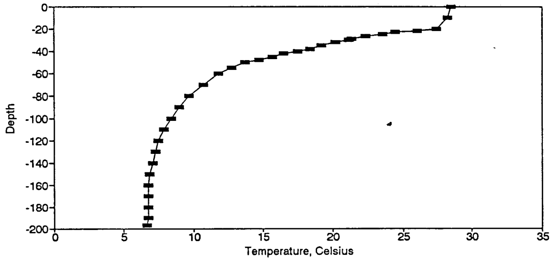
Figure BT185. Temperature Profile for the Eureka Springs Site-July 13, 1989.
