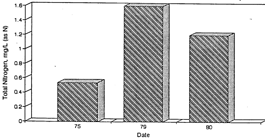
Figure A90. Graph of Total Nitrogen vs. Time for the White River Site-Dec.
