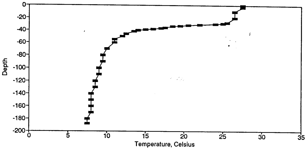
Figure BT164. Temperature Profile for the Eureka Springs Site-September 3, 1987.
