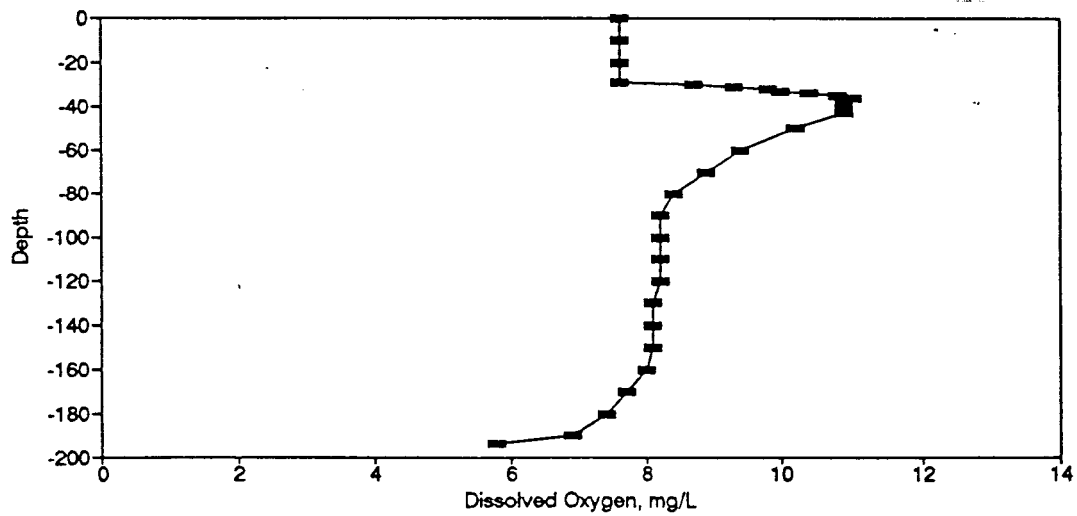
Figure BD78. Dissolved Oxygen Profile for the Eureka Springs Site-June 19, 1980.
