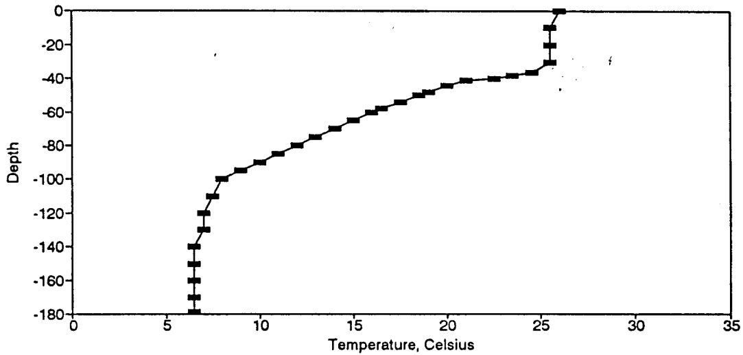
Figure BT92. Temperature Profile for the Eureka Springs Site-September 14, 1981.
