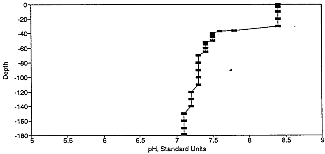
Figure BP104. pH Profile for the Eureka Springs Site-September 23, 1982.
