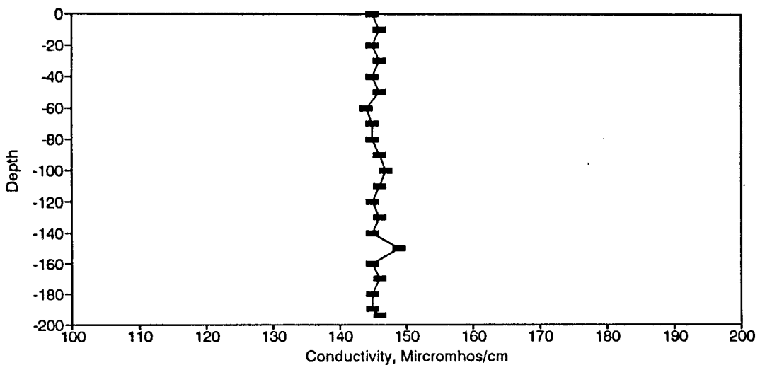
Figure BC171. Conductivity Profile for the Eureka Springs Site-April 13, 1988.
