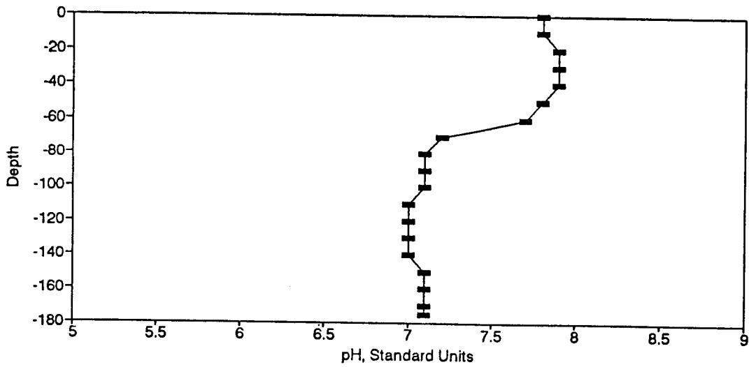
Figure BP106. pH Profile for the Eureka Springs Site-November 24, 1982.
