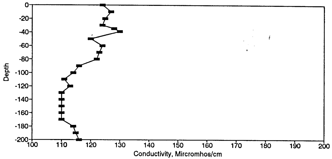
Figure BC8. Conductivity Profile for the Eureka Springs Site - August 13, 1974.
