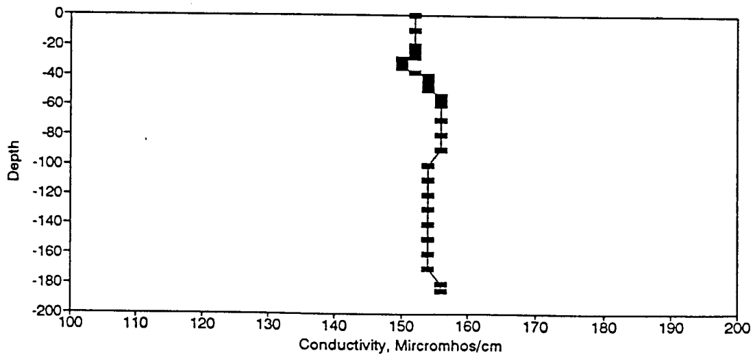
Figure BC102. Conductivity Profile for the Eureka Springs Site-July 20, 1982.
