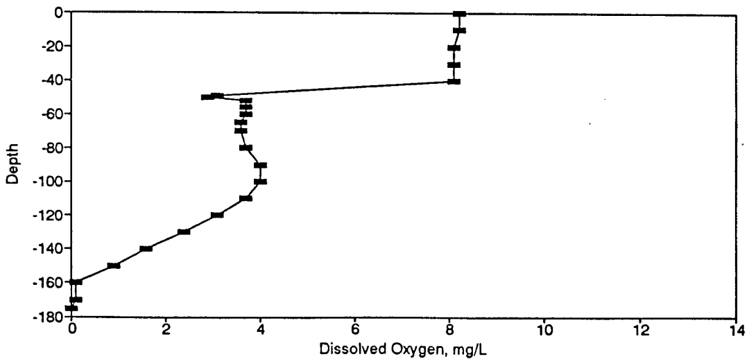
Figure BD105. Dissolved Oxygen Profile for the Eureka Springs Site-October 22, 1982.
