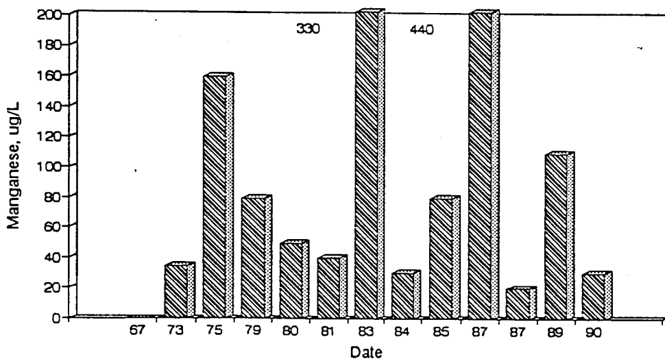
Figure A60. Graph of Manganese vs. Time for the White River Site-Dec.
