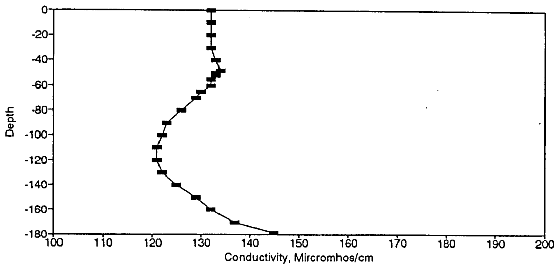
Figure BC117. Conductivity Profile for the Eureka Springs Site-October 20, 1983.
