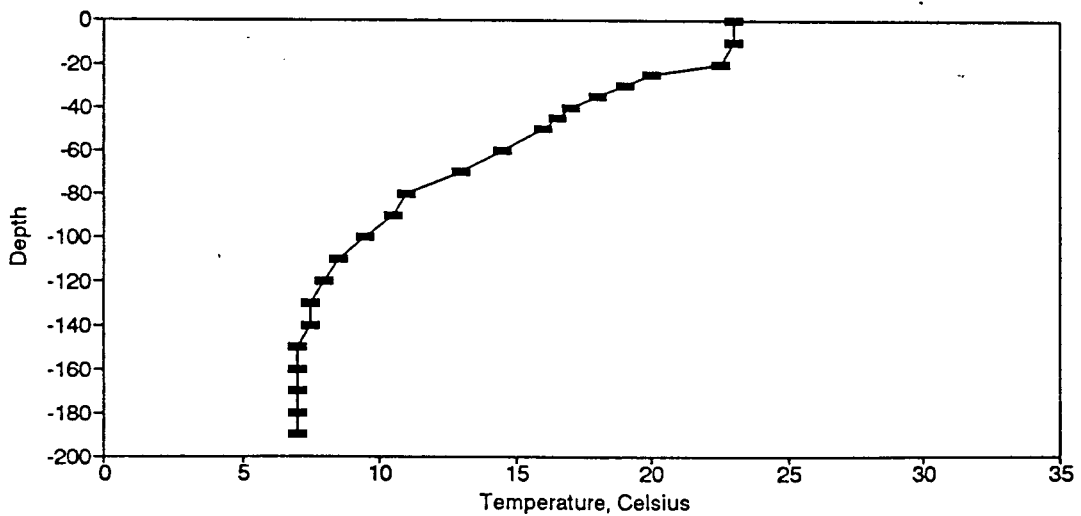
Figure BT30. Temperature Profile for the Eureka Springs Site-June 23, 1976.
