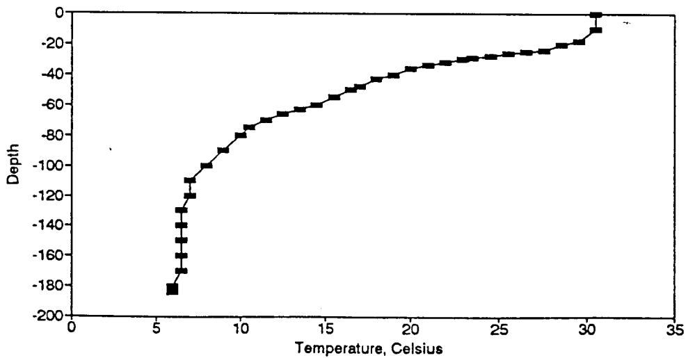
Figure BT90. Temperature Profile for the Eureka Springs Site-July 14, 1981.
