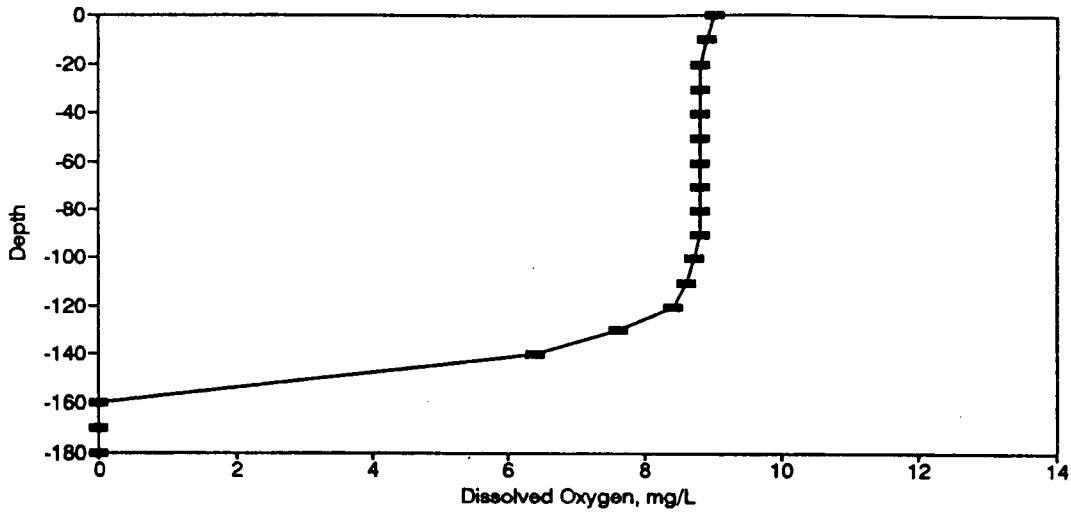
Figure BD73. Dissolved Oxygen Profile for the Eureka Springs Site-January 8, 1980.
