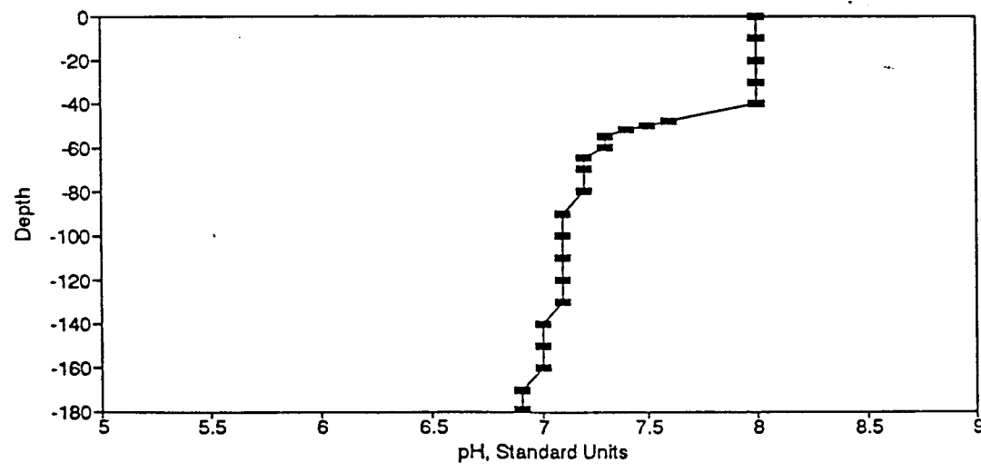
Figure BP117. pH Profile for the Eureka Springs Site-October 20, 1983.
