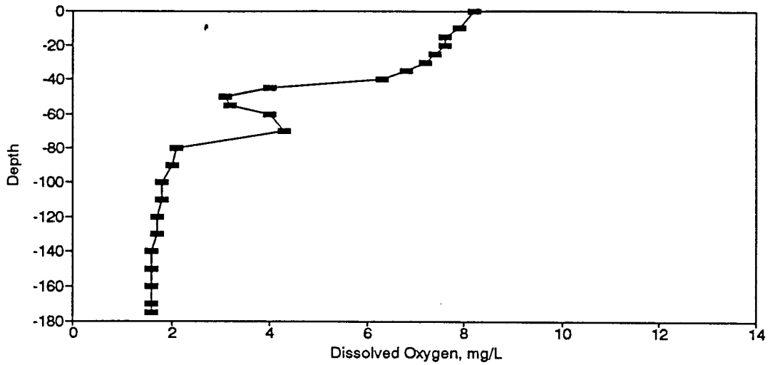
Figure BD22. Dissolved Oxygen Profile for the Eureka Springs Site-October 14, 1975.
