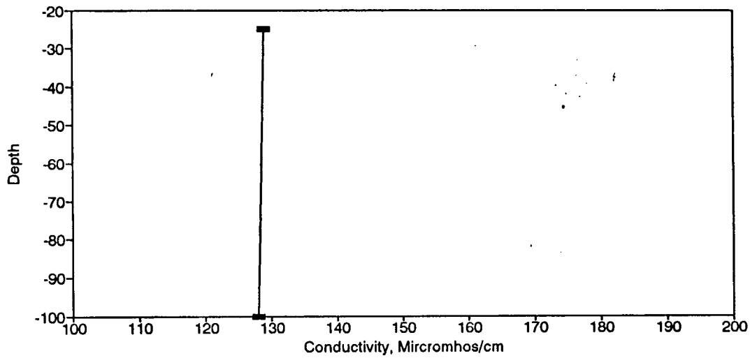
Figure BC188. Conductivity Profile for the Eureka Springs Site-January 10, 1990.
