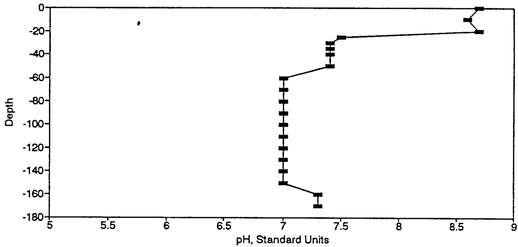
Figure BP19. pH Profile for the Eureka Springs Site-July 8, 1975.
