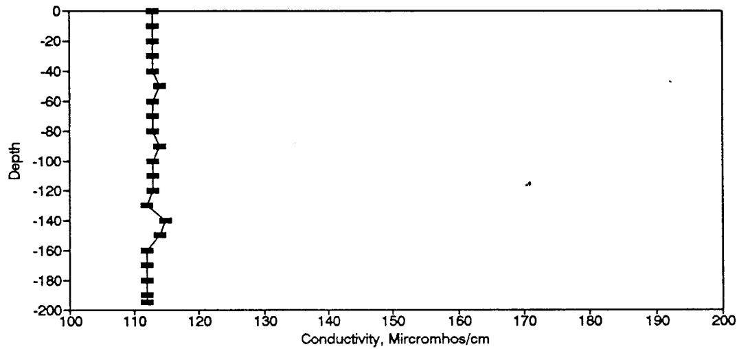
Figure BC5. Conductivity Profile for the Eureka Springs Site-April 16, 1974.
