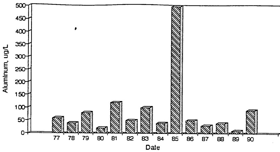
Figure A40. Graph of Aluminum vs. Time for the White River Site-Aug.
