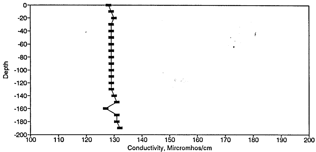
Figure BC158. Conductivity Profile for the Eureka Springs Site-March 11, 1987.
