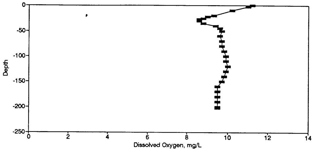
Figure BD136. Dissolved Oxygen Profile for the Eureka Springs Site-May 8, 1985.
