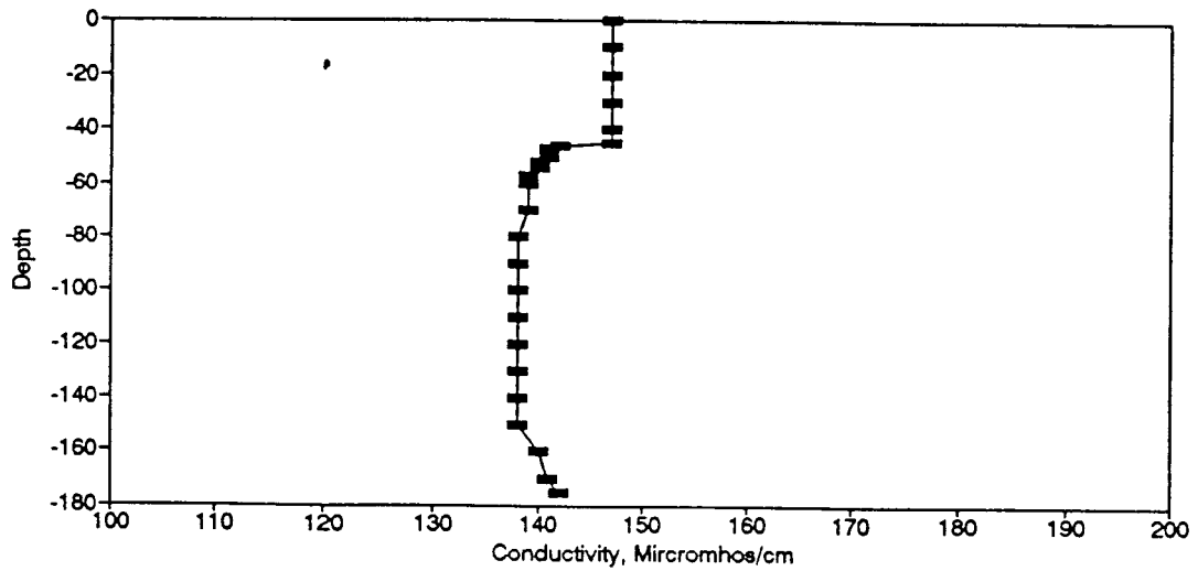
Figure BC82. Conductivity Profile for the Eureka Springs Site-October 6, 1980.
