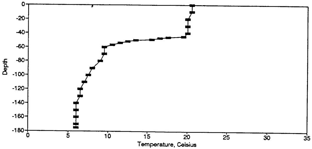
Figure BT82. Temperature Profile for the Eureka Springs Site-October 6, 1980.
