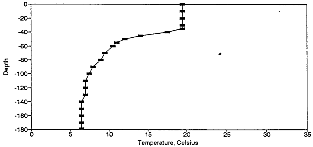
Figure BT47. Temperature Profile for the Eureka Springs Site-October 12, 1977.
