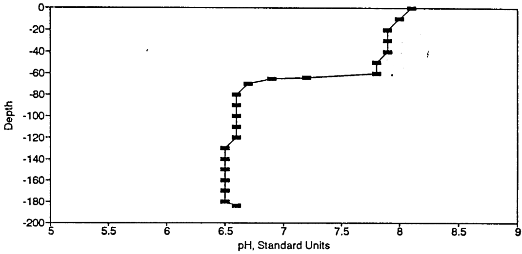
Figure BP71. pH Profile for the Eureka Springs Site-November 6, 1979.
