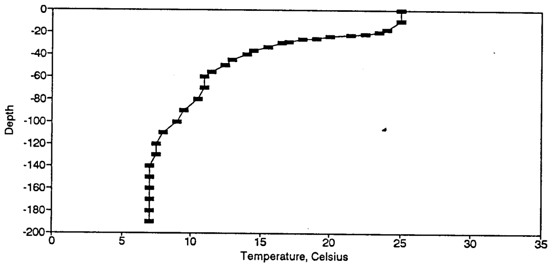
Figure BT173. Temperature Profile for the Eureka Springs Site-June 15, 1988.
