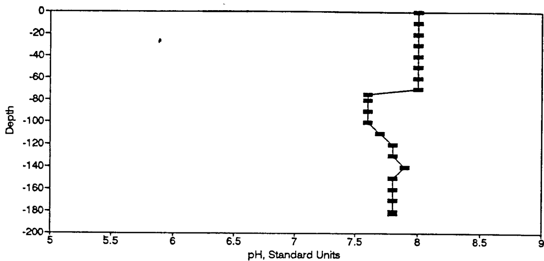
Figure BP49. pH Profile for the Eureka Springs Site-December 7, 1977.
