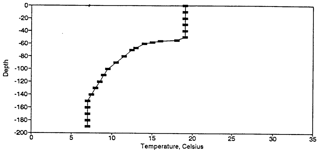
Figure BT70. Temperature Profile for the Eureka Springs Site-October 16, 1979.
