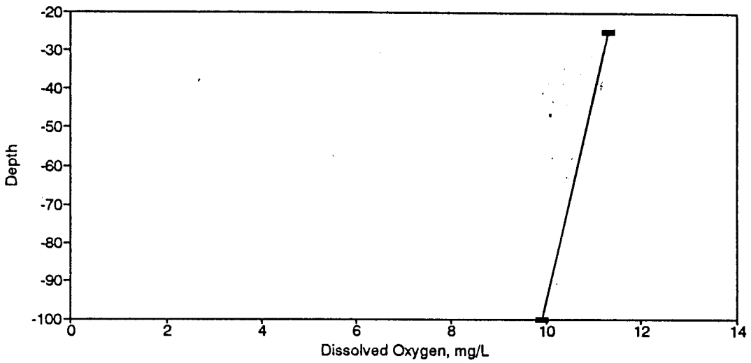
Figure BD188. Dissolved Oxygen Profile for the Eureka Springs Site-January 10, 1990.
