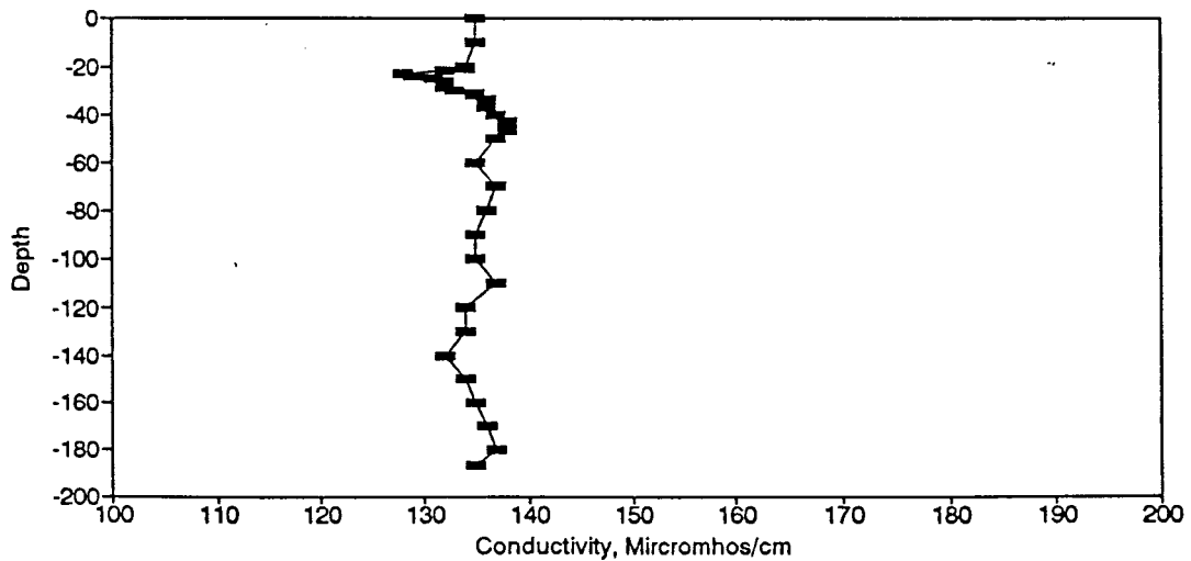
Figure BC174. Conductivity Profile for the Eureka Springs Site-July 12, 1988.
