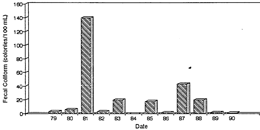
Figure A23. Graph of Fecal Coliform vs. Time for the White River Site-Aug.
