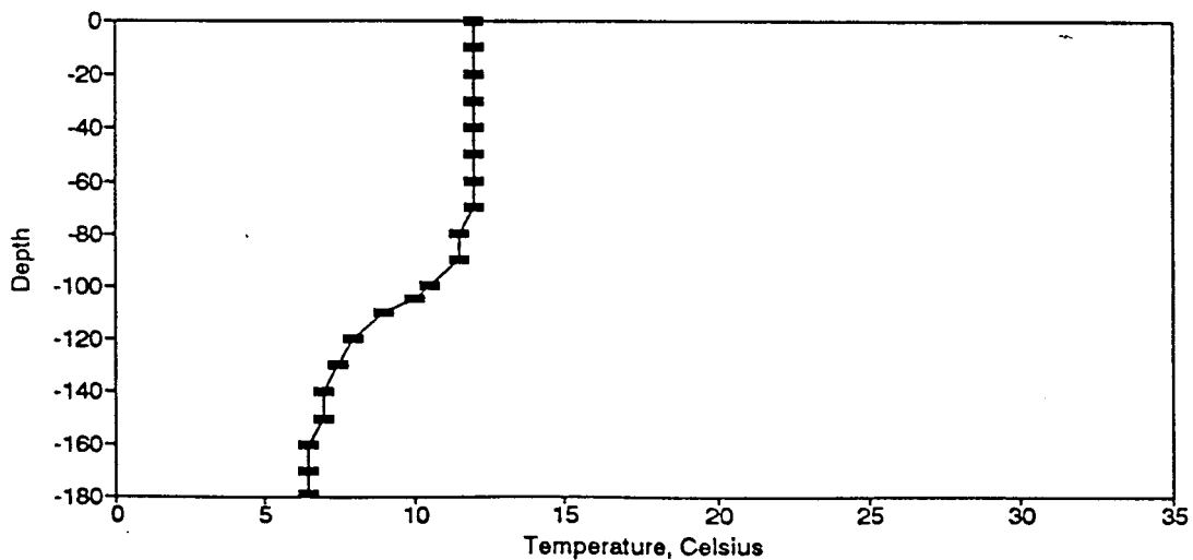
Figure BT60. Temperature Profile for the Eureka Springs Site-December 5, 1978.
