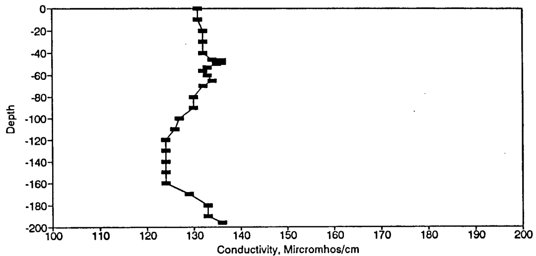
Figure BC153. Conductivity Profile for the Eureka Springs Site-October 9, 1986.
