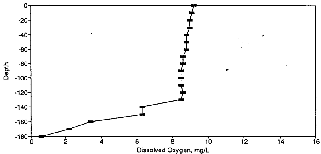
Figure BD50. Dissolved Oxygen Profile for the Eureka Springs Site-January 4, 1978.
