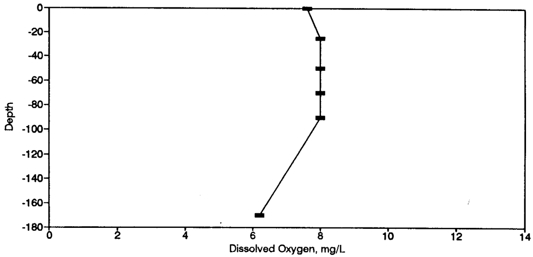
Figure BD19. Dissolved Oxygen Profile for the Eureka Springs Site-July 8, 1975.
