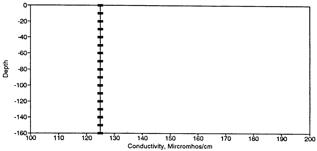
Figure BC37. Conductivity Profile for the Eureka Springs Site-January 26, 1977.
