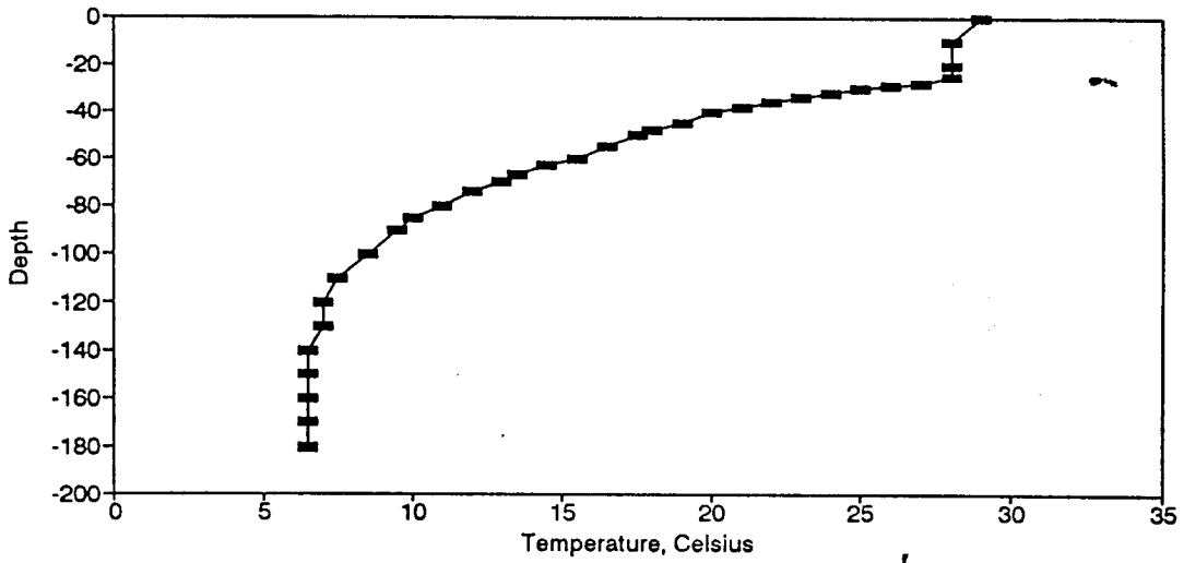
Figure BT91. Temperature Profile for the Eureka Springs Site-August 12, 1981.
