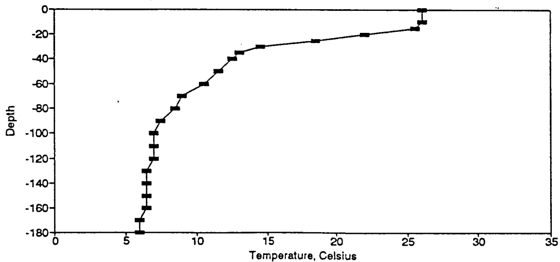
Figure BT42. Temperature Profile for the Eureka Springs Site-May 31, 1977.
