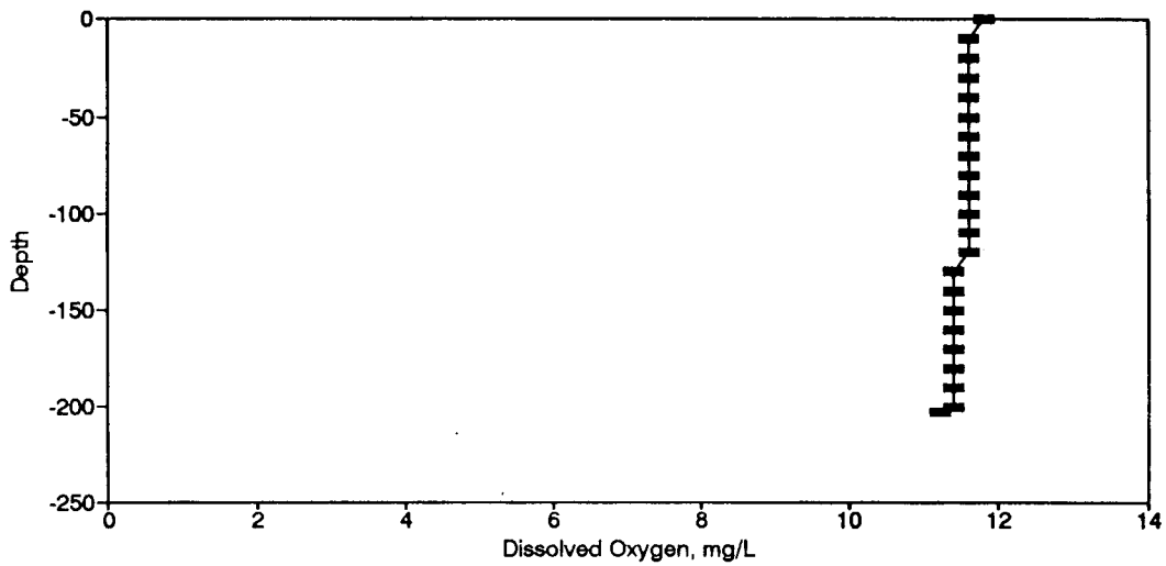
Figure BD133. Dissolved Oxygen Profile for the Eureka Springs Site-February 6, 1985.
