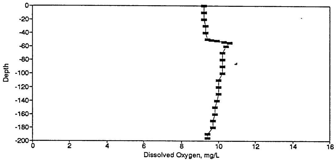
Figure BD65. Dissolved Oxygen Profile for the Eureka Springs Site-May 7, 1979.
