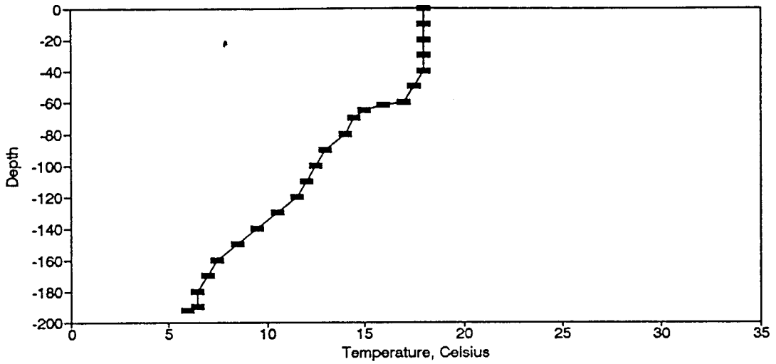
Figure BT142. Temperature Profile for the Eureka Springs Site-November 6, 1985.
