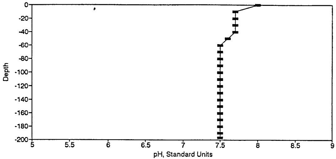
Figure BP109. pH Profile for the Eureka Springs Site-February 11, 1983.
