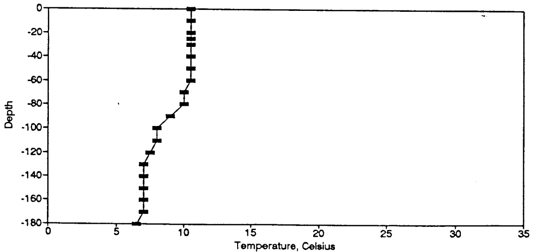
Figure BT84. Temperature Profile for the Eureka Springs Site-December 10, 1980.
