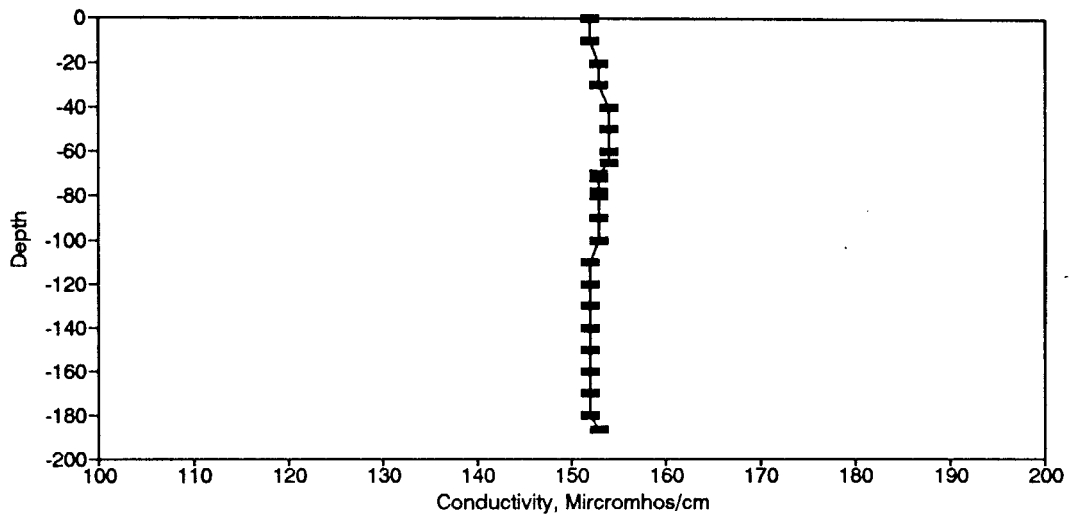
Figure BC87. Conductivity Profile for the Eureka Springs Site-April 13, 1981.
