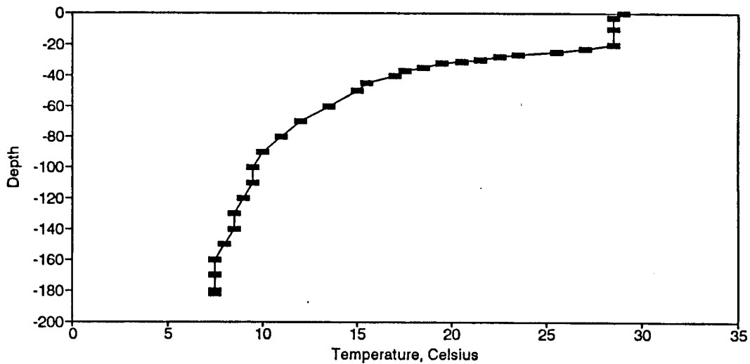
Figure BT151. Temperature Profile for the Eureka Springs Site-August 4, 1986.
