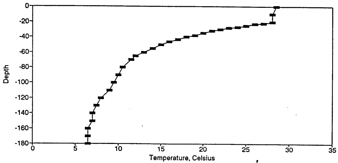
Figure BT103. Temperature Profile for the Eureka Springs Site-August 18, 1982.
