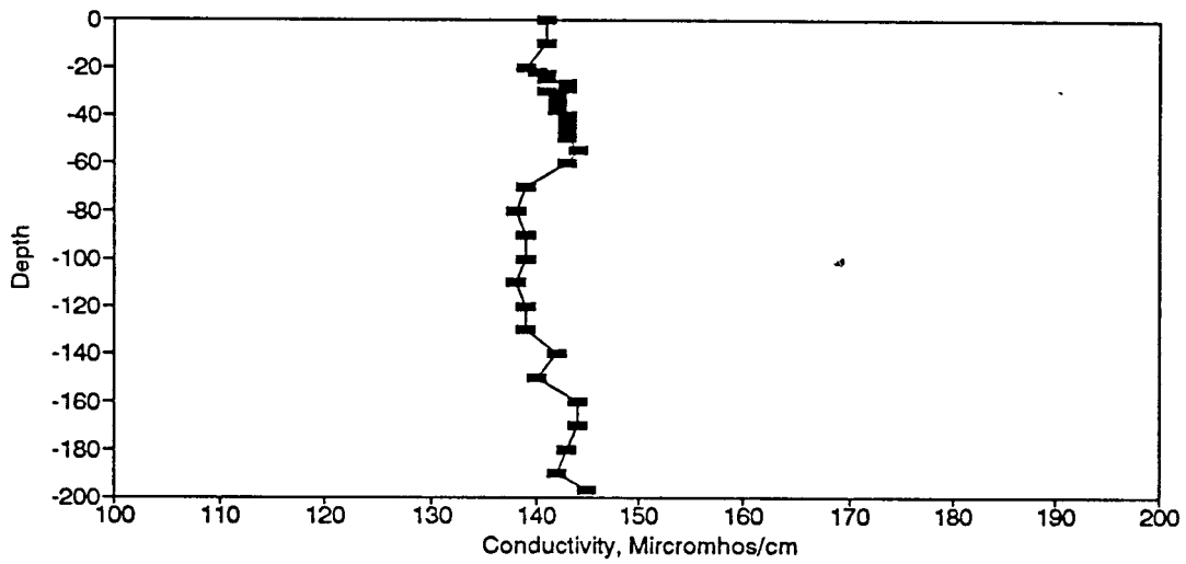
Figure BC185. Conductivity Profile for the Eureka Springs Site-July 13, 1989.
