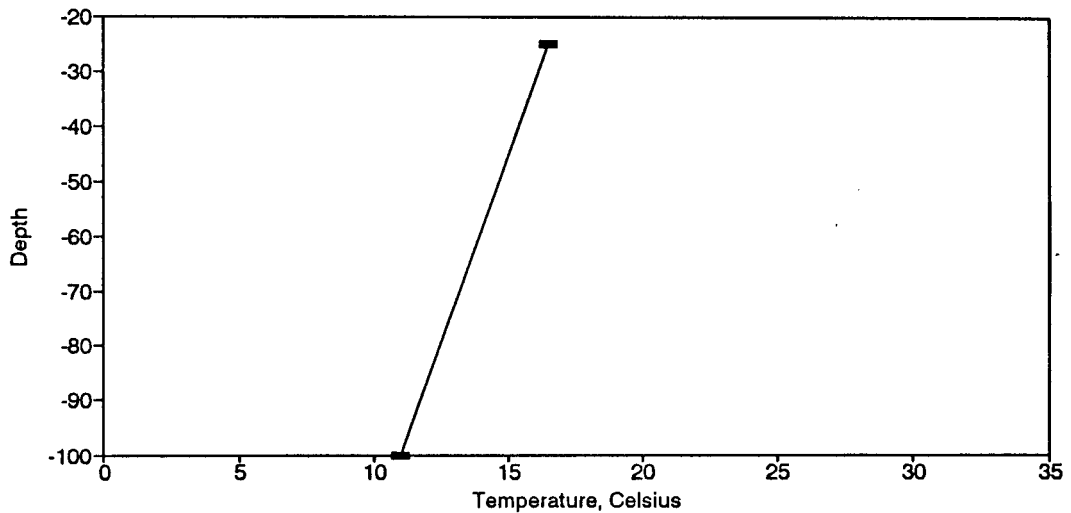
Figure BT189. Temperature Profile for the Eureka Springs Site-May 15, 1990.
