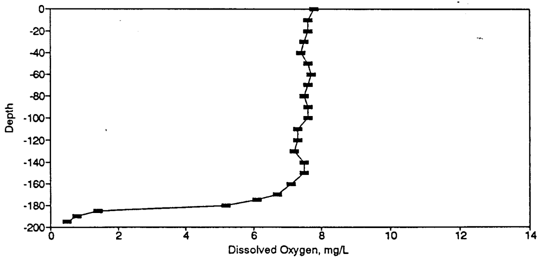
Figure BD12. Dissolved Oxygen Profile for the Eureka Springs Site-December 16, 1974.
