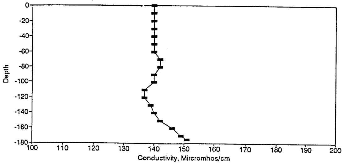
Figure BC106. Conductivity Profile for the Eureka Springs Site-November 24, 1982.
