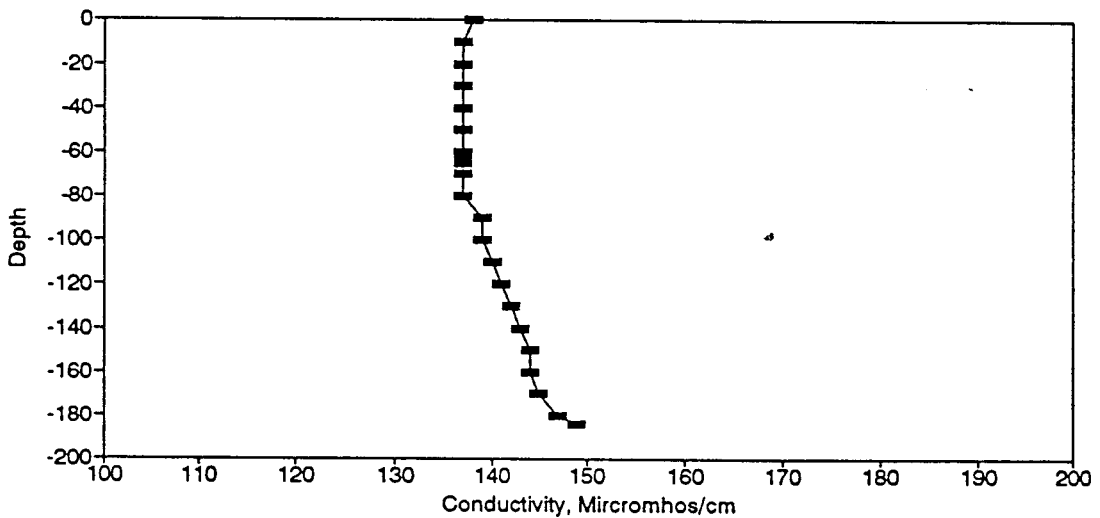
Figure BC71. Conductivity Profile for the Eureka Springs Site-November 6, 1979.
