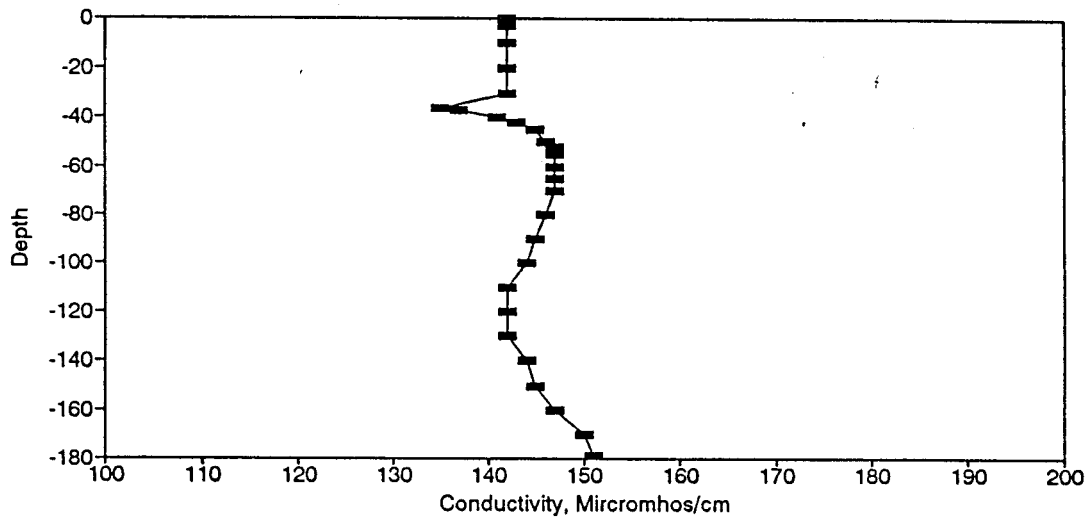
Figure BC104. Conductivity Profile for the Eureka Springs Site-September 23, 1982.
