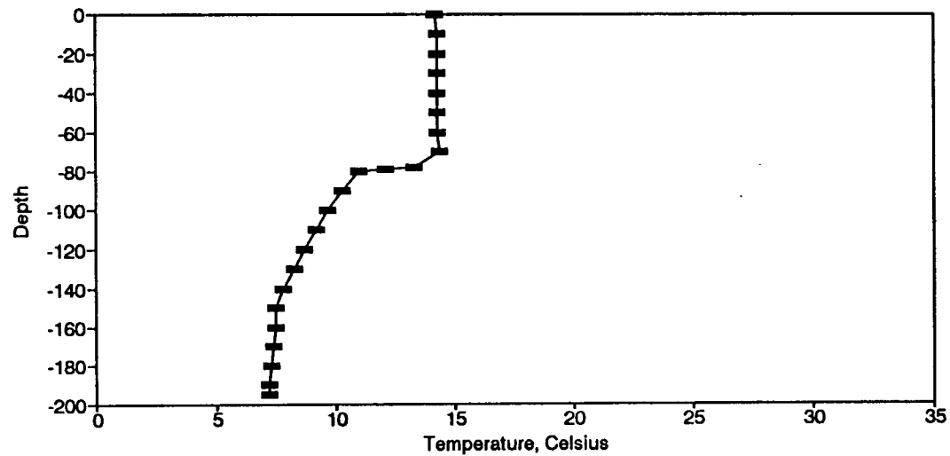
Figure BT177. Temperature Profile for the Eureka Springs Site-November 16, 1988.
