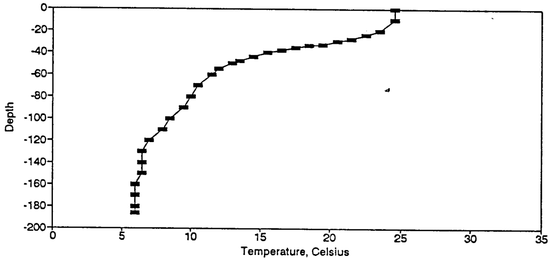
Figure BT101. Temperature Profile for the Eureka Springs Site-June 22, 1982.
