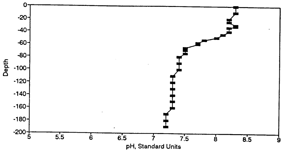
Figure BP88. pH Profile for the Eureka Springs Site-May 13, 1981.
