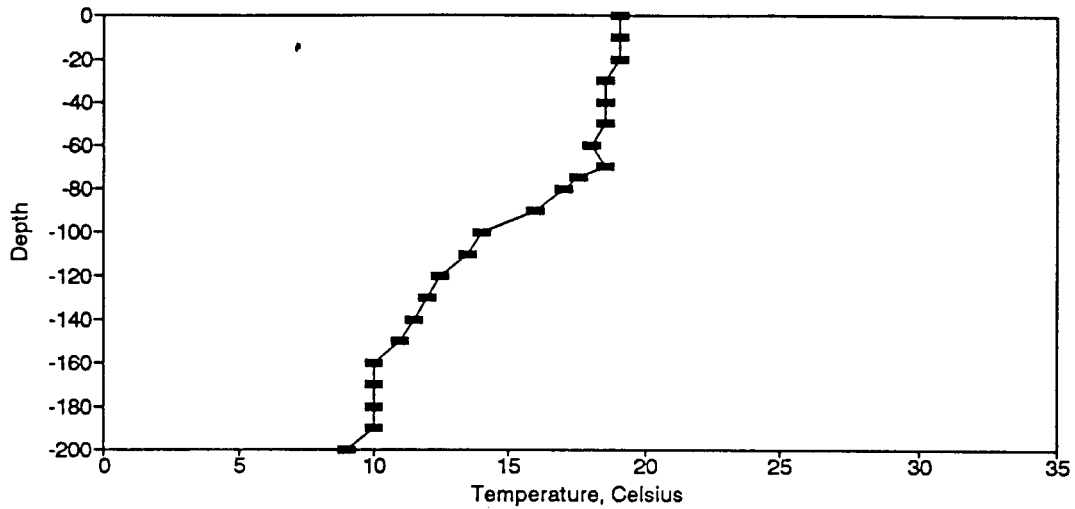
Figure BT10. Temperature Profile for the Eureka Springs Site-October 22, 1974.
