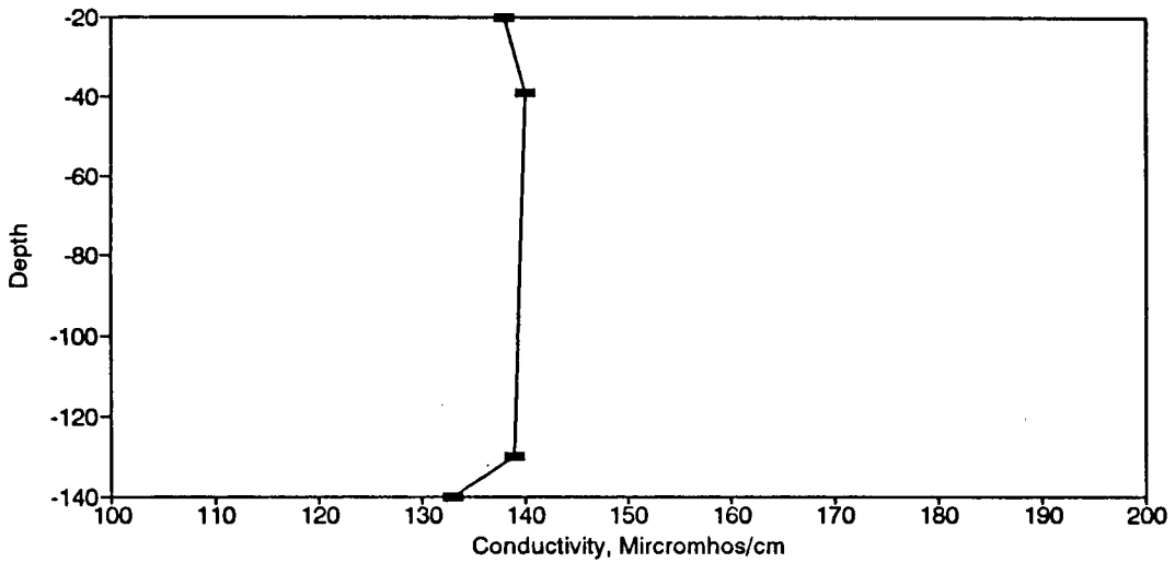
Figure BC187. Conductivity Profile for the Eureka Springs Site-September 11, 1989.
