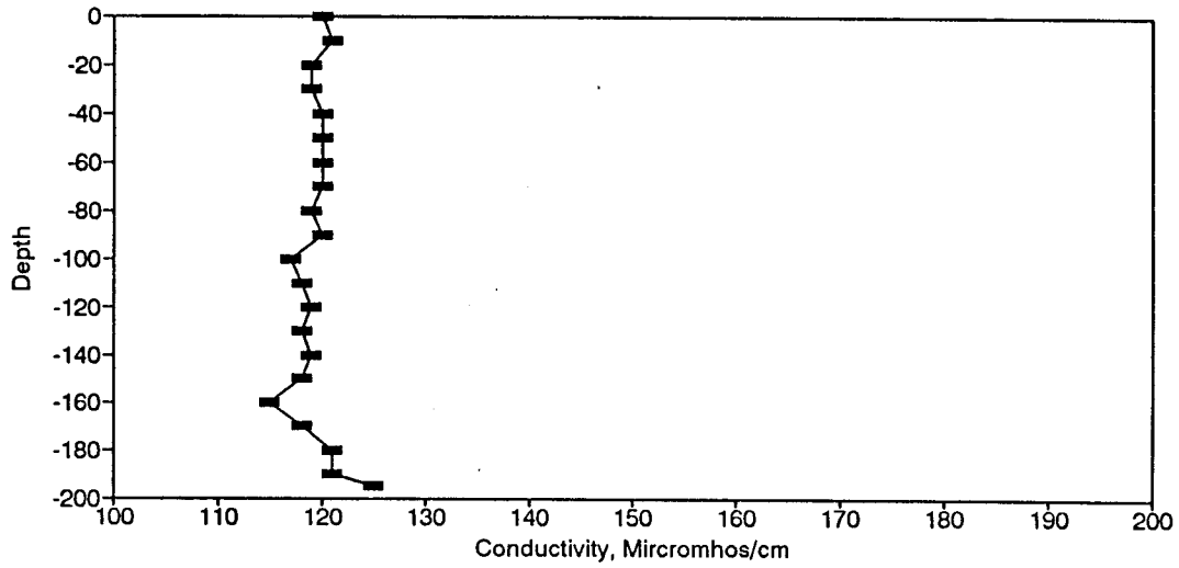
Figure BC145. Conductivity Profile for the Eureka Springs Site-February 20, 1986.
