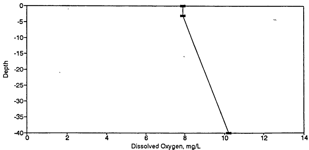
Figure BD162. Dissolved Oxygen Profile for the Eureka Springs Site-July 15, 1987.
