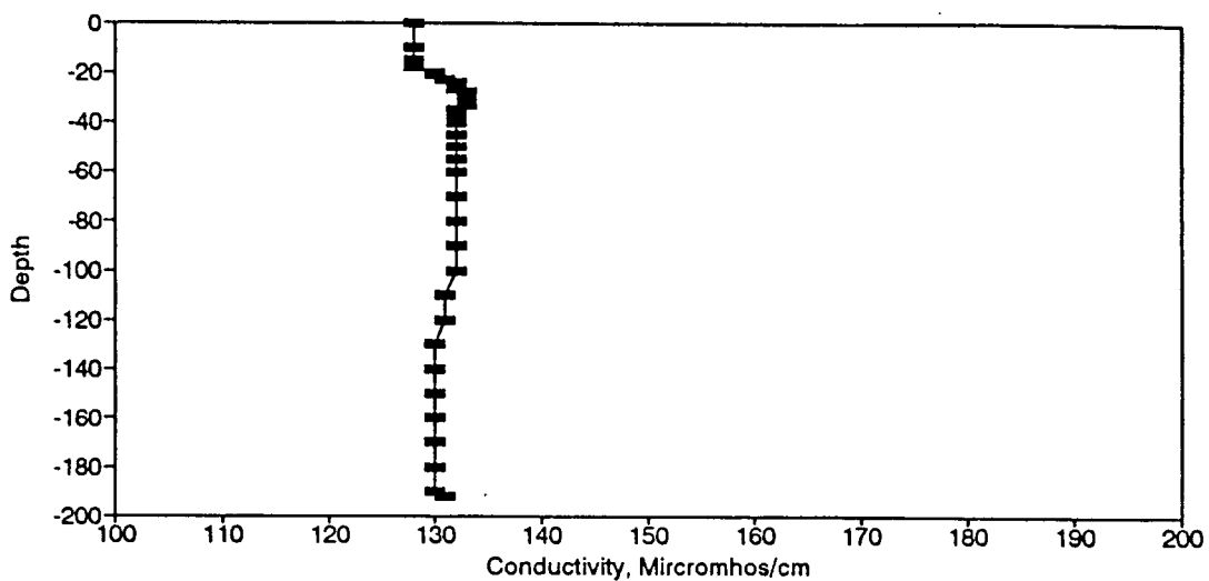
Figure BC67. Conductivity Profile for the Eureka Springs Site-July 17, 1979.
