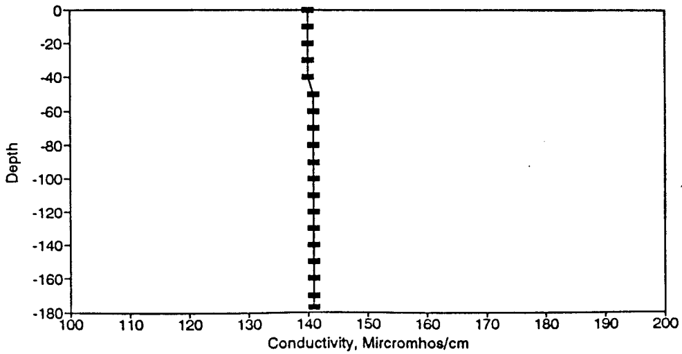
Figure BC75. Conductivity Profile for the Eureka Springs Site-March 12, 1980.
