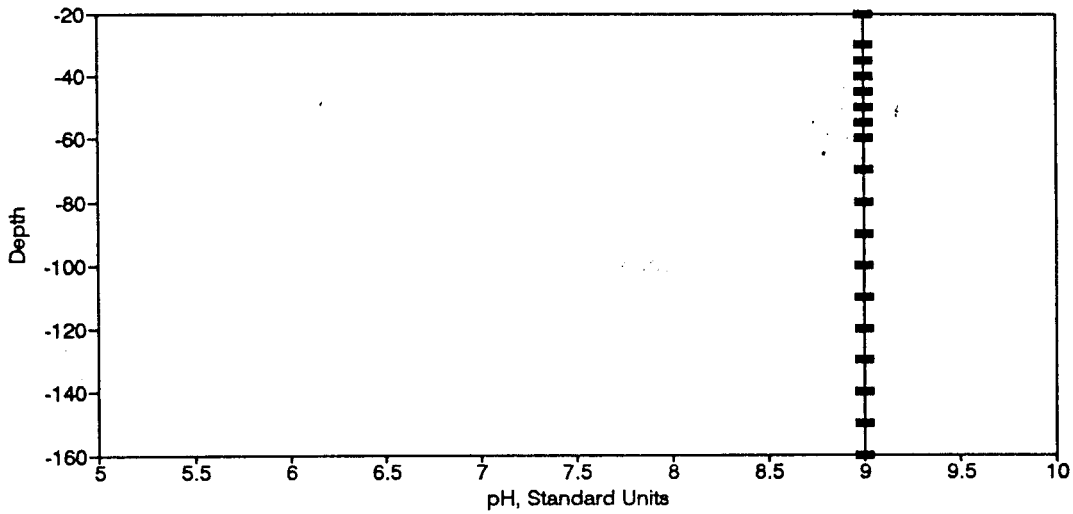
Figure BP47. pH Profile for the Eureka Springs Site-October 12, 1977.
