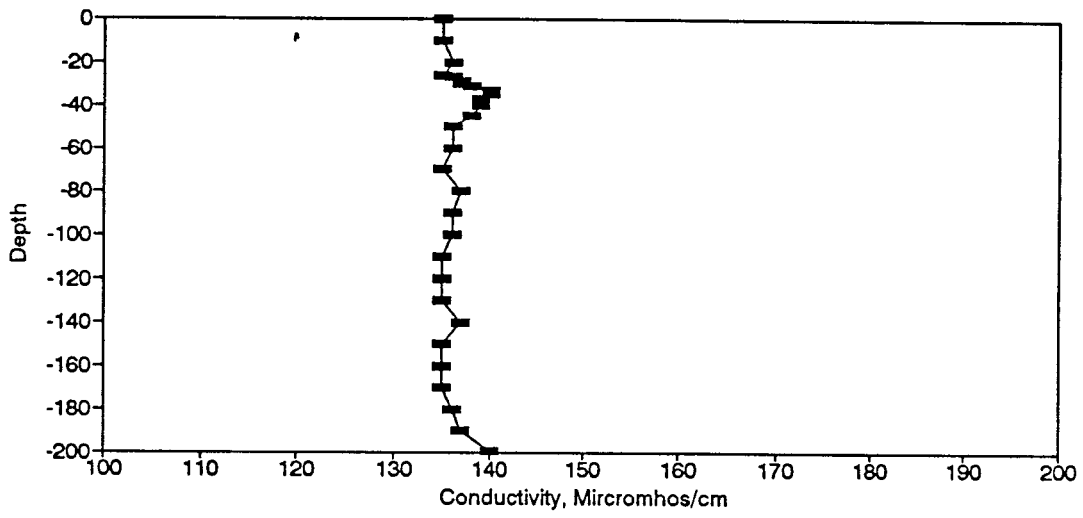
Figure BC184. Conductivity Profile for the Eureka Springs Site-June 7, 1989.
