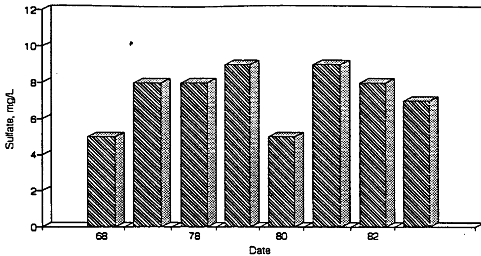
Figure A100. Graph of Sulfate vs. Time for the White River Site-May.
