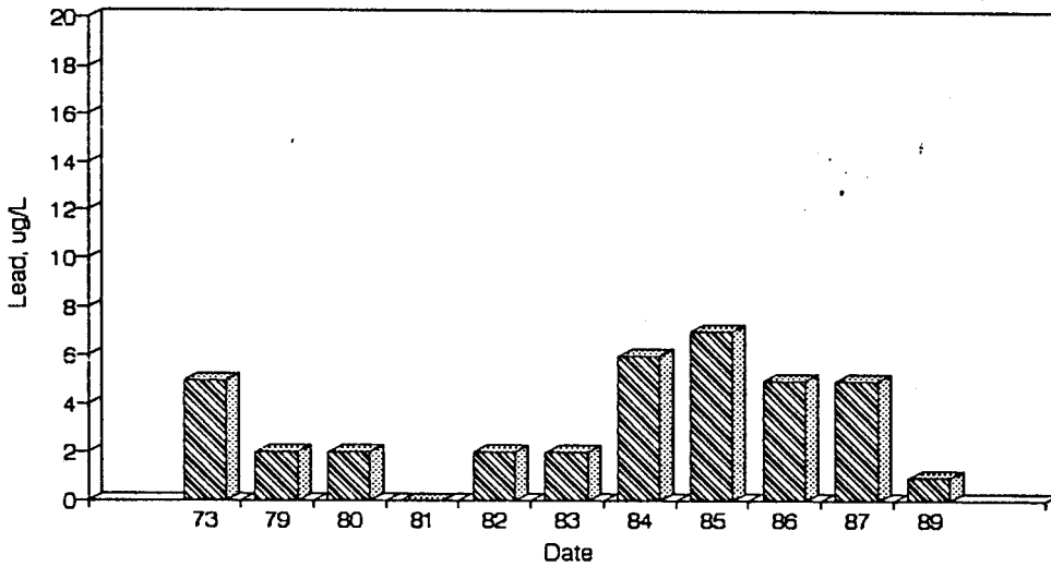
Figure A56. Graph of Lead vs. Time for the White River Site-Aug.
