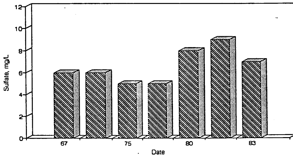
Figure A102. Graph of Sulfate vs. Time for the White River Site-Dec.
