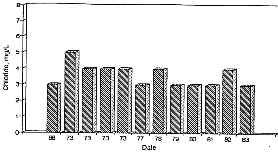
Figure A7. Graph of Chloride vs. Time for the White River Site-May.
