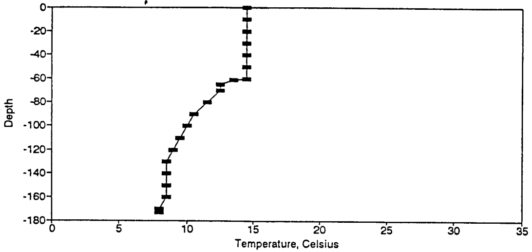
Figure BT118. Temperature Profile for the Eureka Springs Site-November 14, 1983.
