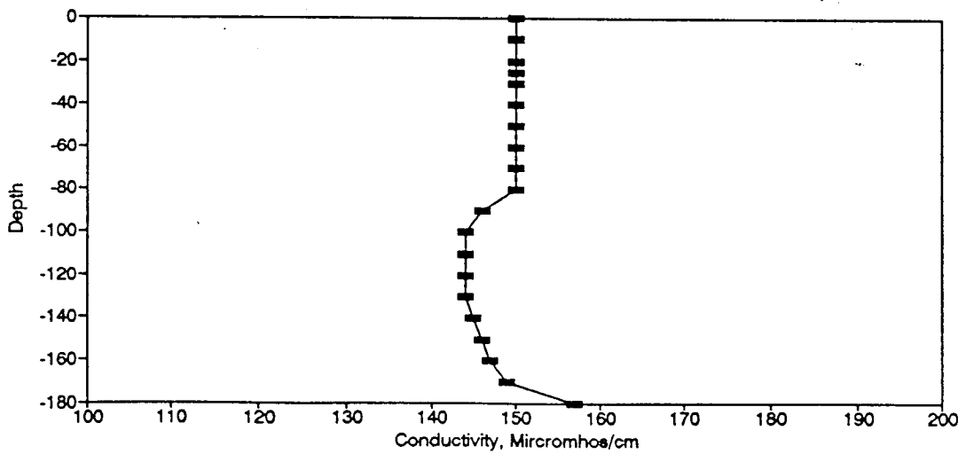
Figure BC84. Conductivity Profile for the Eureka Springs Site-December 10, 1980.
