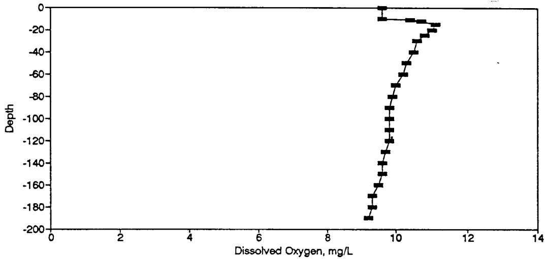
Figure BD77. Dissolved Oxygen Profile for the Eureka Springs Site-May 7, 1980.
