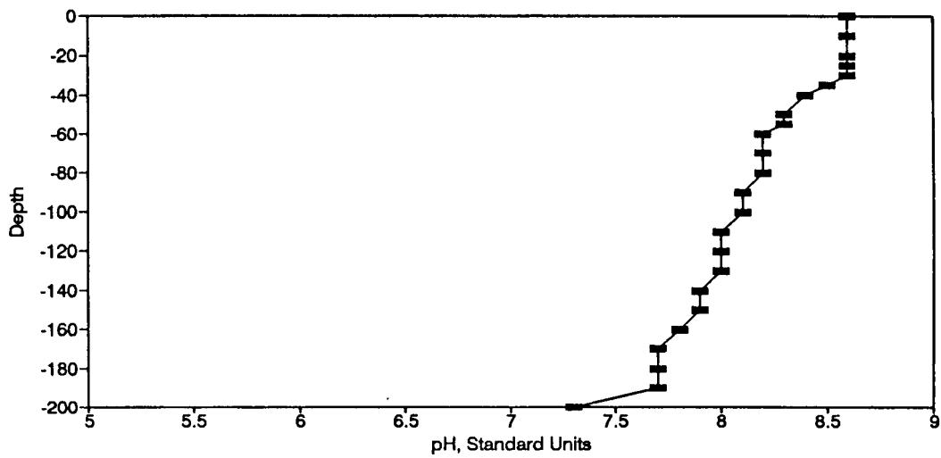
Figure BP112. pH Profile for the Eureka Springs Site-May 18 1983.
