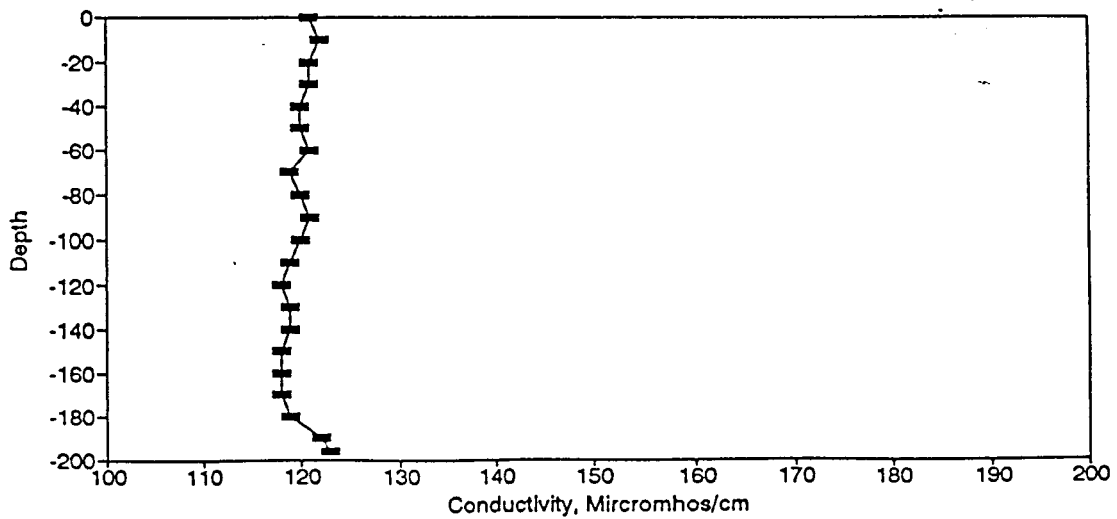
Figure BC144. Conductivity Profile for the Eureka Springs Site-Januray 8, 1986.
