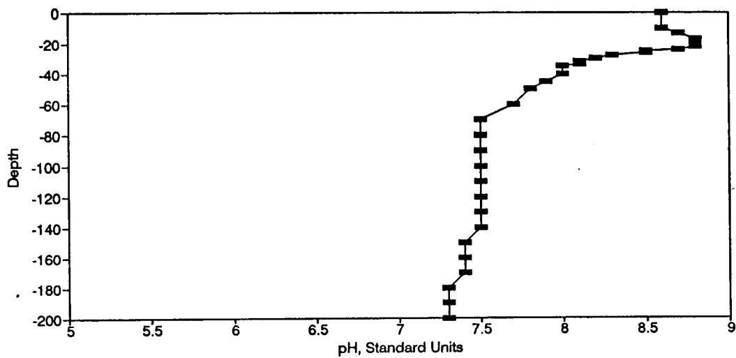
Figure BP114. pH Profile for the Eureka Springs Site-July 12, 1983.
