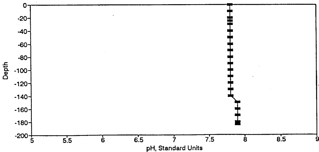
Figure BP108. pH Profile for the Eureka Springs Site-January 25, 1983.
