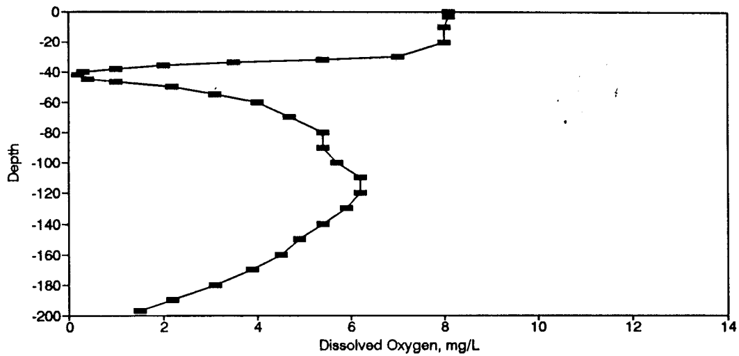
Figure BD140. Dissolved Oxygen Profile for the Eureka Springs Site-September 6, 1985.
