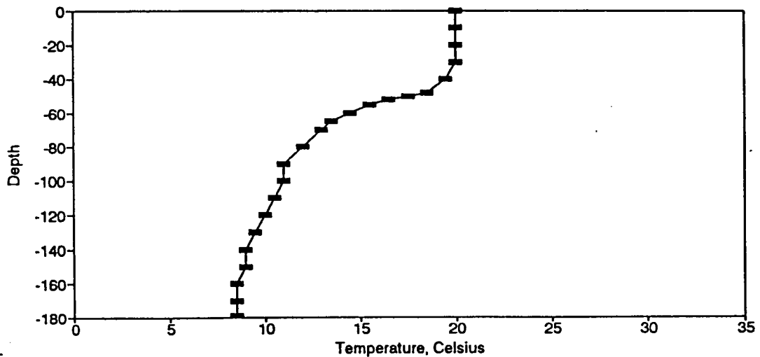
Figure BT117. Temperature Profile for the Eureka Springs Site-October 20, 1983.
