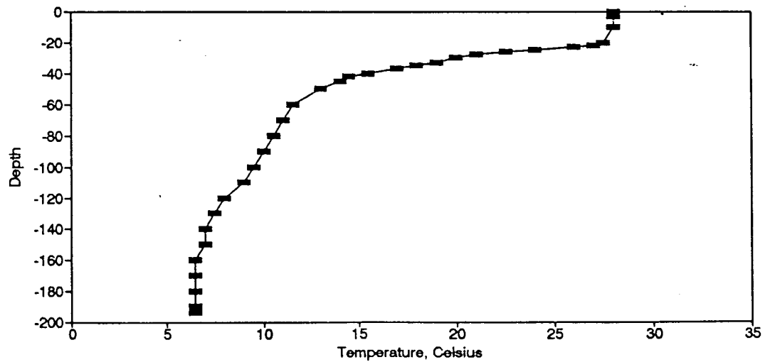
Figure BT138. Temperature Profile for the Eureka Springs Site-July 11, 1985.
