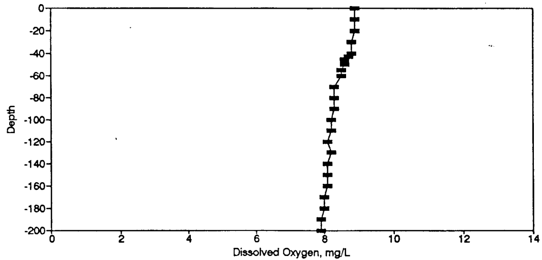
Figure BD6. Dissolved Oxygen Profile for the Eureka Springs Site-May 14, 1974.
