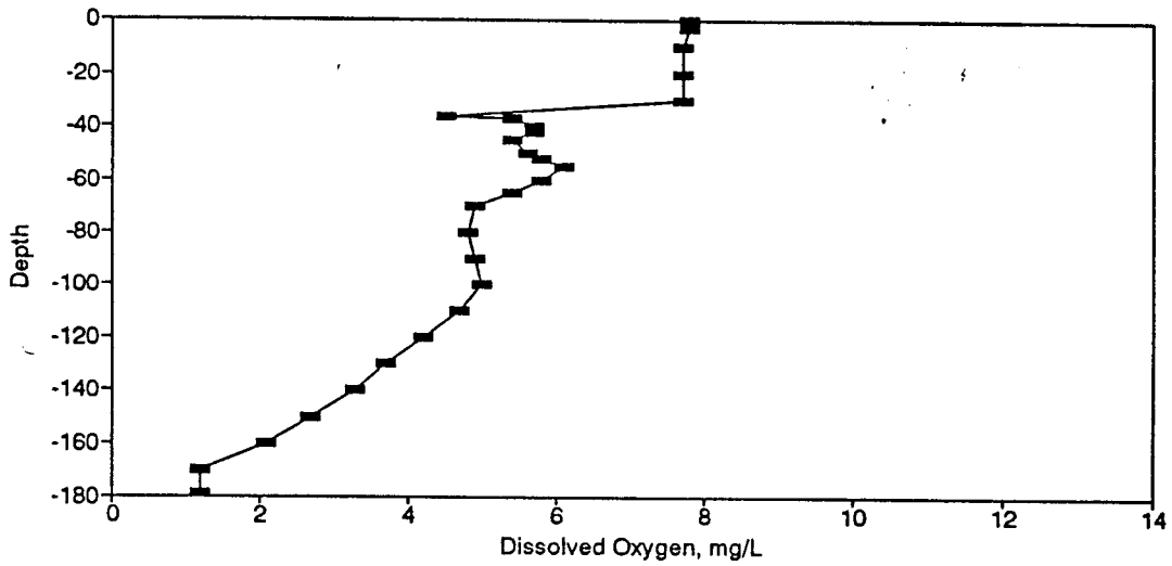
Figure BD104. Dissolved Oxygen Profile for the Eureka Springs Site-September 23, 1982.
