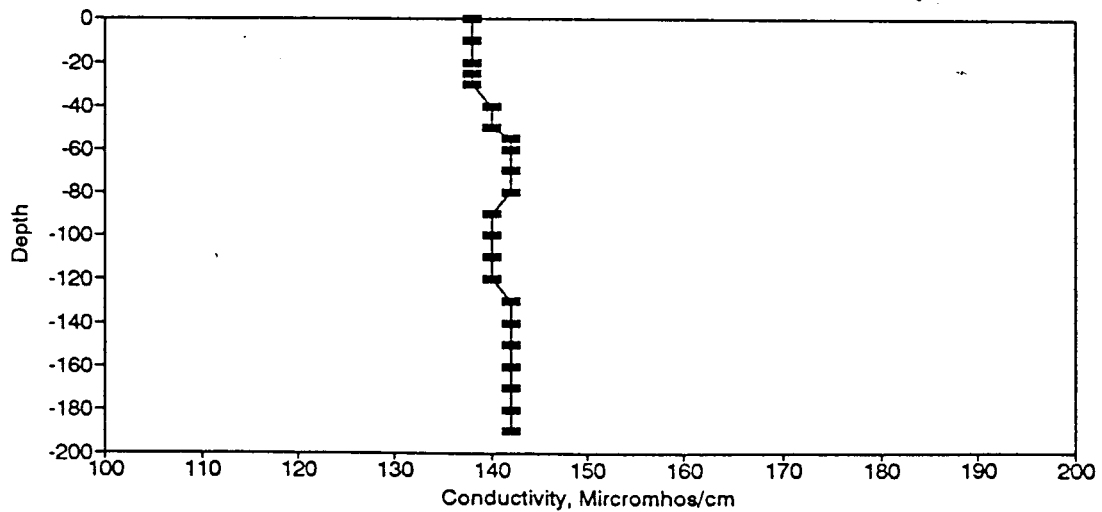
Figure BC54. Conductivity Profile for the Eureka Springs Site-June 15, 1978.
