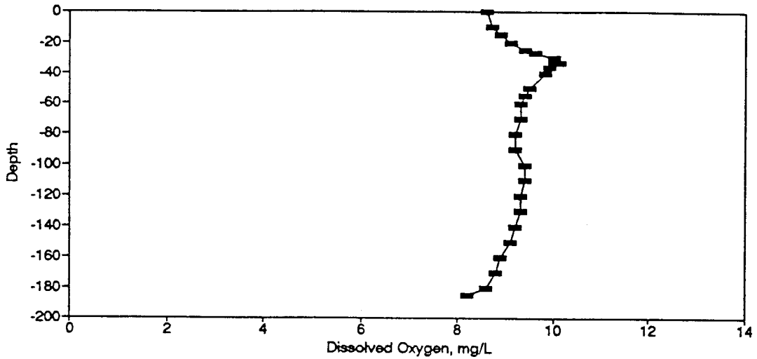
Figure BD100. Dissolved Oxygen Profile for the Eureka Springs Site-May 19, 1982.
