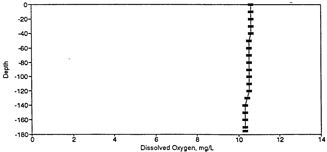
Figure BD96. Dissolved Oxygen Profile for the Eureka Springs Site-January 26, 1982.
