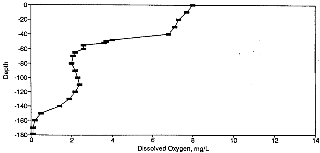
Figure BD117. Dissolved Oxygen Profile for the Eureka Springs Site-October 20, 1983.
