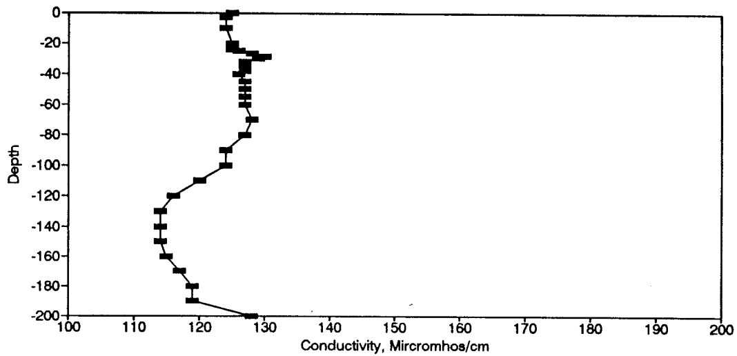
Figure BC139. Conductivity Profile for the Eureka Springs Site-August 7, 1985.
