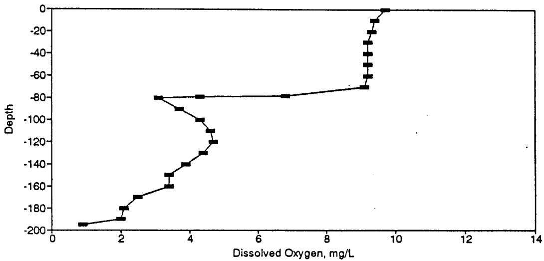
Figure BD177. Dissolved Oxygen Profile for the Eureka Springs Site-November 16, 1988.
