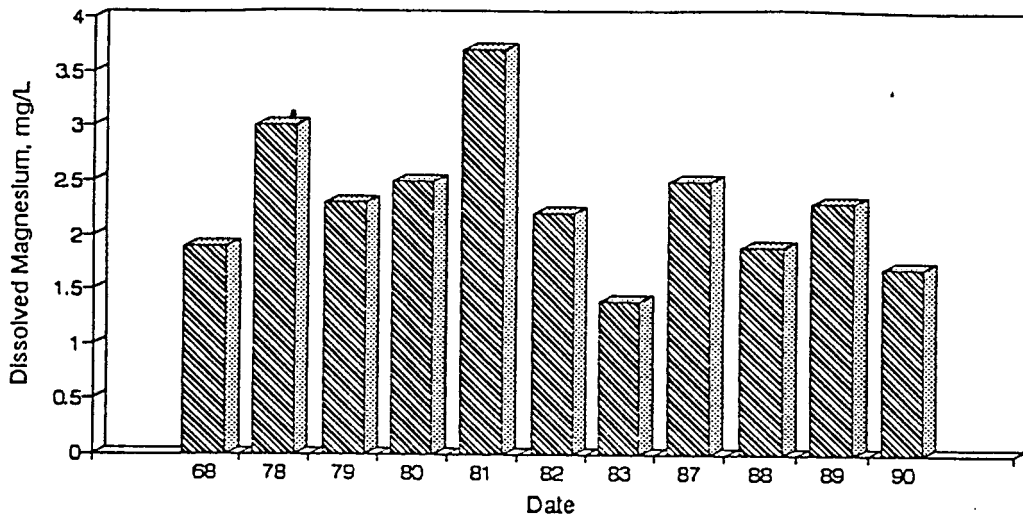
Figure A34. Graph of Dissolved Magnesium vs. Time for the White River Site-May.
