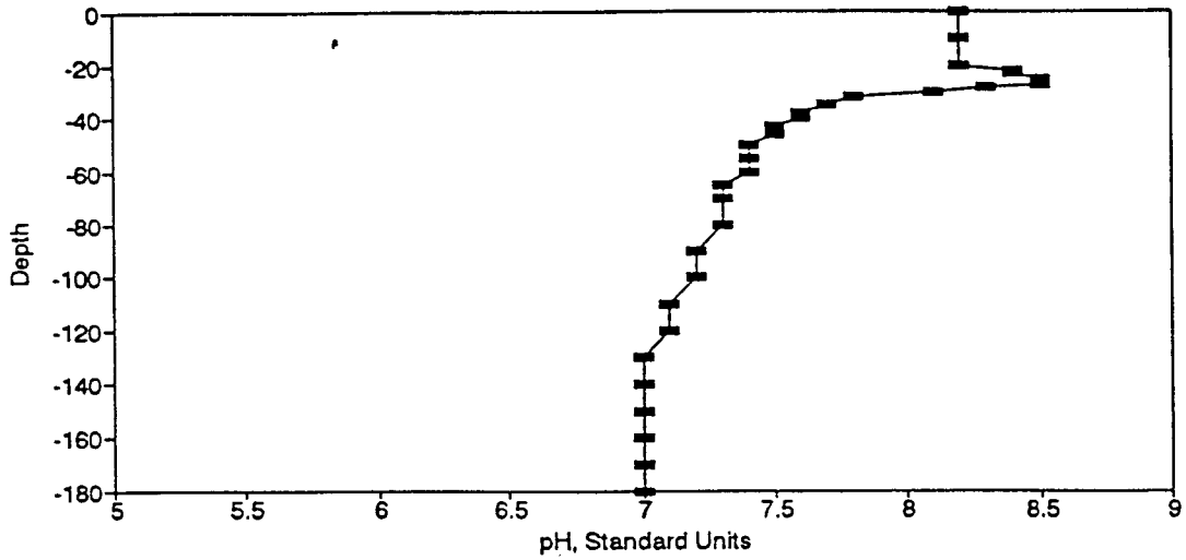
Figure BP103. pH Profile for the Eureka Springs Site-August 18, 1982.
