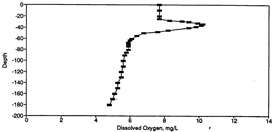
Figure BD91. Dissolved Oxygen Profile for the Eureka Springs Site-August 12, 1981.
