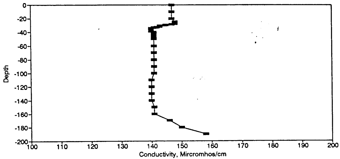
Figure BC80. Conductivity Profile for the Eureka Springs Site - August 13, 1980.
