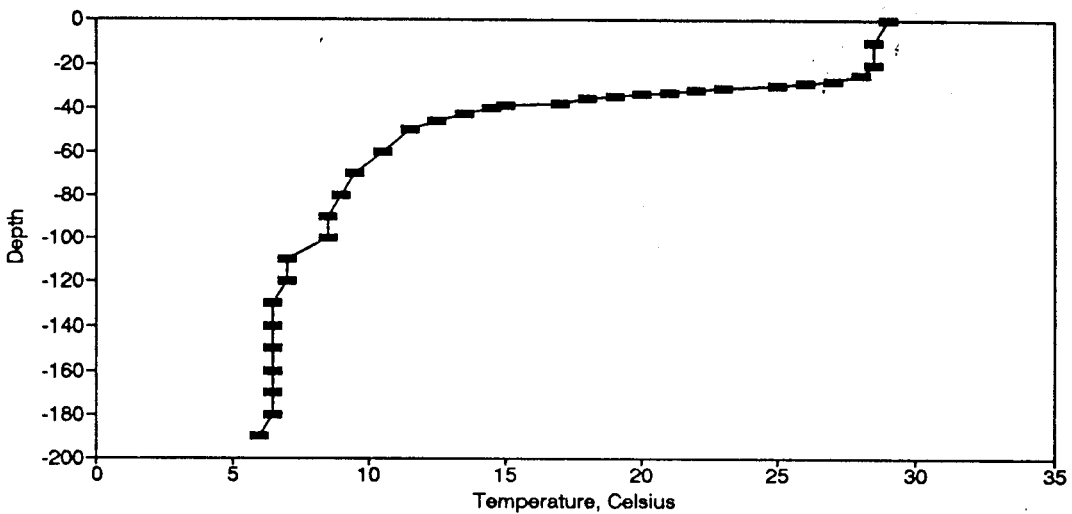
Figure BT80. Temperature Profile for the Eureka Springs Site-August 13, 1980.
