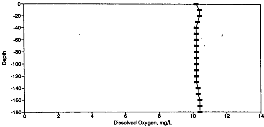
Figure BD74. Dissolved Oxygen Profile for the Eureka Springs Site-February 14, 1980.
