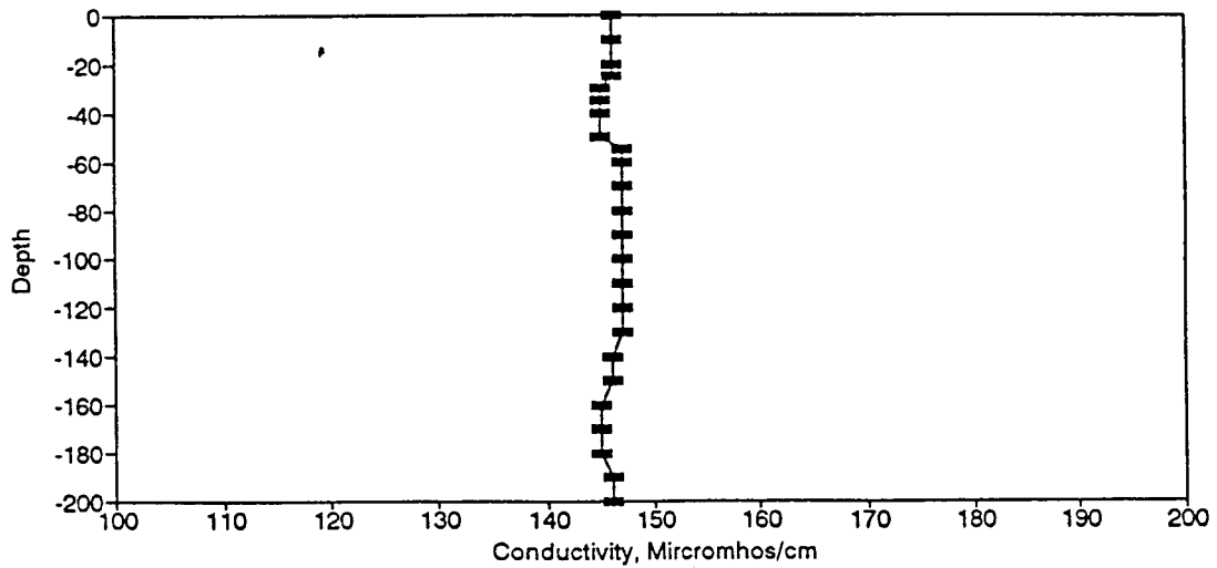
Figure BC112. Conductivity Profile for the Eureka Springs Site-May 18 1983.
