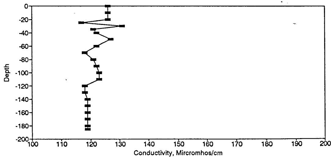
Figure BC18. Conductivity Profile for the Eureka Springs Site-June 11, 1975.
