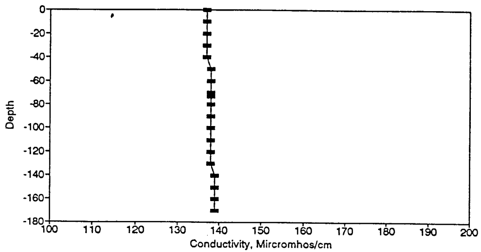
Figure BC76. Conductivity Profile for the Eureka Springs Site-April 8, 1980.
