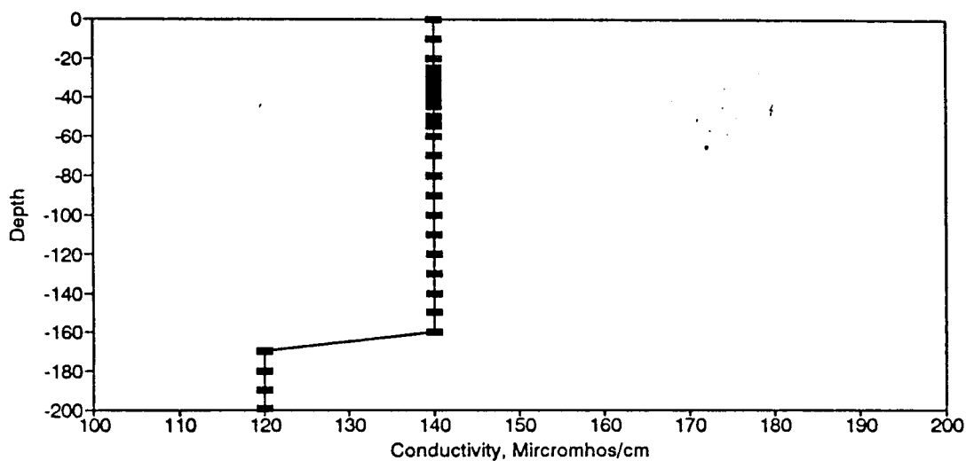
Figure BC68. Conductivity Profile for the Eureka Springs Site-August 22, 1979.
