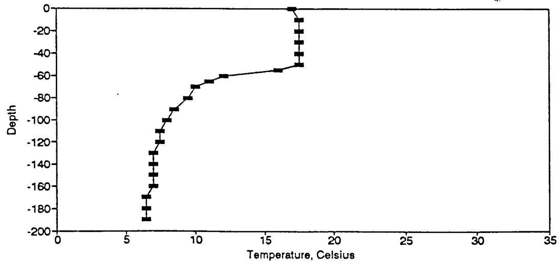
Figure BT48. Temperature Profile for the Eureka Springs Site-November 9, 1977.
