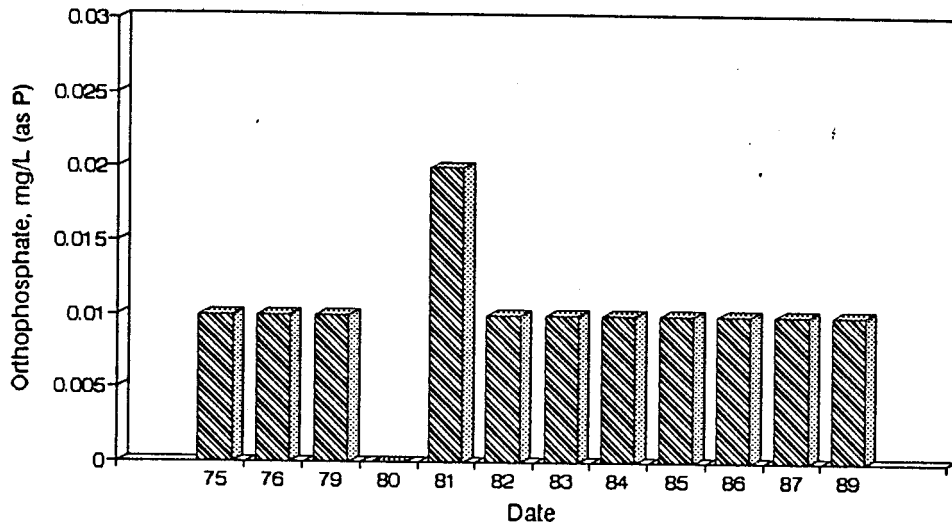
Figure A98. Graph of Orthophosphate vs. Time for the White River Site-Aug.
