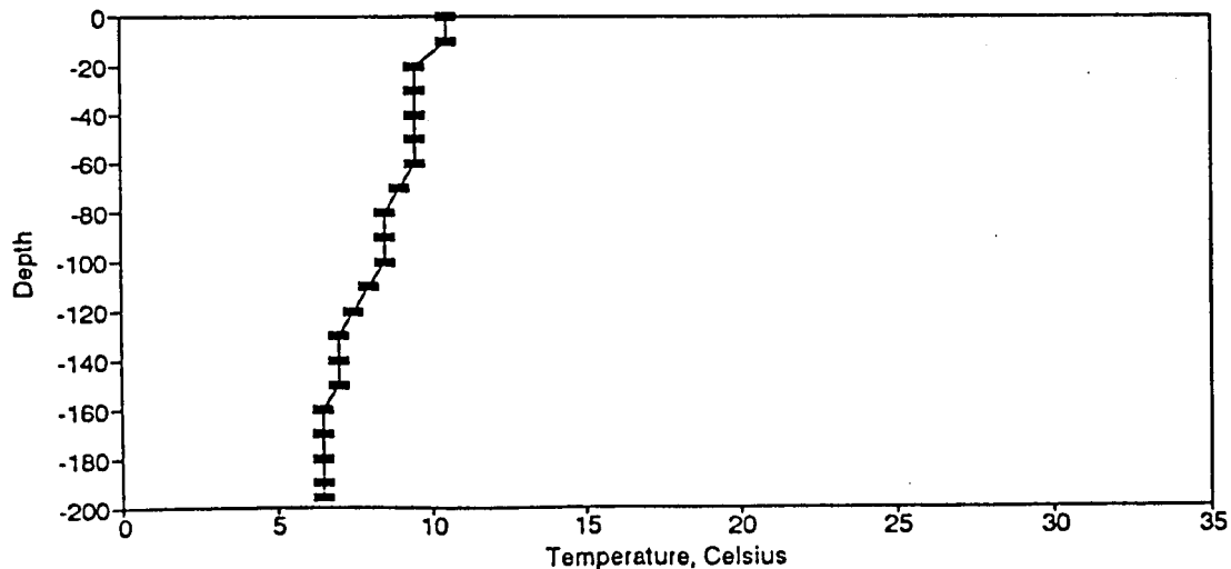
Figure BT111. Temperature Profile for the Eureka Springs Site, April 21, 1983.
