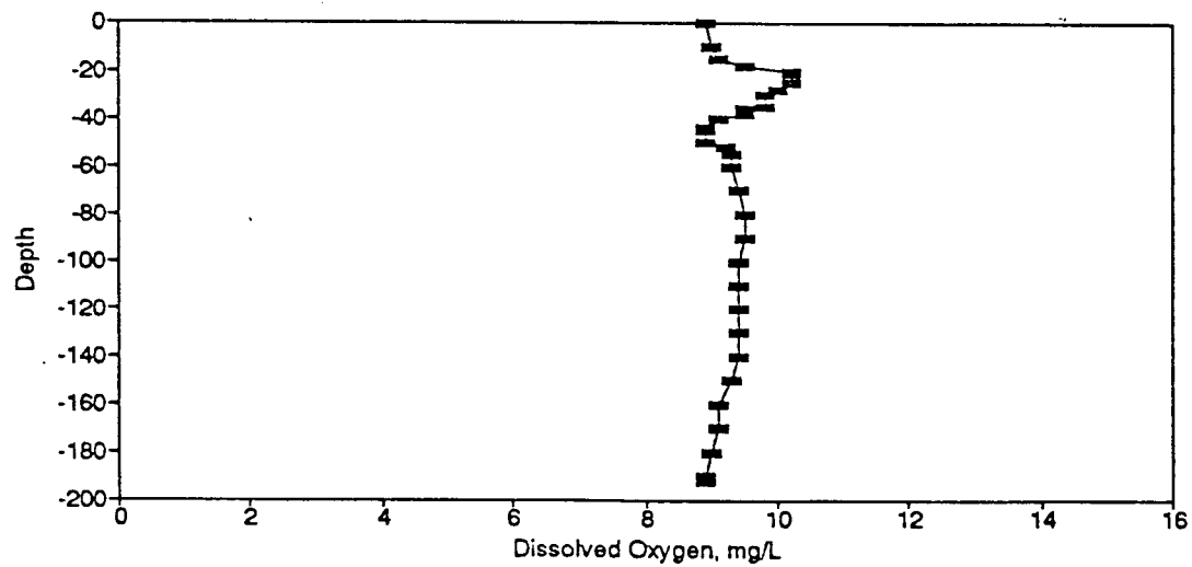
Figure BD66. Dissolved Oxygen Profile for the Eureka Springs Site-June 6, 1979.
