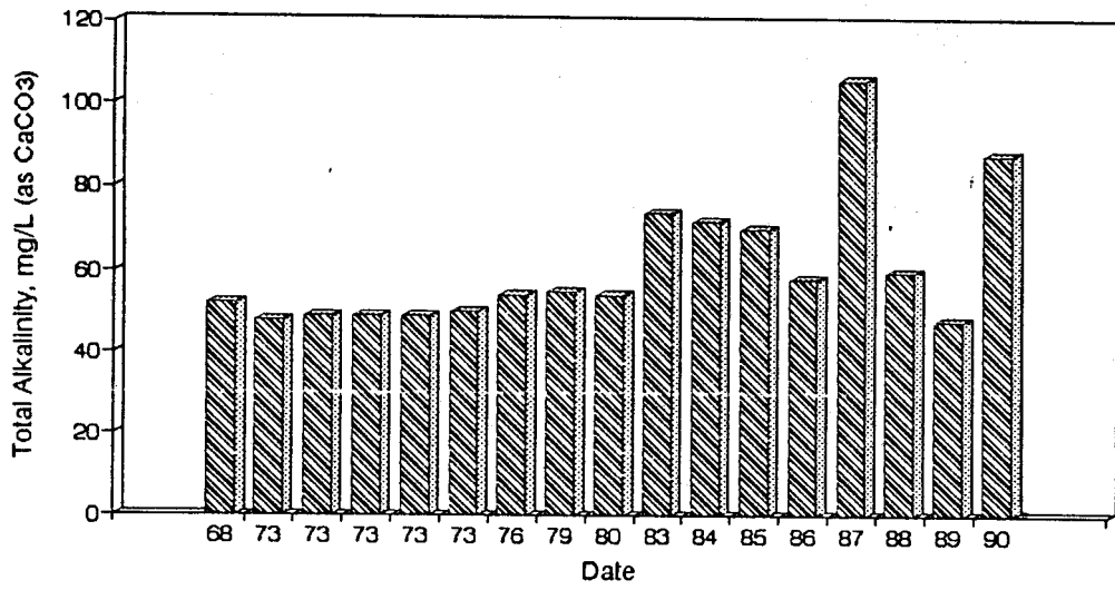
Figure A2. Graph of Total Alkalinity vs. Time for the White River Site-Aug.
