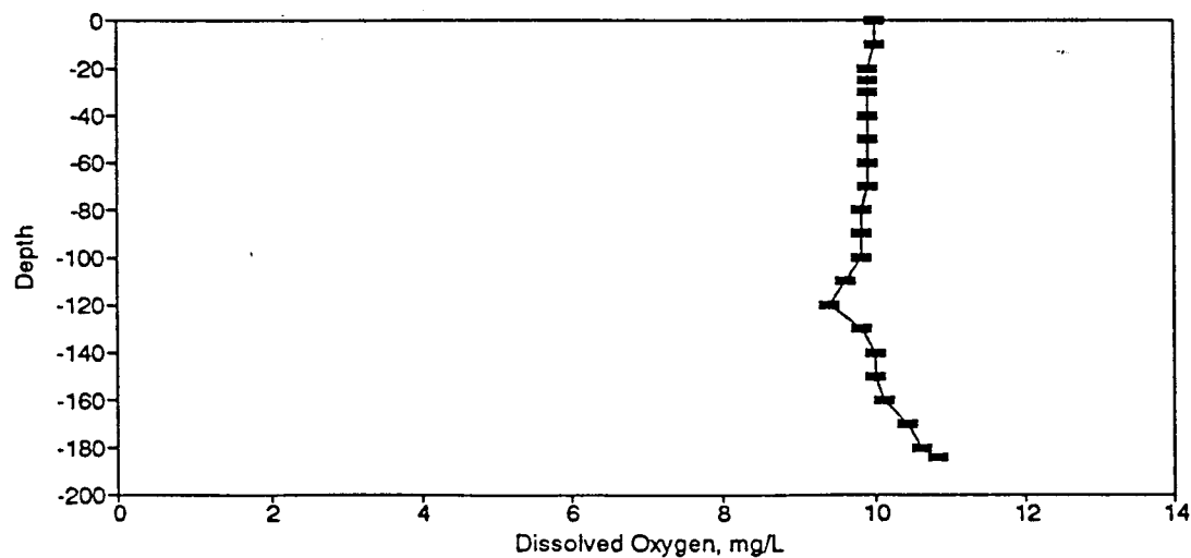
Figure BD108. Dissolved Oxygen Profile for the Eureka Springs Site-January 25, 1983.
