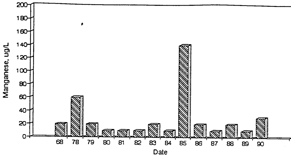
Figure A58. Graph of Manganese vs. Time for the White River Site-May.
