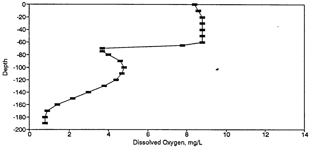
Figure BD23. Dissolved Oxygen Profile for the Eureka Springs Site-November 18, 1975.
