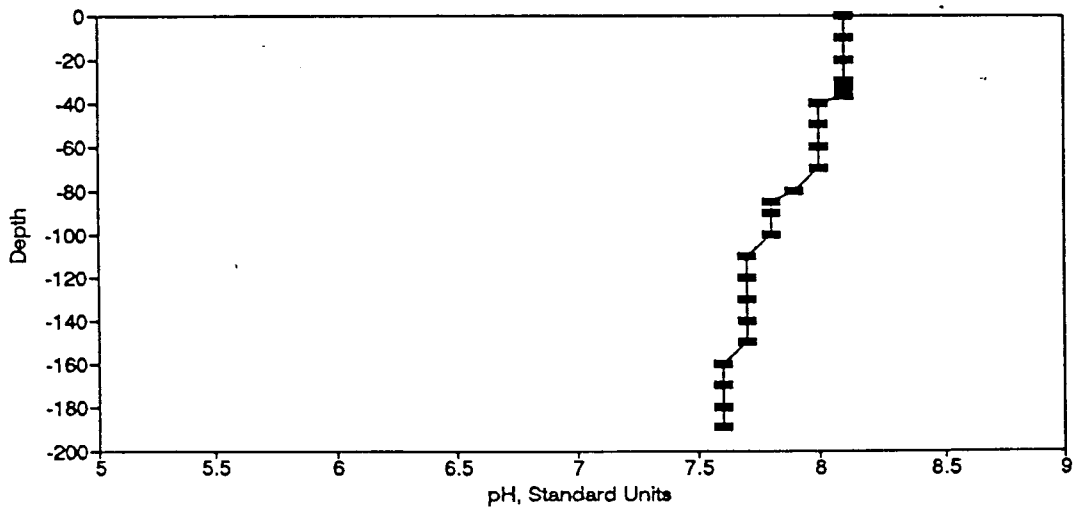
Figure BP99. pH Profile for the Eureka Springs Site-April 20, 1982.
