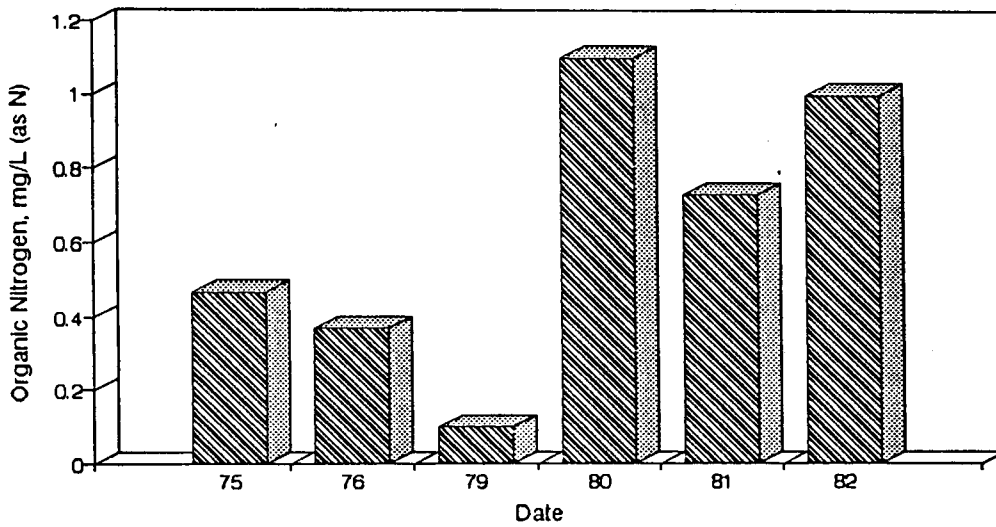
Figure A80. Graph of Organic Nitrogen vs. Time for the White River Site-Aug.
