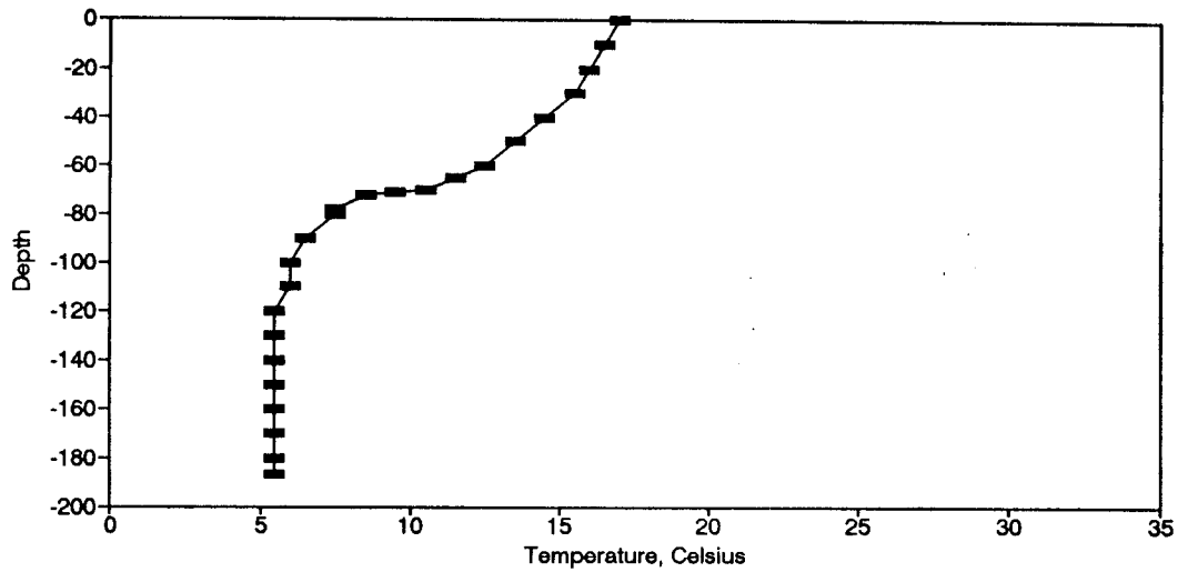
Figure BT87. Temperature Profile for the Eureka Springs Site-April 13, 1981.
