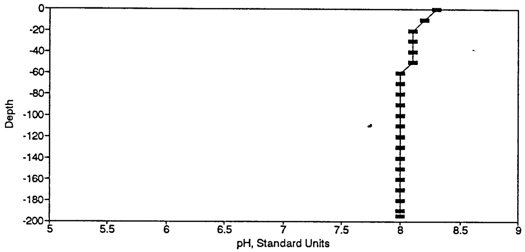
Figure BP14. pH Profile for the Eureka Springs Site-February 18, 1975.
