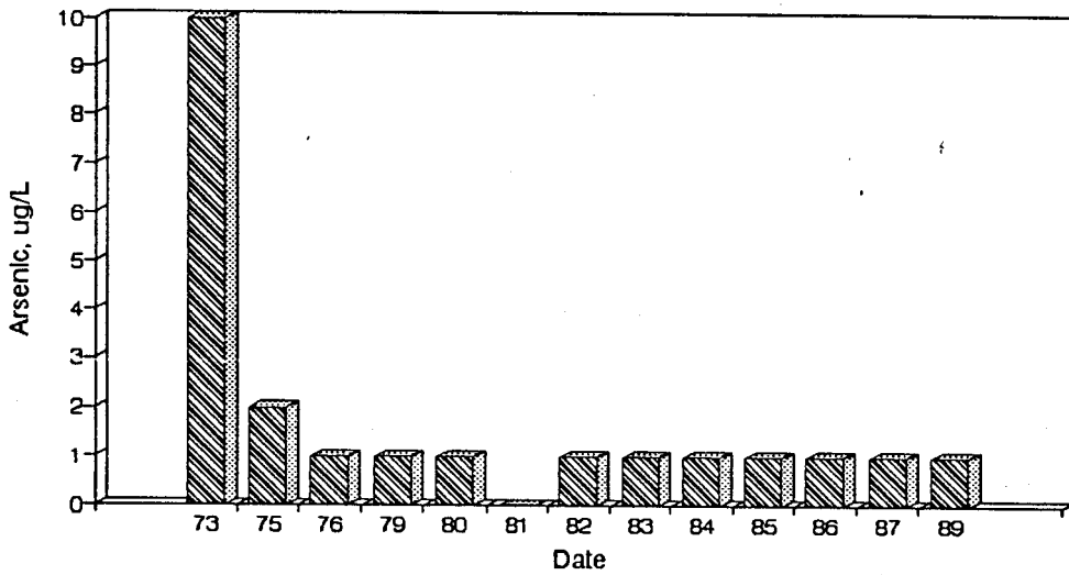
Figure A44. Graph of Arsenic vs. Time for the White River Site-Aug.
