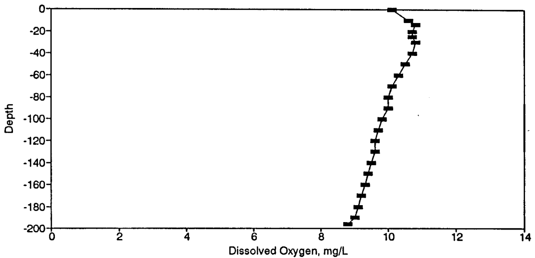
Figure BD147. Dissolved Oxygen Profile for the Eureka Springs Site-April 9, 1986.
