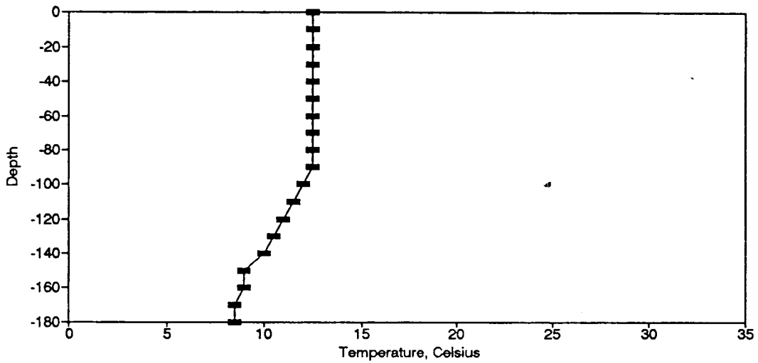
Figure BT35. Temperature Profile for the Eureka Springs Site-November 16, 1976.
