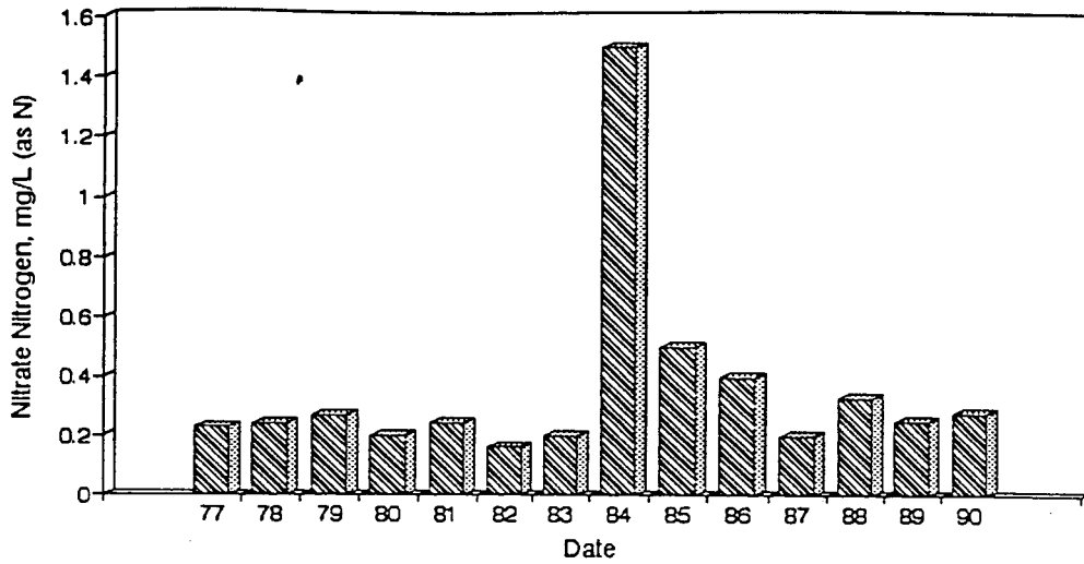
Figure A82. Graph of Nitrate Nitrogen vs. Time for the White River Site-May.
