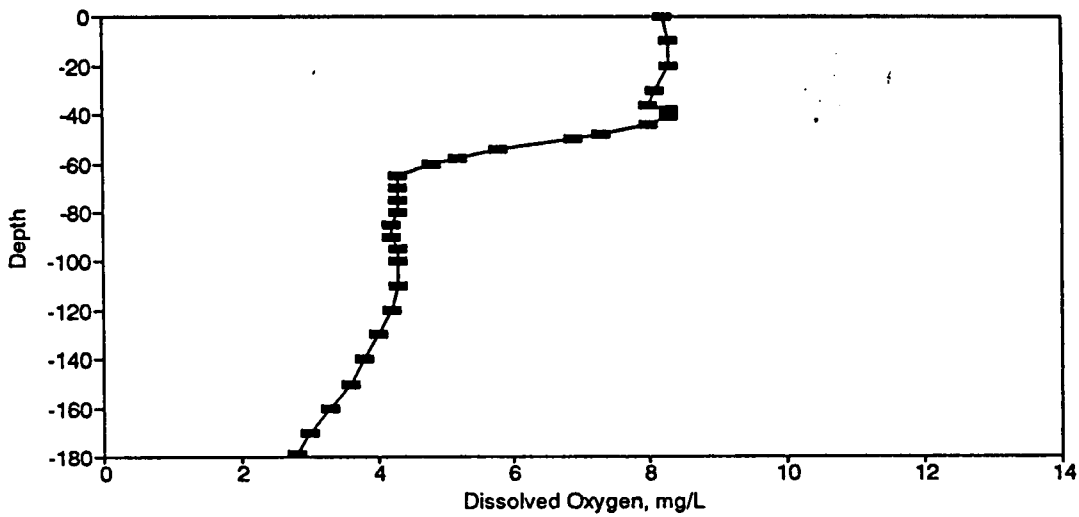
Figure BD92. Dissolved Oxygen Profile for the Eureka Springs Site-September 14, 1981.
