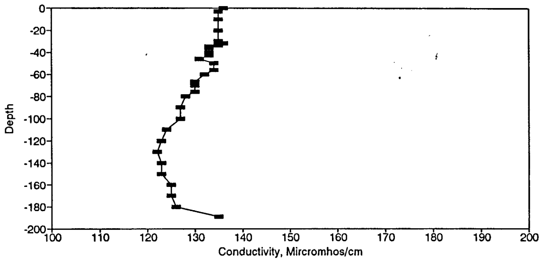
Figure BC152. Conductivity Profile for the Eureka Springs Site-September 4, 1986.
