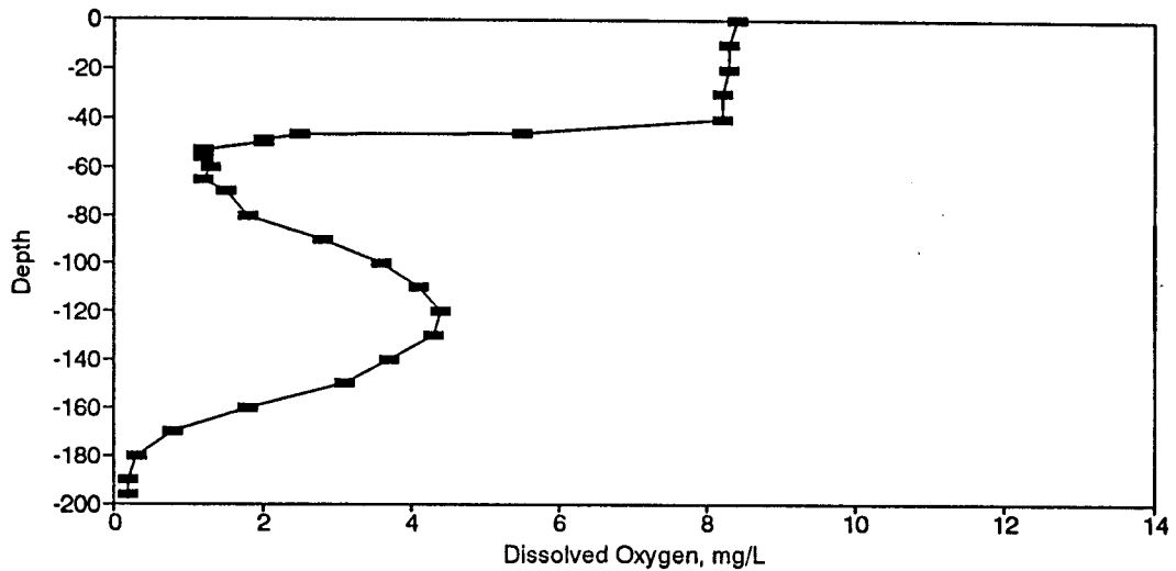
Figure BD153. Dissolved Oxygen Profile for the Eureka Springs Site-October 9, 1986.
