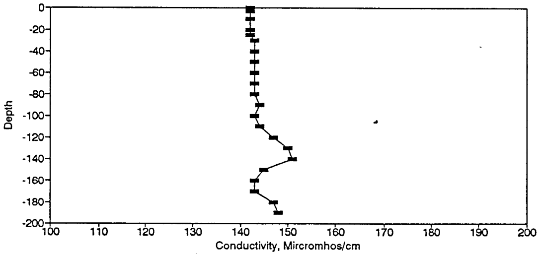
Figure BC179. Conductivity Profile for the Eureka Springs Site-January 4, 1989.
