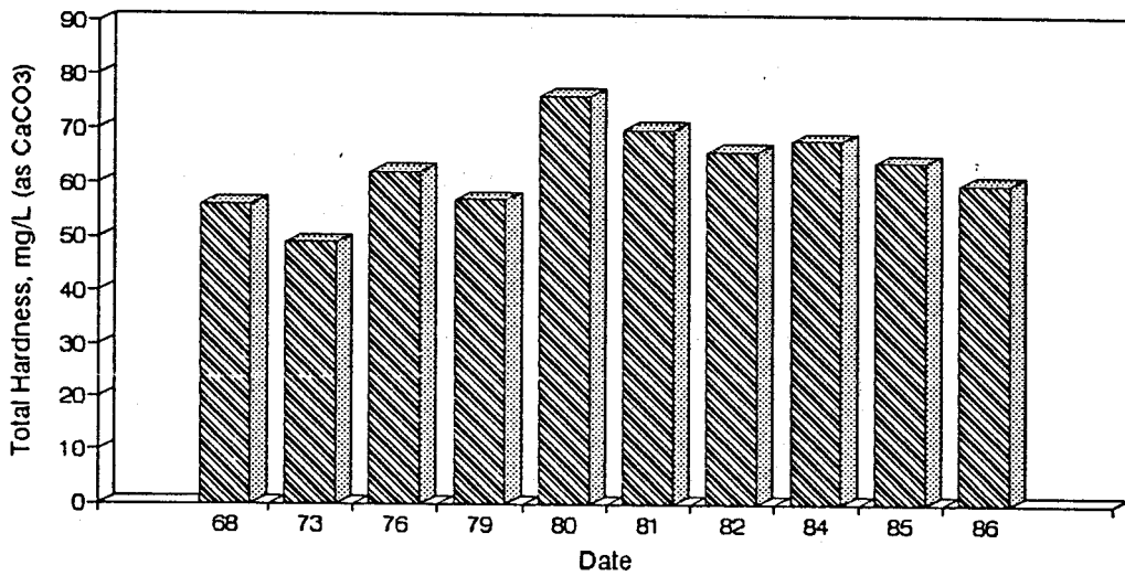
Figure A26. Graph of Total Hardness vs. Time for the White River Site-Aug.
