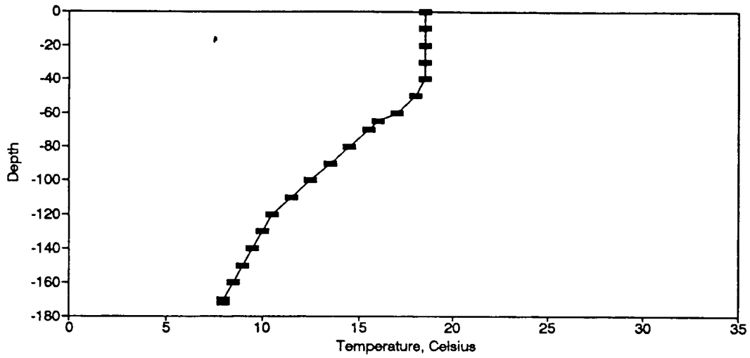
Figure BT34. Temperature Profile for the Eureka Springs Site-October 18, 1976.
