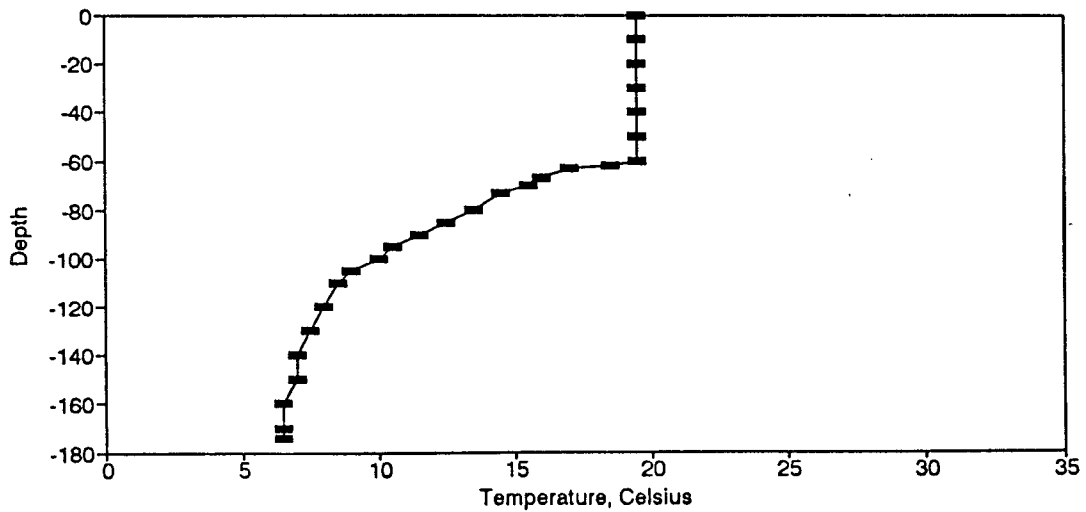
Figure BT93. Temperature Profile for the Eureka Springs Site-October 20, 1981.
