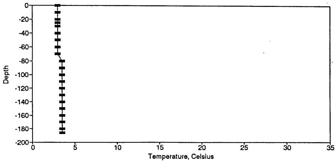
Figure BT51. Temperature Profile for the Eureka Springs Site-March 2, 1978.
