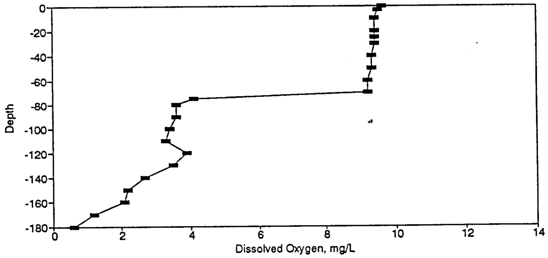
Figure BD167. Dissolved Oxygen Profile for the Eureka Springs Site-December 2, 1987.
