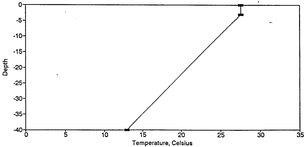
Figure BT162. Temperature Profile for the Eureka Springs Site-July 15, 1987.
