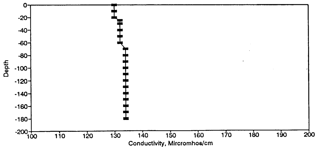
Figure BC63. Conductivity Profile for the Eureka Springs Site-March 8, 1979.
