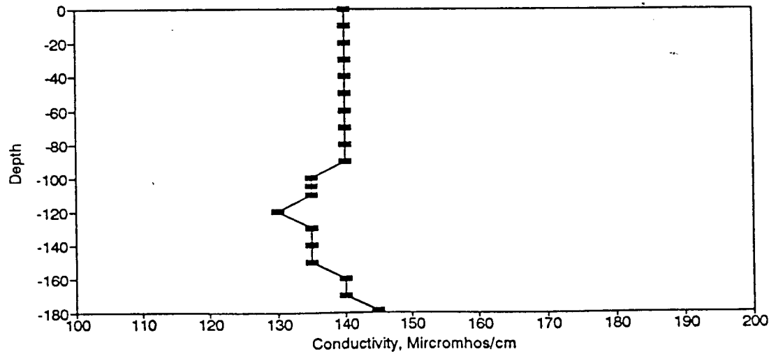
Figure BC60. Conductivity Profile for the Eureka Springs Site-December 5, 1978.
