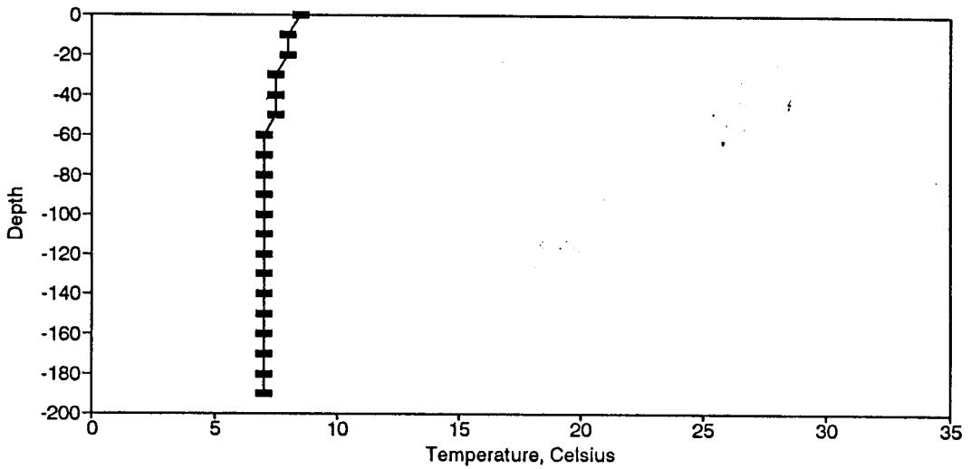
Figure BT158. Temperature Profile for the Eureka Springs Site-March 11, 1987.
