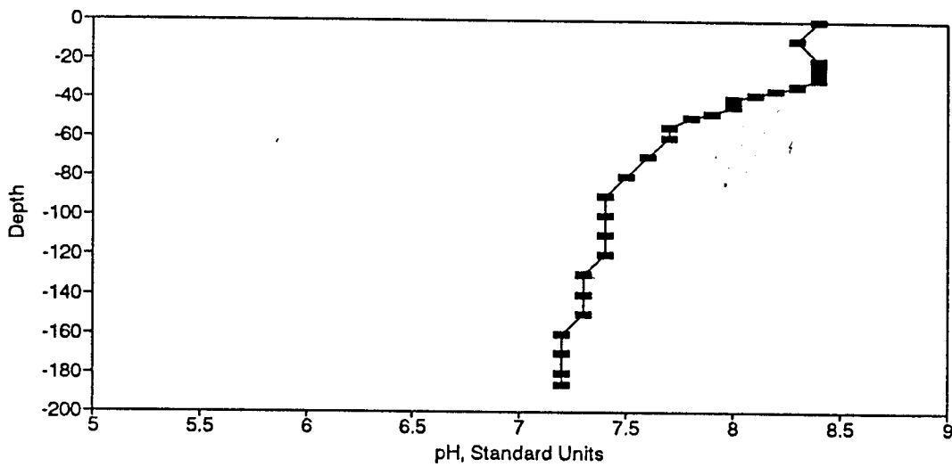
Figure BP101. pH Profile for the Eureka Springs Site-June 22, 1982.
