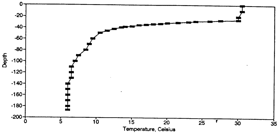
Figure BT79. Temperature Profile for the Eureka Springs Site-July 16, 1980.
