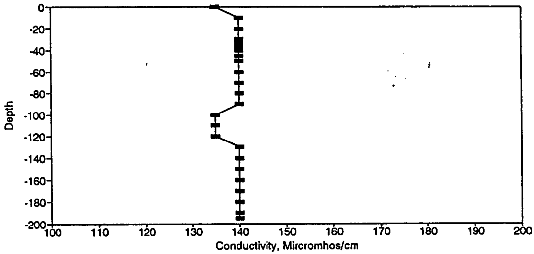
Figure BC56. Conductivity Profile for the Eureka Springs Site-August 15, 1978.
