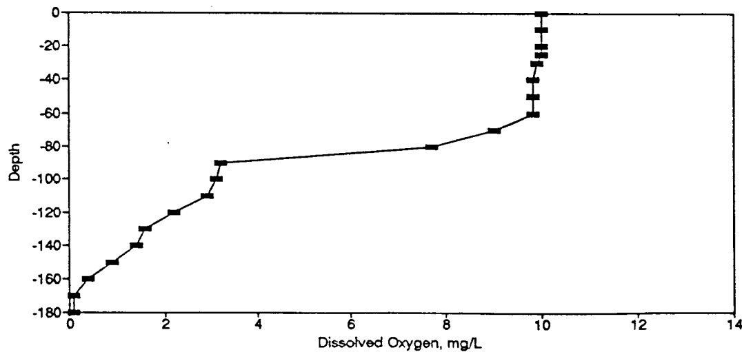
Figure BD84. Dissolved Oxygen Profile for the Eureka Springs Site-December 10, 1980.
