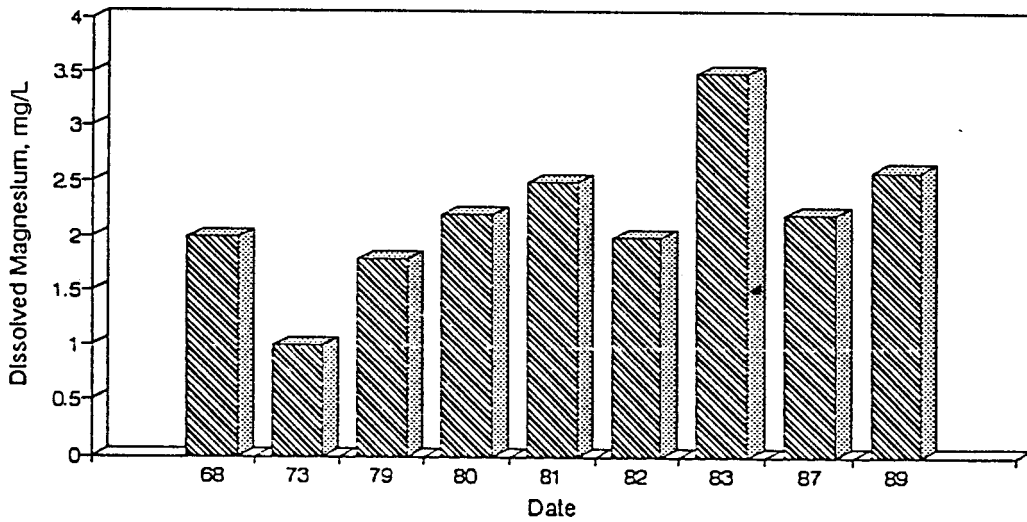
Figure A35. Graph of Dissolved Magnesium vs. Time for the White River Site-Aug.
