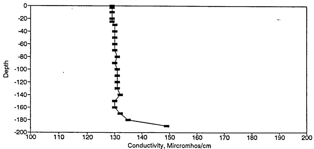
Figure BC156. Conductivity Profile for the Eureka Springs Site-January 13, 1987.
