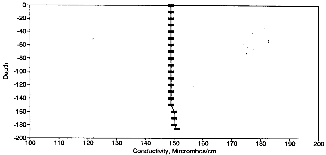
Figure BC86. Conductivity Profile for the Eureka Springs Site-March 3, 1981.
