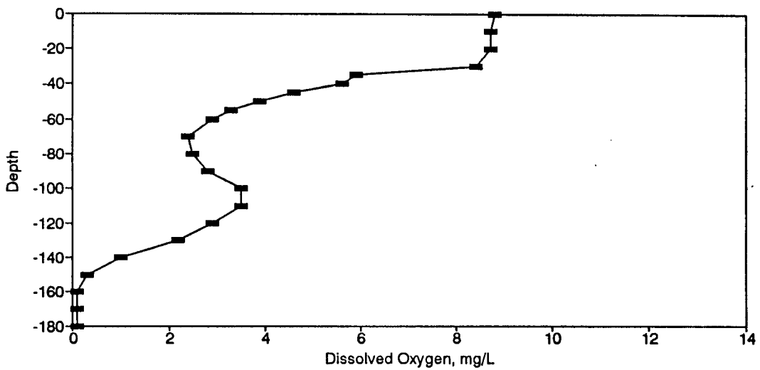
Figure BD33. Dissolved Oxygen Profile for the Eureka Springs Site-September 22, 1976.
