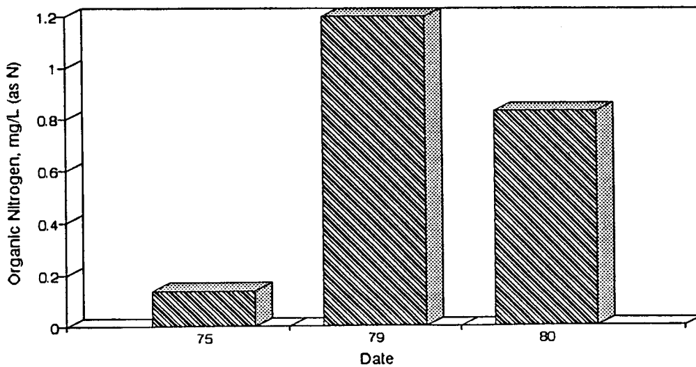
Figure A81. Graph of Organic Nitrogen vs. Time for the White River Site-Dec.
