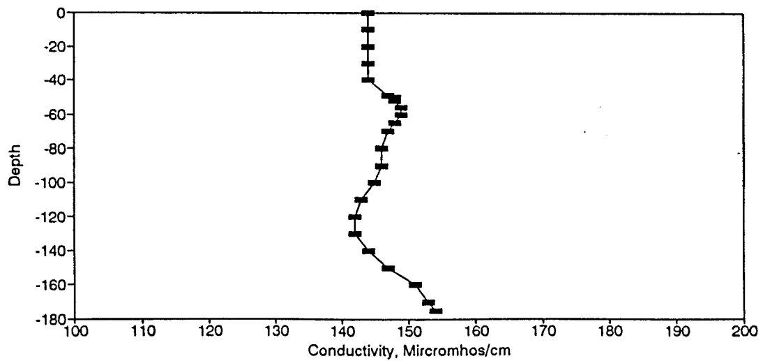
Figure BC105. Conductivity Profile for the Eureka Springs Site-October 22, 1982.
