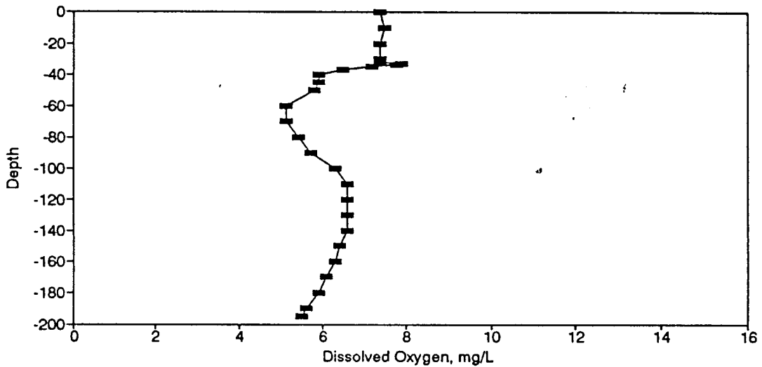
Figure BD56. Dissolved Oxygen Profile for the Eureka Springs Site-August 15, 1978.
