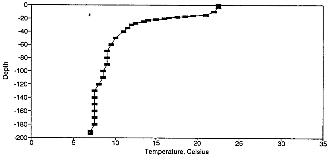
Figure BT160. Temperature Profile for the Eureka Springs Site-May 13, 1987.
