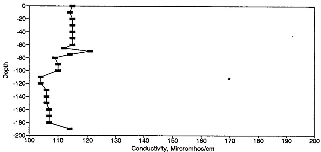
Figure BC23. Conductivity Profile for the Eureka Springs Site-November 18, 1975.
