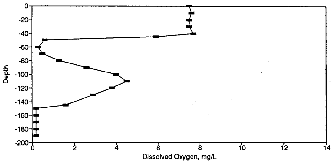
Figure BD9. Dissolved Oxygen Profile for the Eureka Springs Site-September 24, 1974.
