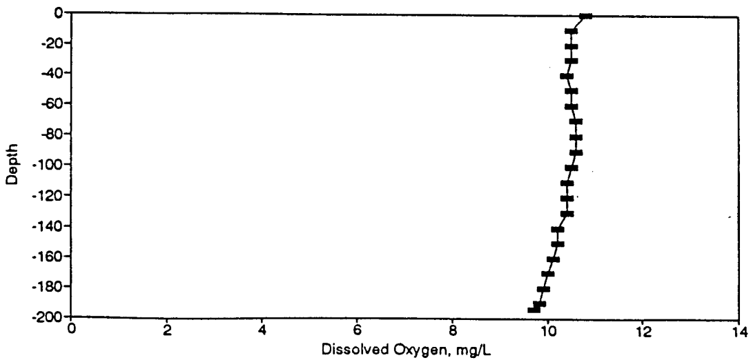
Figure BD171. Dissolved Oxygen Profile for the Eureka Springs Site-April 13, 1988.
