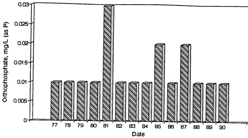
Figure A97. Graph of Orthophosphate vs. Time for the White River Site-May.
