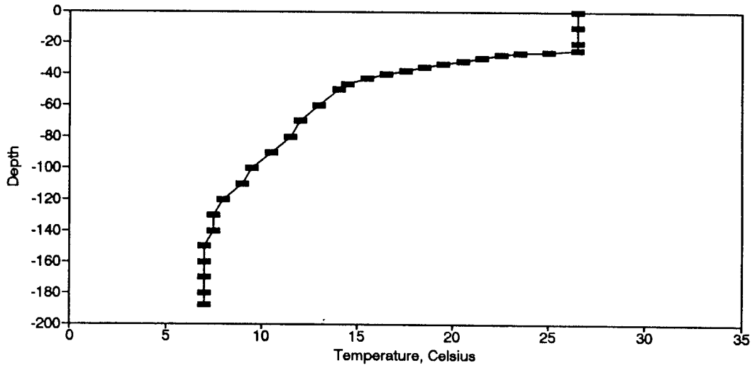
Figure BT127. Temperature Profile for the Eureka Springs Site-August 14, 1984.
