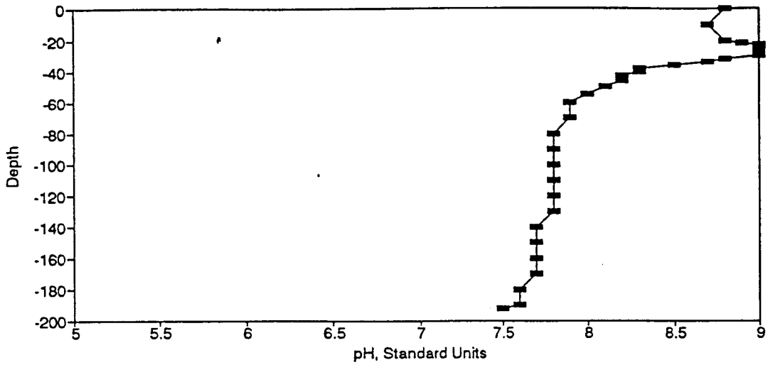
Figure BP115. pH Profile for the Eureka Springs Site-August 17, 1983.
