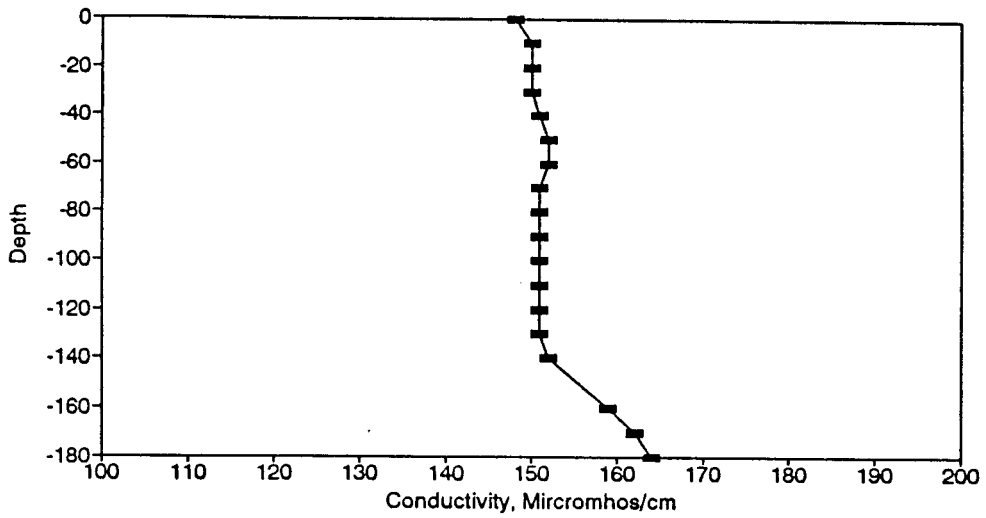
Figure BC73. Conductivity Profile for the Eureka Springs Site-January 8, 1980,
