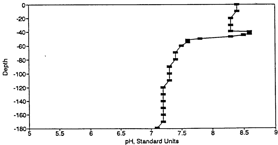
Figure BP81. pH Profile for the Eureka Springs Site-September 16, 1980.
