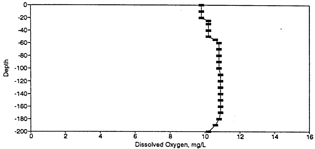
Figure BD53. Dissolved Oxygen Profile for the Eureka Springs Site-May 9, 1978.
