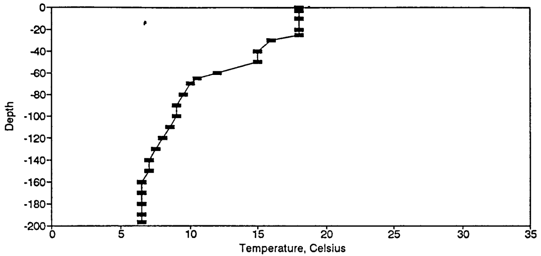
Figure BT148. Temperature Profile for the Eureka Springs Site-May 6, 1986.
