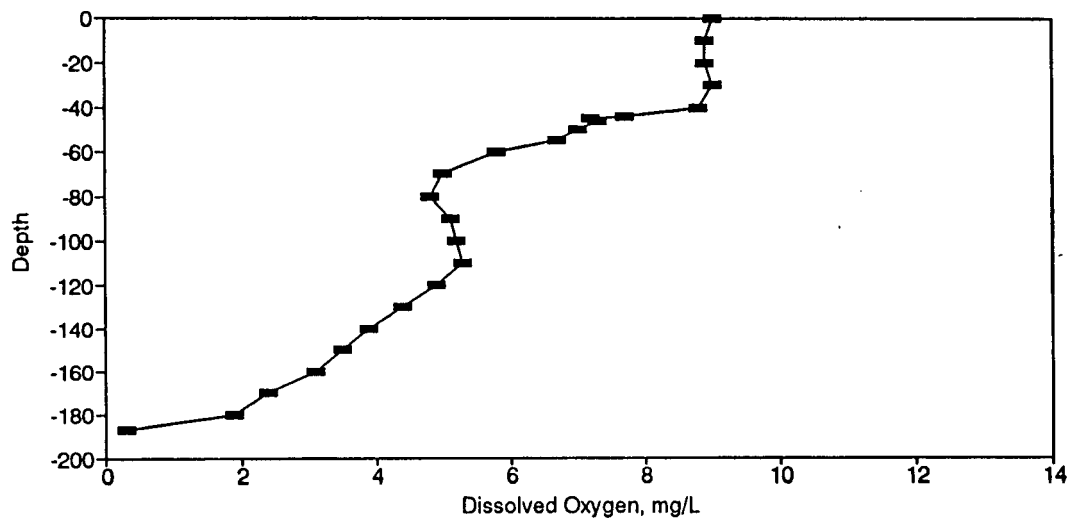
Figure BD165. Dissolved Oxygen Profile for the Eureka Springs Site-October 15, 1987.
