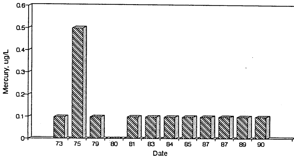
Figure A63. Graph of Mercury vs. Time for the White River Site-Dec.
