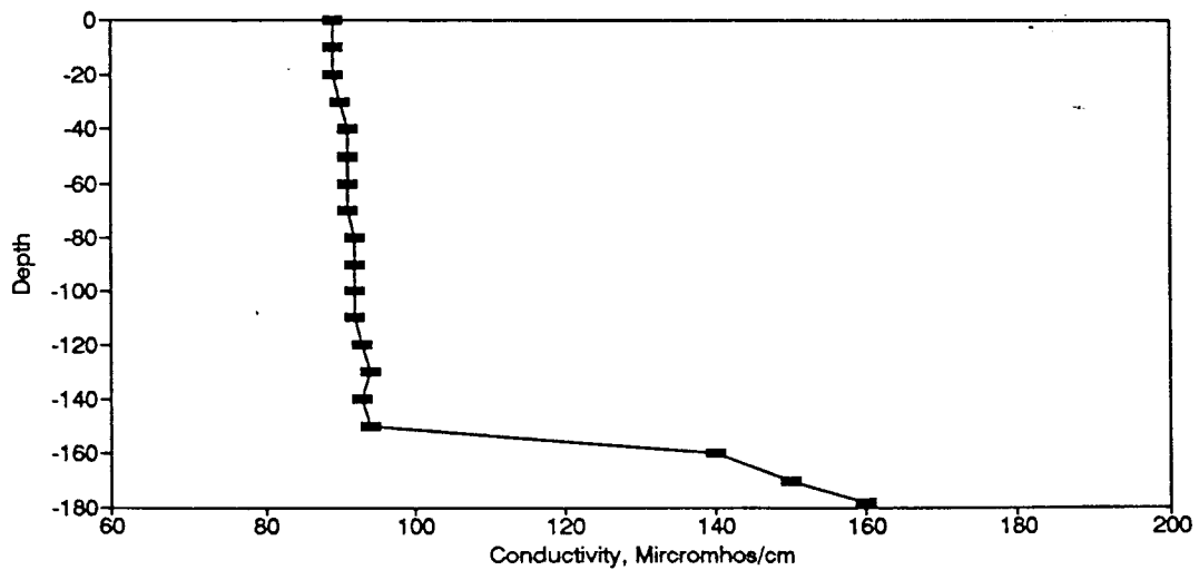
Figure BC36. Conductivity Profile for the Eureka Springs Site-December 14, 1976.
