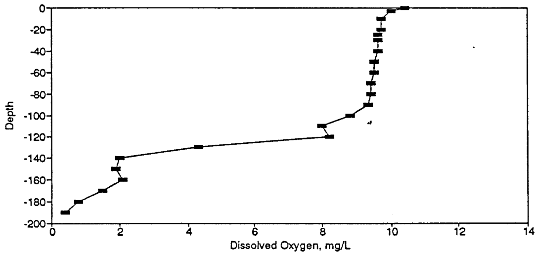
Figure BD179. Dissolved Oxygen Profile for the Eureka Springs Site-January 4, 1989.
