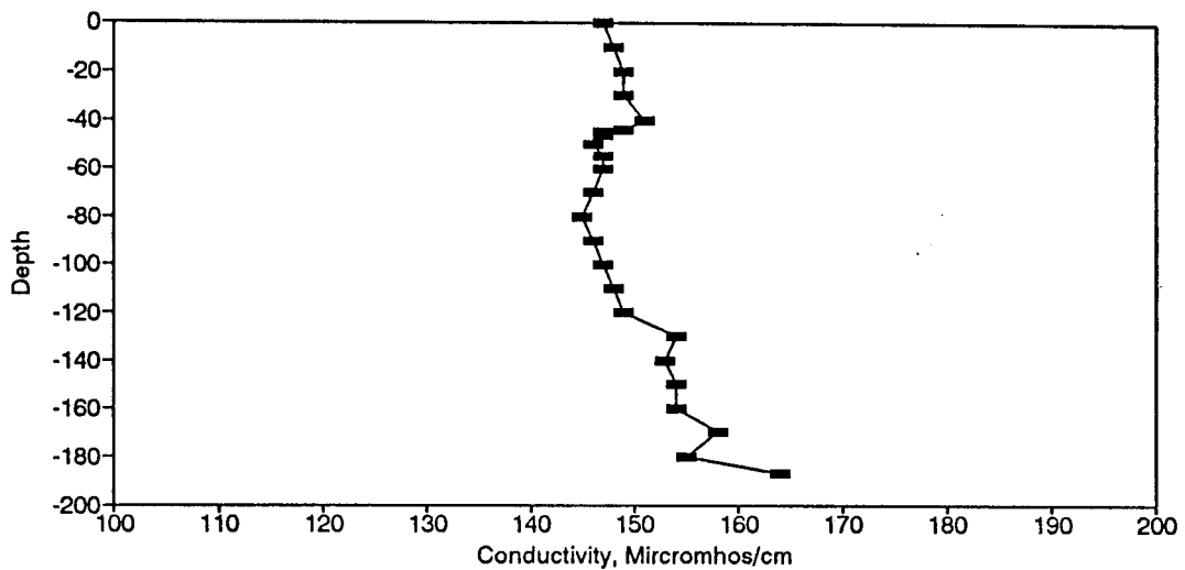
Figure BC165. Conductivity Profile for the Eureka Springs Site-October 15, 1987.
