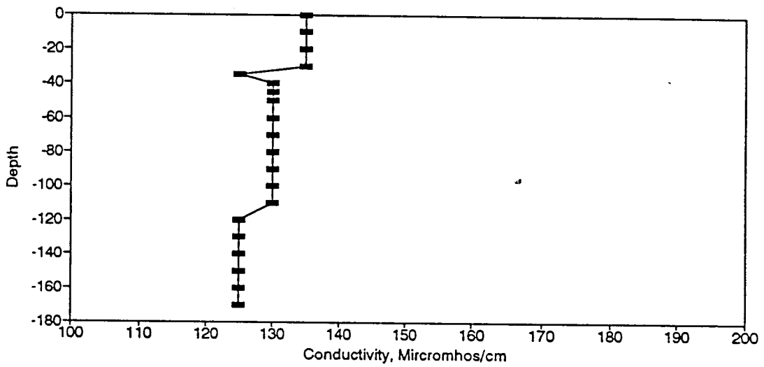
Figure BC41. Conductivity Profile for the Eureka Springs Site-May 1, 1977.
