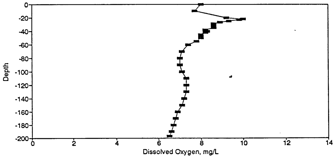
Figure BD185. Dissolved Oxygen Profile for the Eureka Springs Site-July 13, 1989.
