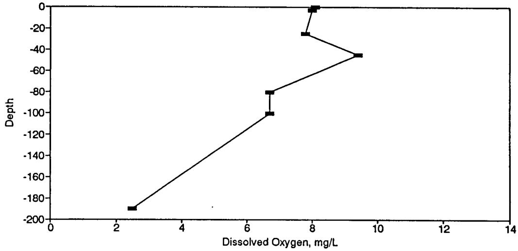
Figure BD163. Dissolved Oxygen Profile for the Eureka Springs Site-August 19, 1987.
