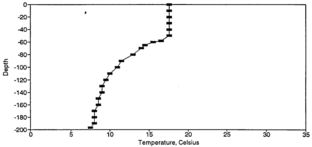
Figure BT154. Temperature Profile for the Eureka Springs Site-November 5, 1986.
