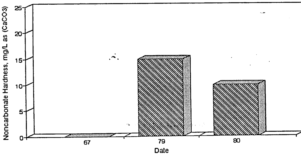
Figure A39. Graph of Noncarbonate Hardness vs. Time for the White River Site-Dec.
