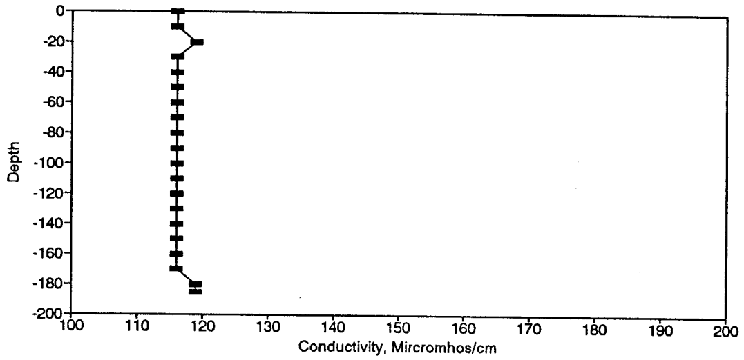
Figure BC25. Conductivity Profile for the Eureka Springs Site-January 20, 1976.
