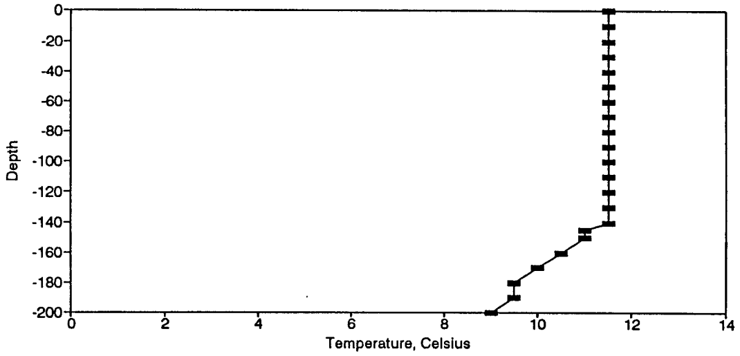
Figure BT1. Temperature Profile for the Eureka Springs Site-December 18, 1973.
