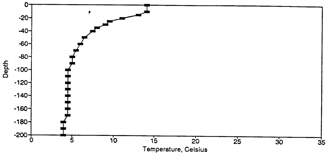
Figure BT52. Temperature Profile for the Eureka Springs Site-April 11, 1978.
