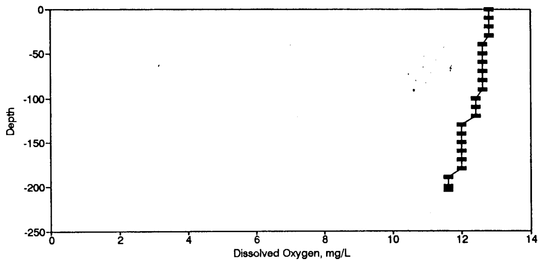
Figure BD134. Dissolved Oxygen Profile for the Eureka Springs Site-March 7, 1985.
