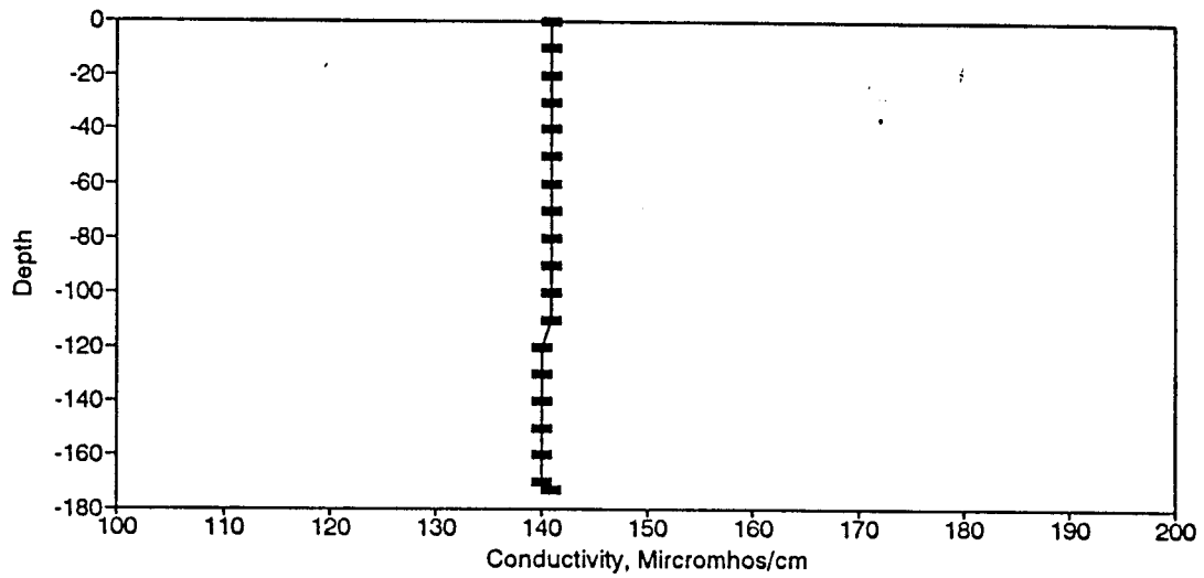
Figure BC122. Conductivity Profile for the Eureka Springs Site-March 28, 1984.
