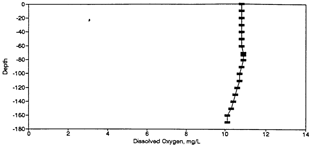
Figure BD76. Dissolved Oxygen Profile for the Eureka Springs Site-April 8, 1980.
