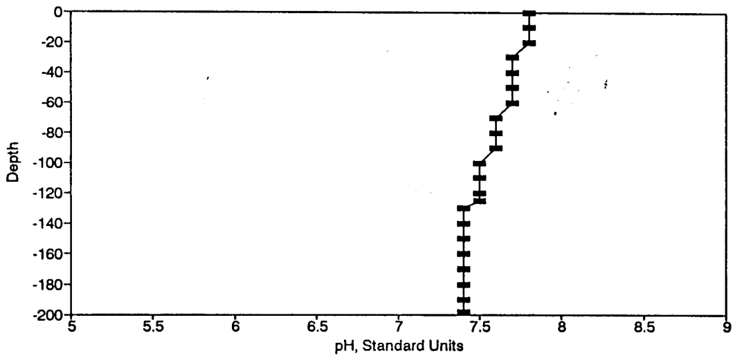
Figure BP11. pH Profile for the Eureka Springs Site-November 20, 1974.
