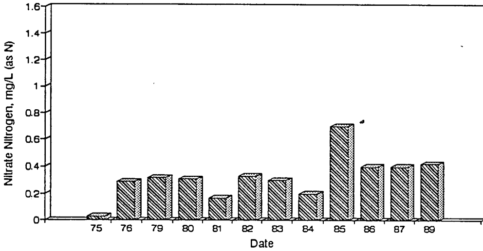
Figure A83. Graph of Nitrate Nitrogen vs. Time for the White River Site-Aug.
