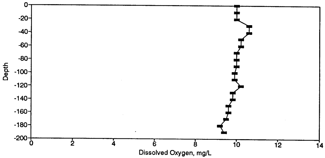
Figure BD13. Dissolved Oxygen Profile for the Eureka Springs Site-January 21, 1975.
