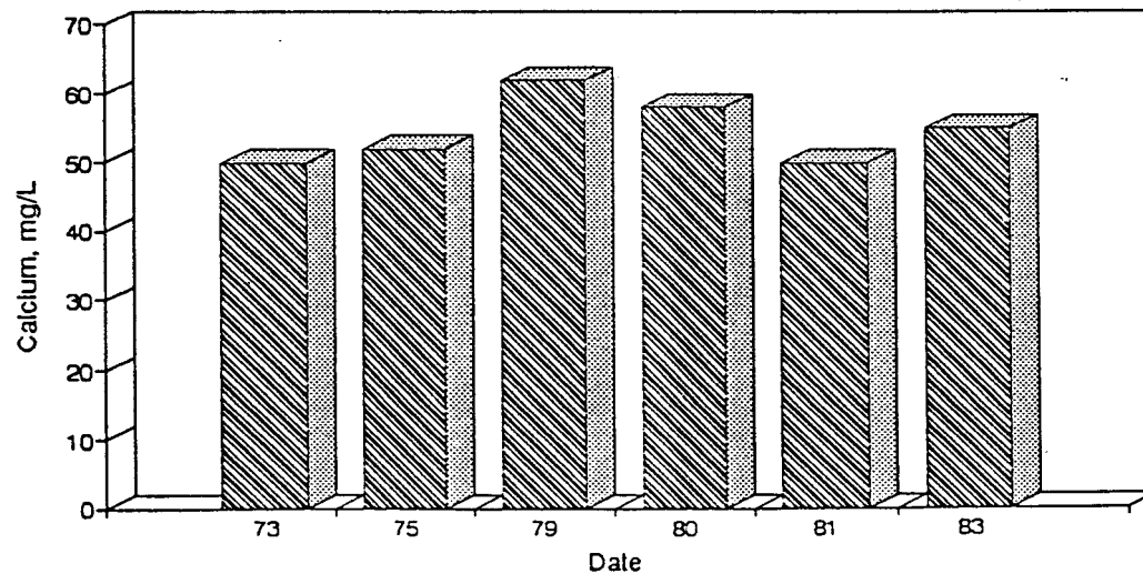
Figure A30. Graph of Calcium vs. Time for the White River Site-Dec.
