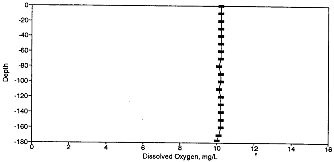
Figure BD61. Dissolved Oxygen Profile for the Eureka Springs Site-January 9, 1979.
