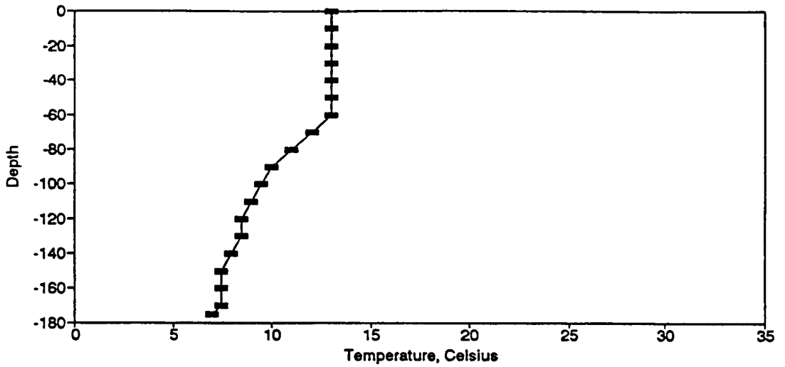
Figure BT106. Temperature Profile for the Eureka Springs Site-November 24, 1982.
