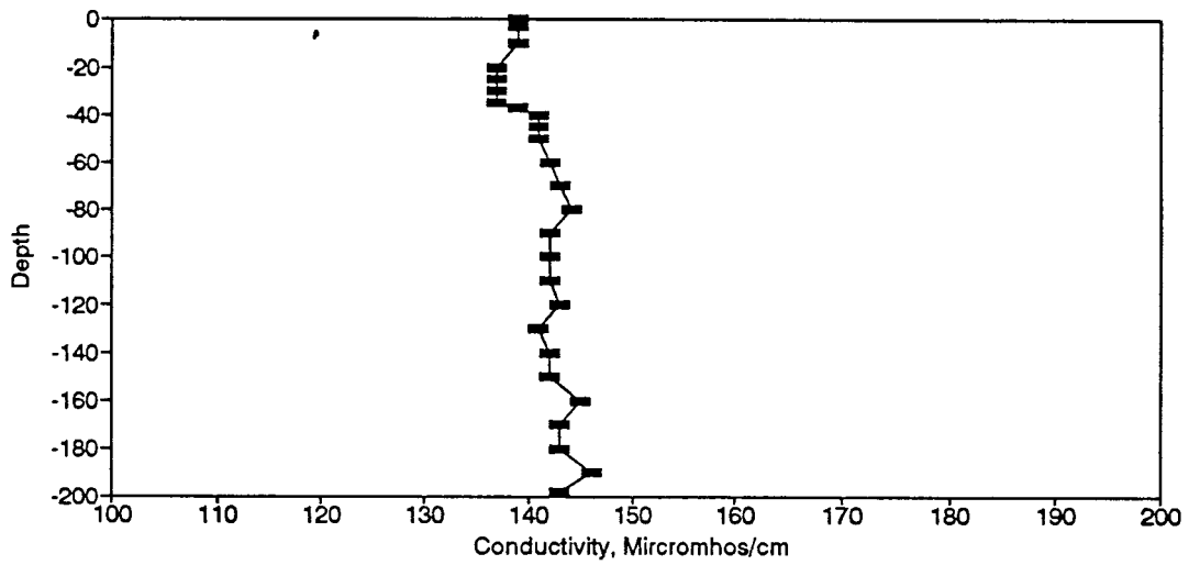
Figure BC172. Conductivity Profile for the Eureka Springs Site-May 10, 1988.
