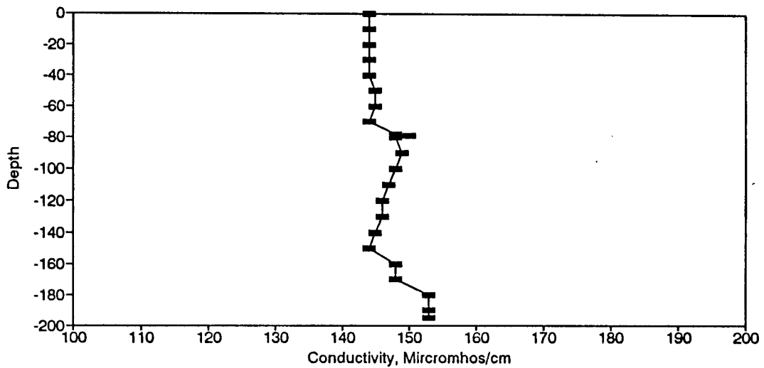
Figure BC177. Conductivity Profile for the Eureka Springs Site-November 16, 1988.
