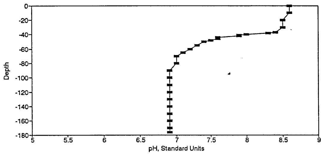
Figure BP116. pH Profile for the Eureka Springs Site-September 19, 1983.
