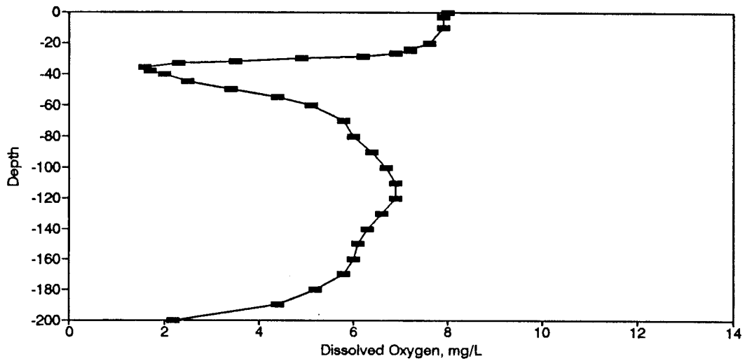
Figure BD139. Dissolved Oxygen Profile for the Eureka Springs Site-August 7, 1985.
