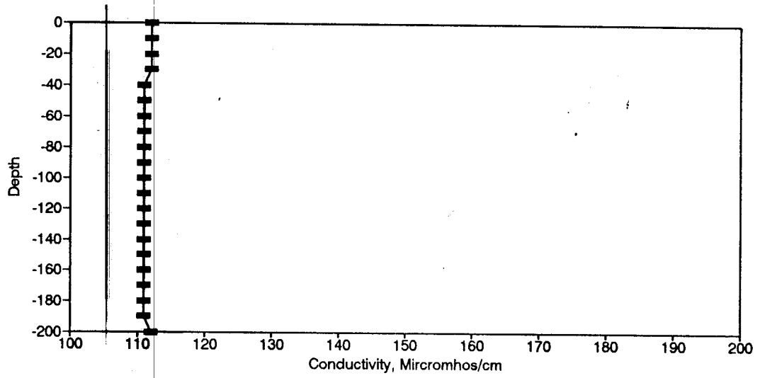
Figure BC2. Conductivity Profile for the Eureka Springs Site-January 15, 1974.
