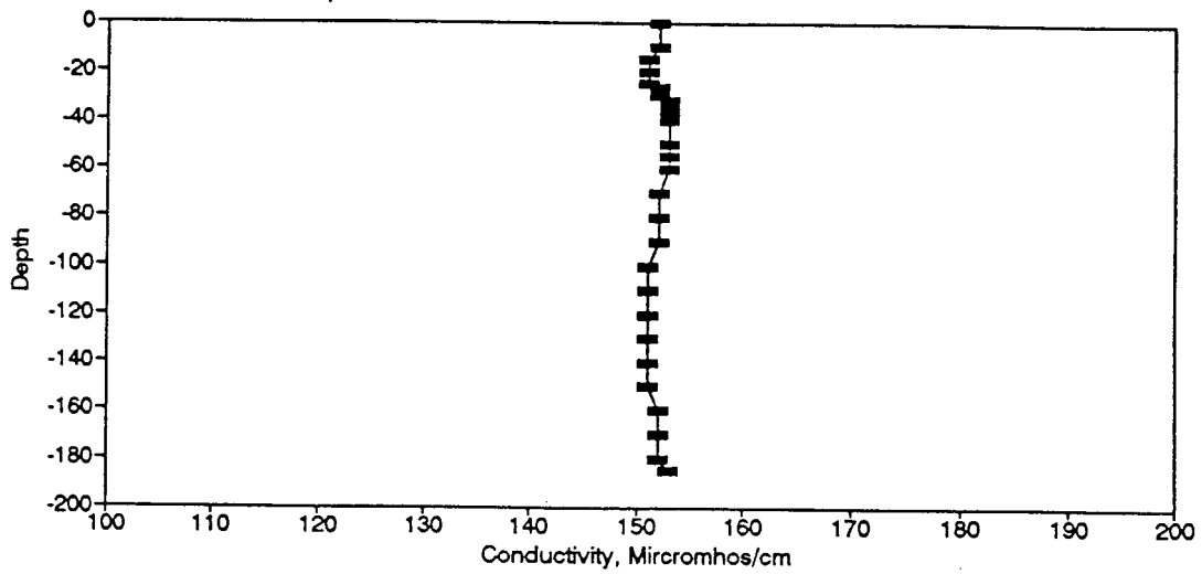
Figure BC100. Conductivity Profile for the Eureka Springs Site-May 19, 1982.
