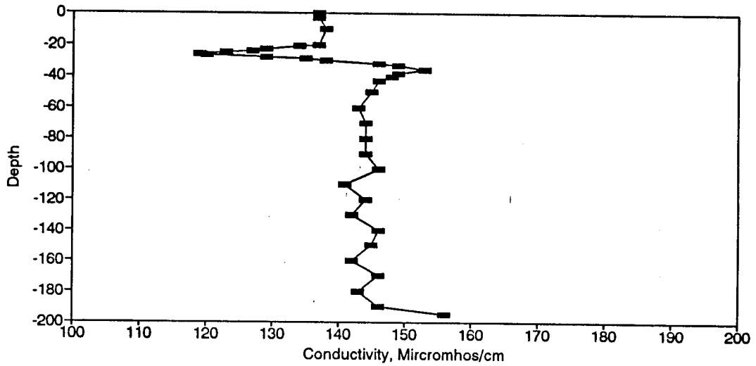
Figure BC175. Conductivity Profile for the Eureka Springs Site-August 9, 1988.
