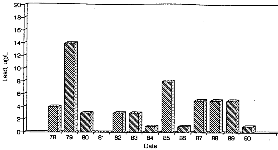
Figure A55. Graph of Lead vs. Time for the White River Site-May.
