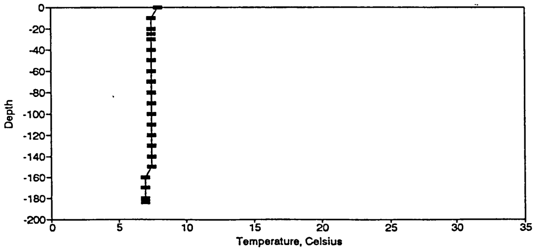
Figure BT108. Temperature Profile for the Eureka Springs Site-January 25, 1983.
