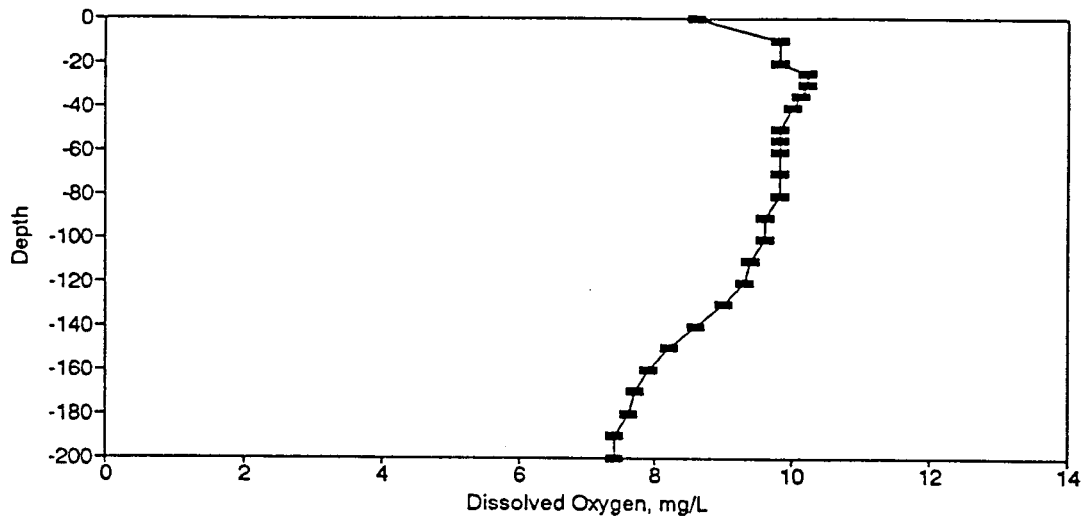
Figure BD112. Dissolved Oxygen Profile for the Eureka Springs Site-May 18 1983.
