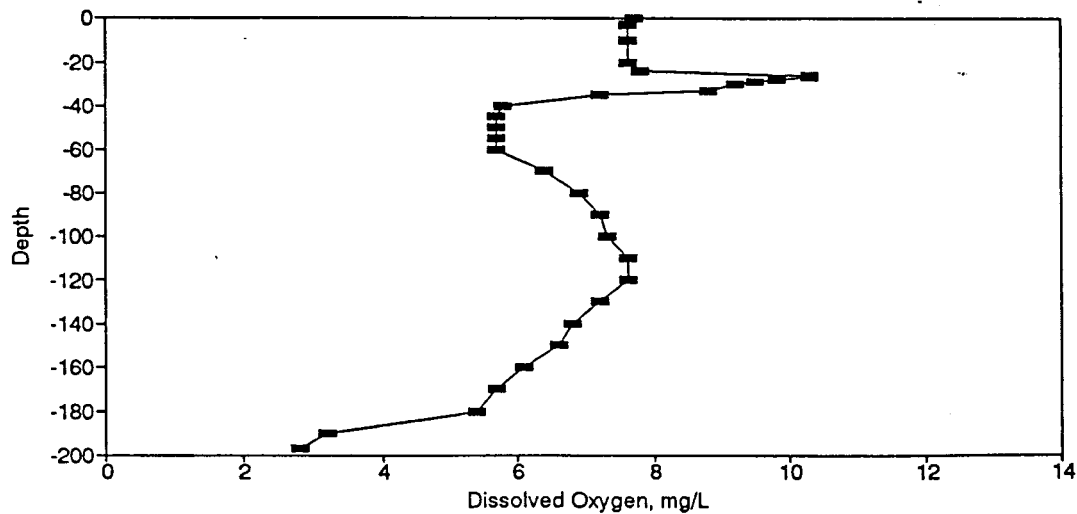
Figure BD150. Dissolved Oxygen Profile for the Eureka Springs Site-July 9, 1986.
