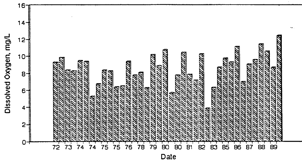
Figure A18. Graph of Dissolved Oxygen vs. Time for the White River Site-Dec.
