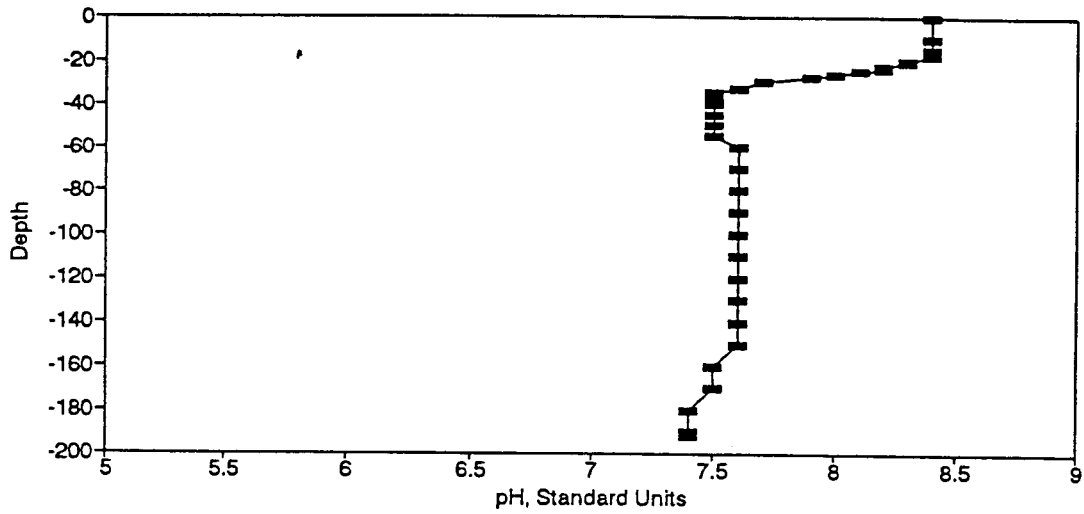
Figure BP67. pH Profile for the Eureka Springs Site - July 17, 1979.
