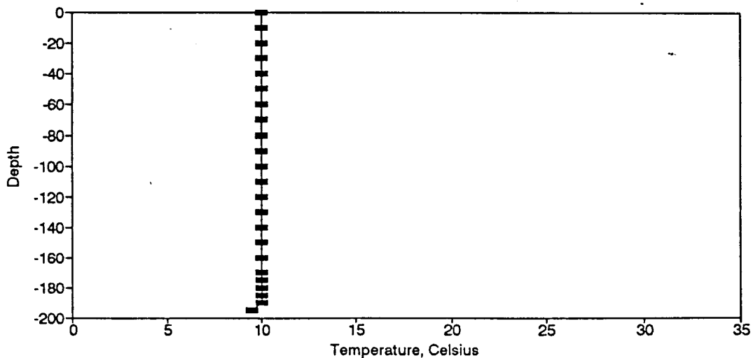
Figure BT12. Temperature Profile for the Eureka Springs Site-December 16, 1974.
