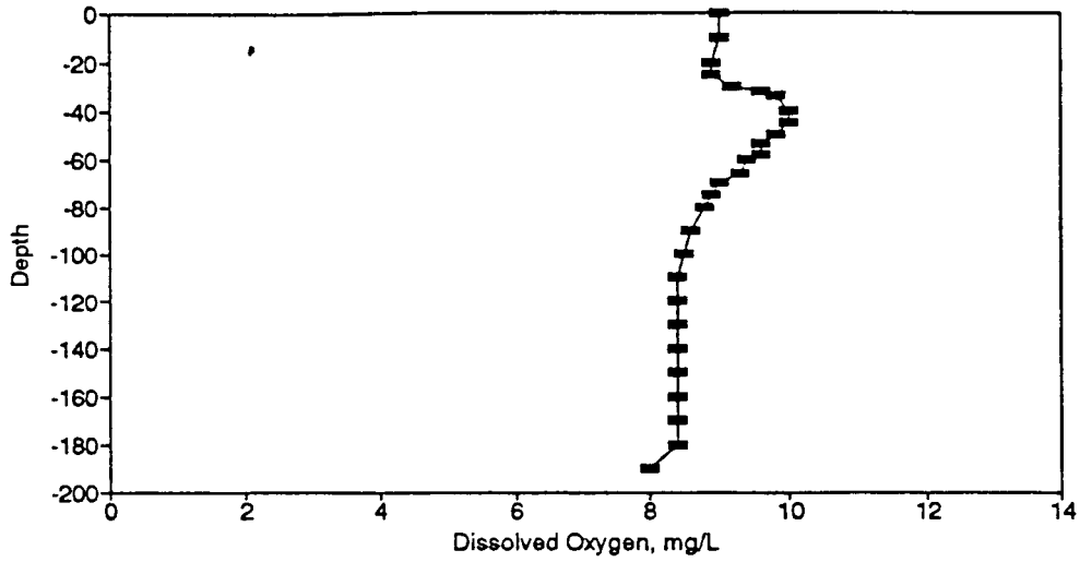
Figure BD88. Dissolved Oxygen Profile for the Eureka Springs Site-May 13, 1981.
