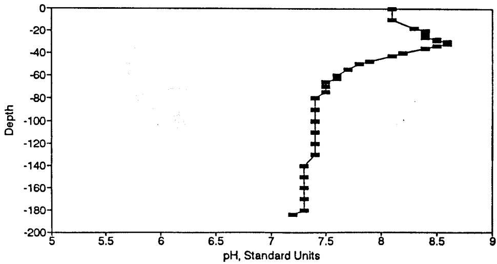
Figure BP90. pH Profile for the Eureka Springs Site-July 14, 1981.
