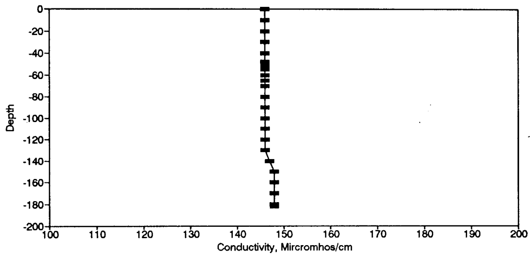
Figure BC129. Conductivity Profile for the Eureka Springs Site-October 18, 1984.
