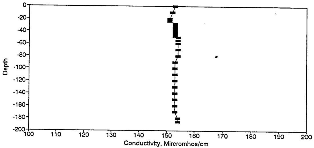
Figure BC101. Conductivity Profile for the Eureka Springs Site-June 22, 1982.
