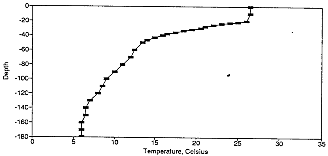
Figure BT125. Temperature Profile for the Eureka Springs Site-June 26, 1984.
