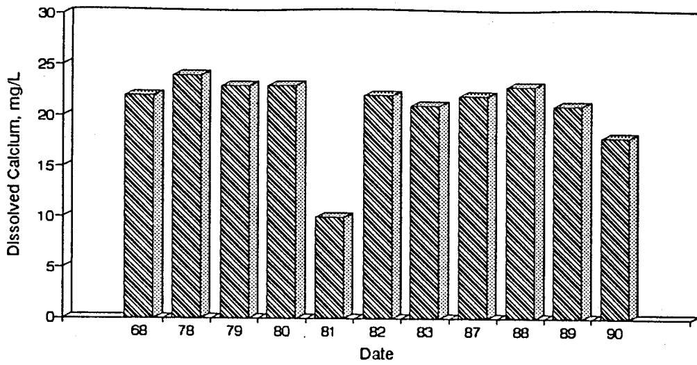
Figure A31. Graph of Dissolved Calcium vs. Time for the White River Site-May.
