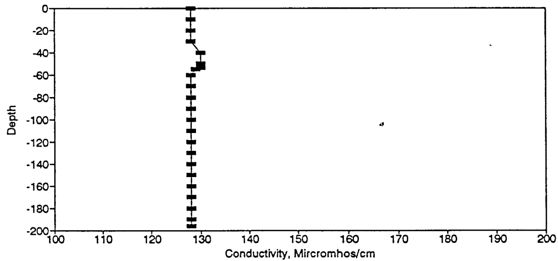
Figure BC65. Conductivity Profile for the Eureka Springs Site-May 7, 1979.
