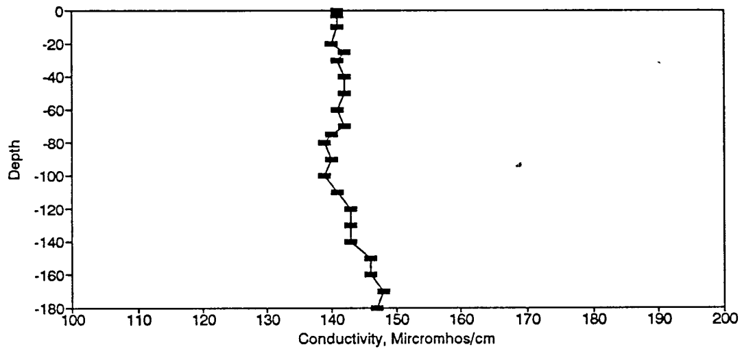
Figure BC167. Conductivity Profile for the Eureka Springs Site-December 2, 1987.
