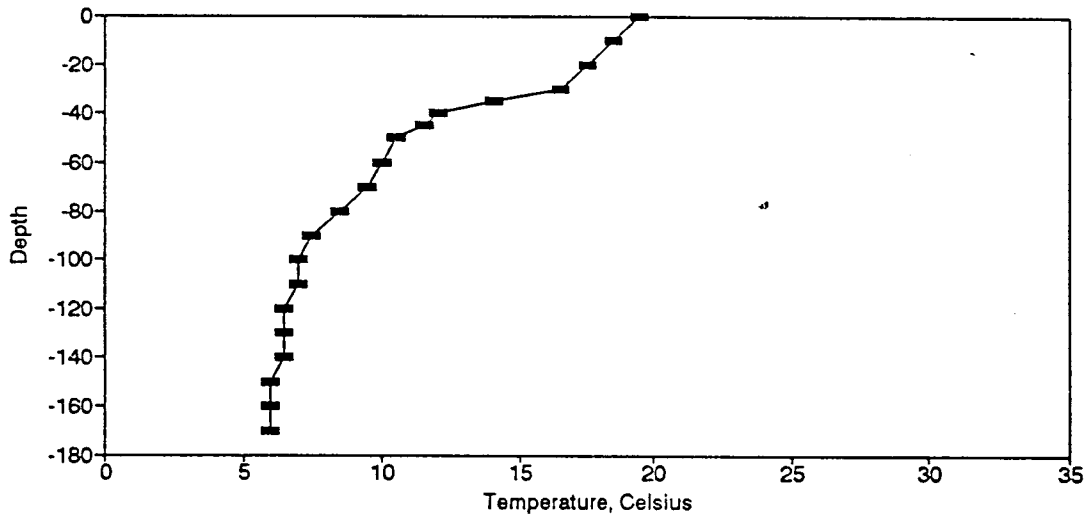
Figure BT41. Temperature Profile for the Eureka Springs Site-May 1, 1977.
