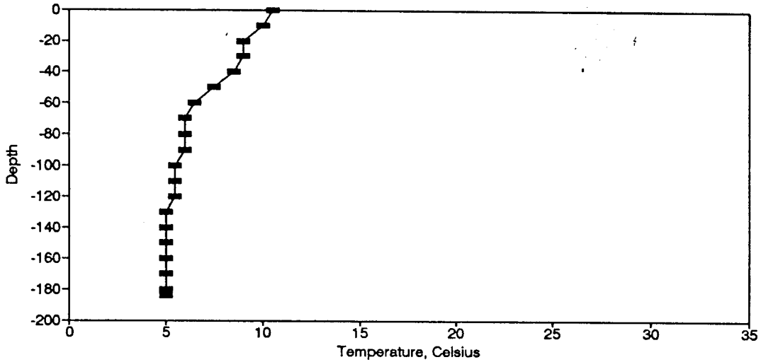
Figure BT98. Temperature Profile for the Eureka Springs Site-March 23, 1982.
