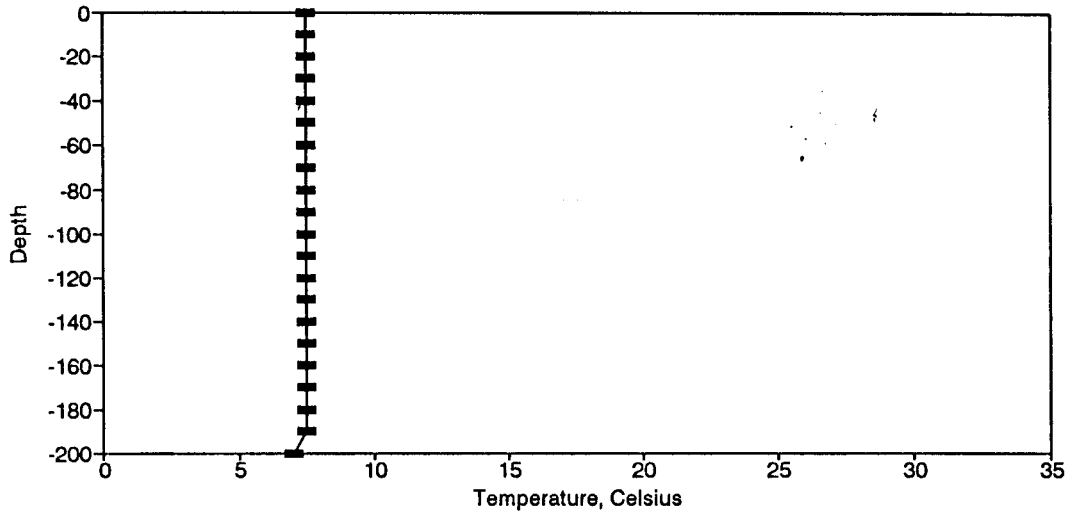
Figure BT2. Temperature Profile for the Eureka Springs Site-January 15, 1974.
