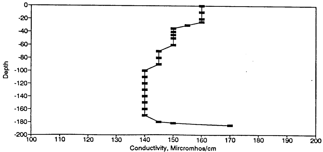
Figure BC45. Conductivity Profile for the Eureka Springs Site-August 22, 1977.
