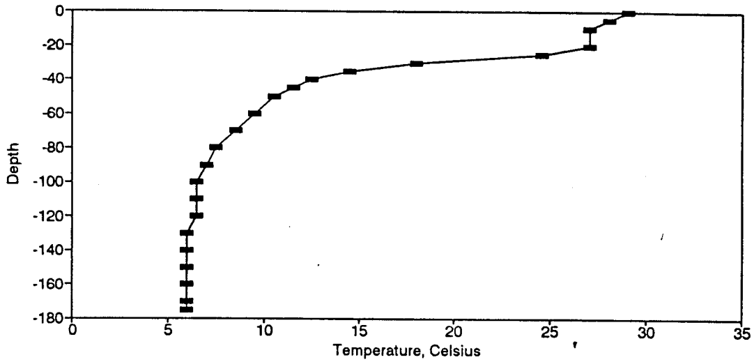
Figure BT43. Temperature Profile for the Eureka Springs Site-June 27, 1977.
