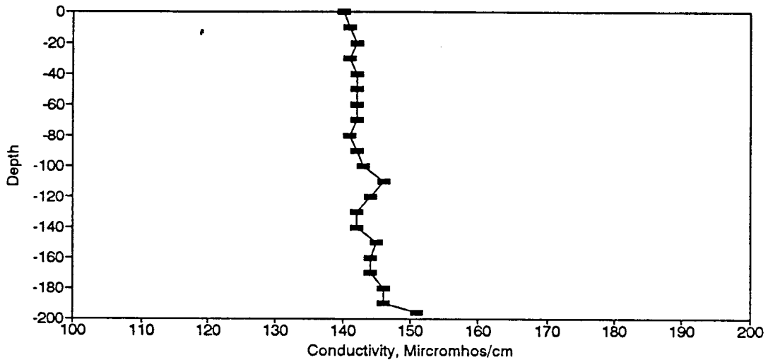
Figure BC178. Conductivity Profile for the Eureka Springs Site-December 14, 1988.
