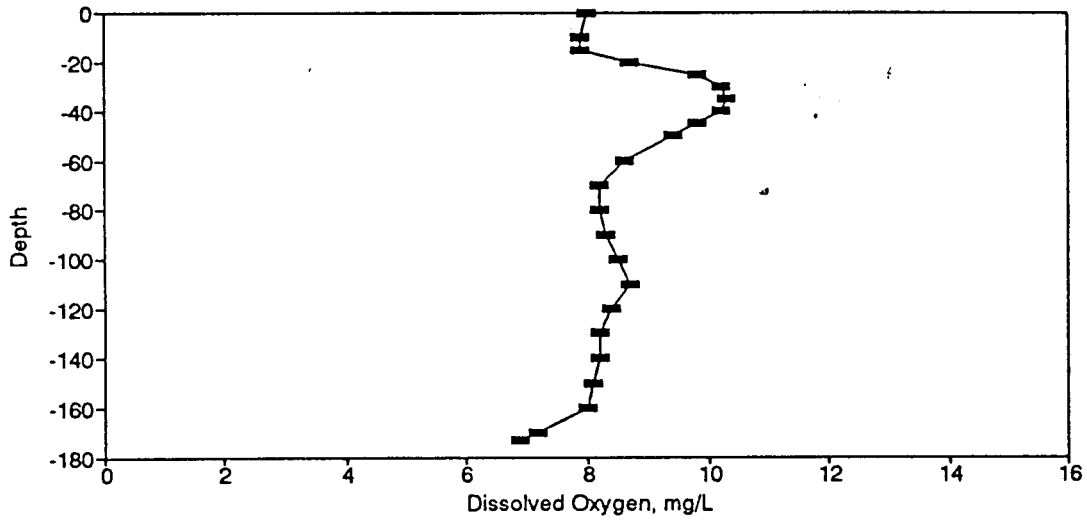
Figure BD44. Dissolved Oxygen Profile for the Eureka Springs Site-July 26, 1977.
