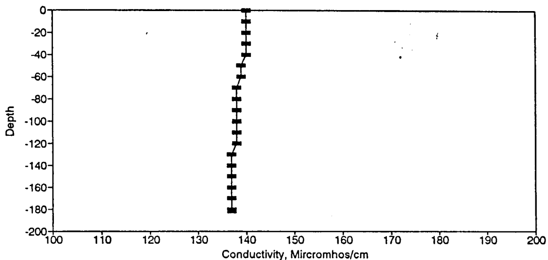
Figure BC110. Conductivity Profile for the Eureka Springs Site-March 23, 1983.
