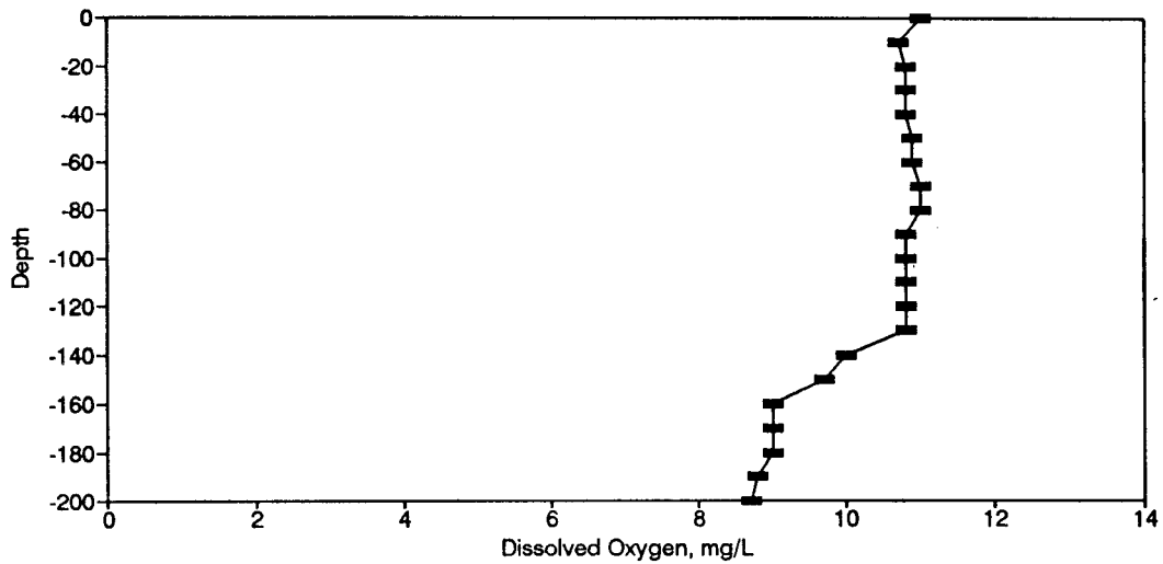
Figure BD3. Dissolved Oxygen Profile for the Eureka Springs Site-February 20, 1974.
