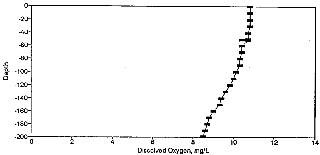
Figure BD159. Dissolved Oxygen Profile for the Eureka Springs Site-April 15, 1987.
