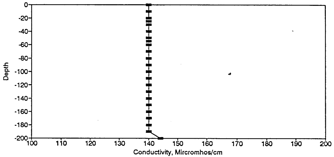
Figure BC53. Conductivity Profile for the Eureka Springs Site-May 9, 1978.
