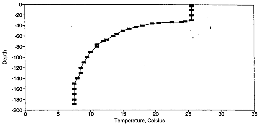
Figure BT152. Temperature Profile for the Eureka Springs Site-September 4, 1986.
