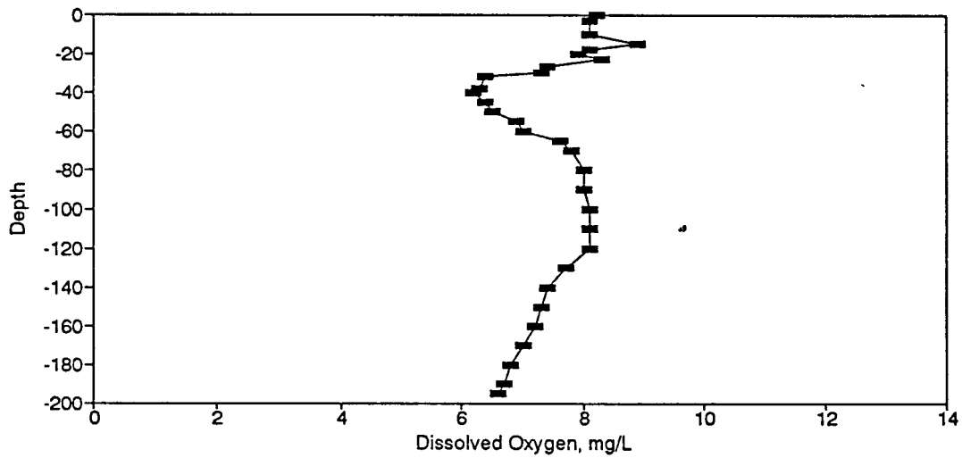
Figure BD149. Dissolved Oxygen Profile for the Eureka Springs Site-June 4, 1986.
