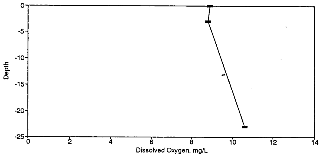
Figure BD161. Dissolved Oxygen Profile for the Eureka Springs Site-June 10, 1987.
