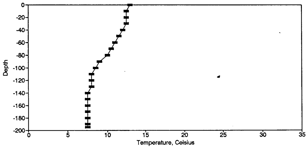
Figure BT5. Temperature Profile for the Eureka Springs Site-April 16, 1974.
