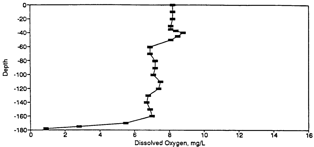
Figure BD46. Dissolved Oxygen Profile for the Eureka Springs Site-September 12, 1977.
