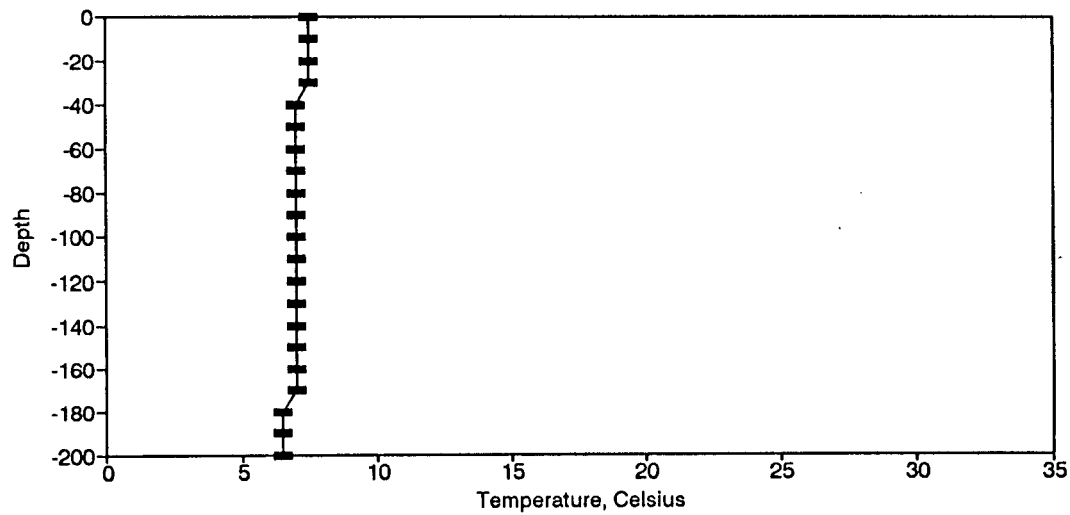
Figure BT3. Temperature Profile for the Eureka Springs Site-February 20, 1974.
