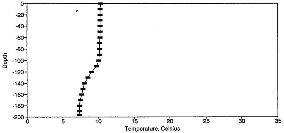
Figure BT178. Temperature Profile for the Eureka Springs Site-December 14, 1988.
