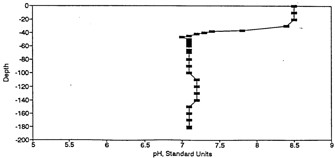
Figure BP69. pH Profile for the Eureka Springs Site - September 17, 1979.
