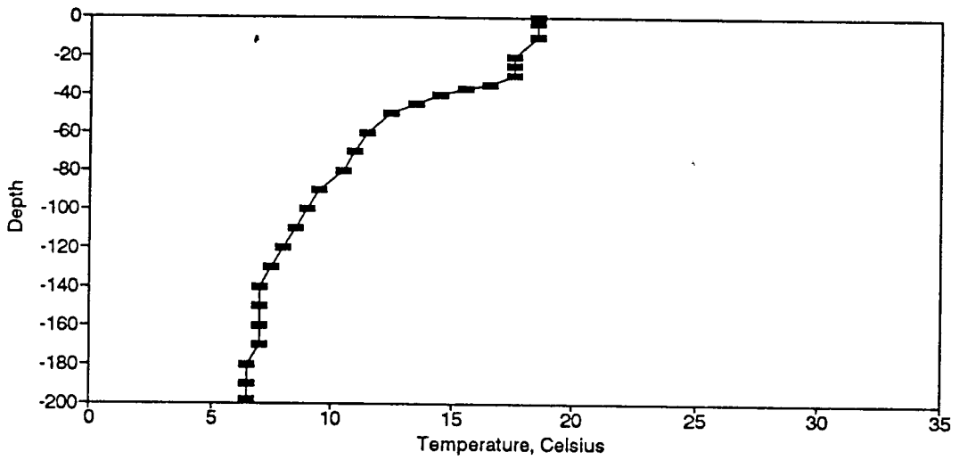
Figure BT172. Temperature Profile for the Eureka Springs Site-May 10, 1988.
