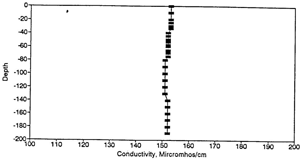
Figure BC88. Conductivity Profile for the Eureka Springs Site-May 13, 1981
