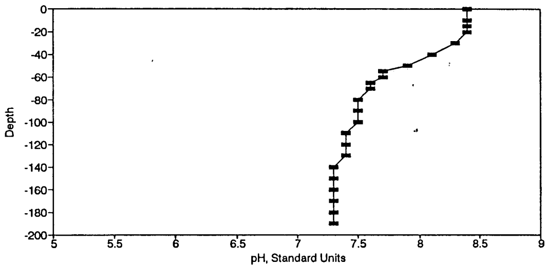
Figure BP29. pH Profile for the Eureka Springs Site-May 25, 1976.
