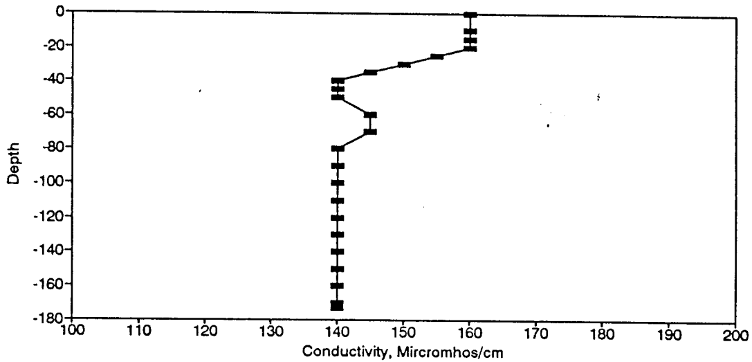
Figure BC44. Conductivity Profile for the Eureka Springs Site-July 26, 1977.
