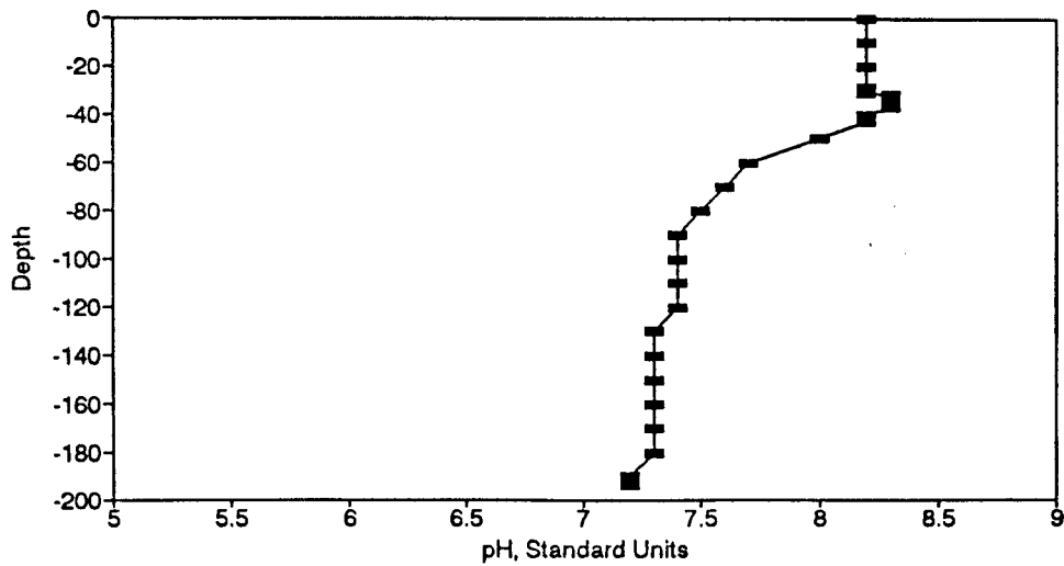
Figure BP78. pH Profile for the Eureka Springs Site-June 19, 1980.
