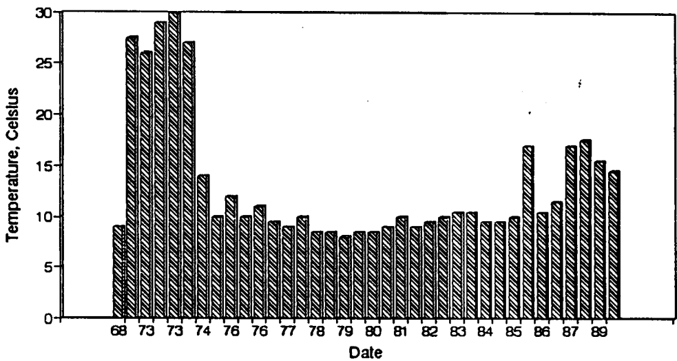
Figure A104. Graph of Temperature vs. Time for the White River Site-Aug.
