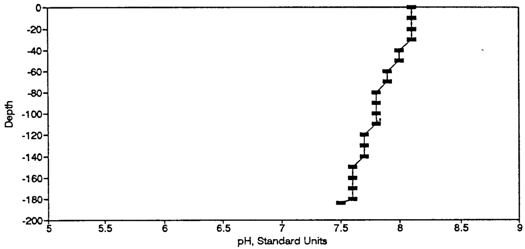
Figure BP98. pH Profile for the Eureka Springs Site-March 23, 1982.
