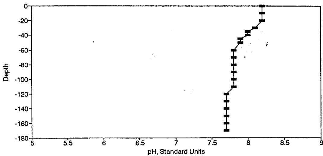
Figure BP41. pH Profile for the Eureka Springs Site-May 1, 1977.
