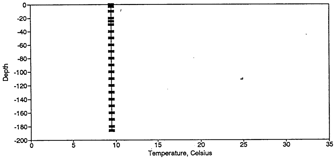
Figure BT143. Temperature Profile for the Eureka Springs Site-December 19, 1985.
