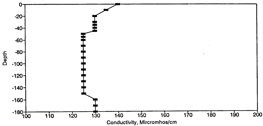
Figure BC33. Conductivity Profile for the Eureka Springs Site-September 22, 1976.
