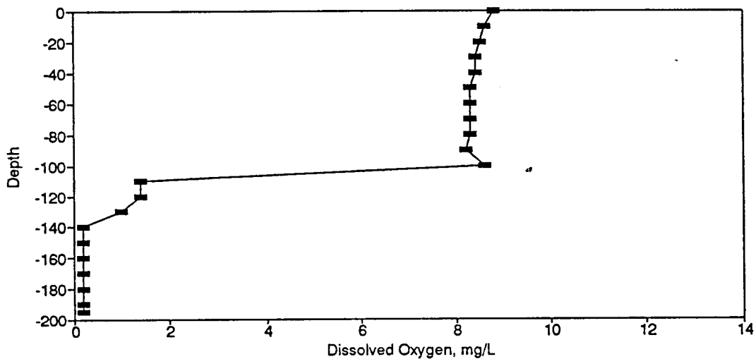
Figure BD155. Dissolved Oxygen Profile for the Eureka Springs Site-December 4, 1986.
