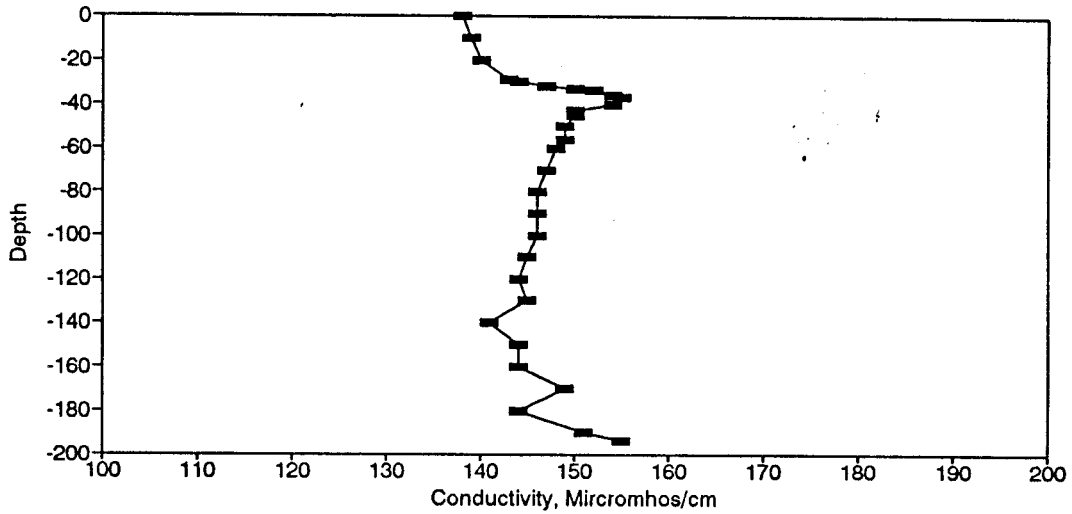
Figure BC176. Conductivity Profile for the Eureka Springs Site-September 21, 1988.
