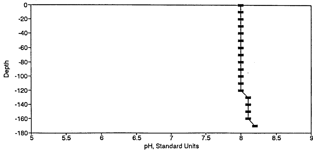
Figure BP120. pH Profile for the Eureka Springs Site-January 25, 1984.
