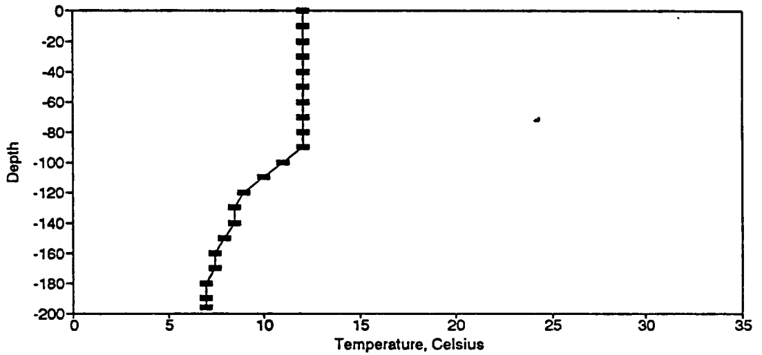
Figure BT107. Temperature Profile for the Eureka Springs Site-December 8, 1982.
