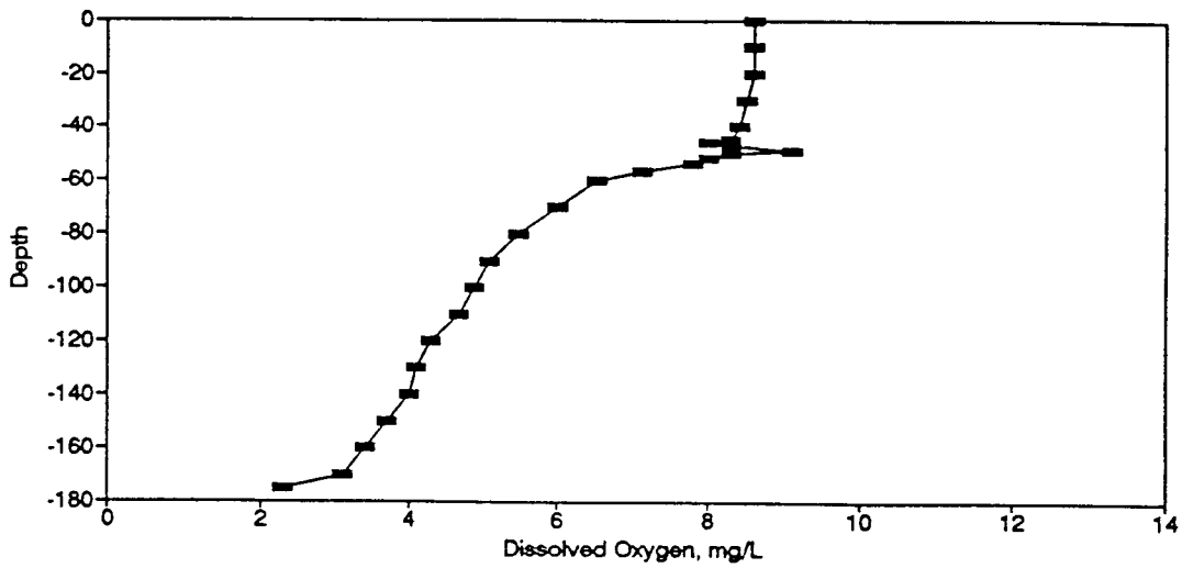
Figure BD82. Dissolved Oxygen Profile for the Eureka Springs Site-October 6, 1980.
