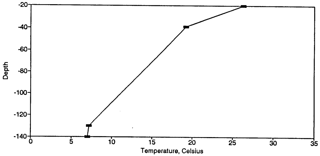
Figure BT187. Temperature Profile for the Eureka Springs Site-September 11, 1989.
