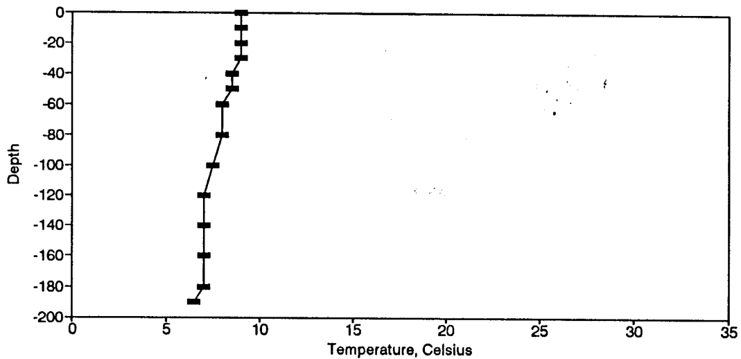
Figure BT26. Temperature Profile for the Eureka Springs Site-February 24, 1976.
