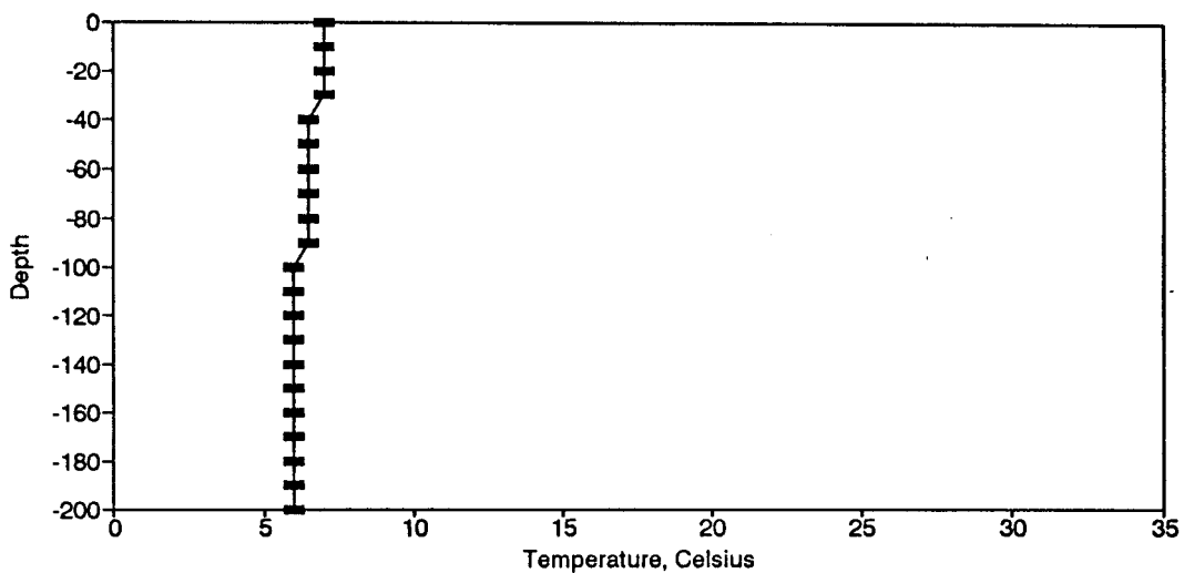
Figure BT15. Temperature Profile for the Eureka Springs Site-March 17, 1975.
