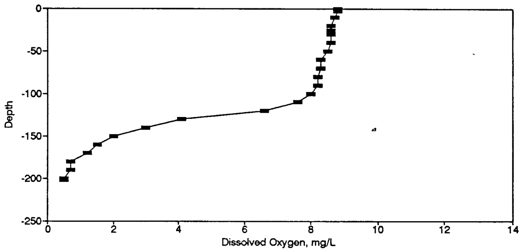
Figure BD131. Dissolved Oxygen Profile for the Eureka Springs Site-December 13, 1984.
