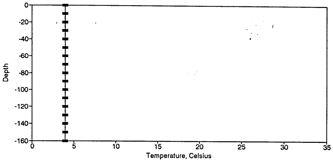
Figure BT38. Temperature Profile for the Eureka Springs Site-February 7, 1977.
