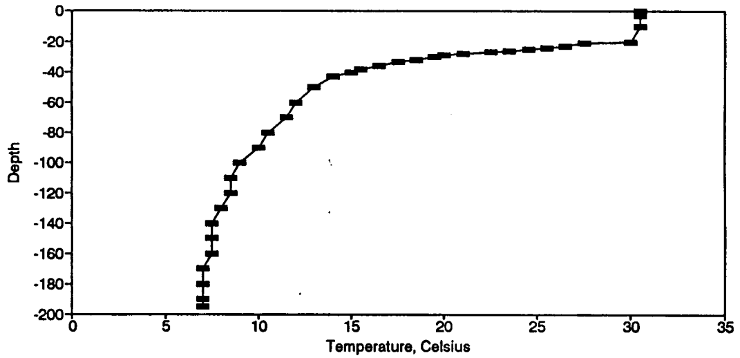
Figure BT175. Temperature Profile for the Eureka Springs Site-August 9, 1988.
