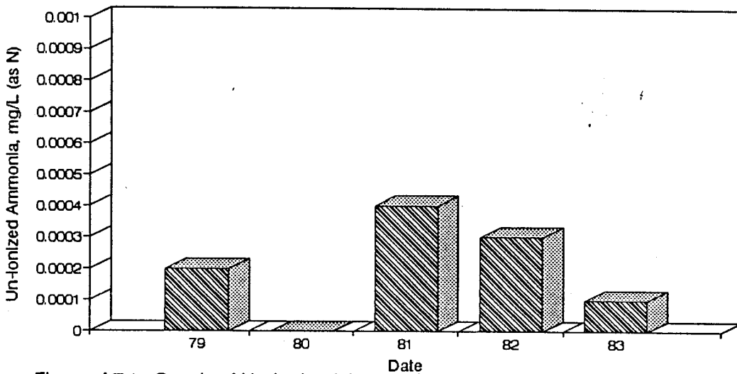
Figure A74. Graph of Un-ionized Ammonia vs. Time for the White River Site-Aug.
