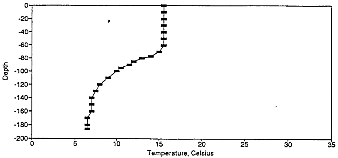
Figure BT94. Temperature Profile for the Eureka Springs Site-November 16, 1981.
