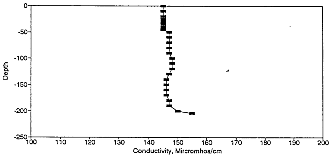
Figure BC113. Conductivity Profile for the Eureka Springs Site-June 14, 1983.
