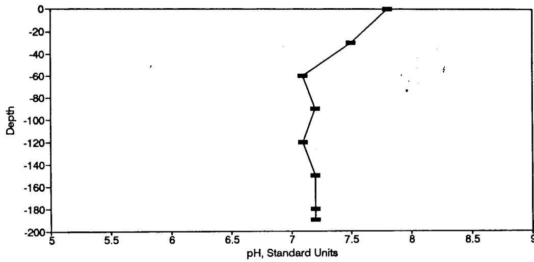
Figure BP23. pH Profile for the Eureka Springs Site-November 18, 1975.
