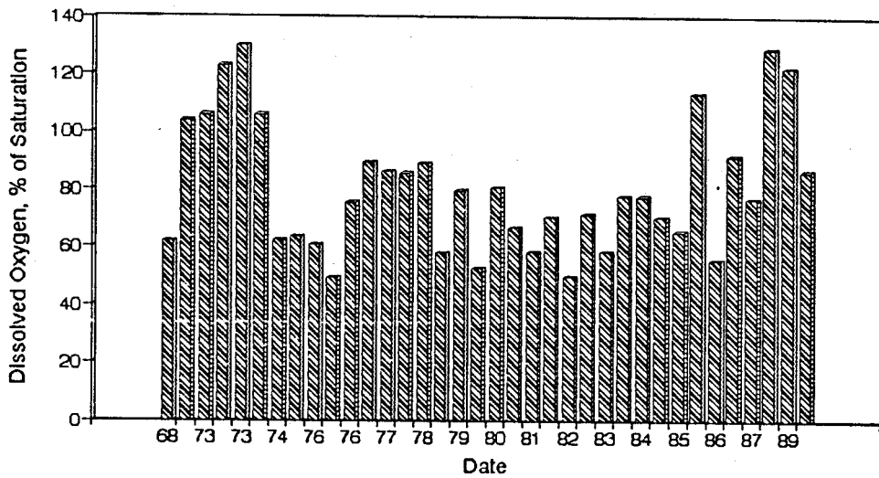
Figure A20. Graph of Dissolved Oxygen vs. Time for the White River Site-Aug.
