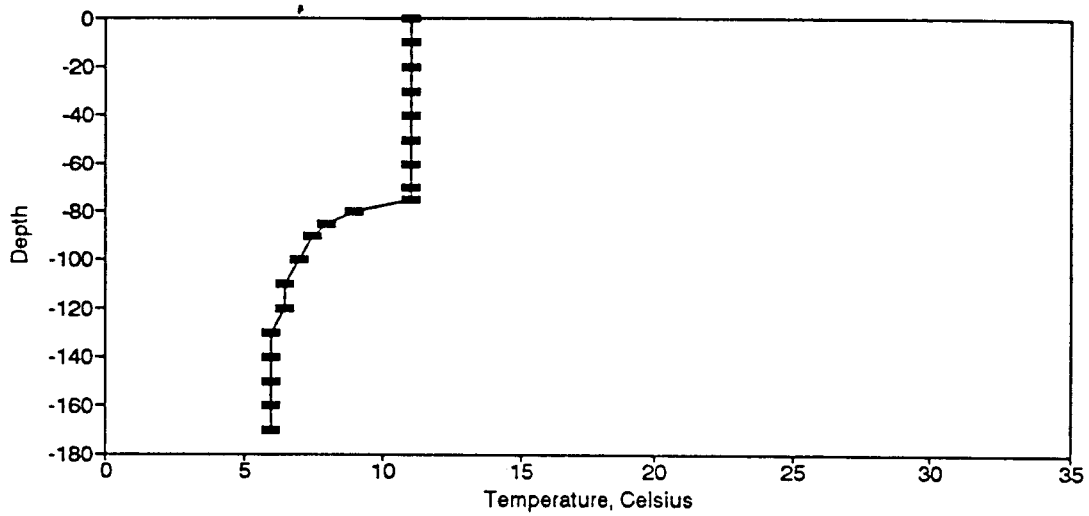
Figure BT40. Temperature Profile for the Eureka Springs Site-April 5, 1977.
