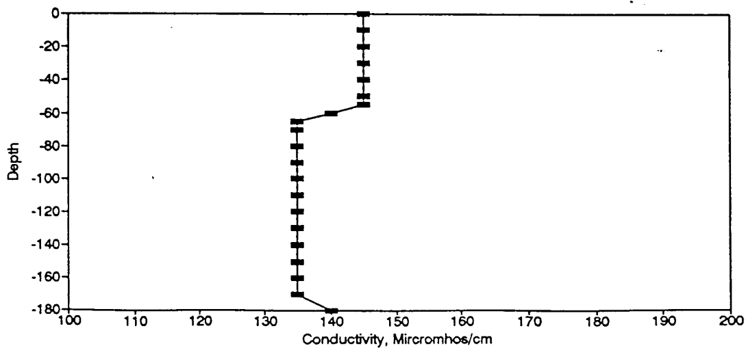
Figure BC48. Conductivity Profile for the Eureka Springs Site-November 9, 1977.
