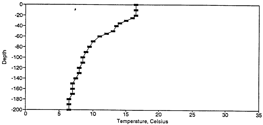
Figure BT112. Temperature Profile for the Eureka Springs Site-May 18 1983.
