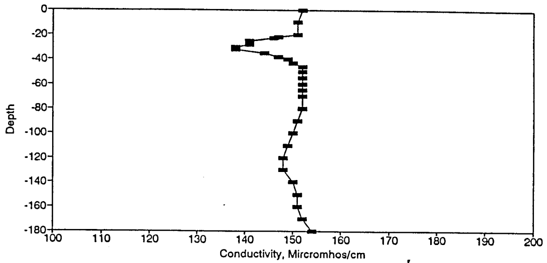
Figure BC103. Conductivity Profile for the Eureka Springs Site-August 18, 1982.
