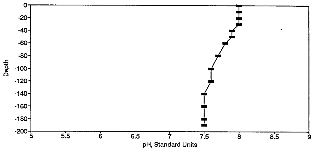
Figure BP26. pH Profile for the Eureka Springs Site-February 24, 1976.
