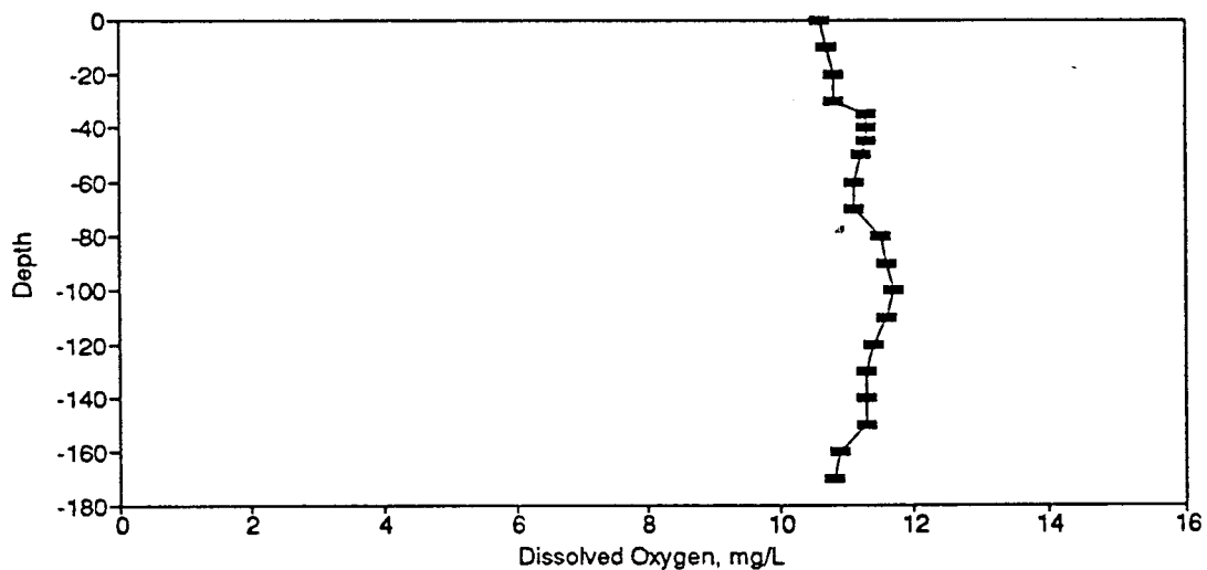
Figure BD41. Dissolved Oxygen Profile for the Eureka Springs Site-May 1, 1977.
