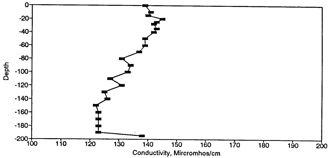
Figure BC7. Conductivity Profile for the Eureka Springs Site - July 8, 1974.
