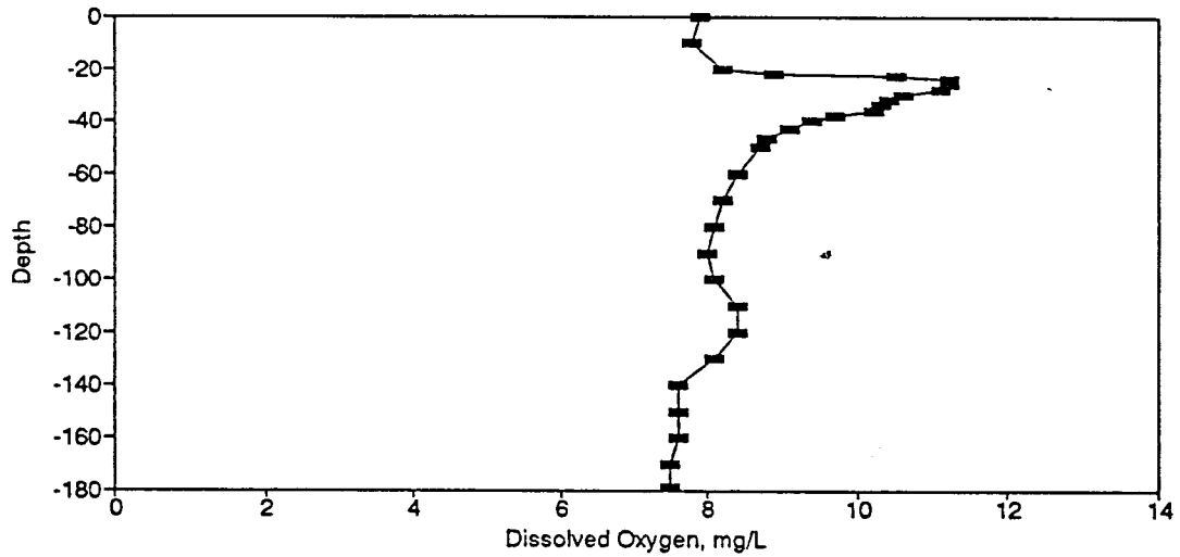
Figure BD125. Dissolved Oxygen Profile for the Eureka Springs Site-June 26, 1984.
