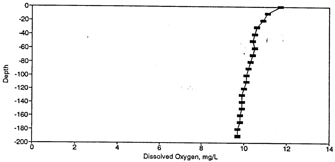
Figure BD182. Dissolved Oxygen Profile for the Eureka Springs Site-April 11, 1989.
