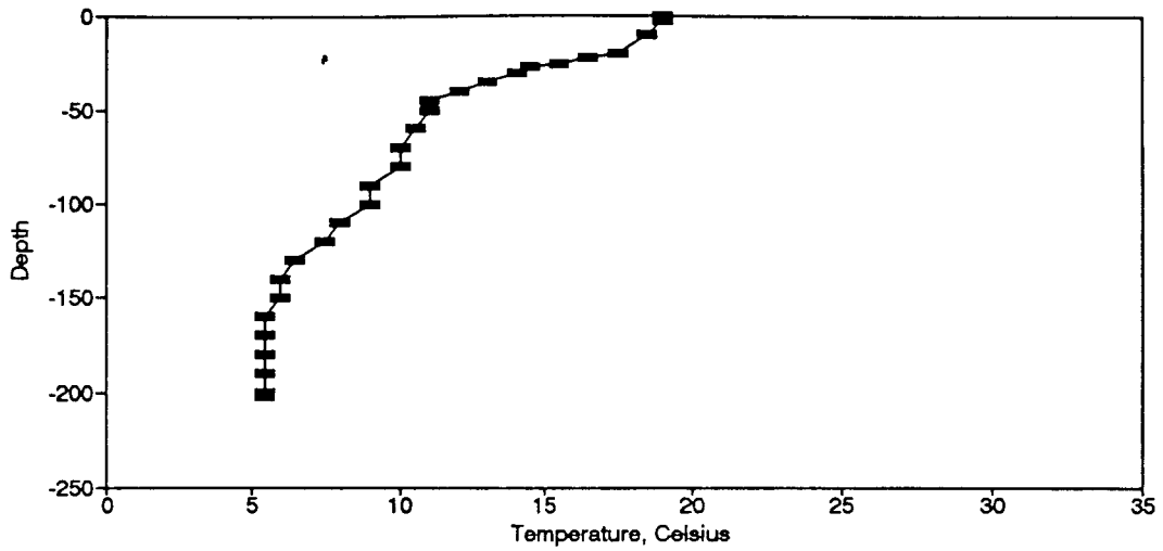
Figure BT136. Temperature Profile for the Eureka Springs Site-May 8, 1985.
