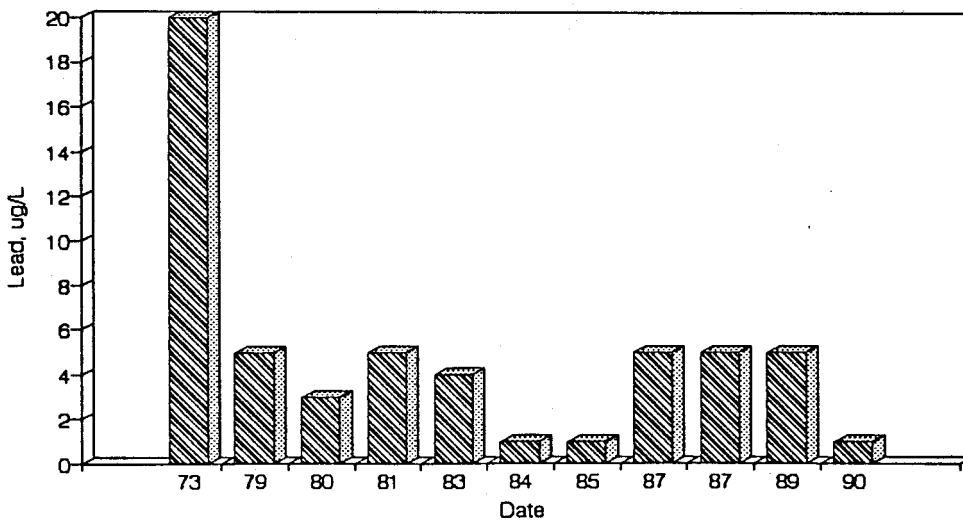
Figure A57. Graph of Lead vs. Time for the White River Site-Dec.
