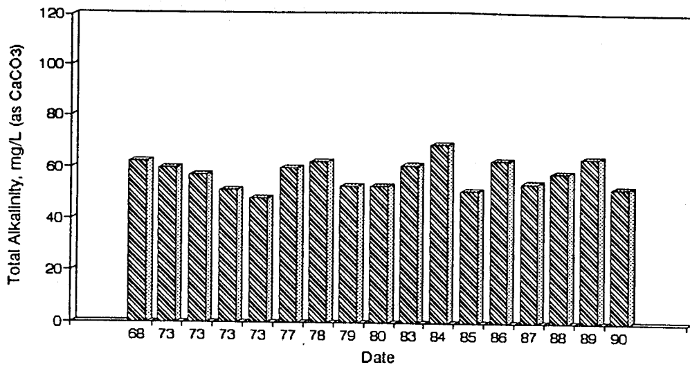
Figure A1. Graph of Total Alkalinity vs. Time for the White River Site-May.
