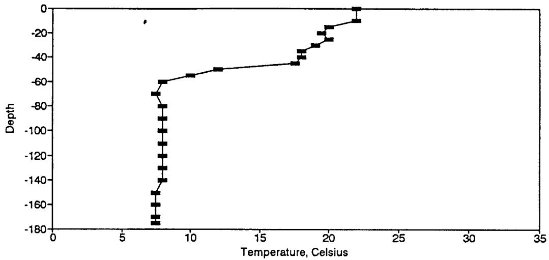
Figure BT22. Temperature Profile for the Eureka Springs Site-October 14, 1975.
