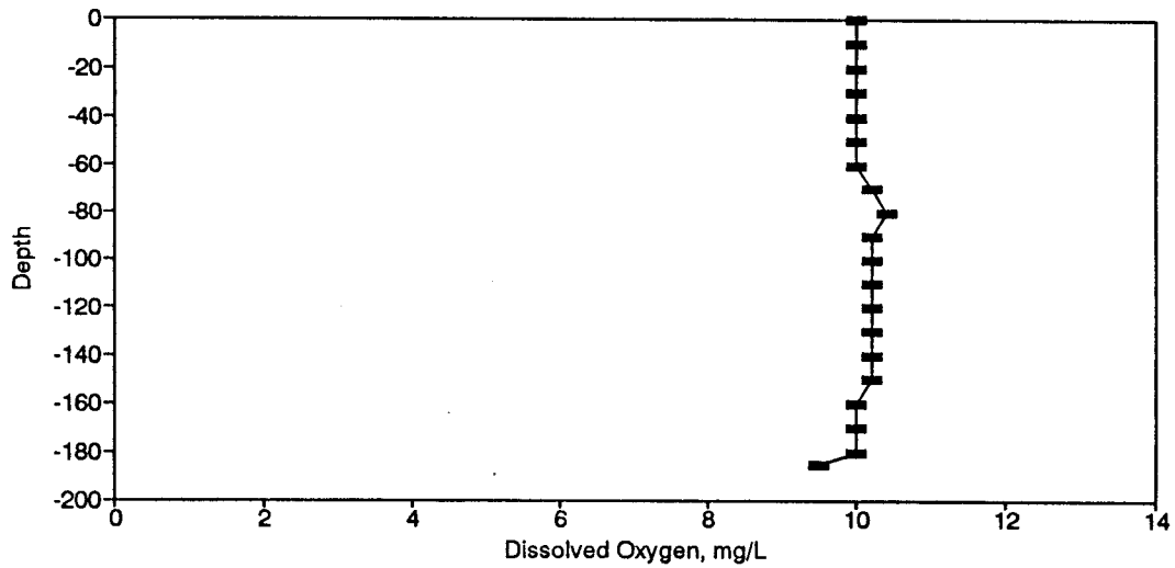
Figure BD25. Dissolved Oxygen Profile for the Eureka Springs Site-January 20, 1976.
