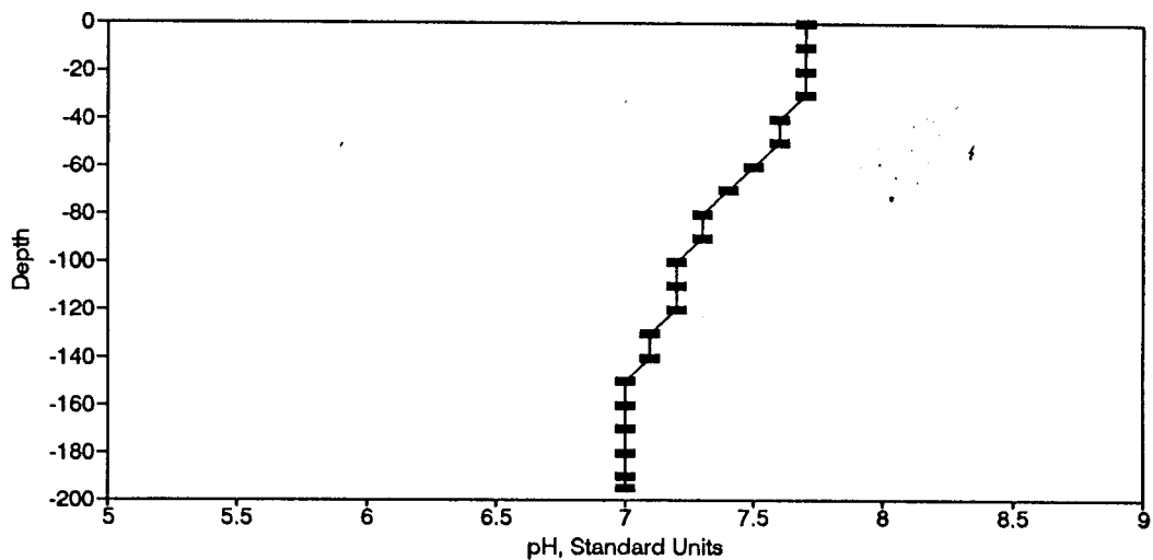
Figure BP5. pH Profile for the Eureka Springs Site-April 16, 1974.
