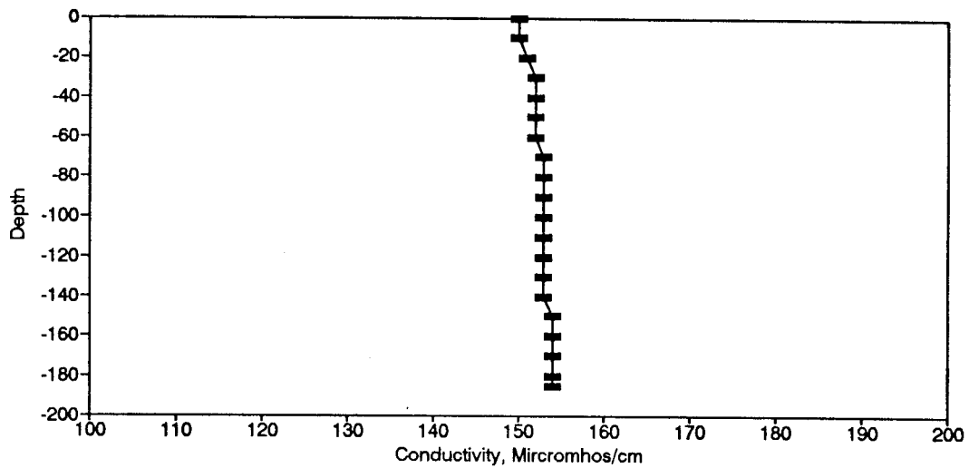
Figure BC85. Conductivity Profile for the Eureka Springs Site-February 3, 1981.
