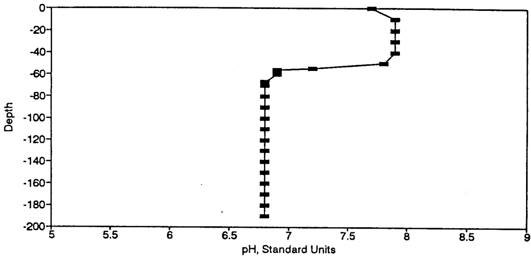
Figure BP70. pH Profile for the Eureka Springs Site-October 16, 1979.
