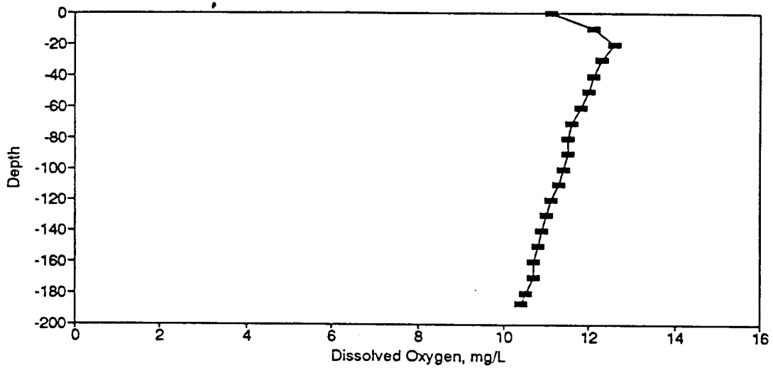
Figure BD64. Dissolved Oxygen Profile for the Eureka Springs Site-April 9, 1979.
