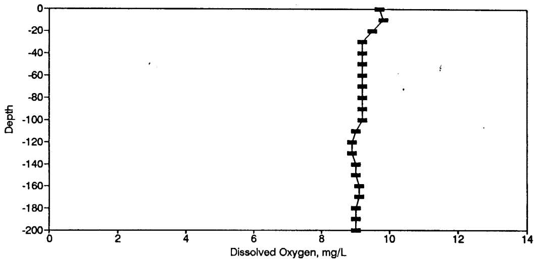
Figure BD2. Dissolved Oxygen Profile for the Eureka Springs Site-January 15, 1974.
