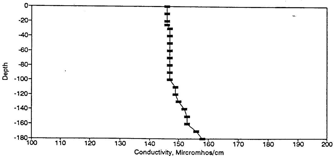
Figure BC72. Conductivity Profile for the Eureka Springs Site-December 5, 1979.
