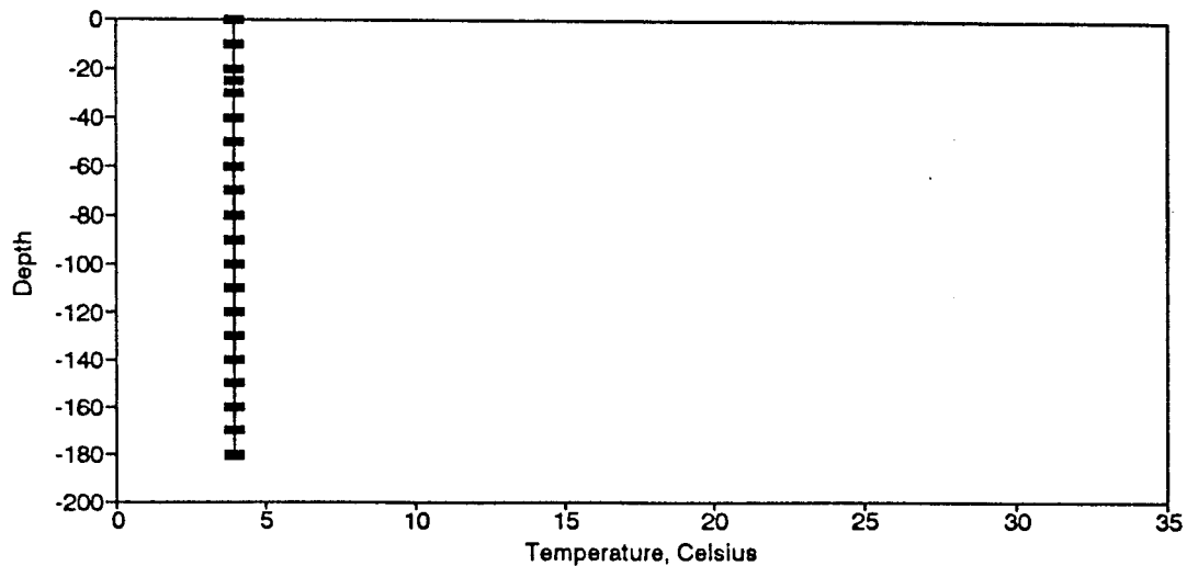
Figure BT63. Temperature Profile for the Eureka Springs Site-March 8, 1979.
