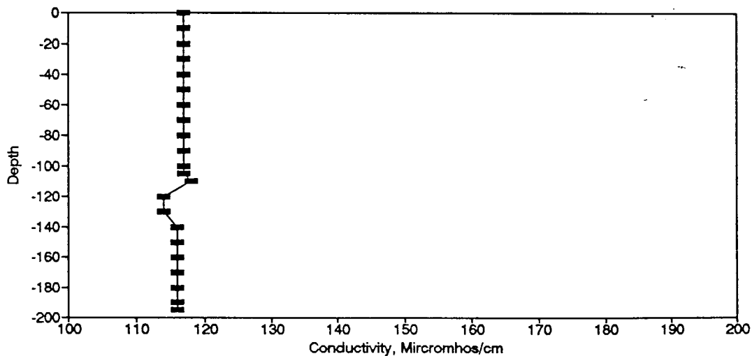
Figure BC24. Conductivity Profile for the Eureka Springs Site-December 16, 1975.
