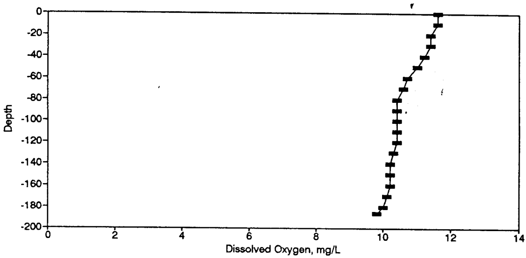
Figure BD86. Dissolved Oxygen Profile for the Eureka Springs Site-March 3, 1981.
