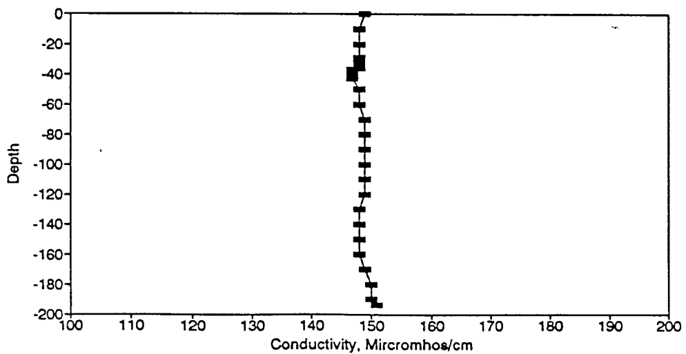
Figure BC78. Conductivity Profile for the Eureka Springs Site-June 19, 1980.
