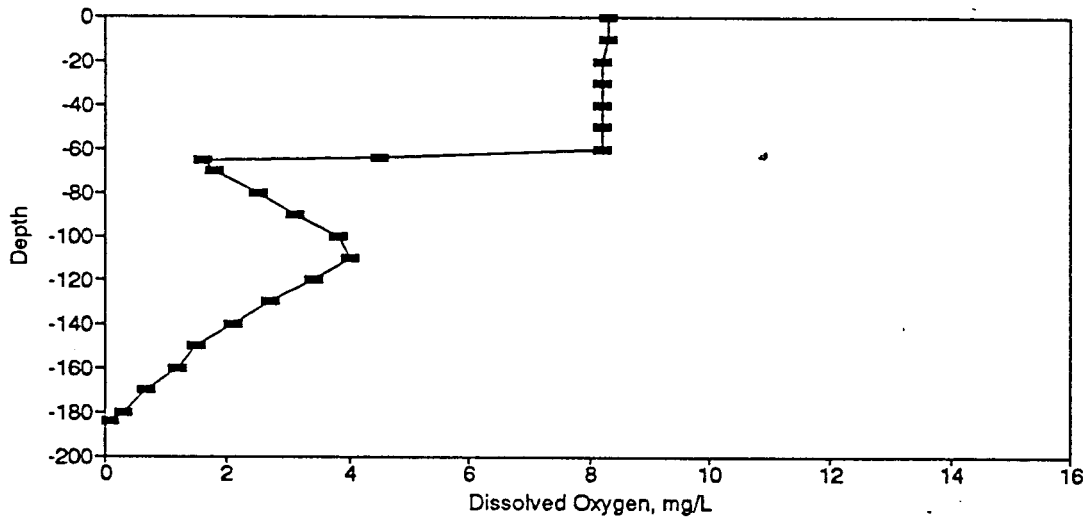
Figure BD71. Dissolved Oxygen Profile for the Eureka Springs Site-November 6, 1979.
