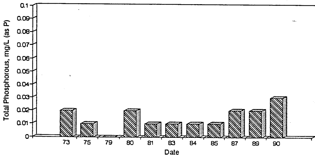
Figure A96. Graph of Total Phosphorous vs. Time for the White River Site-Dec.
