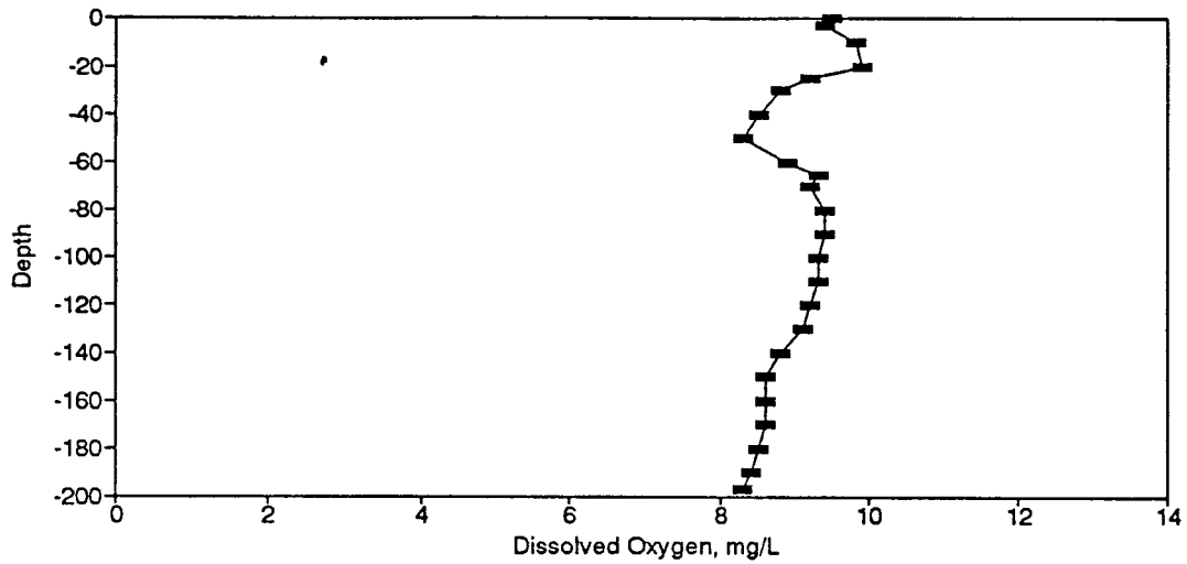
Figure BD148. Dissolved Oxygen Profile for the Eureka Springs Site-May 6, 1986.
