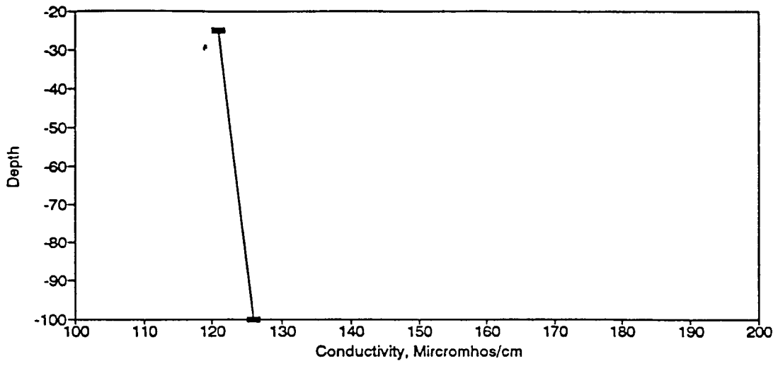
Figure BC190. Conductivity Profile for the Eureka Springs Site-July 31, 1990.
