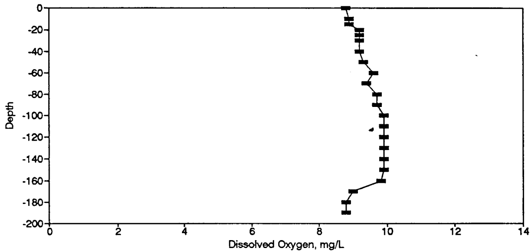
Figure BD17. Dissolved Oxygen Profile for the Eureka Springs Site-May 14, 1975.
