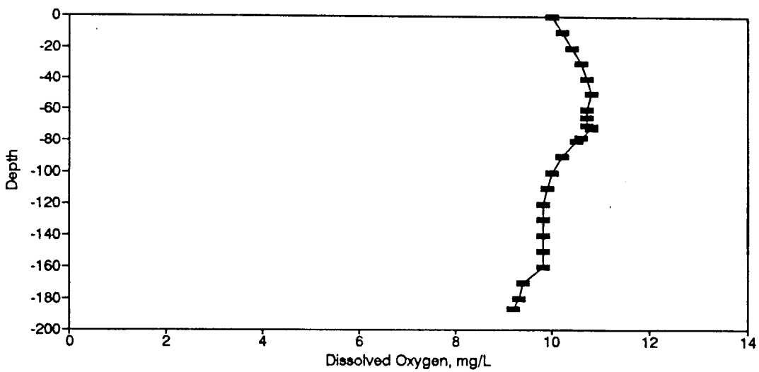
Figure BD87. Dissolved Oxygen Profile for the Eureka Springs Site-April 13, 1981.
