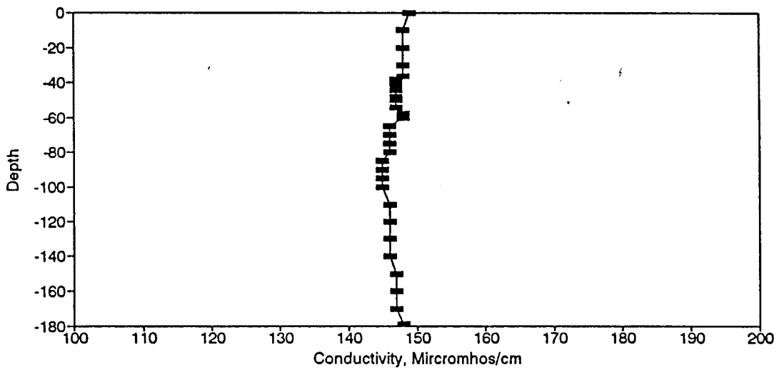
Figure BC92. Conductivity Profile for the Eureka Springs Site-September 14, 1981.
