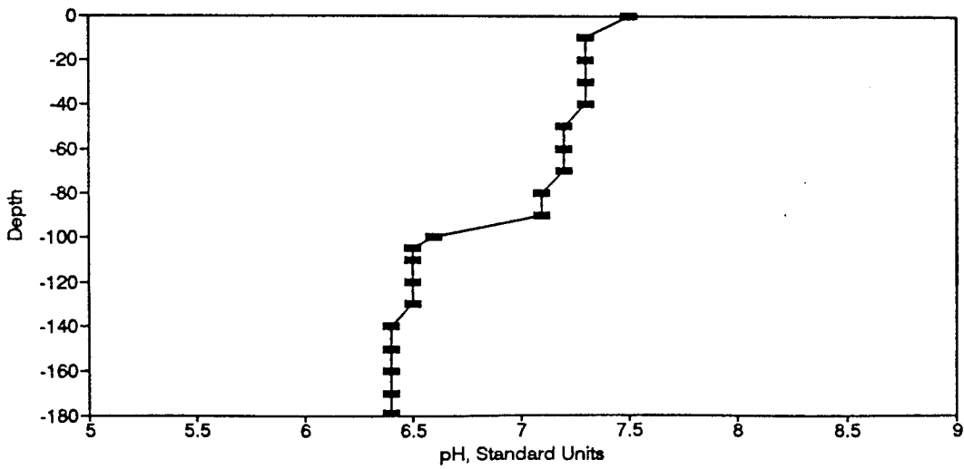
Figure BP60. pH Profile for the Eureka Springs Site-December 5, 1978.
