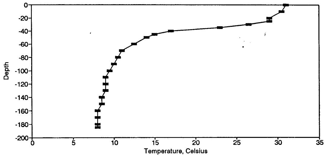
Figure BT20. Temperature Profile for the Eureka Springs Site-August 13, 1975.
