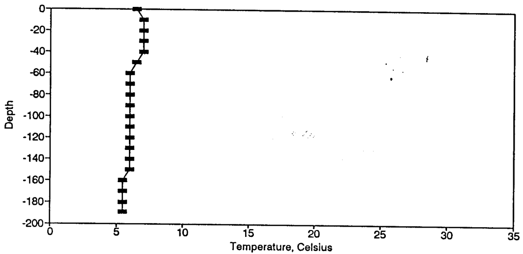
Figure BT146. Temperature Profile for the Eureka Springs Site-March 6, 1986.
