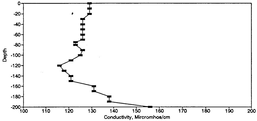
Figure BC10. Conductivity Profile for the Eureka Springs Site-October 22, 1974.
