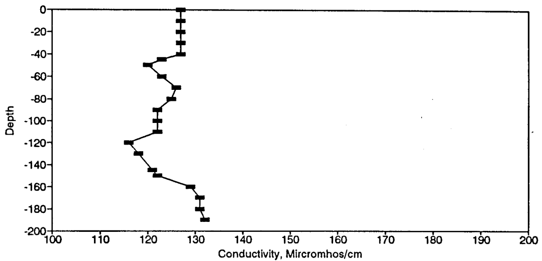
Figure BC9. Conductivity Profile for the Eureka Springs Site - September 24, 1974.
