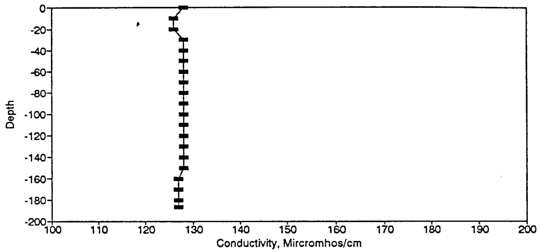
Figure BC64. Conductivity Profile for the Eureka Springs Site-April 9, 1979.
