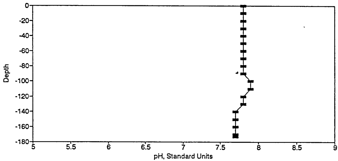
Figure BP122. pH Profile for the Eureka Springs Site-March 28, 1984.
