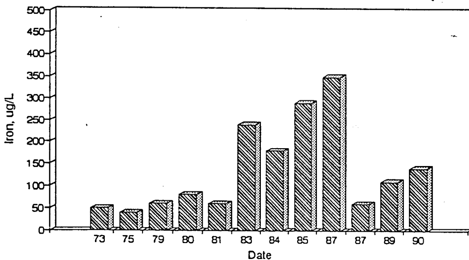
Figure A54. Graph of Iron vs. Time for the White River Site-Dec.
