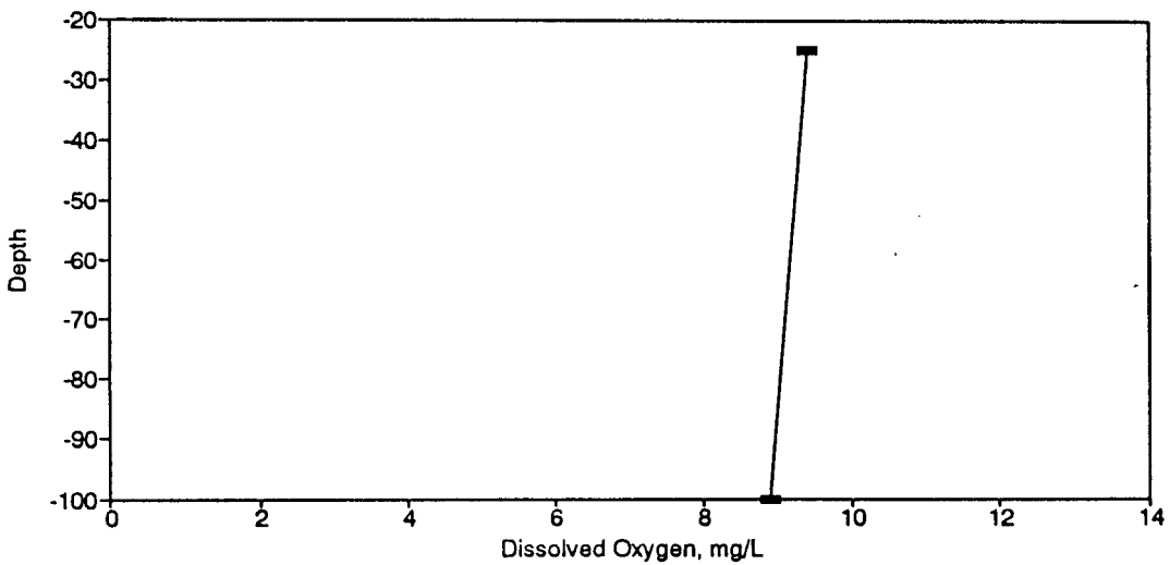
Figure BD189. Dissolved Oxygen Profile for the Eureka Springs Site-May 15, 1990.
