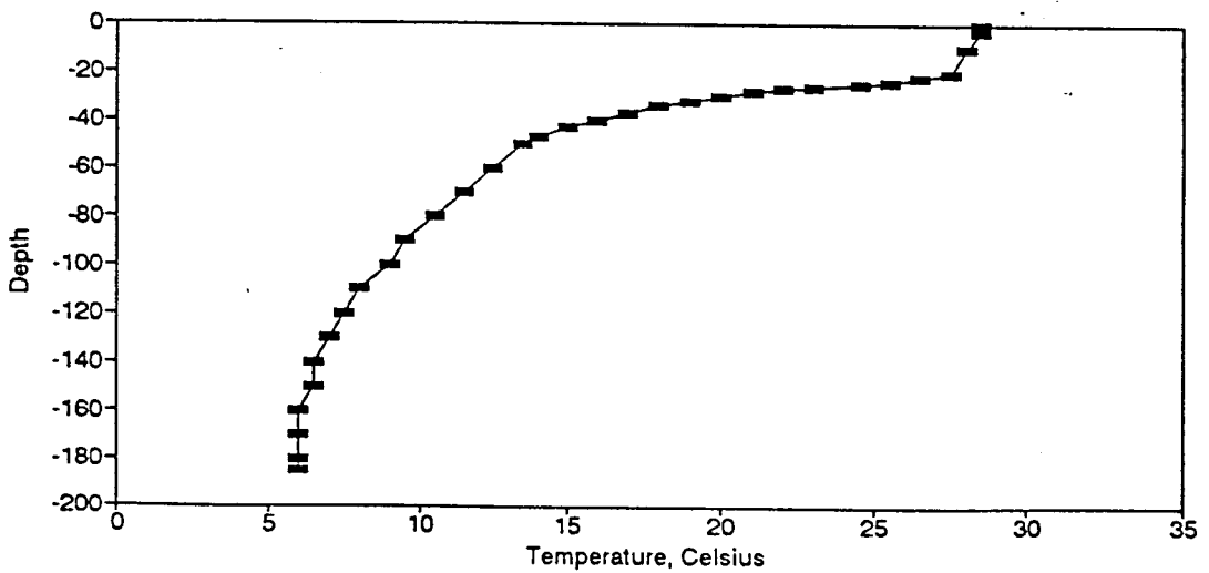
Figure BT126. Temperature Profile for the Eureka Springs Site-July 17, 1984.
