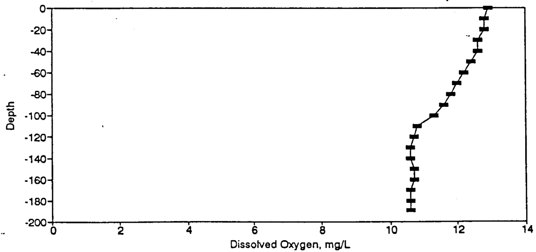
Figure BD180. Dissolved Oxygen Profile for the Eureka Springs Site-February 15, 1989.
