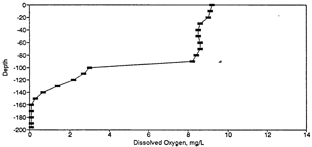
Figure BD107. Dissolved Oxygen Profile for the Eureka Springs Site-December 8, 1982.
