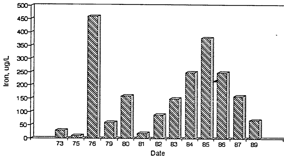
Figure A53. Graph of Iron vs. Time for the White River Site-Aug.
