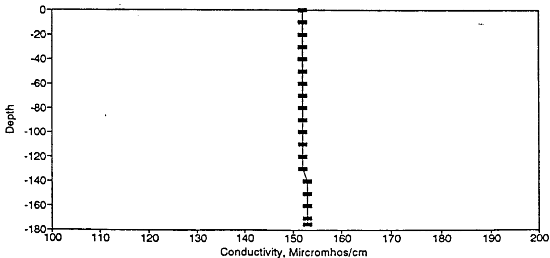
Figure BC96. Conductivity Profile for the Eureka Springs Site-January 26, 1982.
