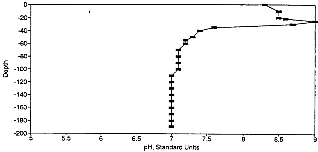
Figure BP55. pH Profile for the Eureka Springs Site-July 18, 1978.
