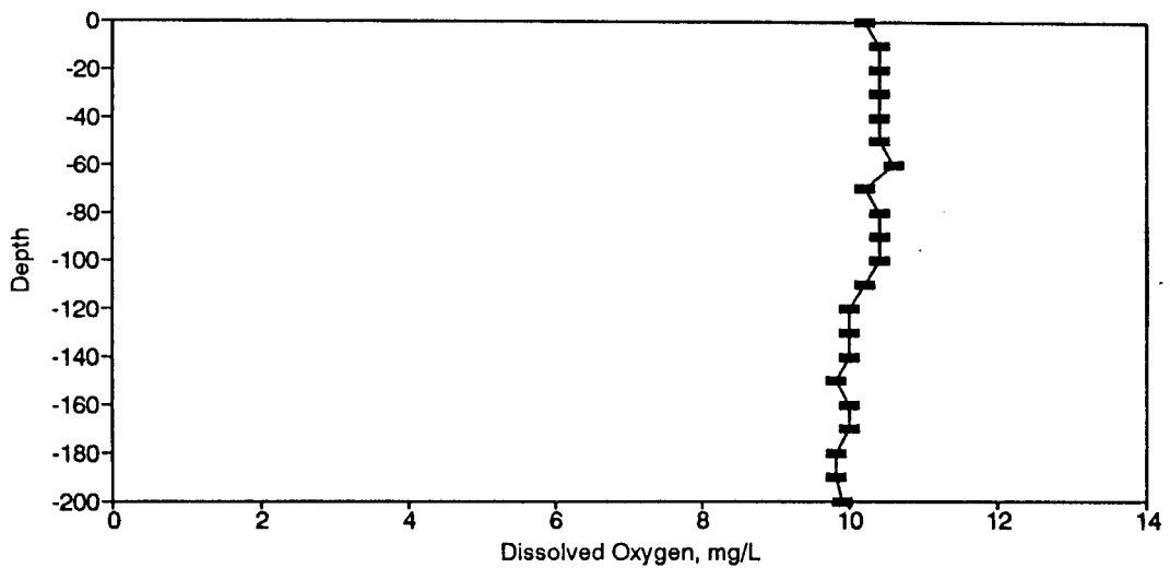
Figure BD15. Dissolved Oxygen Profile for the Eureka Springs Site-March 17, 1975.
