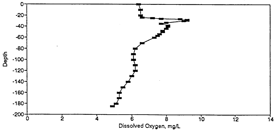
Figure BD102. Dissolved Oxygen Profile for the Eureka Springs Site-July 20, 1982.
