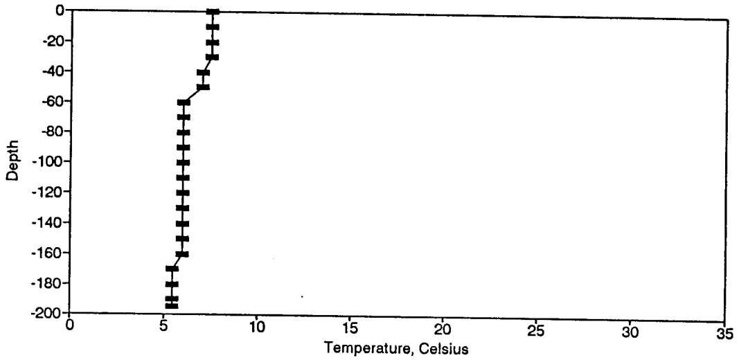
Figure BT145. Temperature Profile for the Eureka Springs Site-February 20, 1986.
