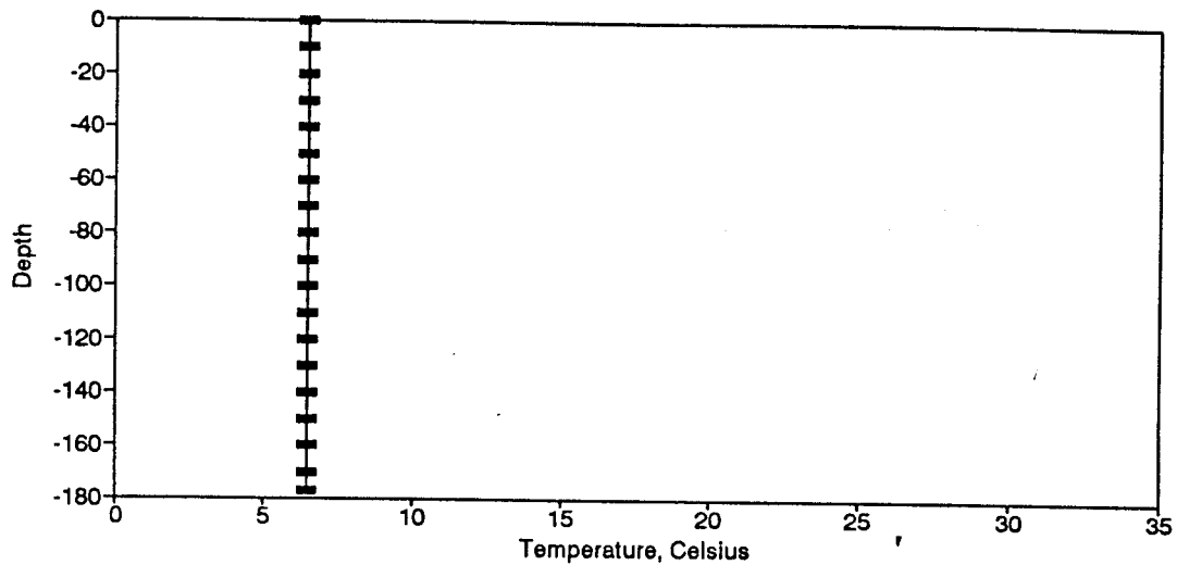
Figure BT61. Temperature Profile for the Eureka Springs Site-January 9, 1979.
