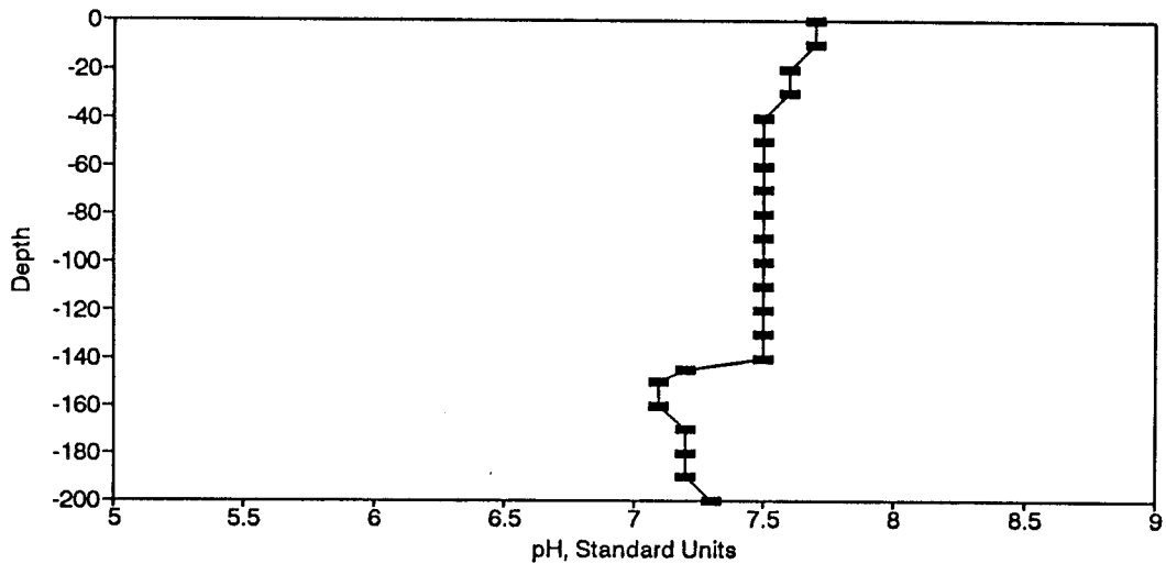
Figure BP1. pH Profile for the Eureka Springs Site-December 18, 1973.
