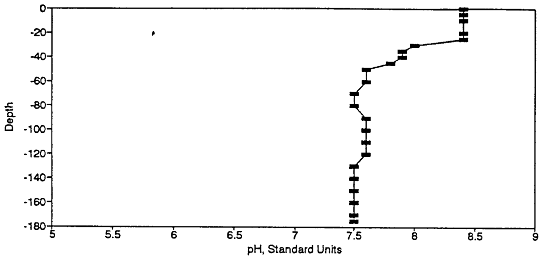
Figure BP43. pH Profile for the Eureka Springs Site-June 27, 1977.
