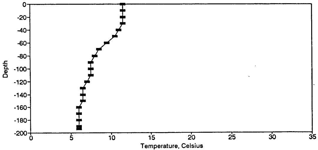
Figure BT171. Temperature Profile for the Eureka Springs Site-April 13, 1988.
