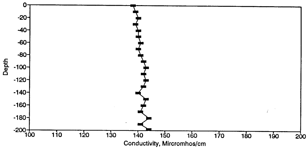
Figure BC169. Conductivity Profile for the Eureka Springs Site-February 24, 1988.
