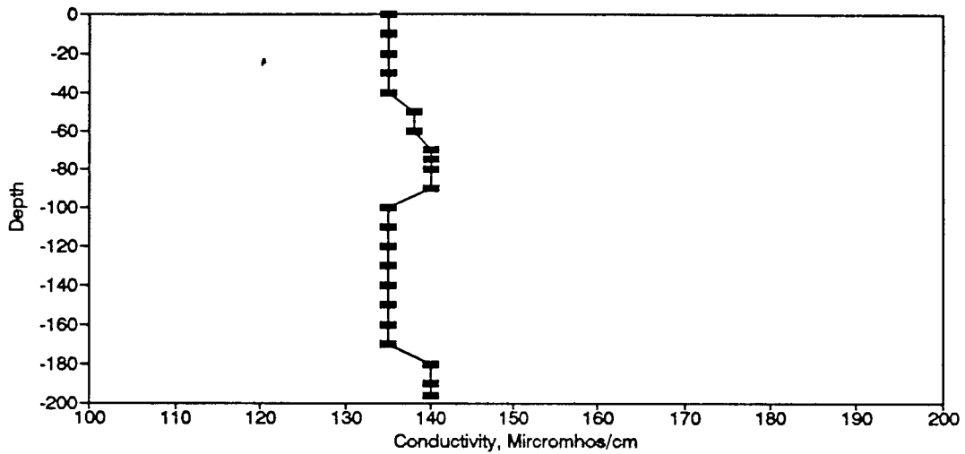
Figure BC130. Conductivity Profile for the Eureka Springs Site-November 8, 1984.
