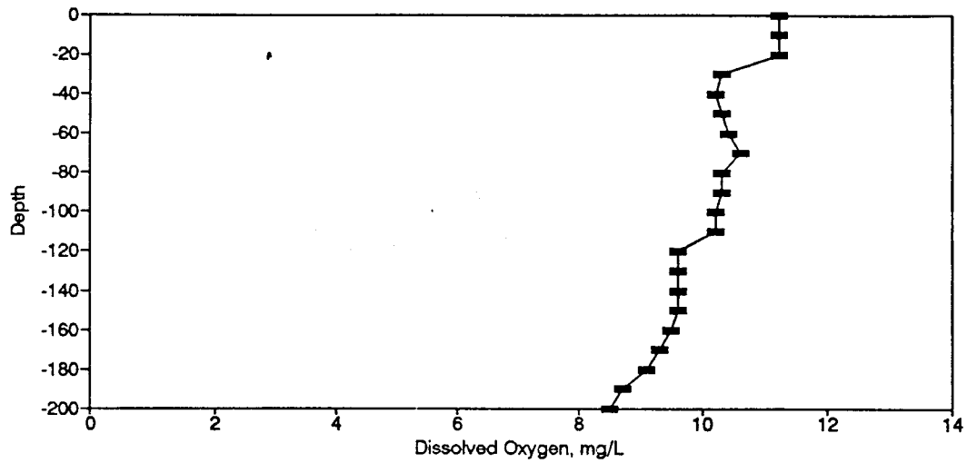
Figure BD4. Dissolved Oxygen Profile for the Eureka Springs Site-March 19, 1974.
