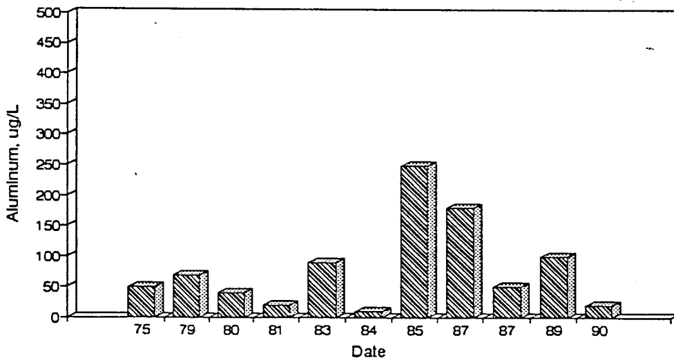
Figure A42. Graph of Aluminum vs. Time for the White River Site-Dec.
