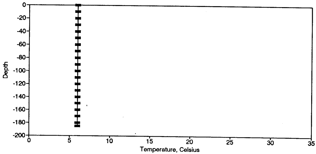
Figure BT85. Temperature Profile for the Eureka Springs Site-February 3, 1981.
