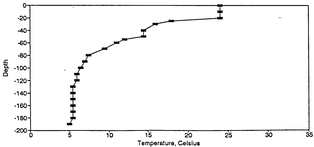
Figure BT54. Temperature Profile for the Eureka Springs Site-June 15, 1978.
