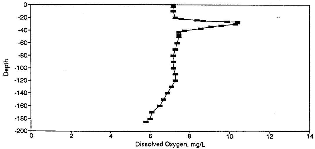
Figure BD126. Dissolved Oxygen Profile for the Eureka Springs Site-July 17, 1984.
