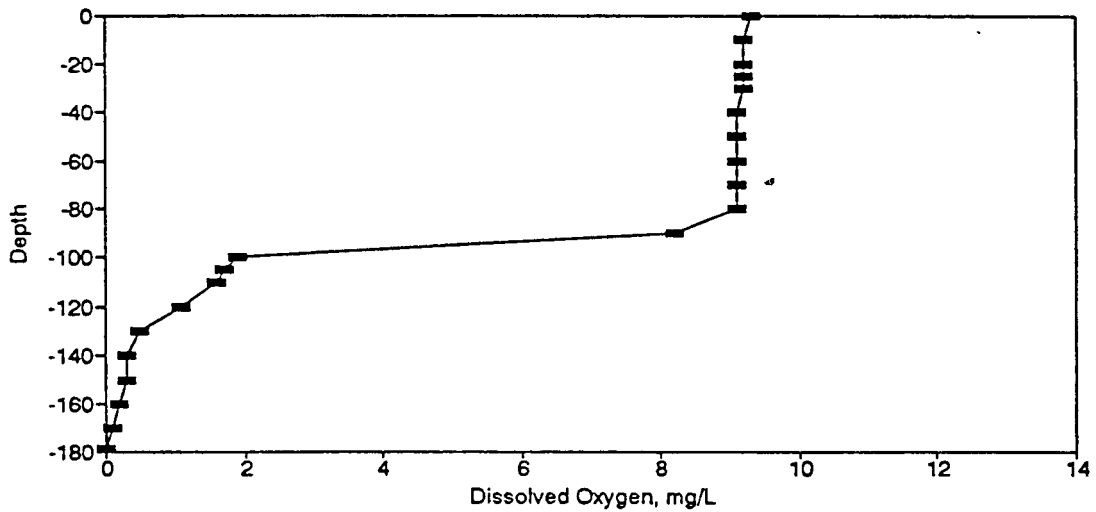
Figure BD95. Dissolved Oxygen Profile for the Eureka Springs Site-December 9, 1981.
