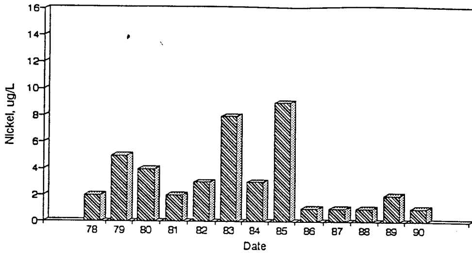
Figure A64. Graph of Nickel vs. Time for the White River Site-May.
