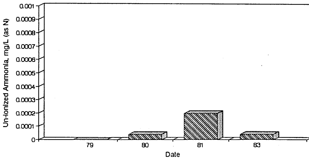
Figure A75. Graph of Un-ionized Ammonia vs. Time for the White River Site-Dec.
