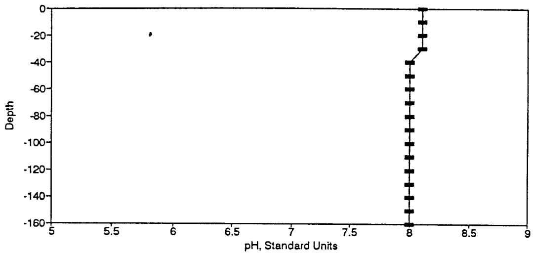
Figure BP37. pH Profile for the Eureka Springs Site-January 26, 1977.
