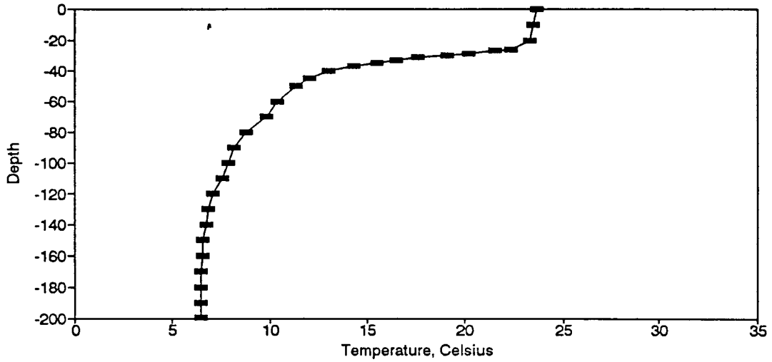
Figure BT184. Temperature Profile for the Eureka Springs Site-June 7, 1989.
