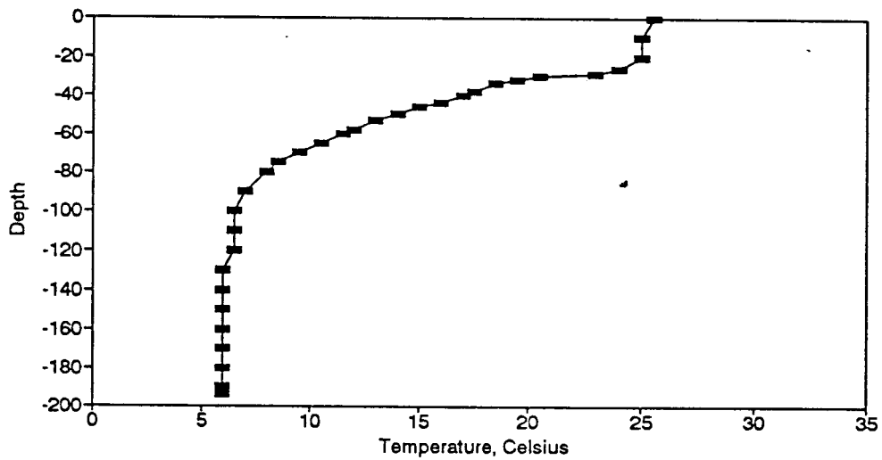
Figure BT89. Temperature Profile for the Eureka Springs Site-June 16, 1981.
