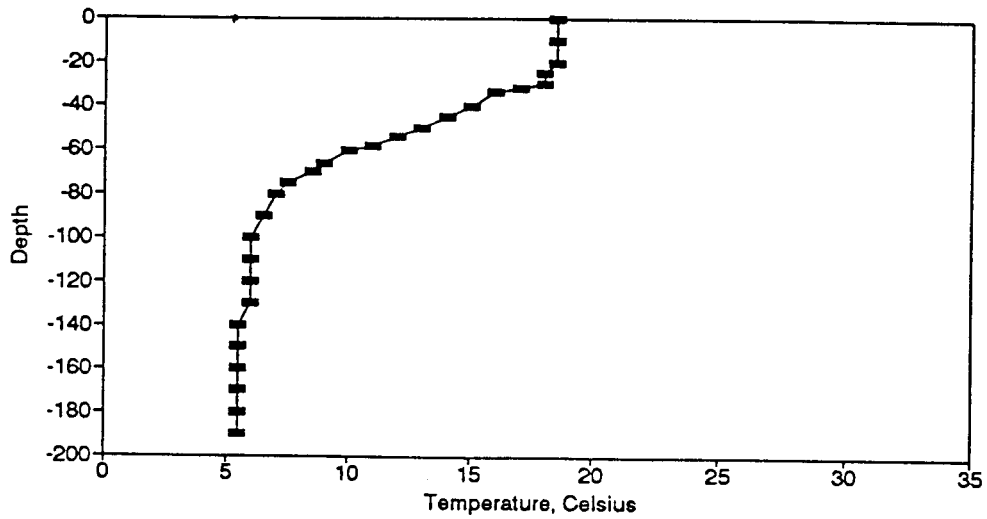
Figure BT88. Temperature Profile for the Eureka Springs Site-May 13, 1981.
