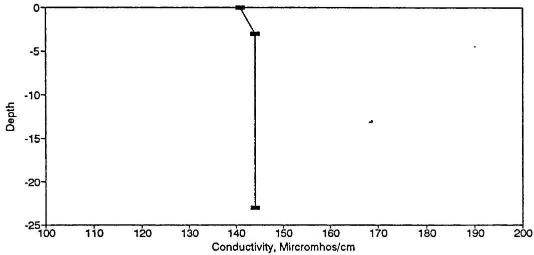
Figure BC161. Conductivity Profile for the Eureka Springs Site-June 10, 1987.
