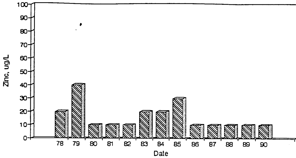
Figure A70. Graph of Zinc vs. Time for the White River Site-May.
