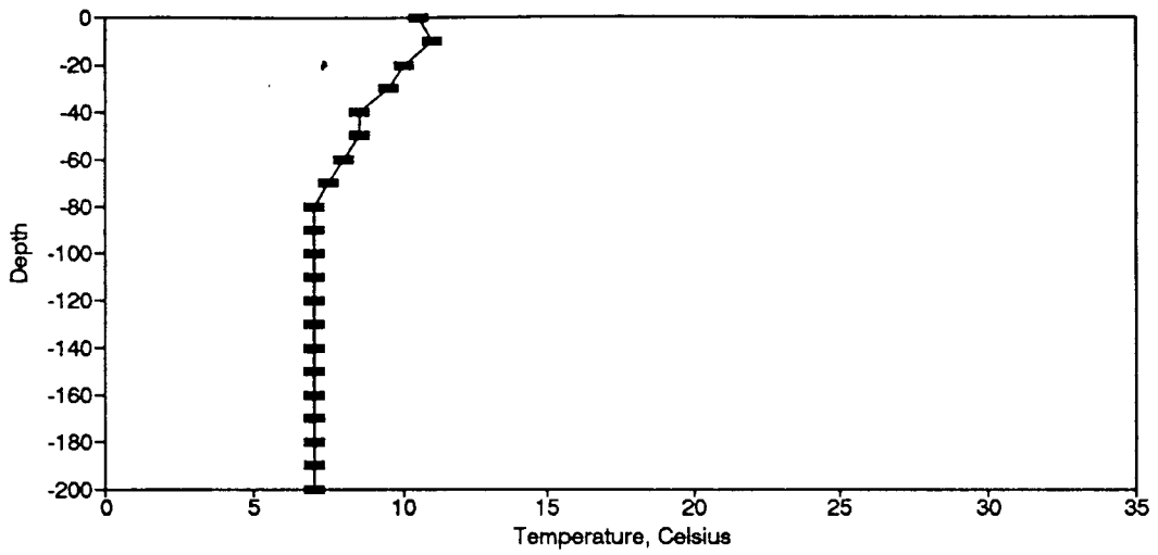
Figure BT4. Temperature Profile for the Eureka Springs Site-March 19, 1974.
