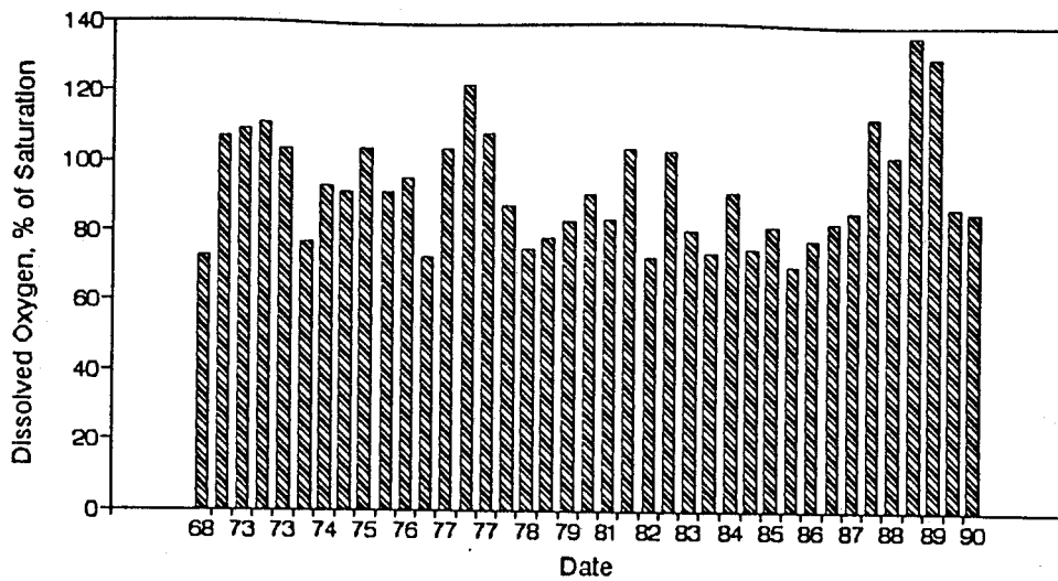
Figure A19. Graph of Dissolved Oxygen vs. Time for the White River Site-May.
