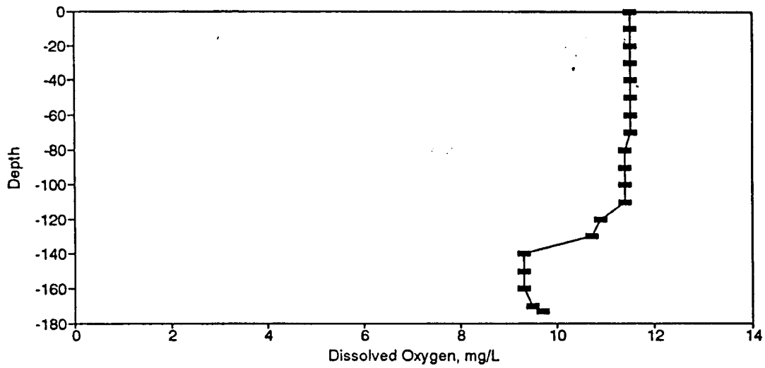
Figure BD122. Dissolved Oxygen Profile for the Eureka Springs Site-March 28, 1984.
