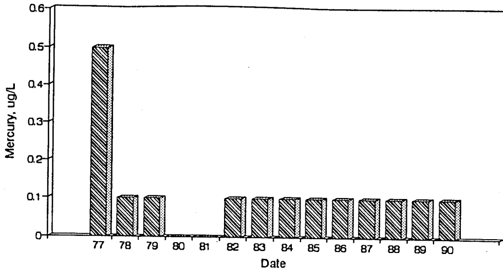
Figure A61. Graph of Mercury vs. Time for the White River Site-May.
