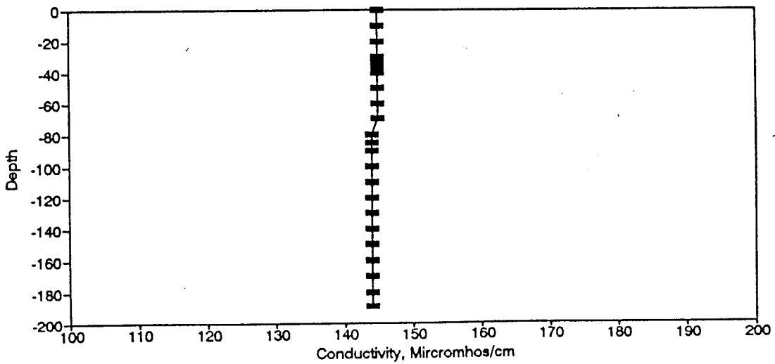
Figure BC99. Conductivity Profile for the Eureka Springs Site-April 20, 1982.
