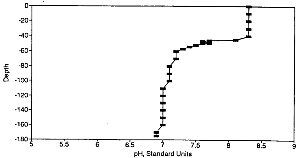
Figure BP82. pH Profile for the Eureka Springs Site-October 6, 1980.
