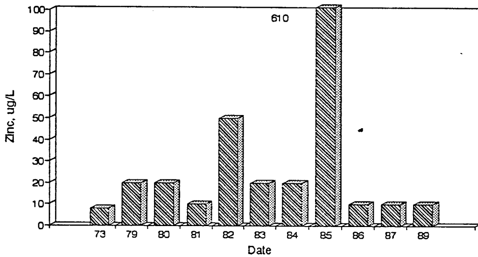
Figure A71. Graph of Zinc vs. Time for the White River Site-Aug.
