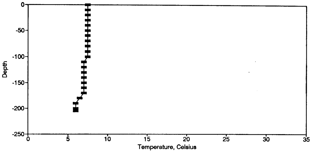
Figure BT132. Temperature Profile for the Eureka Springs Site-January 11, 1985.
