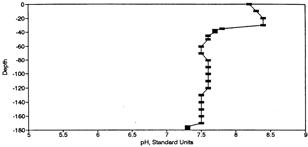
Figure BP46. pH Profile for the Eureka Springs Site-September 12, 1977.
