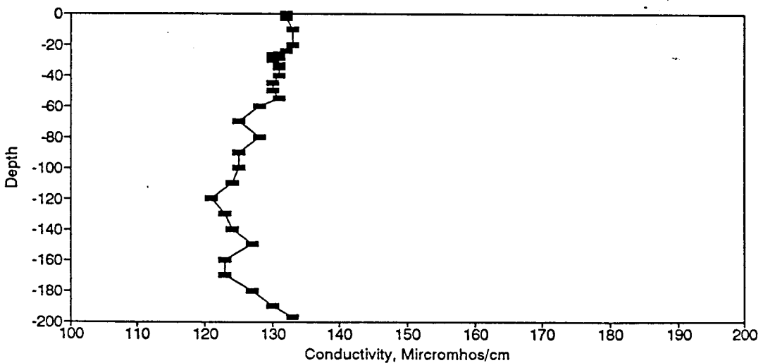
Figure BC150. Conductivity Profile for the Eureka Springs Site-July 9, 1986.
