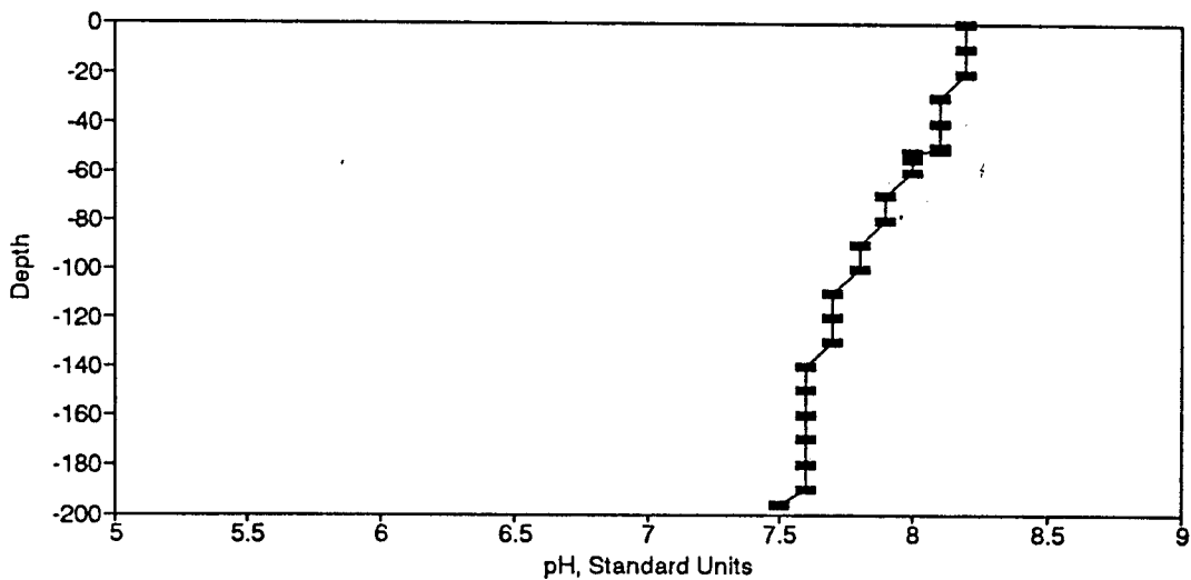
Figure BP65. pH Profile for the Eureka Springs Site-May 7, 1979.
