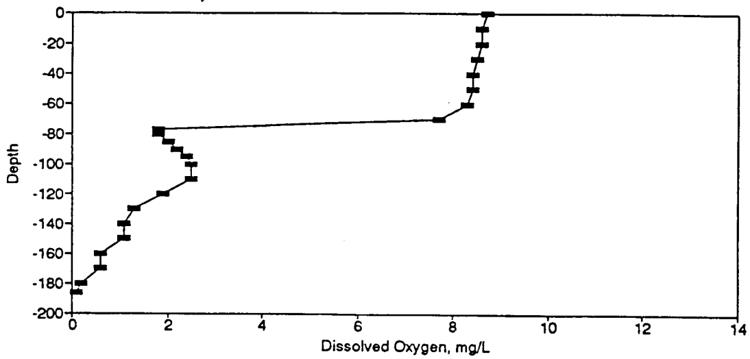
Figure BD94. Dissolved Oxygen Profile for the Eureka Springs Site-November 16, 1981.
