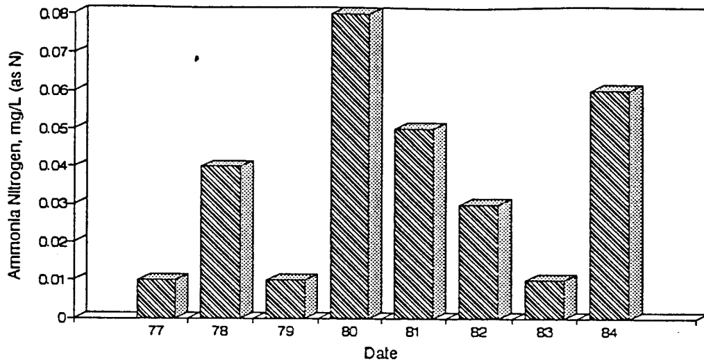
Figure A76. Graph of Ammonia Nitrogen vs. Time for the White River Site-May.
