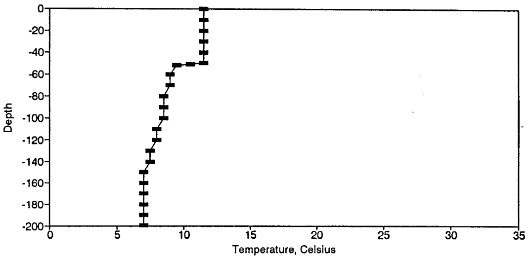
Figure BT159. Temperature Profile for the Eureka Springs Site-April 15, 1987.
