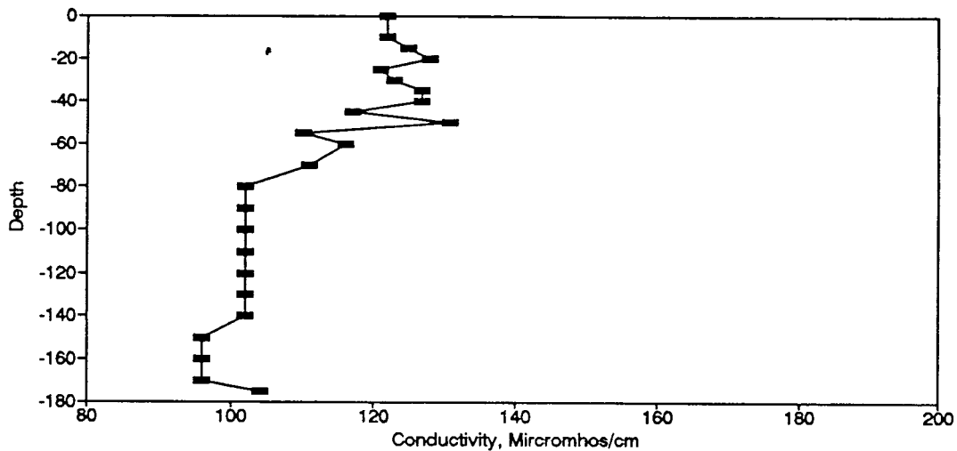
Figure BC22. Conductivity Profile for the Eureka Springs Site-October 14, 1975.
