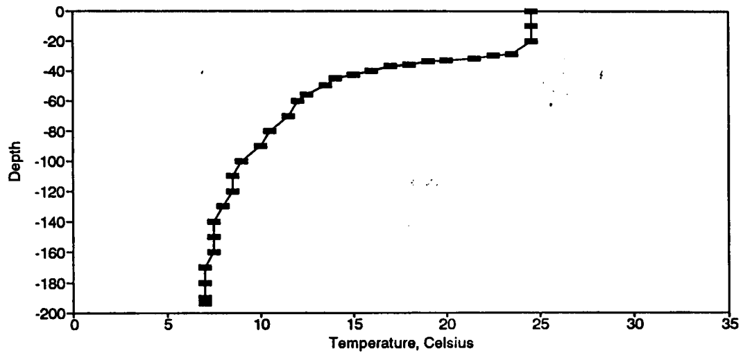
Figure BT176. Temperature Profile for the Eureka Springs Site-September 21, 1988.
