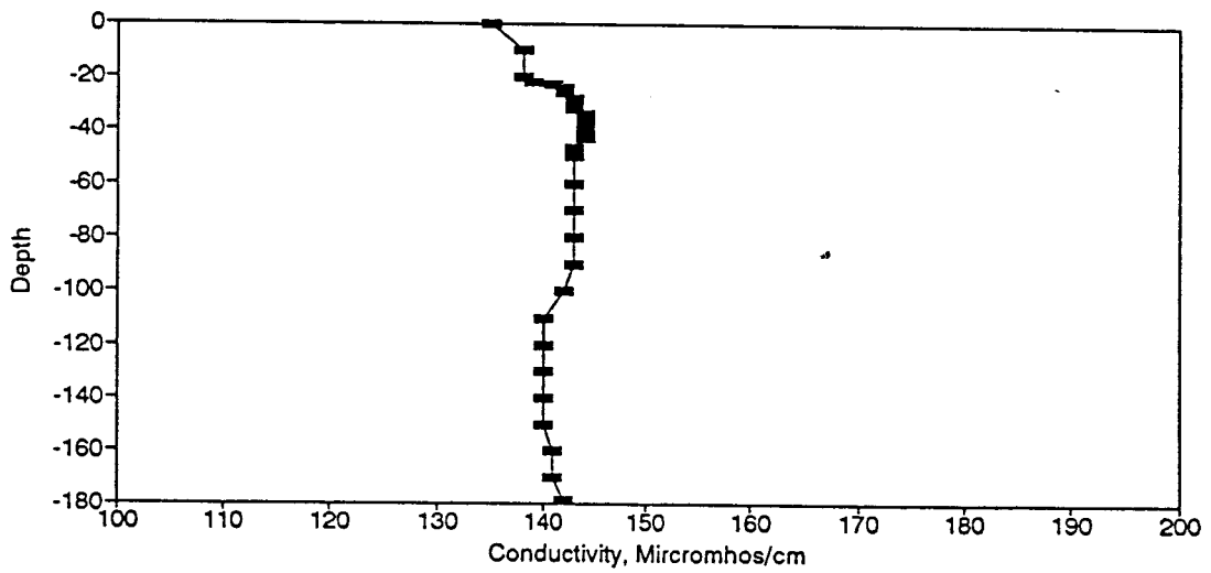
Figure BC125. Conductivity Profile for the Eureka Springs Site-June 26, 1984.
