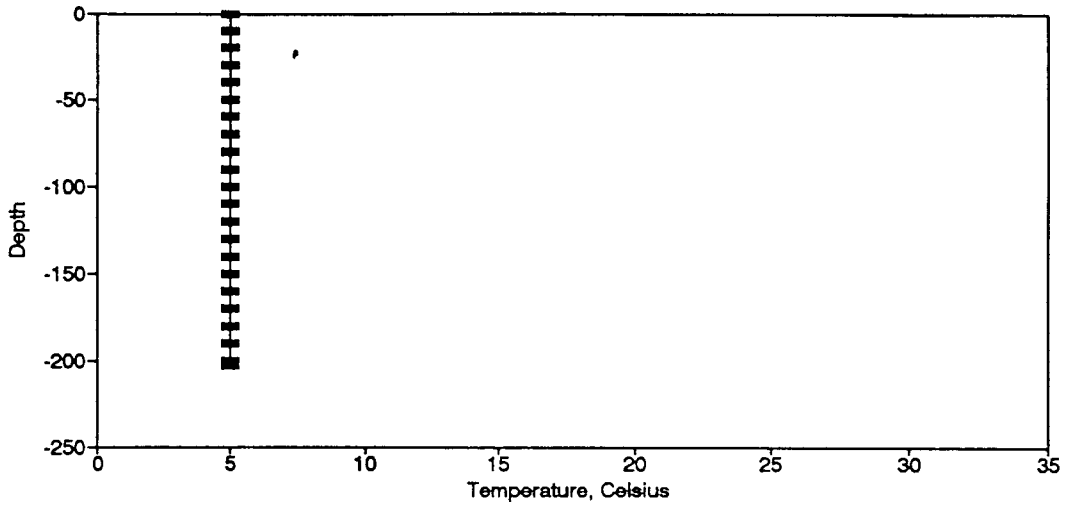
Figure BT133. Temperature Profile for the Eureka Springs Site-February 6, 1985.
