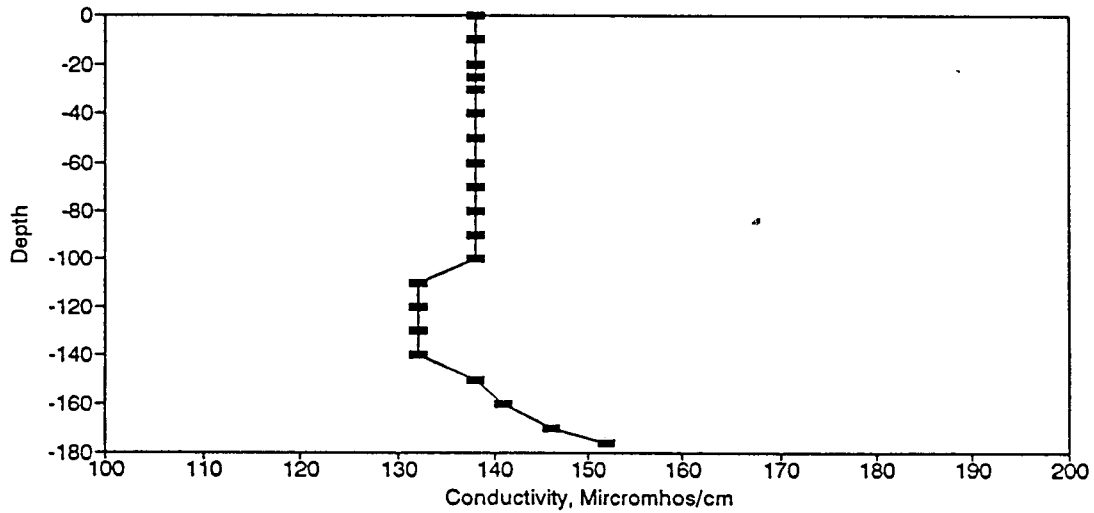
Figure BC119. Conductivity Profile for the Eureka Springs Site-December 7, 1983.
