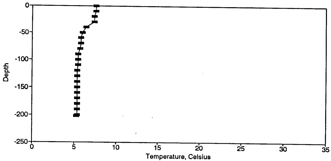
Figure BT181. Temperature Profile for the Eureka Springs Site-March 15, 1989.
