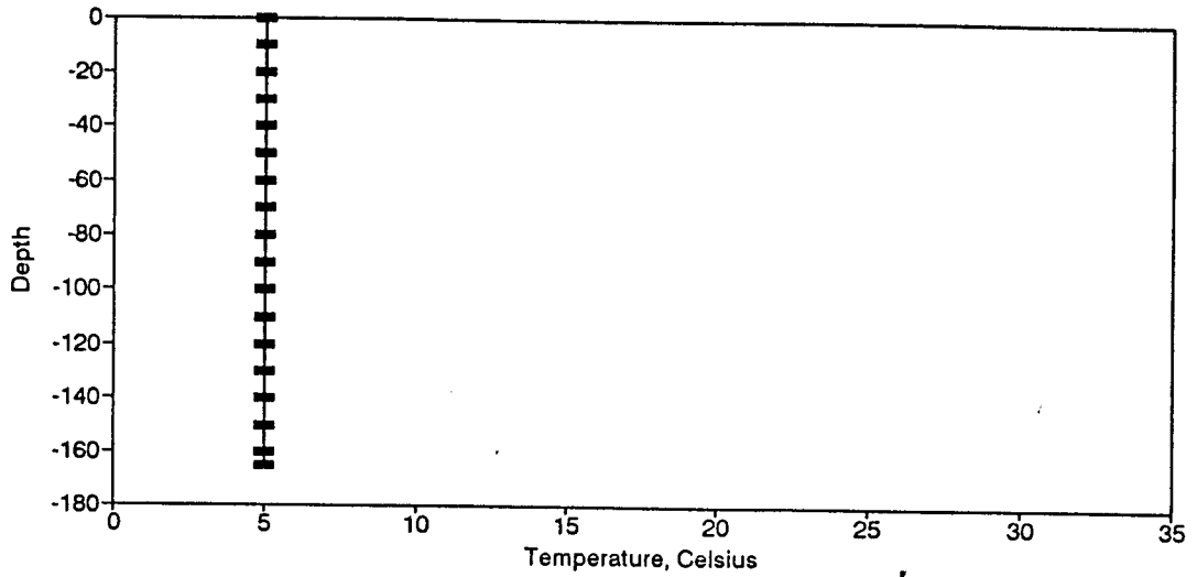
Figure BT121. Temperature Profile for the Eureka Springs Site-February 29, 1984.
