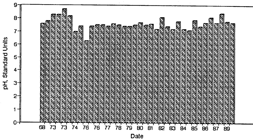
Figure A92. Graph of pH vs. Time for the White River Site-Aug.
