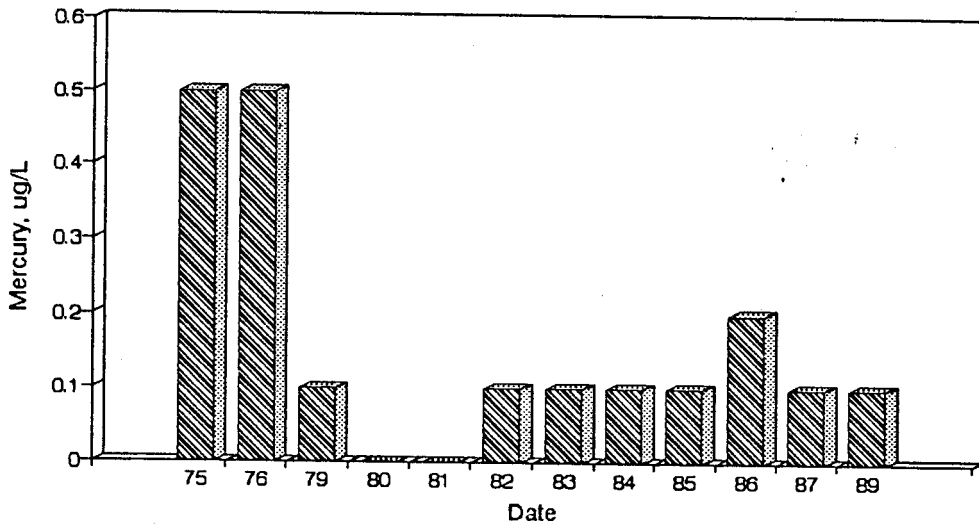
Figure A62. Graph of Mercury vs. Time for the White River Site-Aug.
