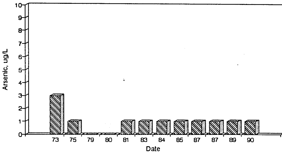
Figure A45. Graph of Arsenic vs. Time for the White River Site-Dec.
