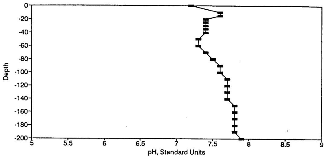
Figure BP52. pH Profile for the Eureka Springs Site-April 11, 1978.
