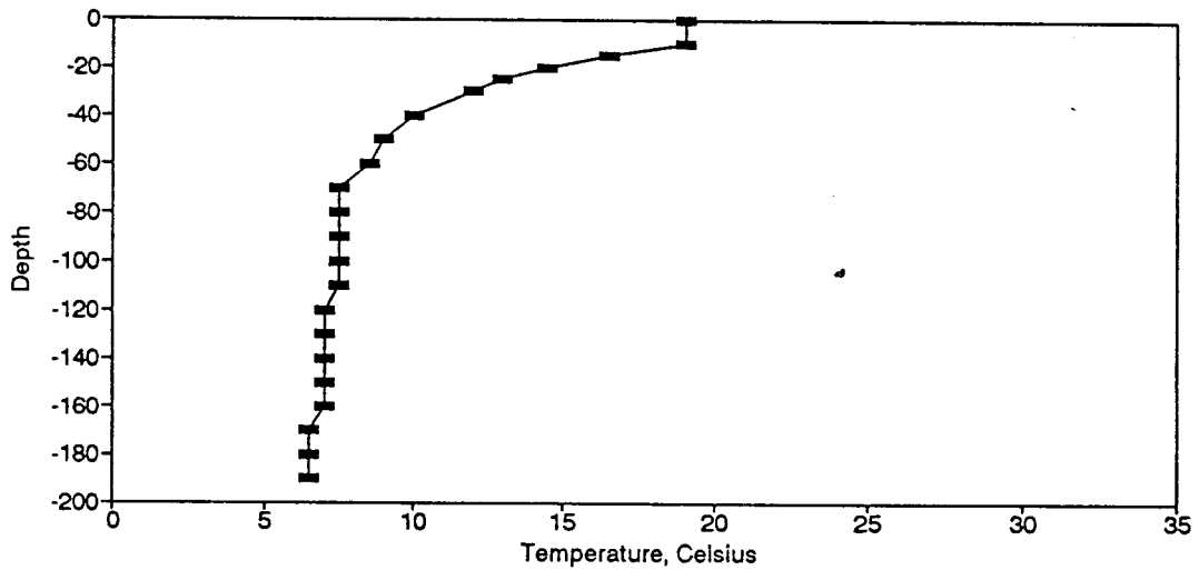
Figure BT17. Temperature Profile for the Eureka Springs Site-May 14, 1975.
