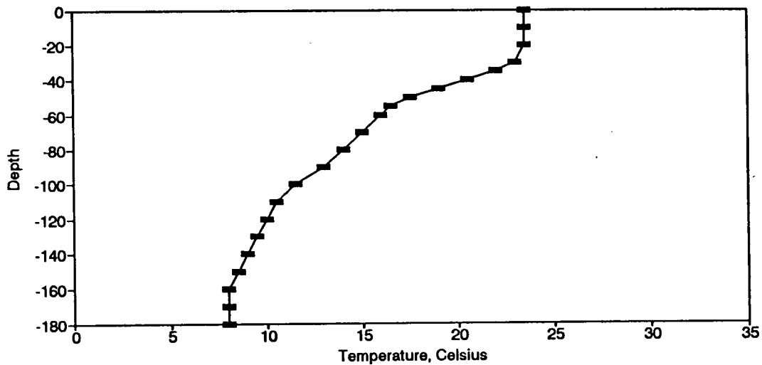
Figure BT33. Temperature Profile for the Eureka Springs Site-September 22, 1976.
