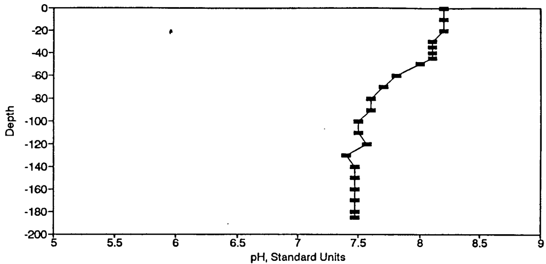
Figure BP28. pH Profile for the Eureka Springs Site-April 20, 1976.
