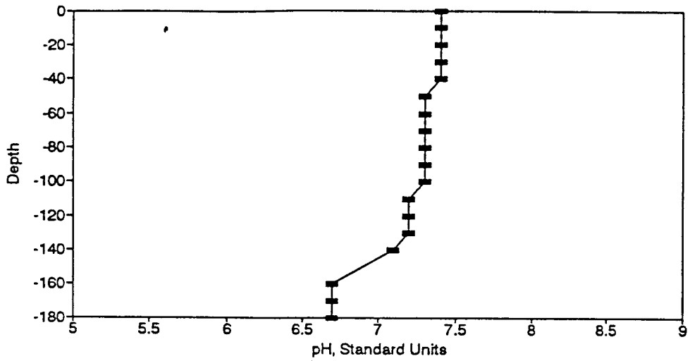
Figure BP73. pH Profile for the Eureka Springs Site-January 8, 1980
