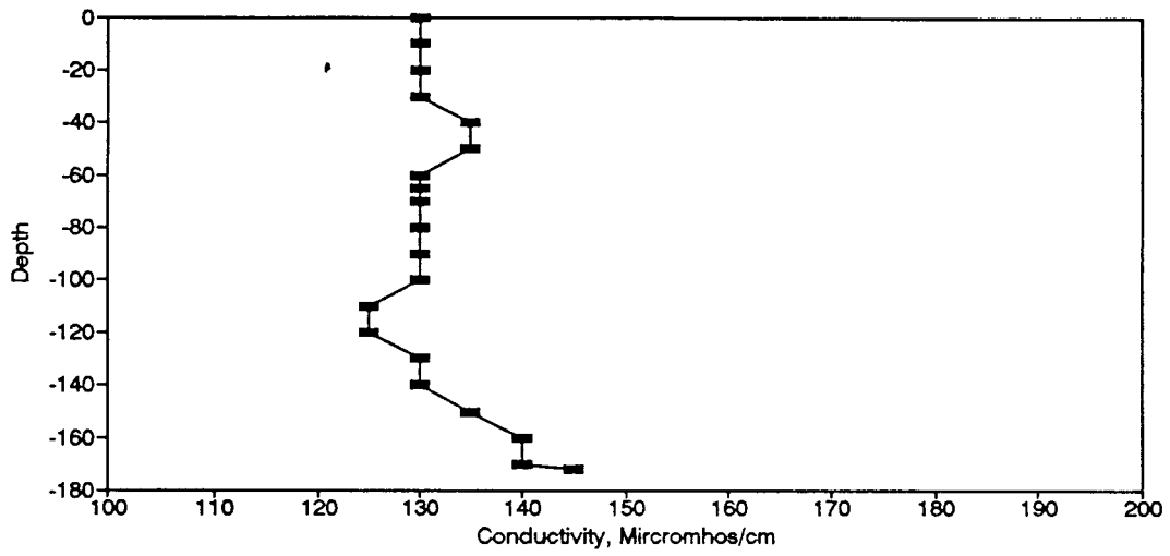
Figure BC34. Conductivity Profile for the Eureka Springs Site-October 18, 1976.
