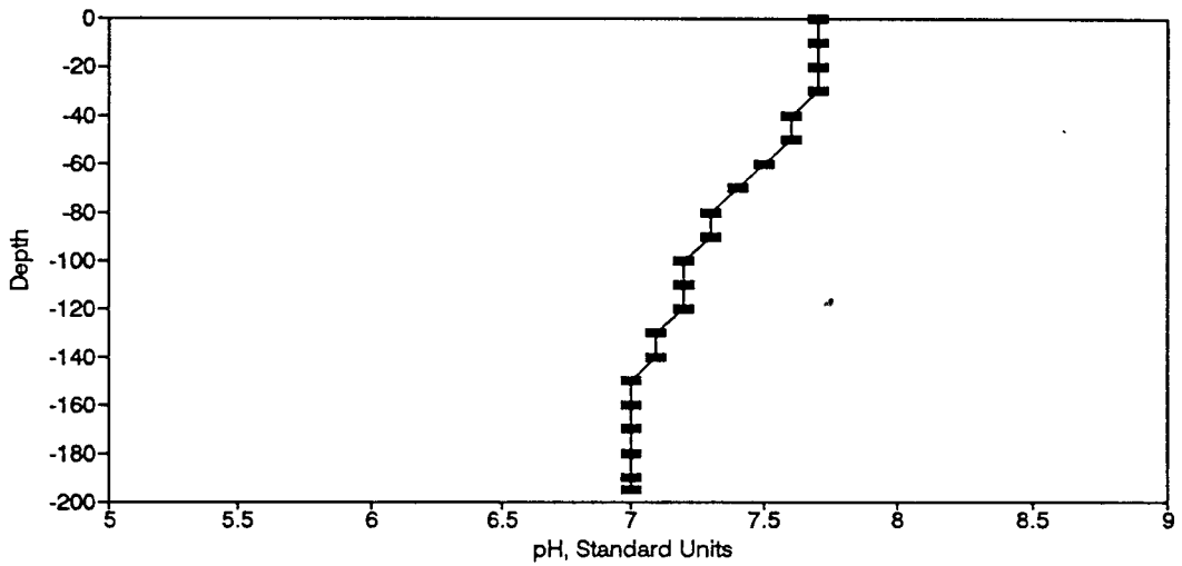
Figure BP5. pH Profile for the Eureka Springs Site-April 16, 1974.
