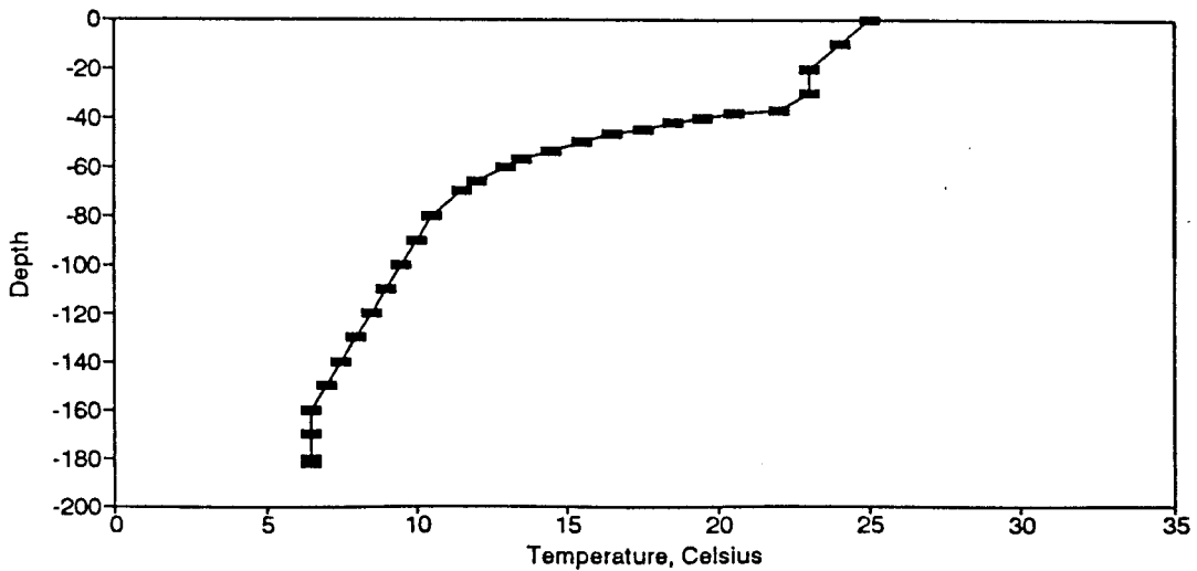
Figure BT69. Temperature Profile for the Eureka Springs Site-September 17, 1979.
