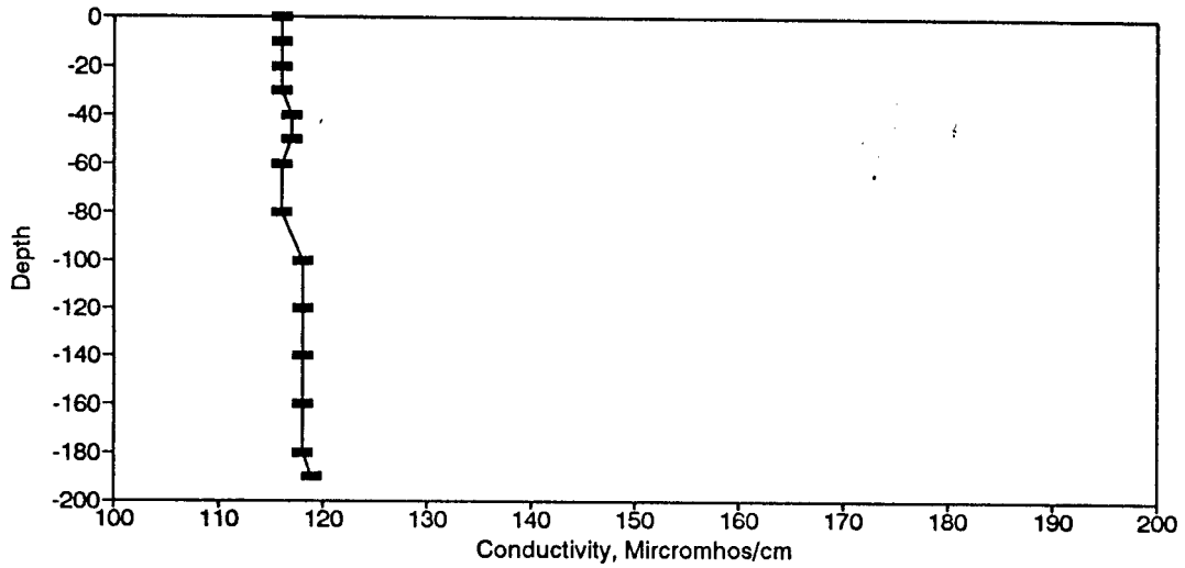
Figure BC26. Conductivity Profile for the Eureka Springs Site-February 24, 1976.
