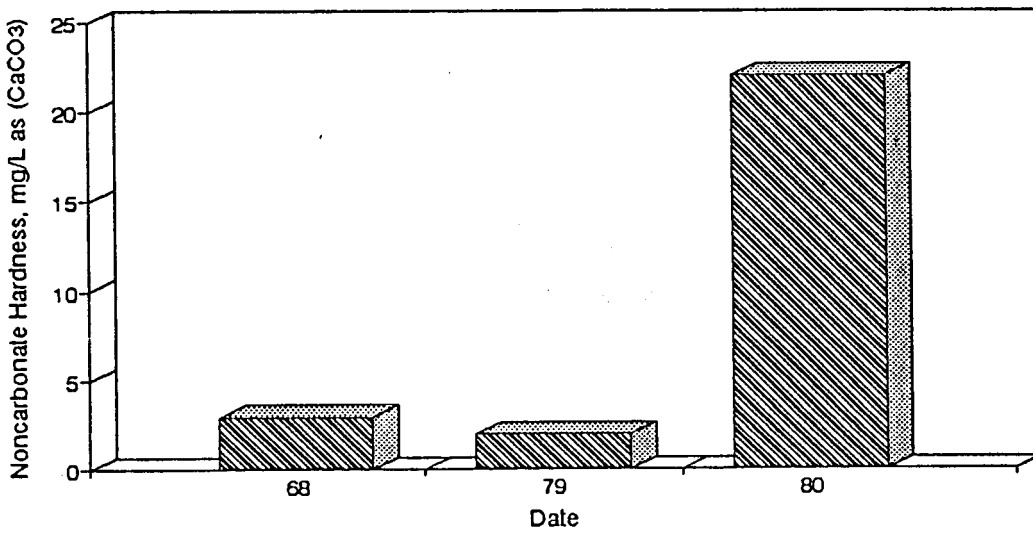
Figure A38. Graph of Noncarbonate Hardness vs. Time for the White River Site-Aug.
