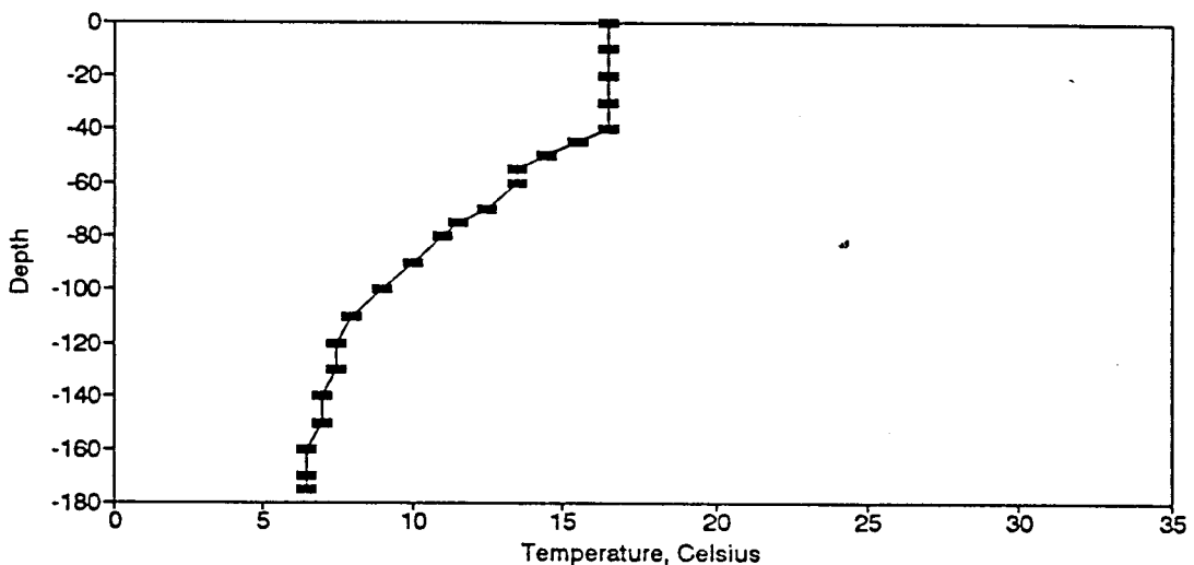
Figure BT59. Temperature Profile for the Eureka Springs Site-November 7, 1978.
