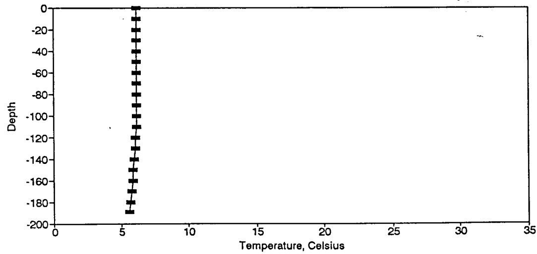
Figure BT180. Temperature Profile for the Eureka Springs Site-February 15, 1989.
