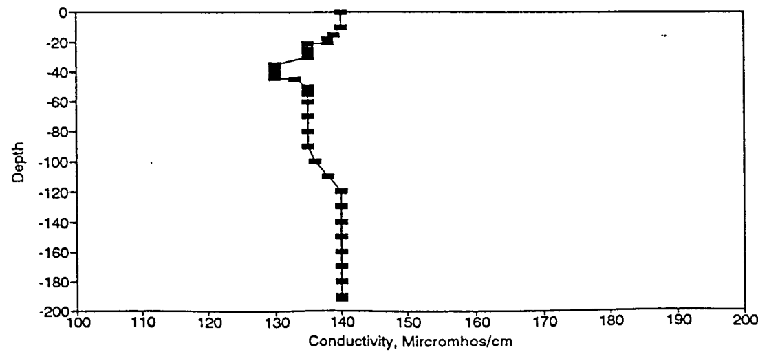
Figure BC66. Conductivity Profile for the Eureka Springs Site-June 6, 1979.
