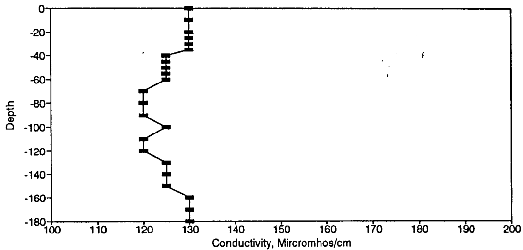
Figure BC32. Conductivity Profile for the Eureka Springs Site-August 24, 1976.
