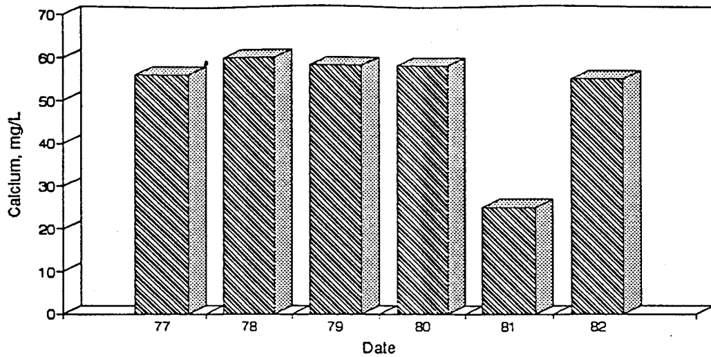
Figure A28. Graph of Calcium vs. Time for the White River Site-May.
