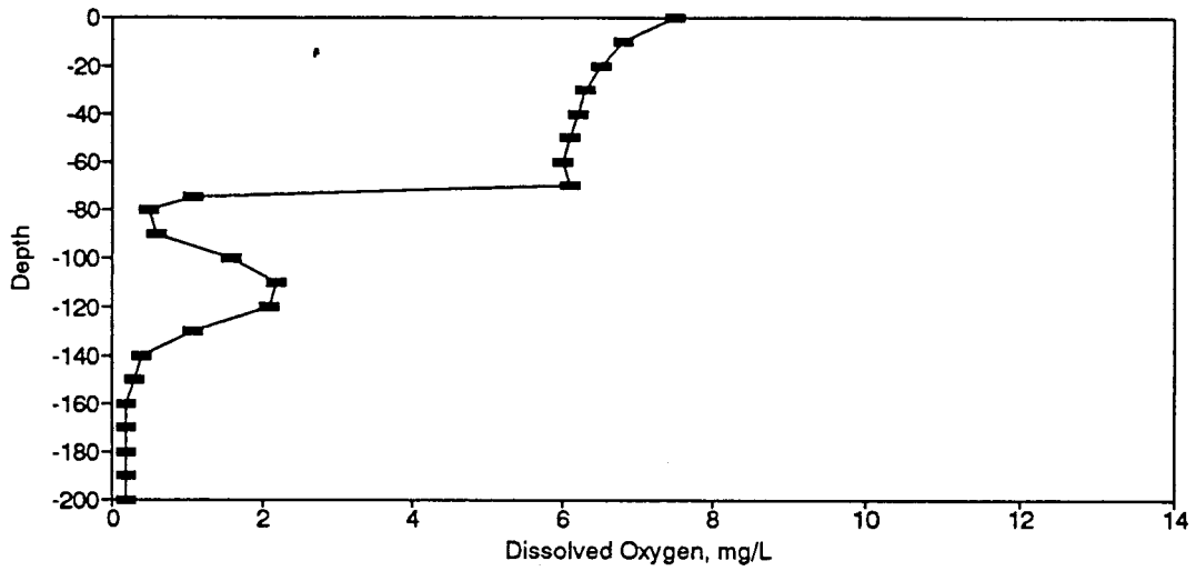
Figure BD10. Dissolved Oxygen Profile for the Eureka Springs Site-October 22, 1974.
