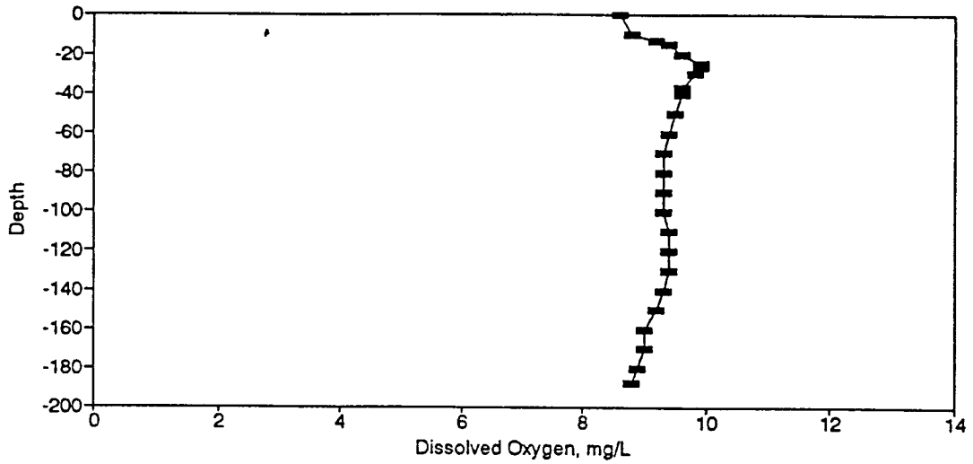
Figure BD124. Dissolved Oxygen Profile for the Eureka Springs Site-May 21, 1984.
