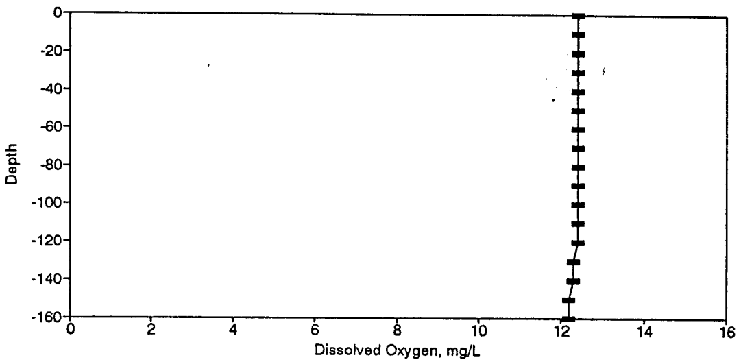
Figure BD38. Dissolved Oxygen Profile for the Eureka Springs Site-February 7, 1977.
