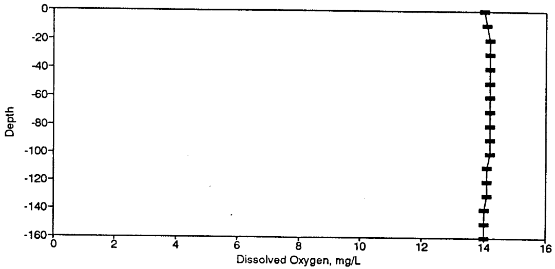
Figure BD37. Dissolved Oxygen Profile for the Eureka Springs Site-January 26, 1977.
