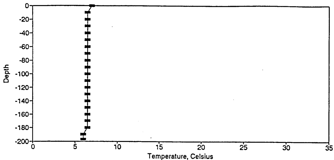
Figure BT109. Temperature Profile for the Eureka Springs Site, February 11, 1983.
