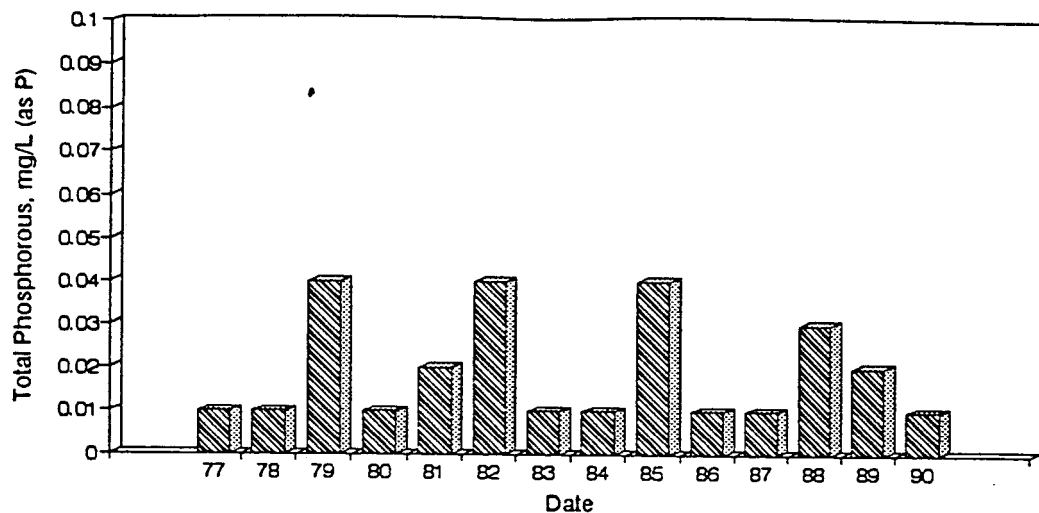
Figure A94. Graph of Total Phosphorous vs. Time for the White River Site-May.
