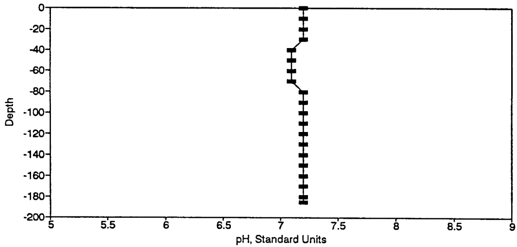
Figure BP25. pH Profile for the Eureka Springs Site-January 20, 1976.
