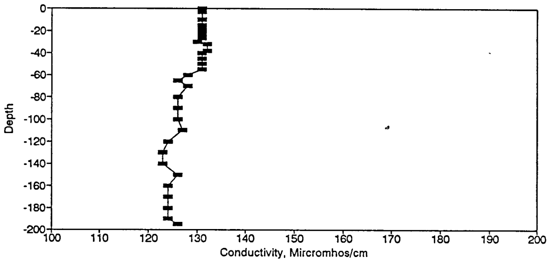
Figure BC149. Conductivity Profile for the Eureka Springs Site-June 4, 1986.
