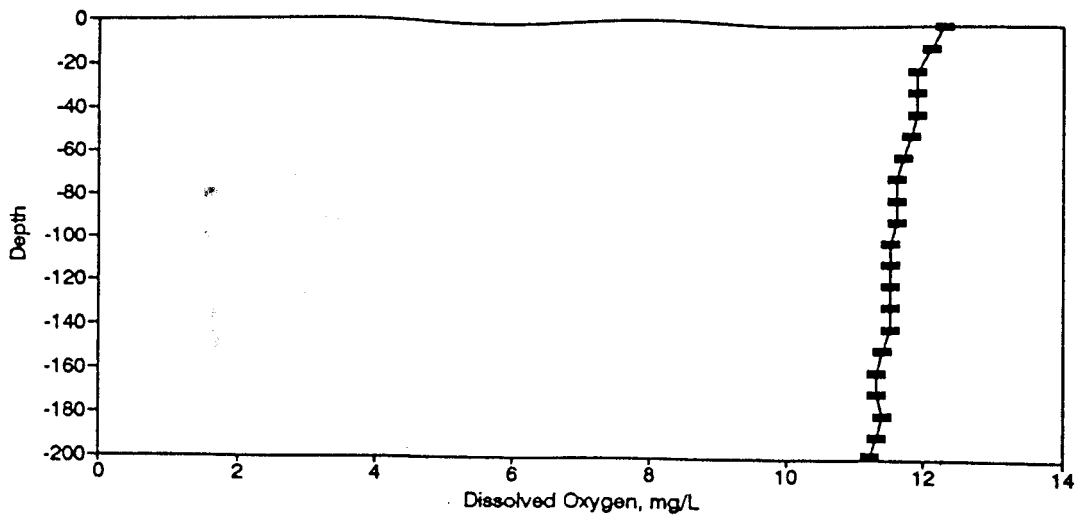
Figure BD169. Dissolved Oxygen Profile for the Eureka Springs Site-February 24, 1988.
