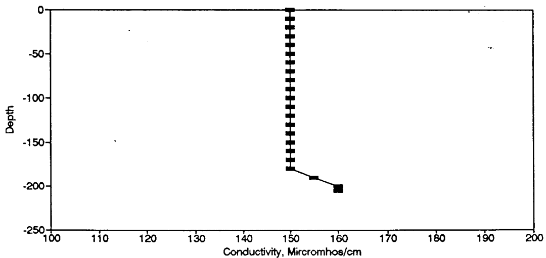
Figure BC132. Conductivity Profile for the Eureka Springs Site-January 11, 1985.
