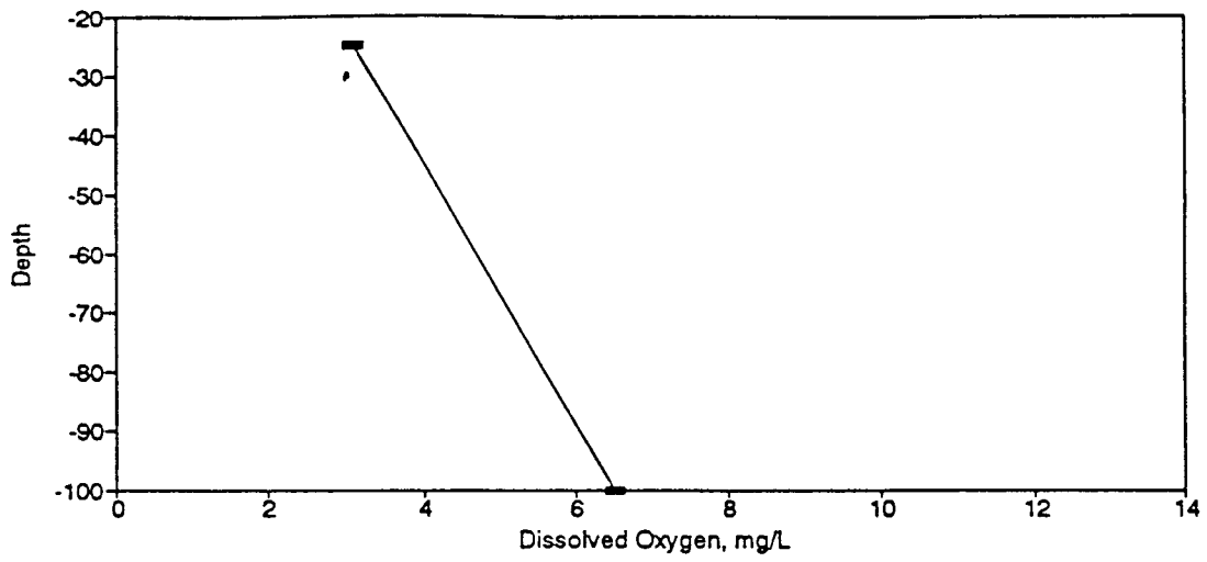
Figure BD190. Dissolved Oxygen Profile for the Eureka Springs Site-July 31, 1990.
