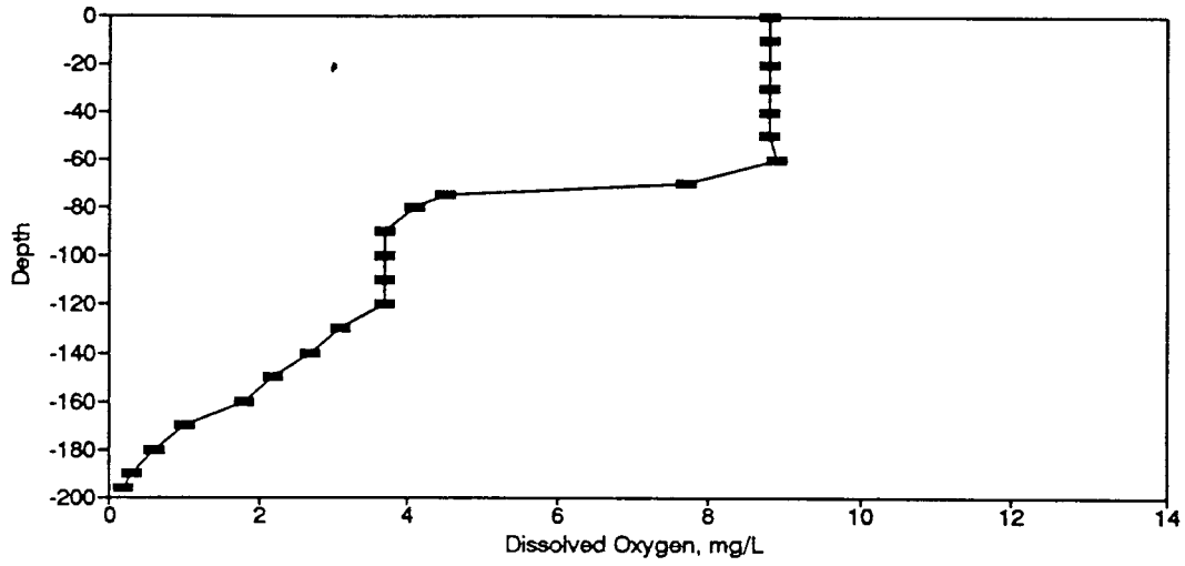
Figure BD130. Dissolved Oxygen Profile for the Eureka Springs Site-November 8, 1984.
