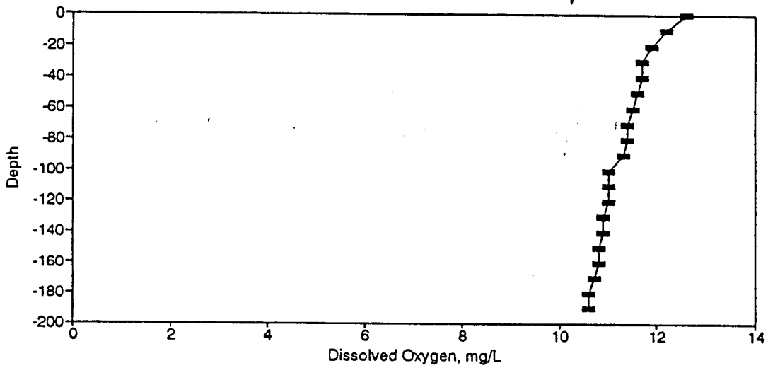
Figure BD170. Dissolved Oxygen Profile for the Eureka Springs Site-March 16, 1988.
