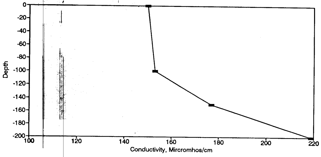
Figure BC1. Conductivity Profile for the Eureka Springs Site-December 18, 1973.
