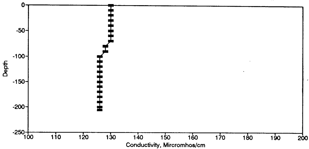
Figure BC135. Conductivity Profile for the Eureka Springs Site-April 3, 1985.
