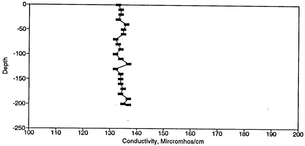
Figure BC181. Conductivity Profile for the Eureka Springs Site-March 15, 1989.
