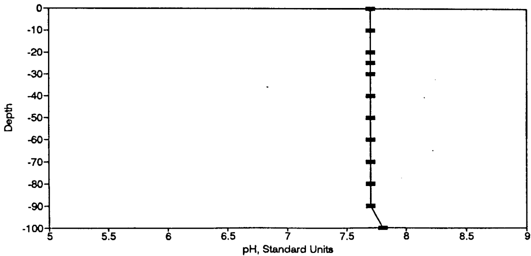
Figure BP72. pH Profile for the Eureka Springs Site-December 5, 1979.
