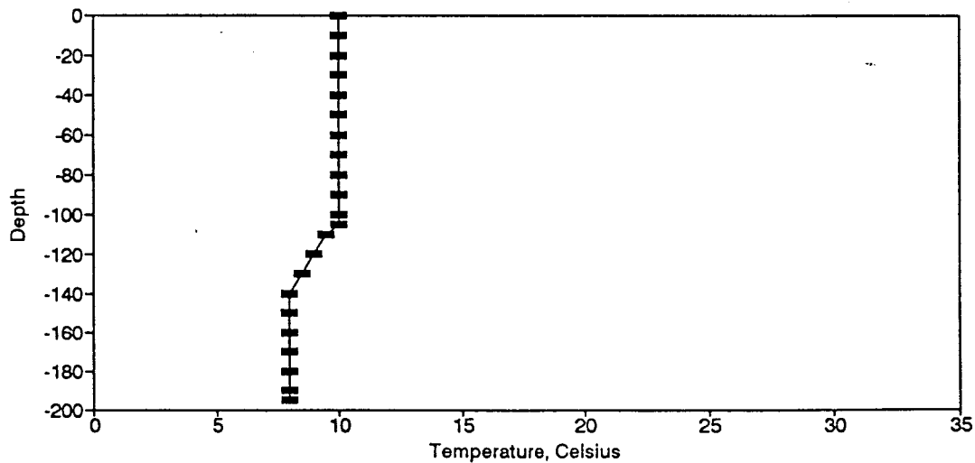
Figure BT24. Temperature Profile for the Eureka Springs Site-December 16, 1975.
