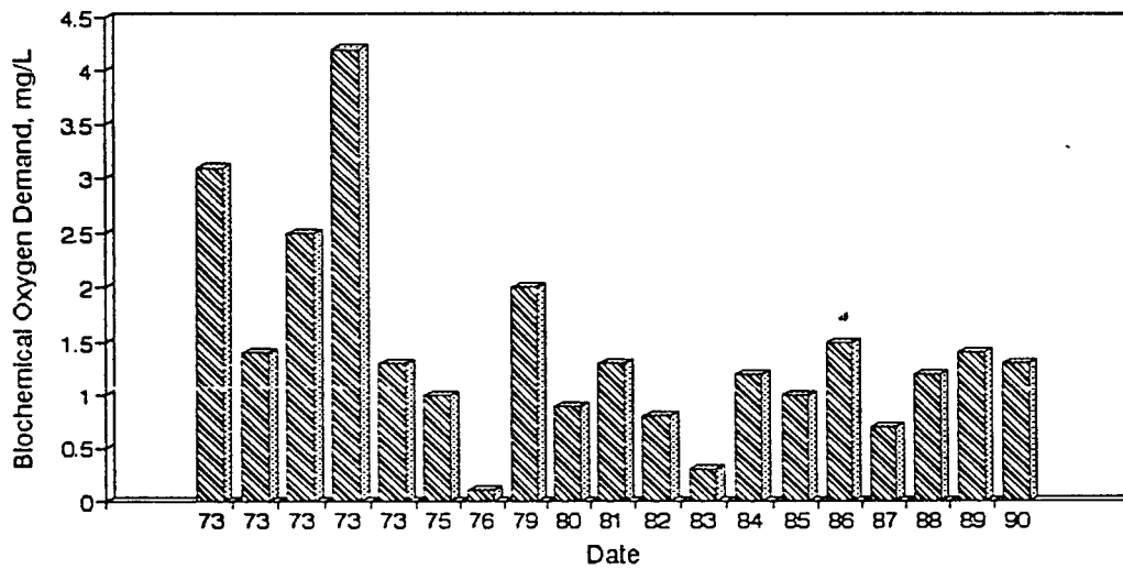
Figure A5. Graph of Biochemical Oxygen Demand vs. Time for the White River Site-Aug.
