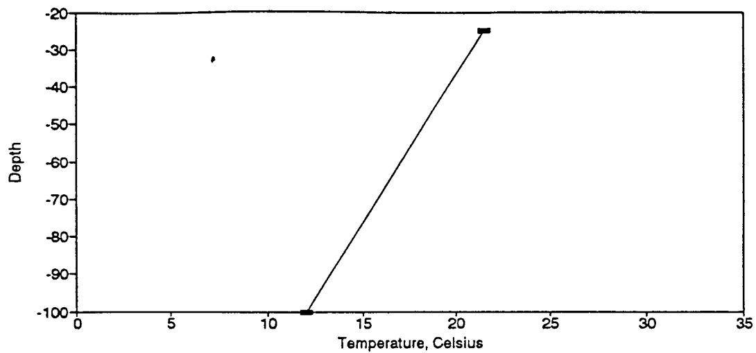
Figure BT190. Temperature Profile for the Eureka Springs Site-July 31, 1990.
