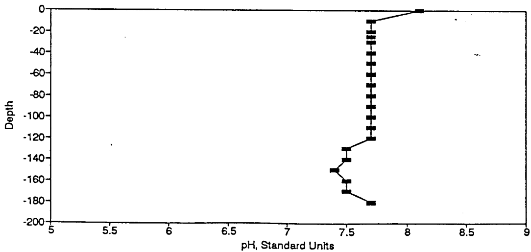
Figure BP63. pH Profile for the Eureka Springs Site-March 8, 1979.
