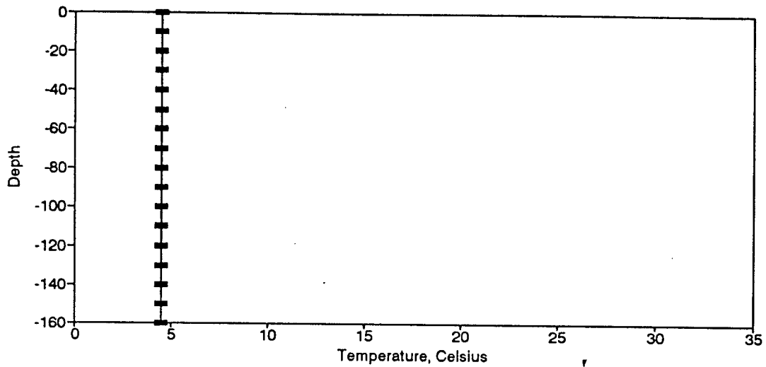
Figure BT37. Temperature Profile for the Eureka Springs Site-January 26, 1977.
