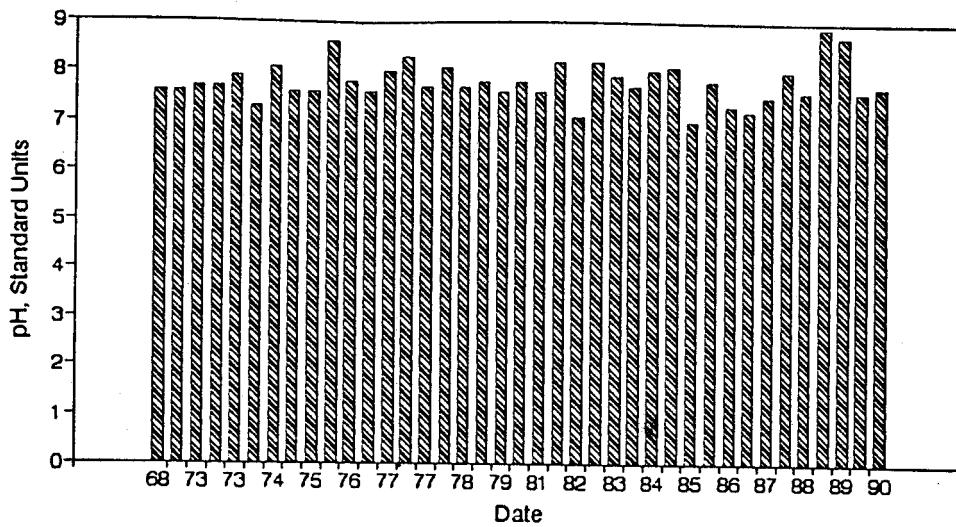
Figure A91. Graph of pH vs. Time for the White River Site-May.
