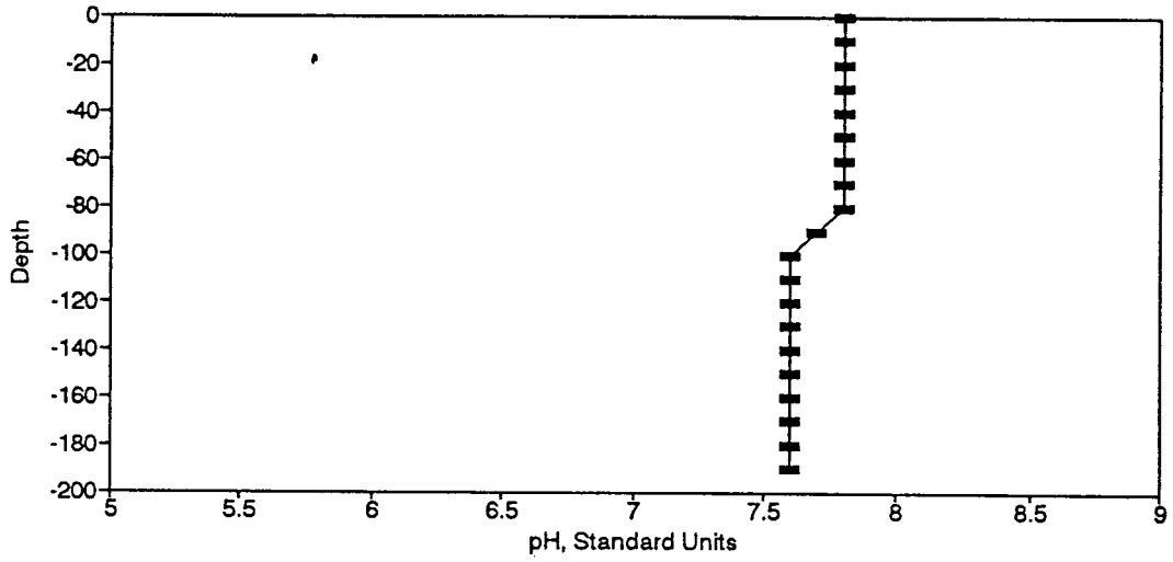
Figure BP13. pH Profile for the Eureka Springs Site-January 21, 1975.
