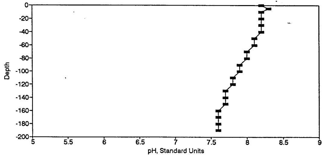
Figure BP27. pH Profile for the Eureka Springs Site-March 23, 1976.
