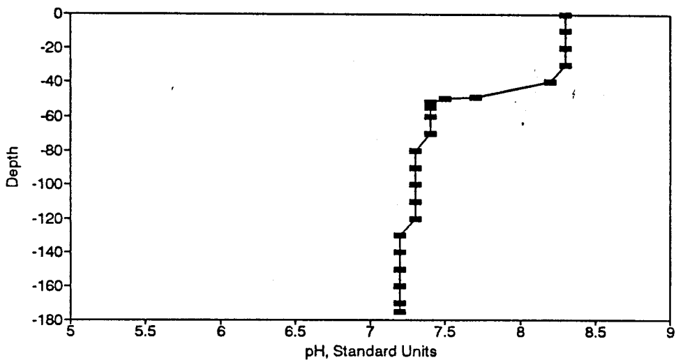
Figure BP83. pH Profile for the Eureka Springs Site-November 5, 1980.
