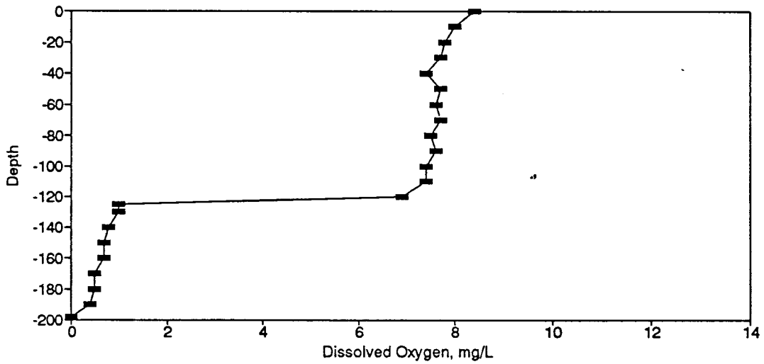
Figure BD11. Dissolved Oxygen Profile for the Eureka Springs Site-November 20, 1974.
