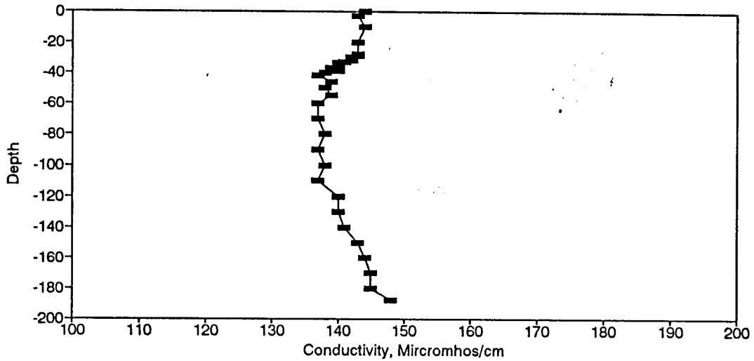
Figure BC164. Conductivity Profile for the Eureka Springs Site-September 3, 1987.
