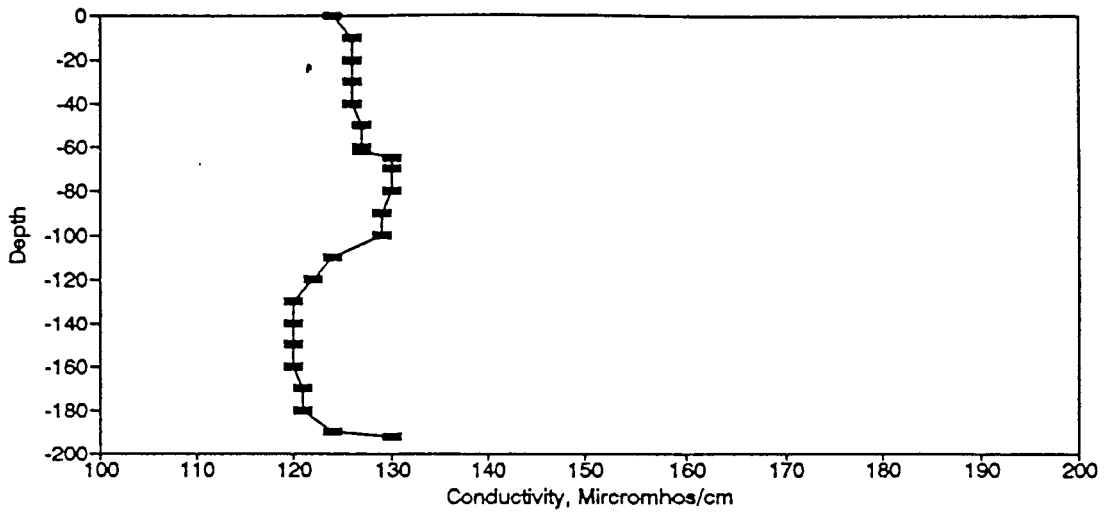
Figure BC142. Conductivity Profile for the Eureka Springs Site-November 6, 1985.
