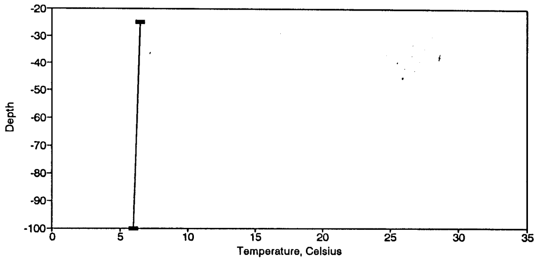
Figure BT188. Temperature Profile for the Eureka Springs Site-January 10, 1990.
