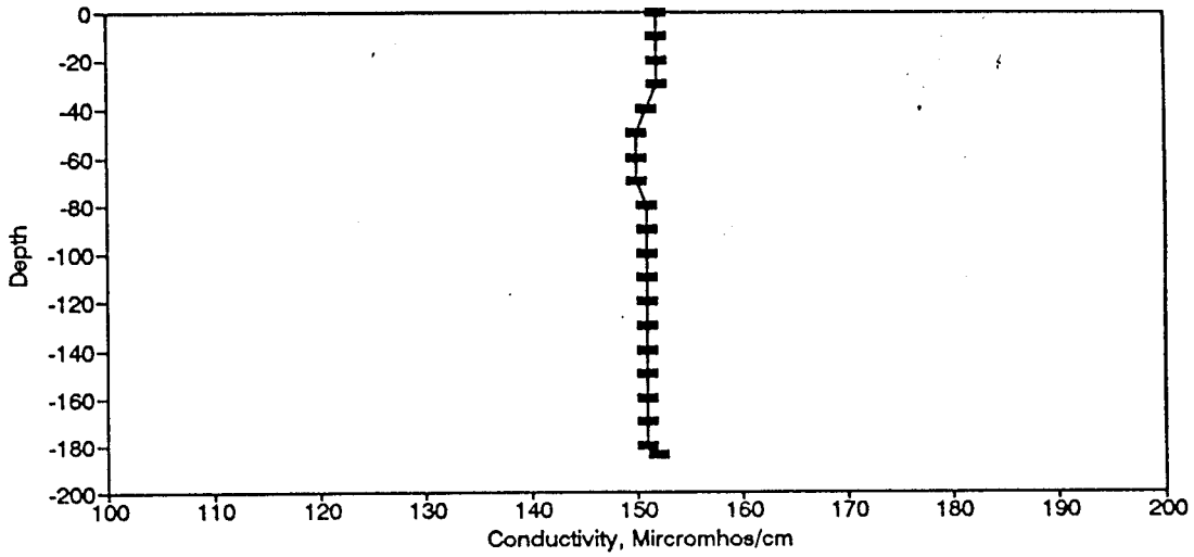
Figure BC98. Conductivity Profile for the Eureka Springs Site-March 23, 1982.
