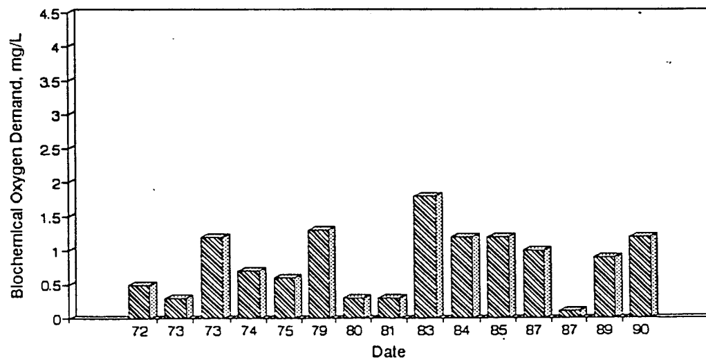
Figure A6. Graph of Biochemical Oxygen Demand vs. Time for the White River Site-Dec.
