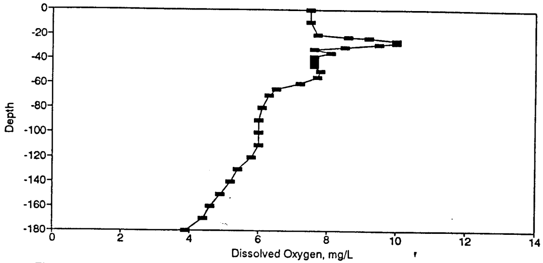
Figure BD103. Dissolved Oxygen Profile for the Eureka Springs Site-August 18, 1982.
