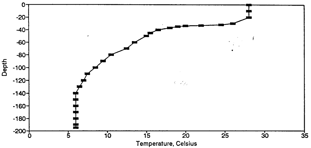
Figure BT56. Temperature Profile for the Eureka Springs Site - August 15, 1978.
