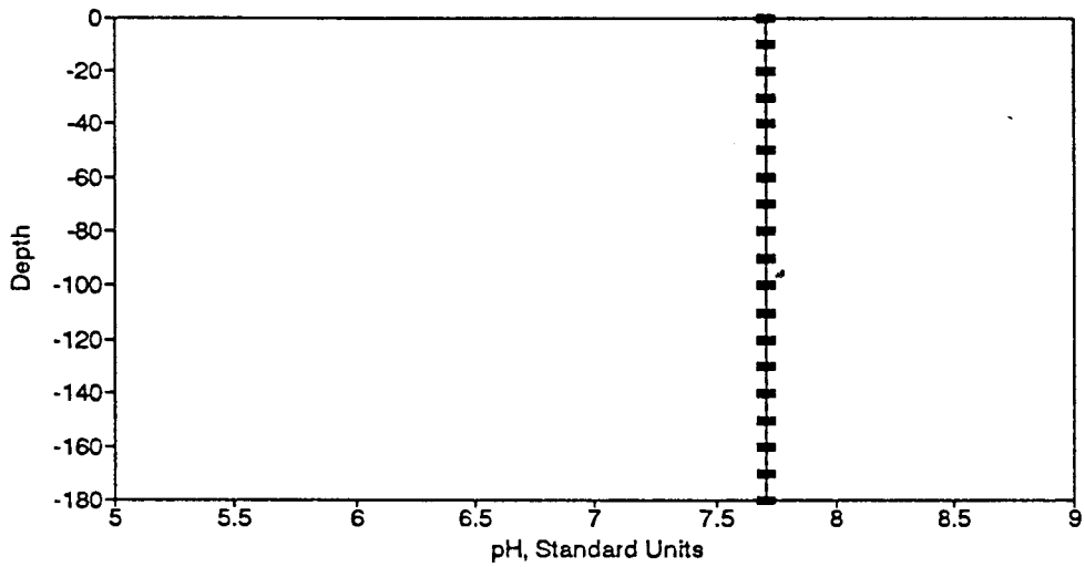
Figure BP74. pH Profile for the Eureka Springs Site-February 14, 1980.
