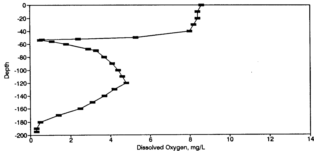
Figure BD141. Dissolved Oxygen Profile for the Eureka Springs Site-October 10, 1985.
