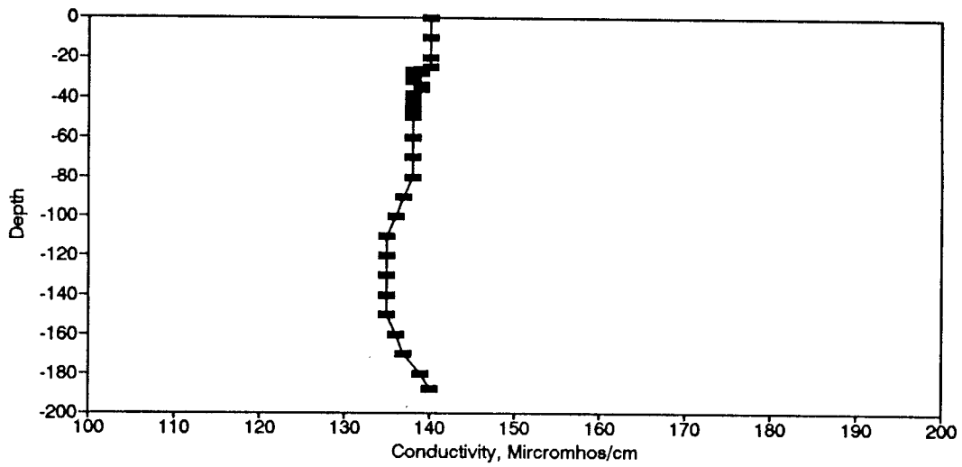
Figure BC127. Conductivity Profile for the Eureka Springs Site-August 14, 1984.
