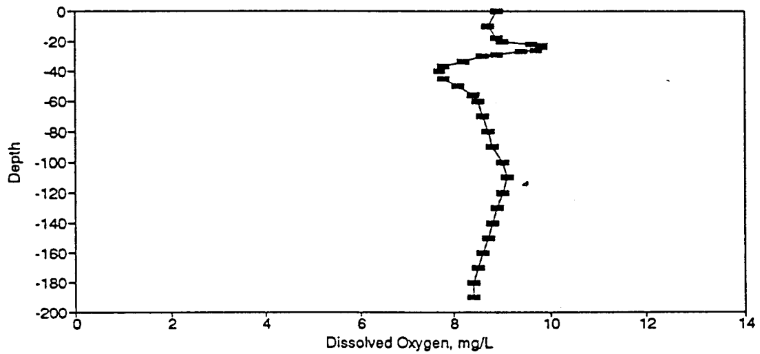
Figure BD173. Dissolved Oxygen Profile for the Eureka Springs Site-June 15, 1988.
