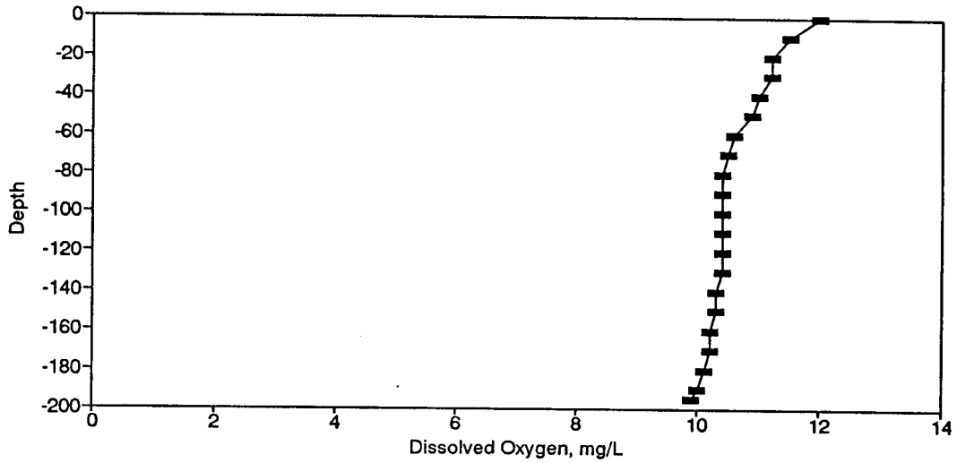
Figure BD145. Dissolved Oxygen Profile for the Eureka Springs Site-February 20, 1986.
