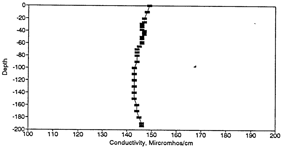
Figure BC89. Conductivity Profile for the Eureka Springs Site-June 16, 1981.
