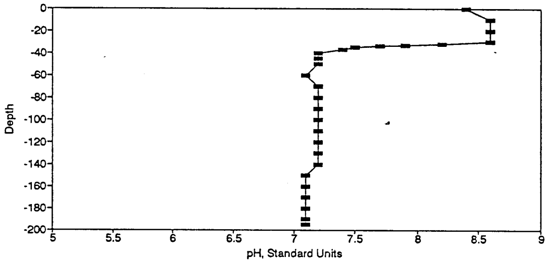
Figure BP56. pH Profile for the Eureka Springs Site-August 15, 1978.
