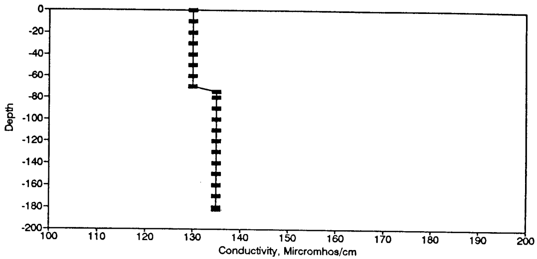
Figure BC49. Conductivity Profile for the Eureka Springs Site-December 7, 1977.
