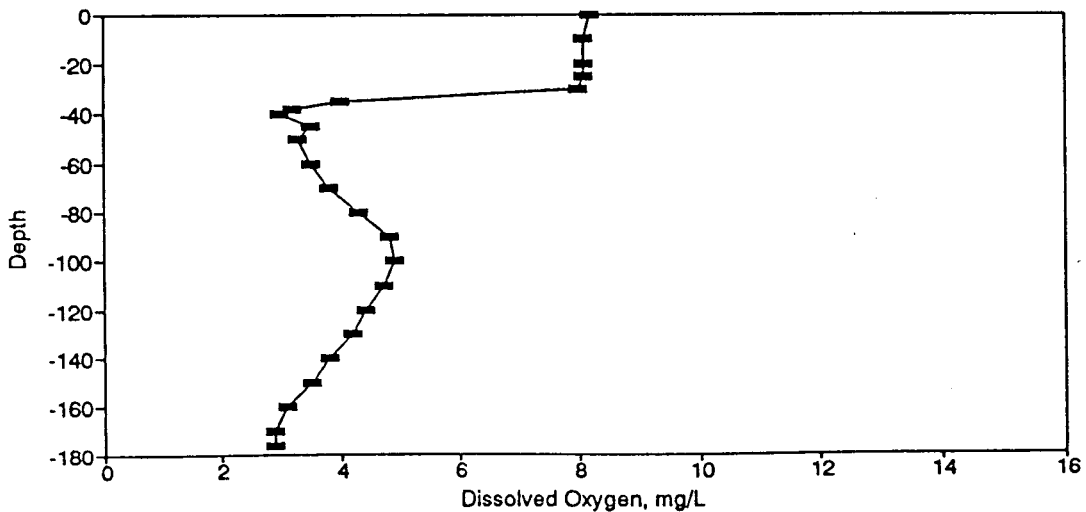
Figure BD57. Dissolved Oxygen Profile for the Eureka Springs Site-September 28, 1978.
