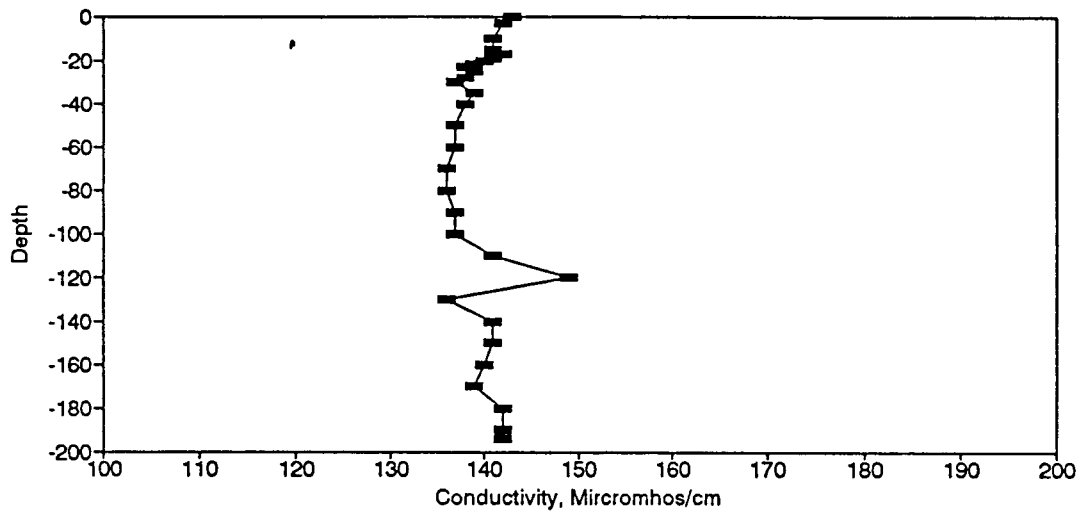
Figure BC160. Conductivity Profile for the Eureka Springs Site-May 13, 1987.
