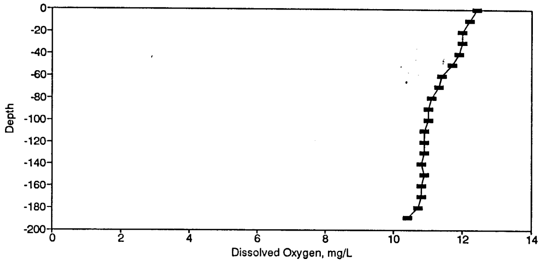
Figure BD146. Dissolved Oxygen Profile for the Eureka Springs Site-March 6, 1986.
