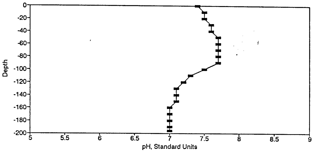
Figure BP107. pH Profile for the Eureka Springs Site-December 8, 1982.
