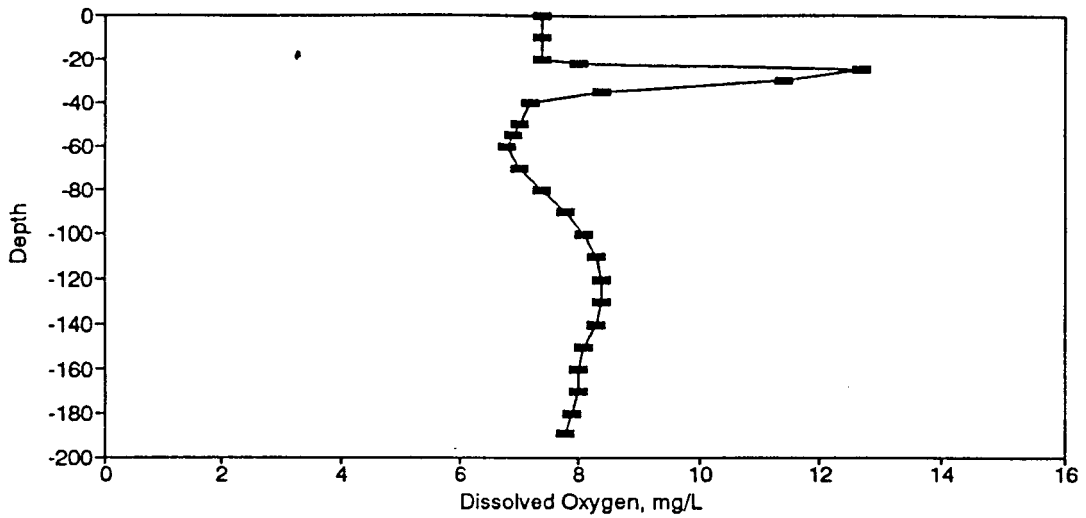
Figure BD55. Dissolved Oxygen Profile for the Eureka Springs Site-July 18, 1978.
