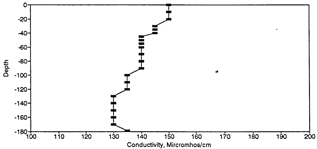
Figure BC47. Conductivity Profile for the Eureka Springs Site-October 12, 1977.
