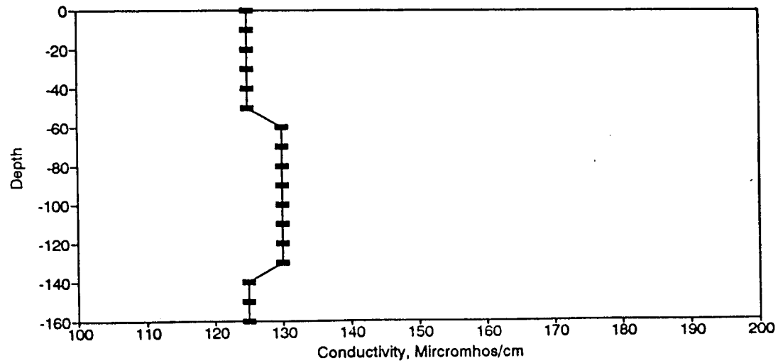
Figure BC39. Conductivity Profile for the Eureka Springs Site-March 8, 1977.
