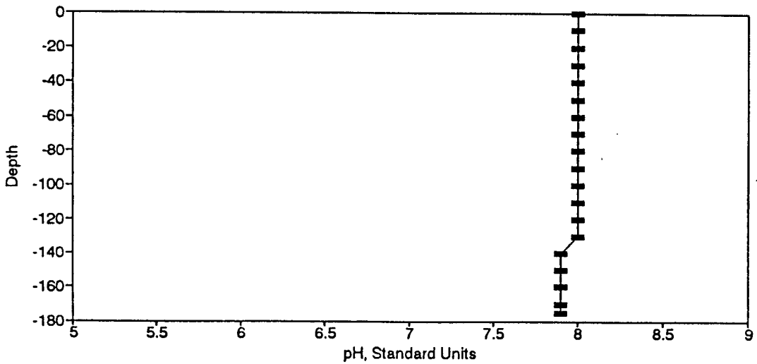
Figure BP96. pH Profile for the Eureka Springs Site-January 26, 1982.
