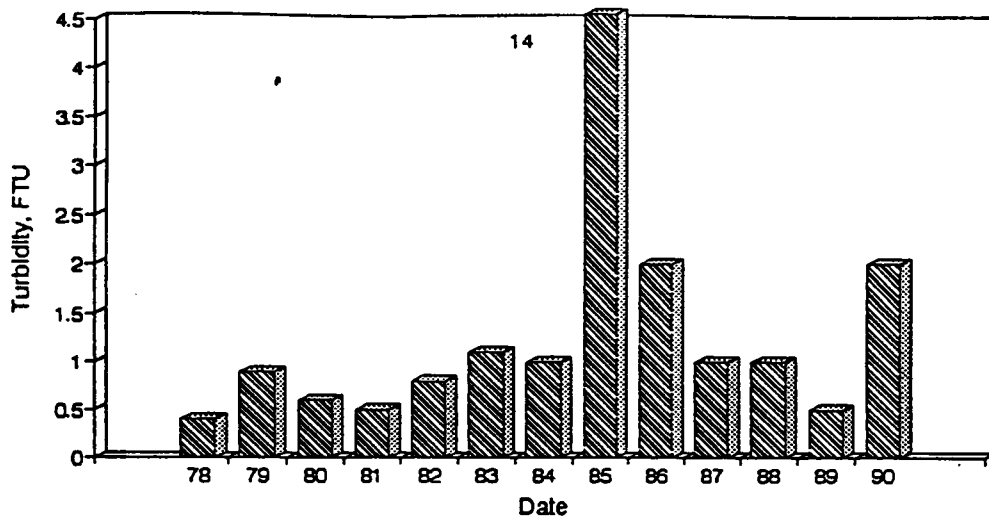
Figure A106. Graph of Turbidity vs. Time for the White River Site-May.
