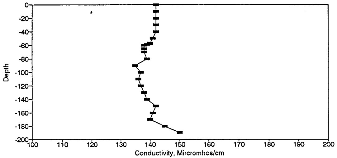
Figure BC166. Conductivity Profile for the Eureka Springs Site-November 12, 1987.
