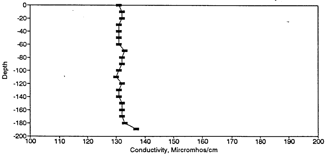
Figure BC180. Conductivity Profile for the Eureka Springs Site-February 15, 1989.
