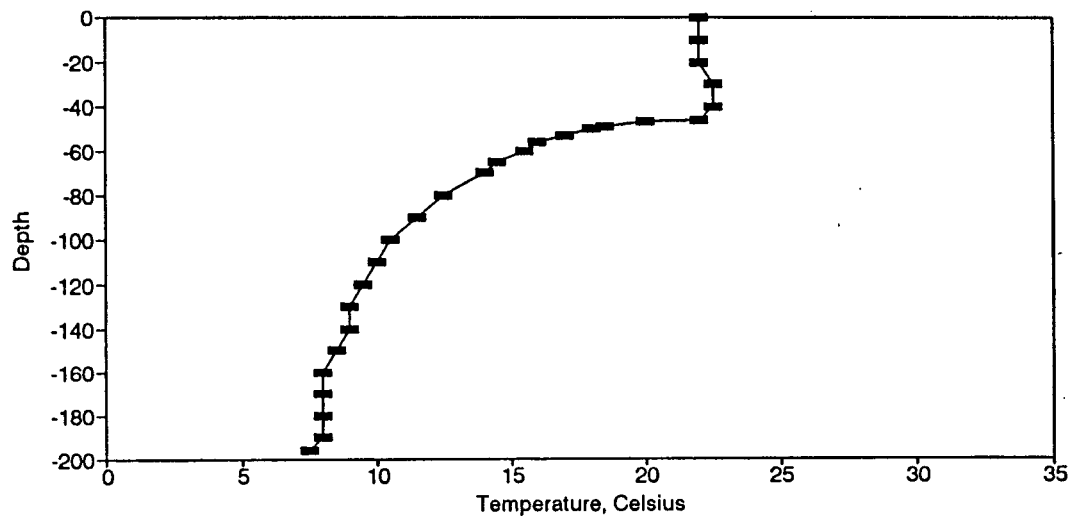
Figure BT153. Temperature Profile for the Eureka Springs Site-October 9, 1986.
