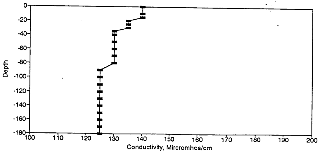
Figure BC42. Conductivity Profile for the Eureka Springs Site-May 31, 1977.
