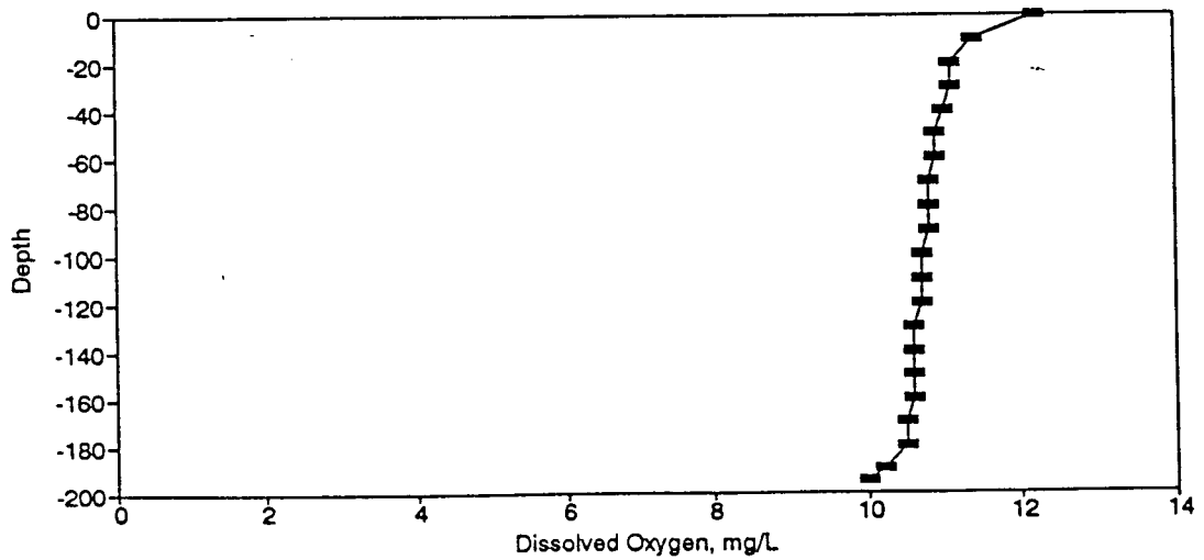
Figure BD168. Dissolved Oxygen Profile for the Eureka Springs Site-January 20, 1988.
