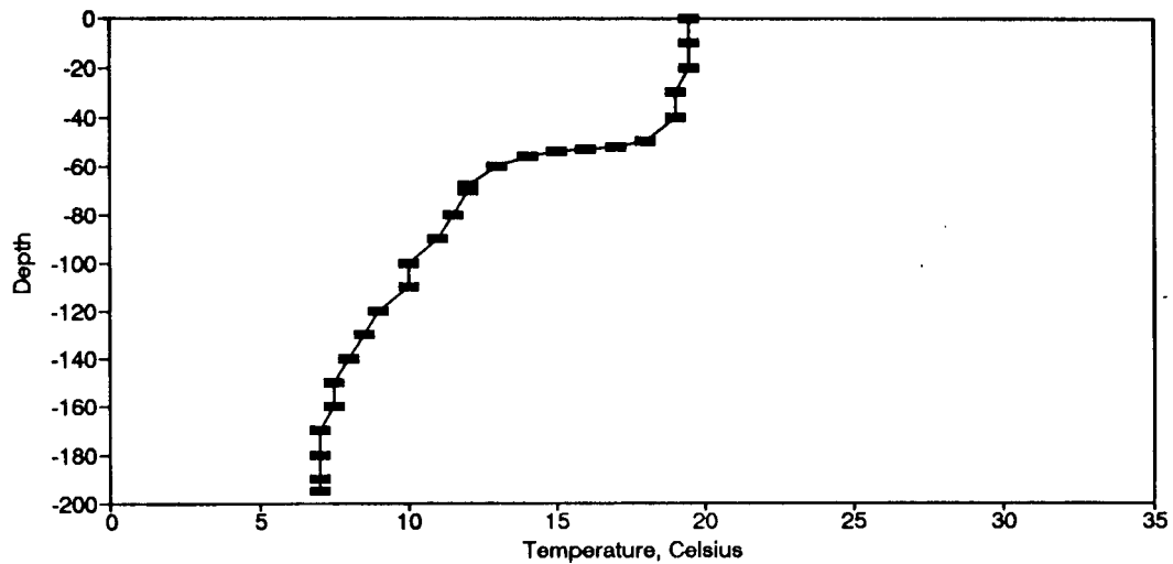
Figure BT141. Temperature Profile for the Eureka Springs Site-October 10, 1985.
