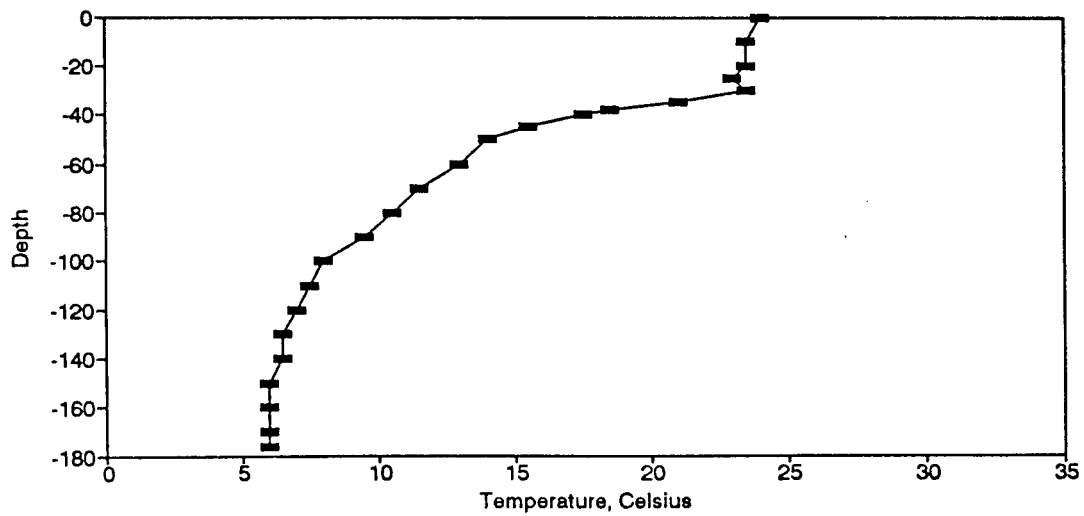
Figure BT57. Temperature Profile for the Eureka Springs Site - September 28, 1978.
