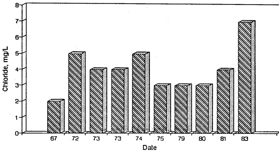
Figure A9. Graph of Chloride vs. Time for the White River Site-Dec.
