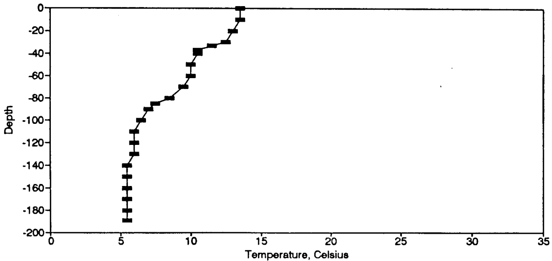
Figure BT99. Temperature Profile for the Eureka Springs Site-April 20, 1982.
