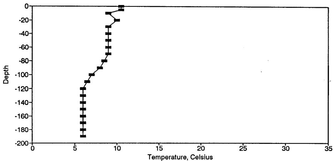
Figure BT27. Temperature Profile for the Eureka Springs Site-March 23, 1976.
