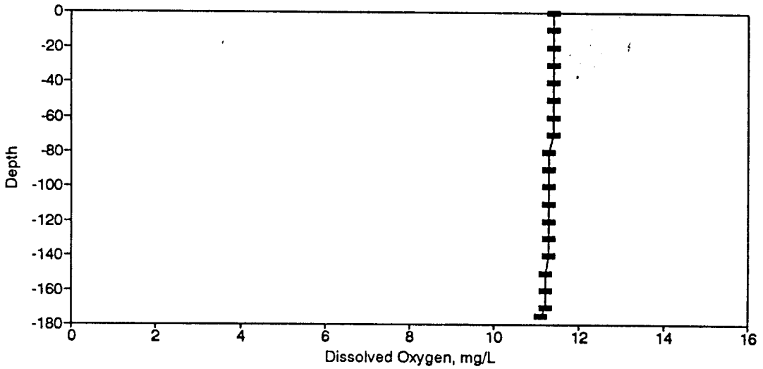
Figure BD62. Dissolved Oxygen Profile for the Eureka Springs Site-February 14, 1979.
