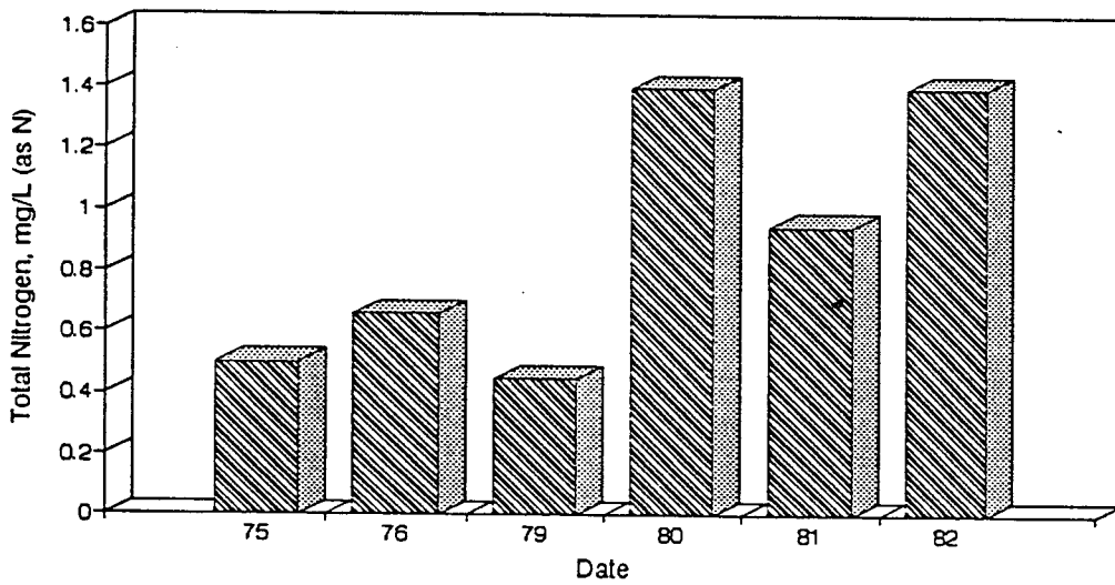
Figure A89. Graph of Total Nitrogen vs. Time for the White River Site-Aug.
