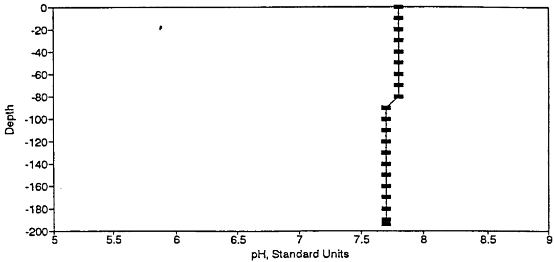
Figure BP97. pH Profile for the Eureka Springs Site-February 16, 1982.
