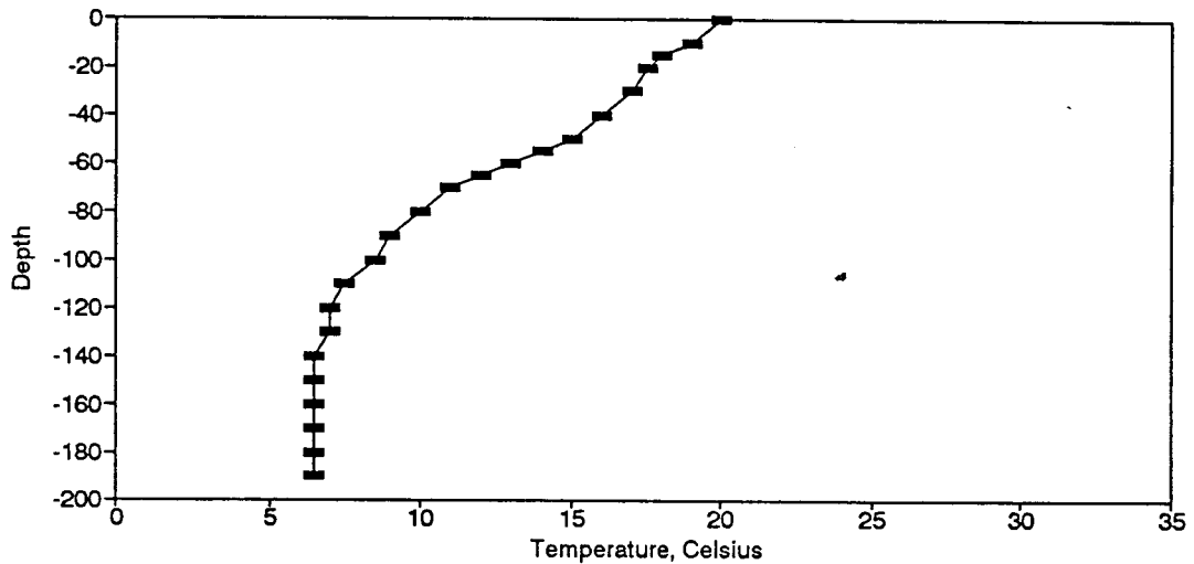
Figure BT29. Temperature Profile for the Eureka Springs Site-May 25, 1976.
