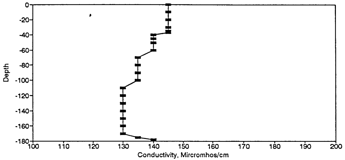
Figure BC46. Conductivity Profile for the Eureka Springs Site-September 12, 1977.
