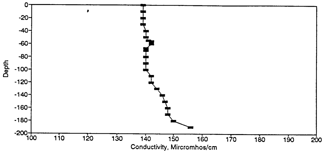
Figure BC70. Conductivity Profile for the Eureka Springs Site-October 16, 1979.
