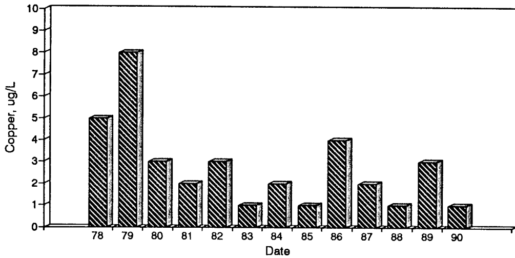
Figure A49. Graph of Copper vs. time for the White River Site-May,
