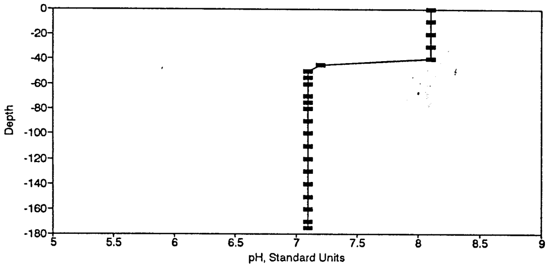
Figure BP59. pH Profile for the Eureka Springs Site-November 7, 1978.
