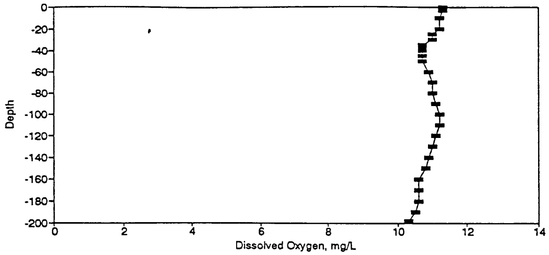
Figure BD172. Dissolved Oxygen Profile for the Eureka Springs Site-May 10, 1988.
