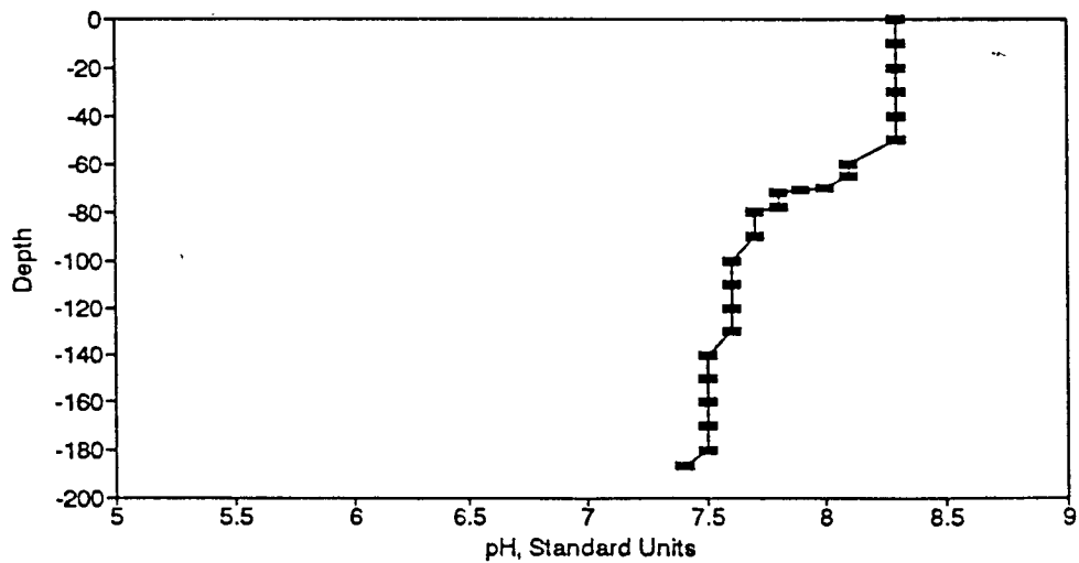
Figure BP87. pH Profile for the Eureka Springs Site-April 13, 1981.
