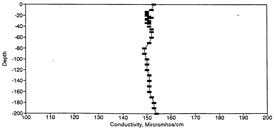
Figure BC114. Conductivity Profile for the Eureka Springs Site-July 12, 1983.
