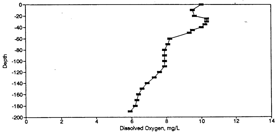
Figure BD30. Dissolved Oxygen Profile for the Eureka Springs Site-June 23, 1976.
