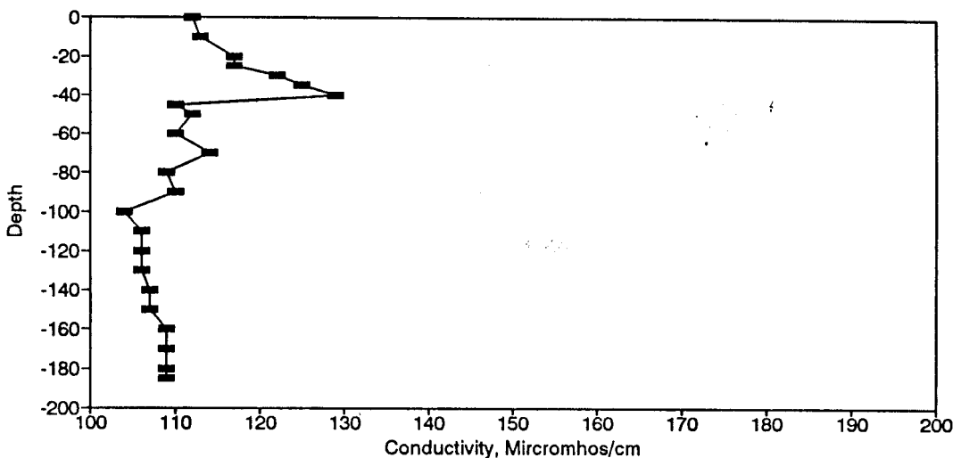
Figure BC20. Conductivity Profile for the Eureka Springs Site-August 13, 1975.
