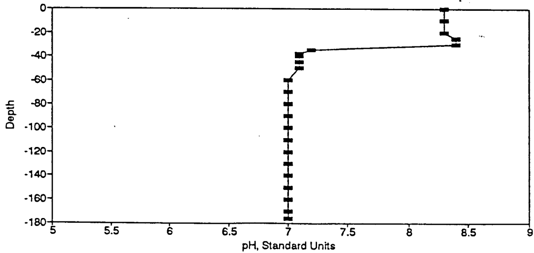
Figure BP57. pH Profile for the Eureka Springs Site-September 28, 1978.
