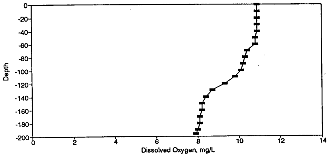
Figure BD111. Dissolved Oxygen Profile for the Eureka Springs Site-April 21, 1983.
