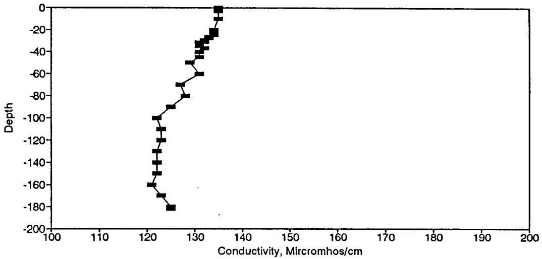
Figure BC151. Conductivity Profile for the Eureka Springs Site-August 4, 1986.
