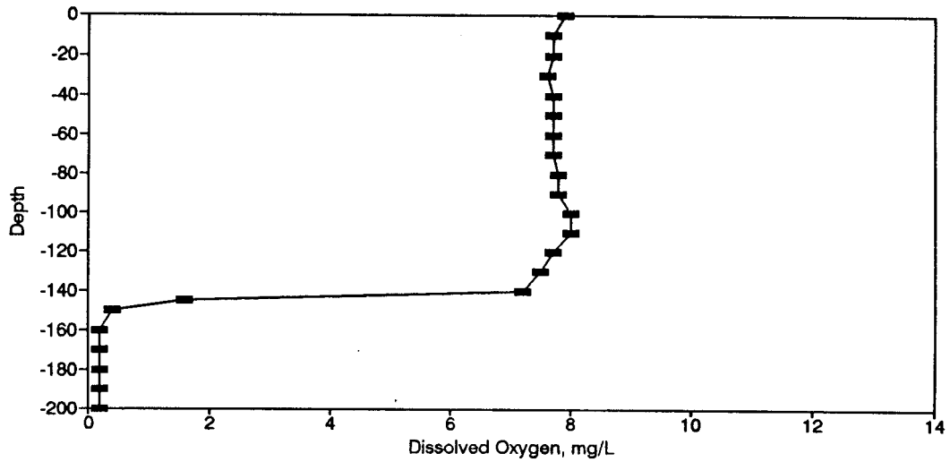
Figure BD1. Dissolved Oxygen Profile for the Eureka Springs Site-December 18, 1973.
