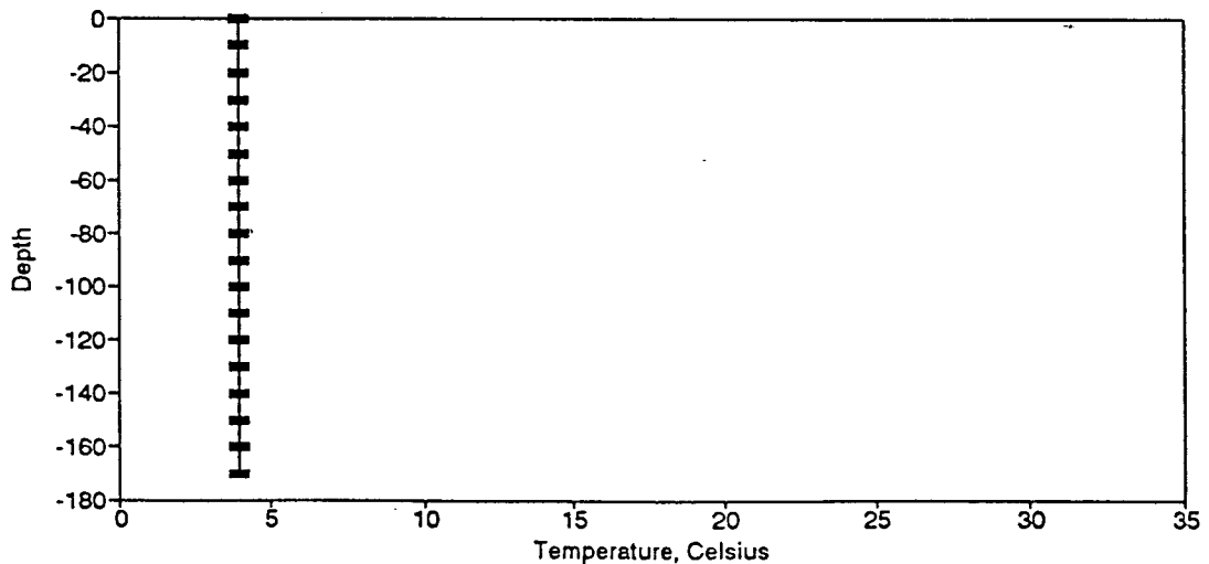
Figure BT120. Temperature Profile for the Eureka Springs Site-January 25, 1984.
