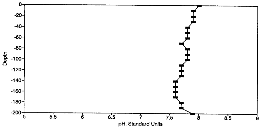
Figure BP4. pH Profile for the Eureka Springs Site-March 19, 1974.
