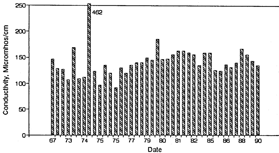
Figure A15. Graph of Conductivity vs. Time for the White River Site-Dec.
