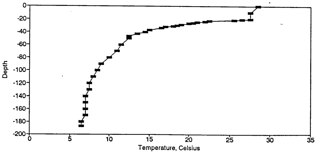
Figure BT174. Temperature Profile for the Eureka Springs Site-July 12, 1988.
