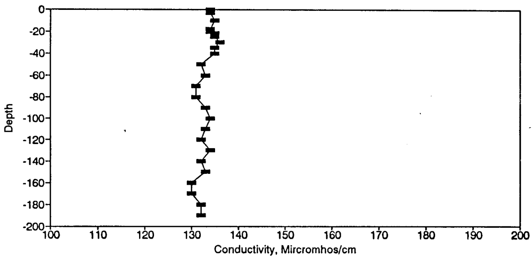
Figure BC183. Conductivity Profile for the Eureka Springs Site-May 2, 1989.
