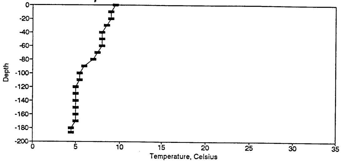
Figure BT64. Temperature Profile for the Eureka Springs Site-April 9, 1979.
