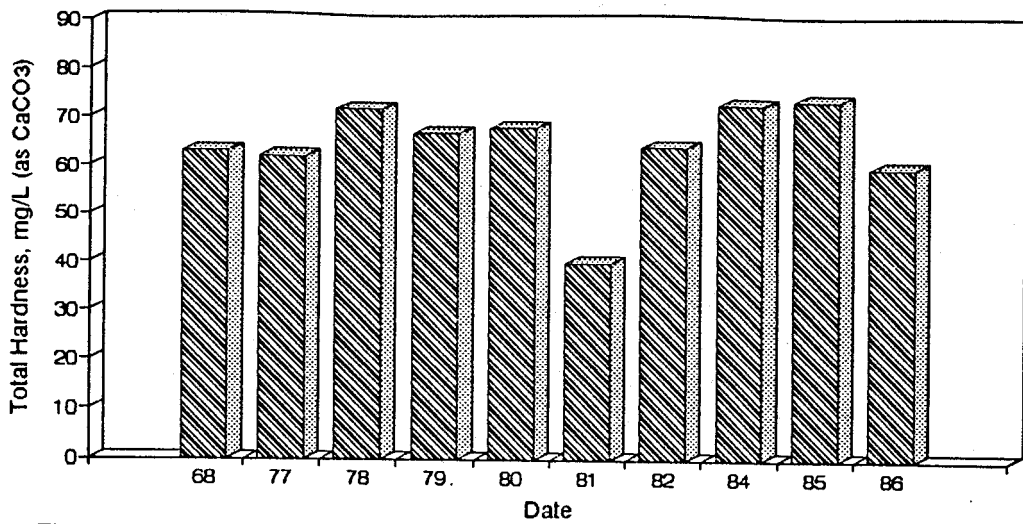
Figure A25. Graph of Total Hardness vs. Time for the White River Site-May.
