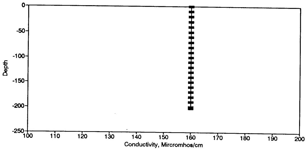
Figure BC133. Conductivity Profile for the Eureka Springs Site-February 6, 1985.
