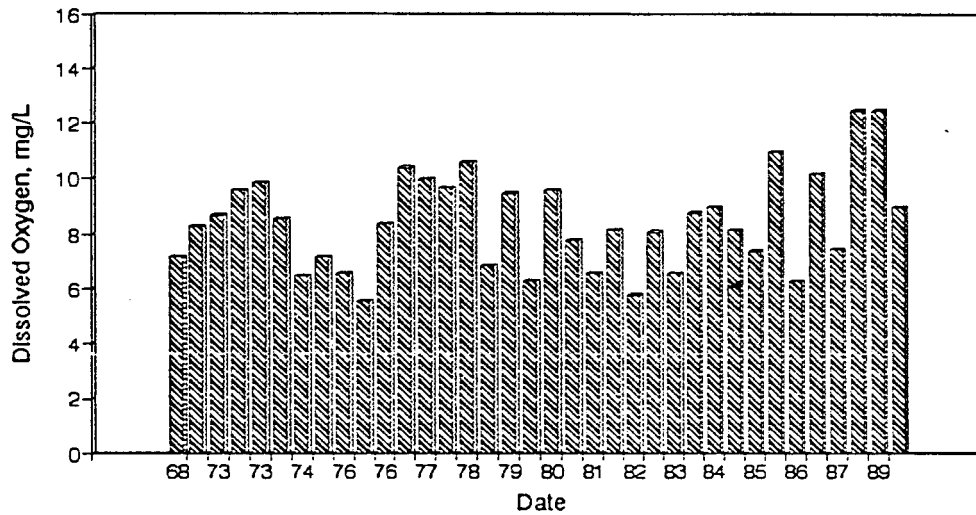
Figure A17. Graph of Dissolved Oxygen vs. Time for the White River Site-Aug.
