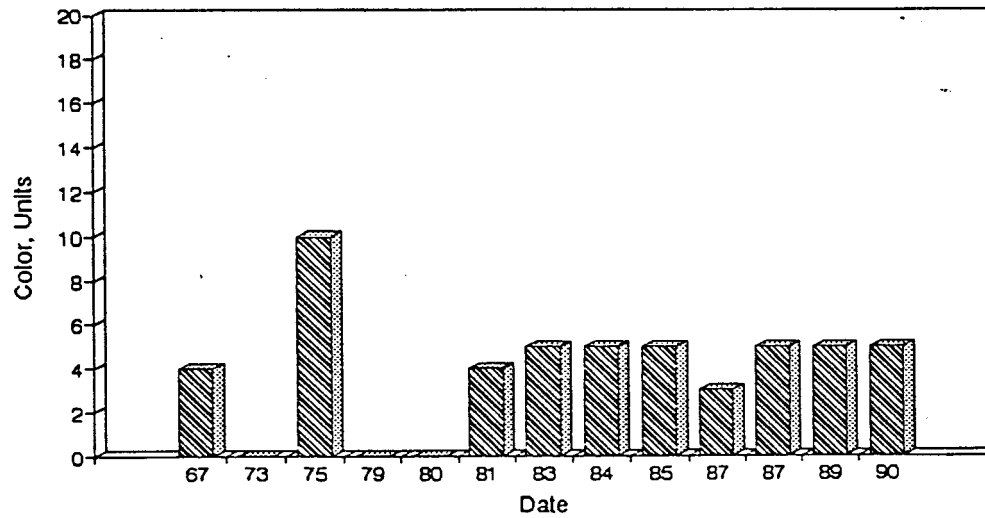
Figure A12. Graph of Color vs. Time for the White River Site-Dec.
