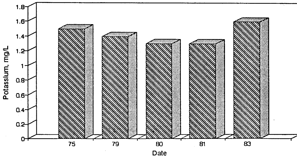
Figure A69. Graph of Potassium vs. Time for the White River Site-Dec.
