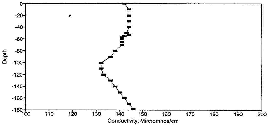
Figure BC58. Conductivity Profile for the Eureka Springs Site-October 10, 1978.
