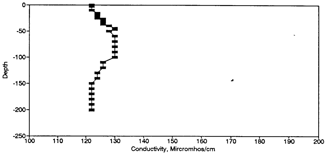
Figure BC137. Conductivity Profile for the Eureka Springs Site-June 5, 1985.
