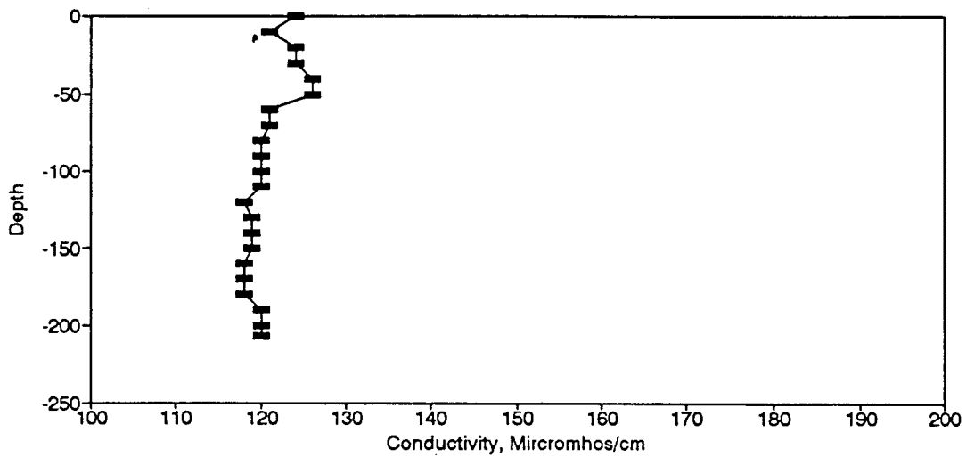
Figure BC16. Conductivity Profile for the Eureka Springs Site-April 15, 1975.
