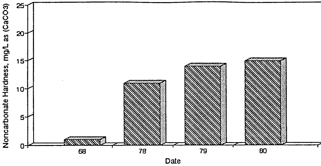
Figure A37. Graph of Noncarbonate Hardness vs. Time for the White River Site-May.
