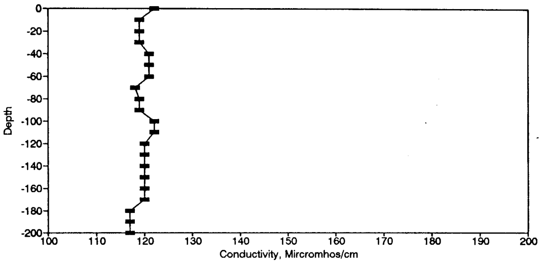
Figure BC15. Conductivity Profile for the Eureka Springs Site - March 17, 1975.
