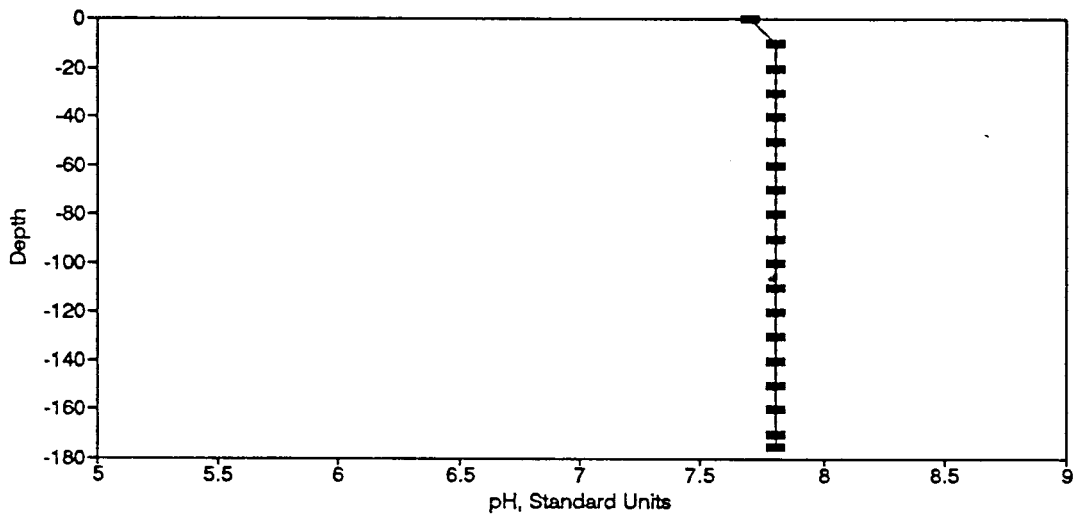
Figure BP62. pH Profile for the Eureka Springs Site-February 14, 1979.
