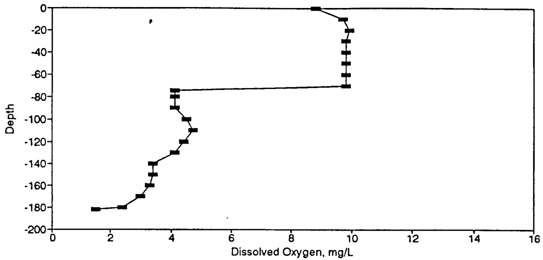
Figure BD49. Dissolved Oxygen Profile for the Eureka Springs Site-December 7, 1977.
