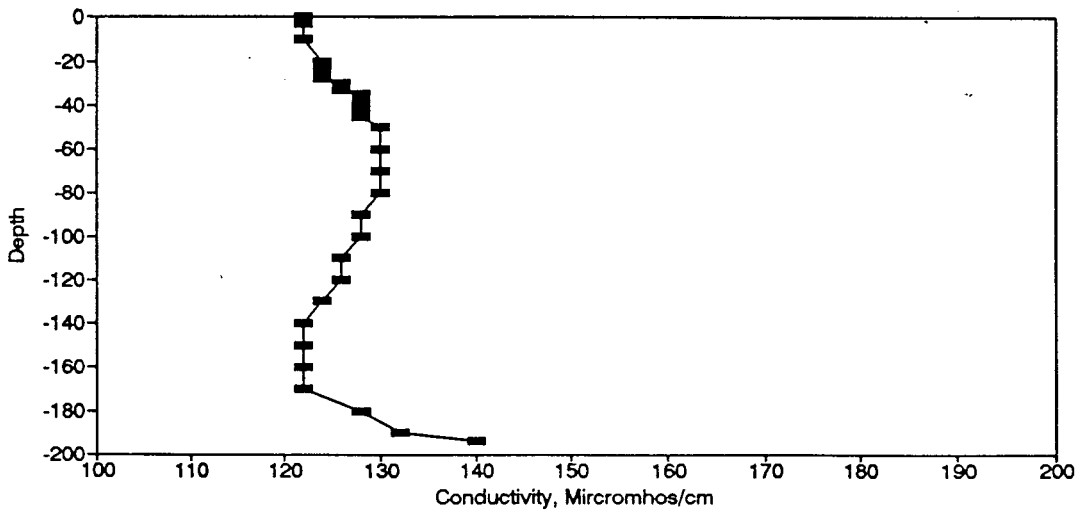
Figure BC138. Conductivity Profile for the Eureka Springs Site-July 11, 1985.
