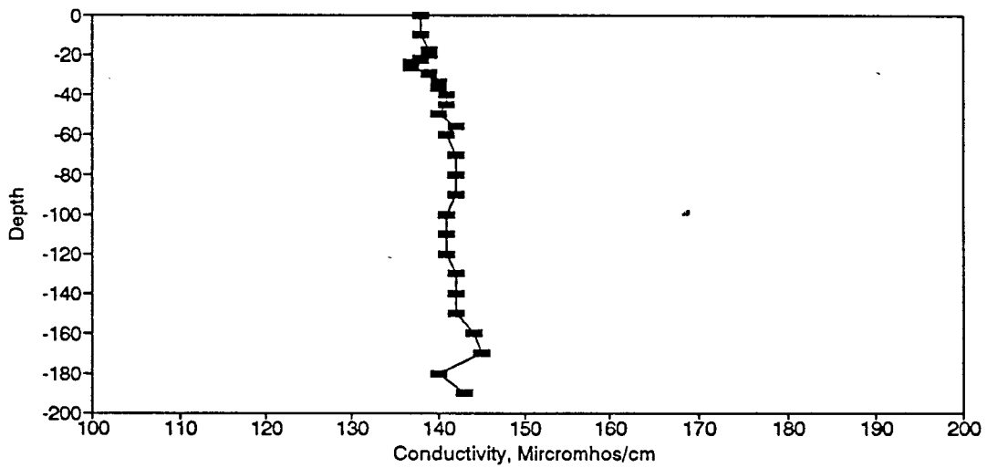
Figure BC173. Conductivity Profile for the Eureka Springs Site-June 15, 1988.
