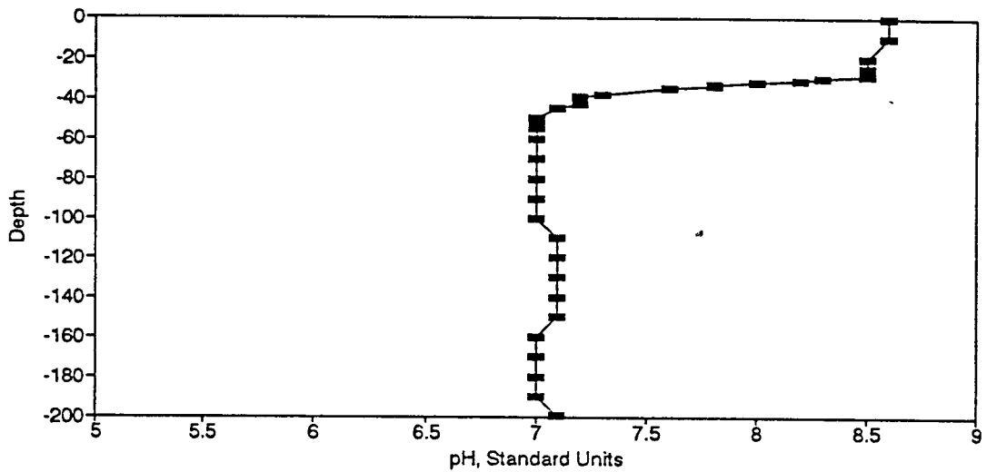
Figure BP68. pH Profile for the Eureka Springs Site - August 22, 1979.
