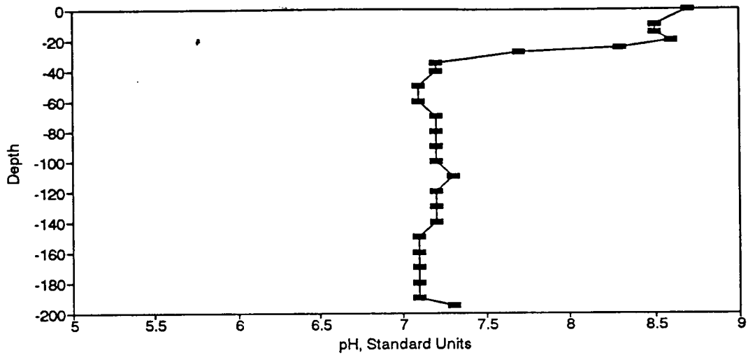
Figure BP7. pH Profile for the Eureka Springs Site-July 8, 1974.
