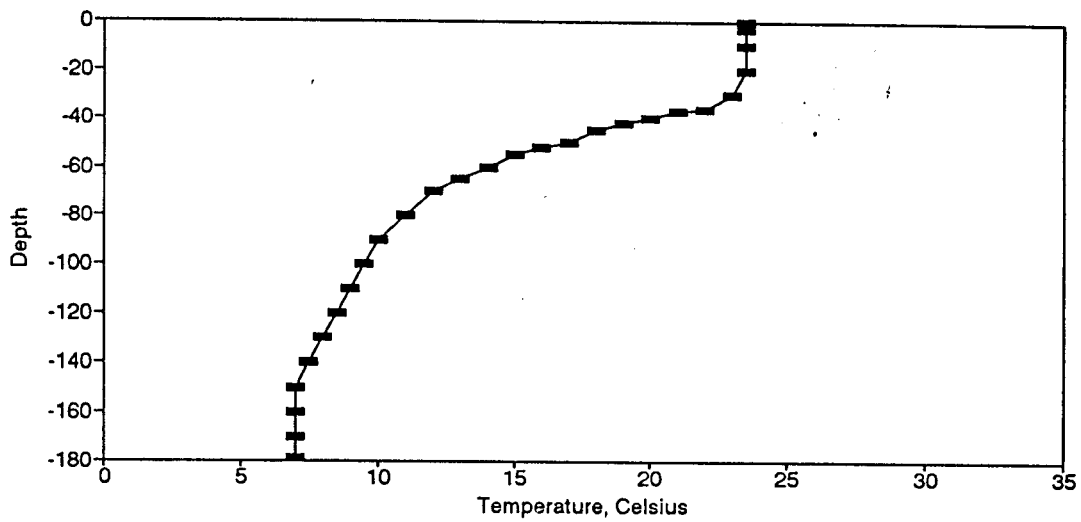
Figure BT104. Temperature Profile for the Eureka Springs Site-September 23, 1982.
