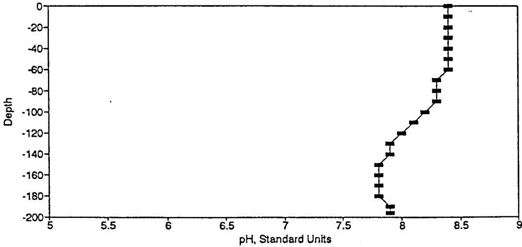
Figure BP111. pH Profile for the Eureka Springs Site-April 21, 1983.
