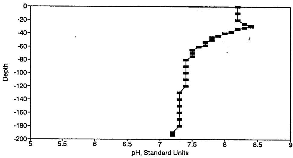
Figure BP89. pH Profile for the Eureka Springs Site-June 16, 1981.
