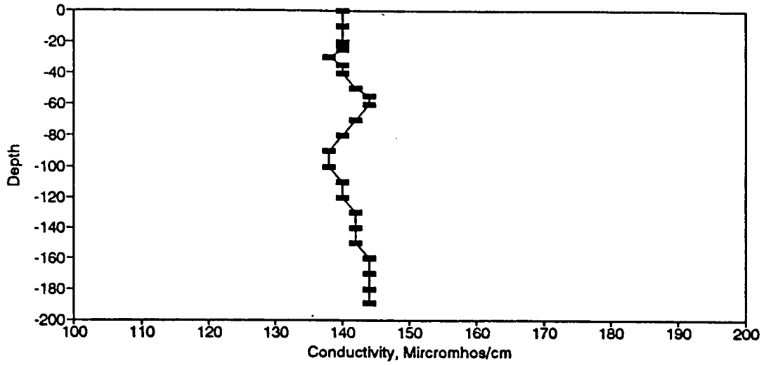
Figure BC55. Conductivity Profile for the Eureka Springs Site-July 18, 1978.
