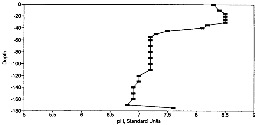
Figure BP22. pH Profile for the Eureka Springs Site-October 14, 1975.
