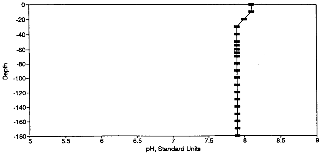
Figure BP48. pH Profile for the Eureka Springs Site-November 9, 1977.
