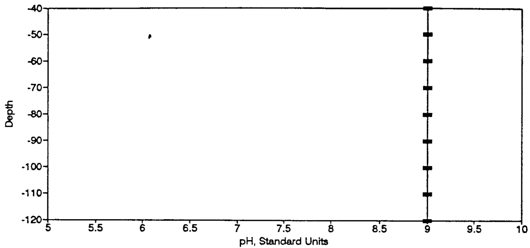
Figure BP61. pH Profile for the Eureka Springs Site-January 9, 1979.
