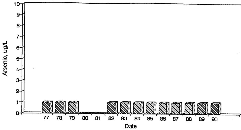
Figure A43. Graph of Arsenic vs. Time for the White River Site-May.
