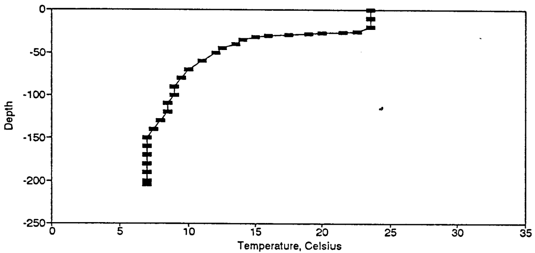
Figure BT113. Temperature Profile for the Eureka Springs Site-June 14, 1983.
