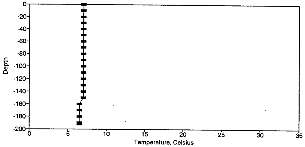
Figure BT157. Temperature Profile for the Eureka Springs Site-February 4, 1987.
