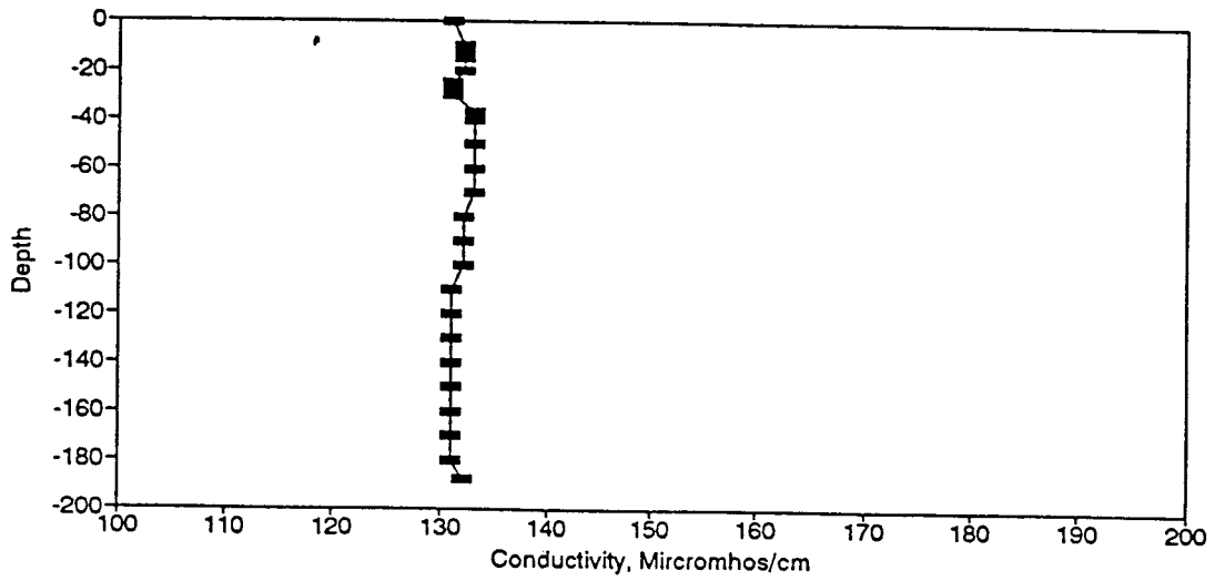
Figure BC124. Conductivity Profile for the Eureka Springs Site-May 21, 1984.
