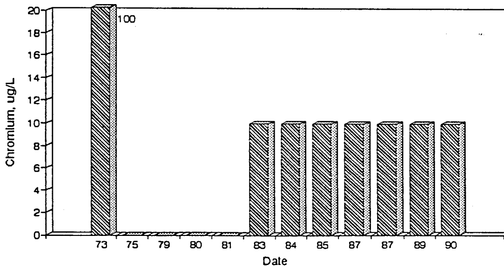
Figure A48. Graph of Chromium vs. Time for the White River Site-Dec.
