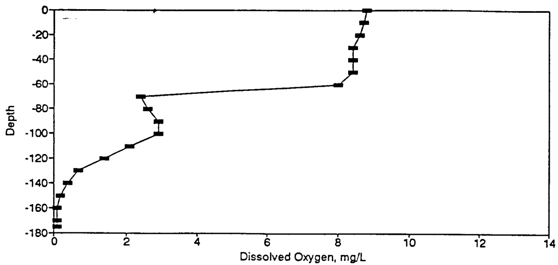
Figure BD106. Dissolved Oxygen Profile for the Eureka Springs Site-November 24, 1982.
