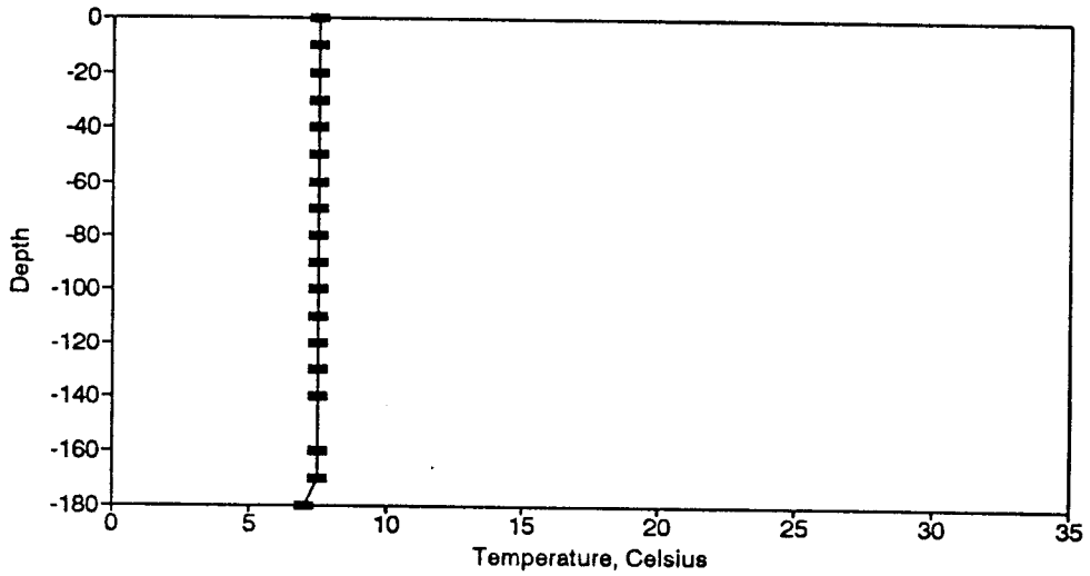
Figure BT73. Temperature Profile for the Eureka Springs Site-January 8, 1980
