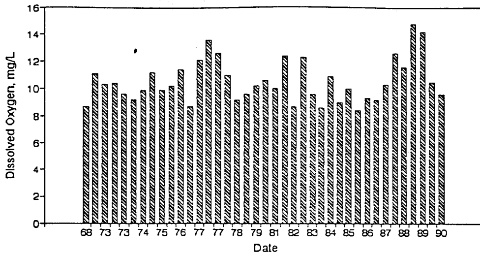
Figure A16. Graph of Dissolved Oxygen vs. Time for the White River Site-May.
