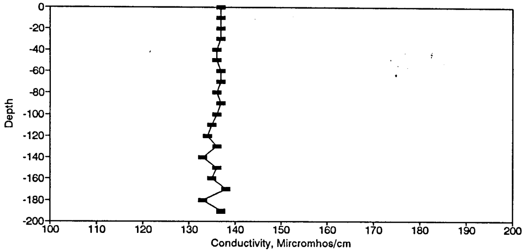
Figure BC182. Conductivity Profile for the Eureka Springs Site-April 11, 1989.
