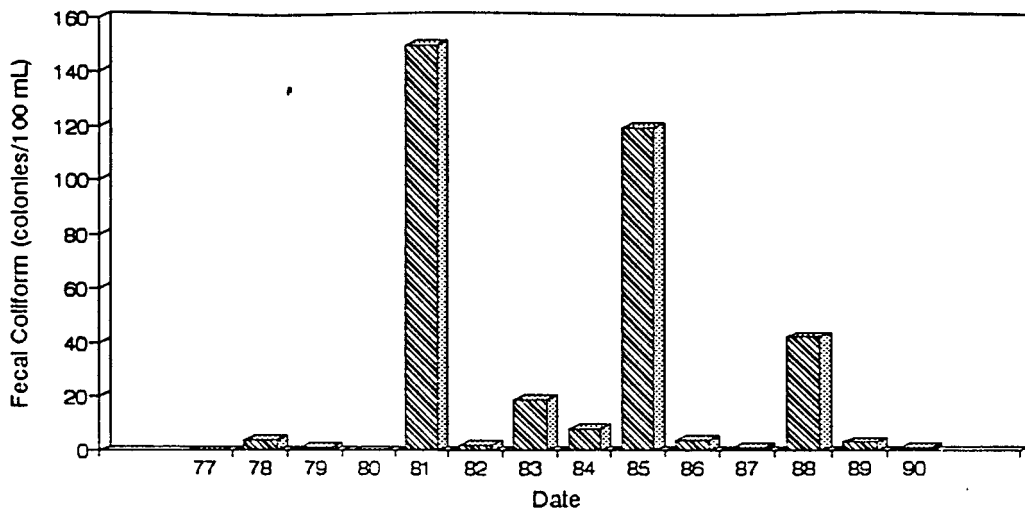
Figure A22. Graph of Fecal Coliform vs. Time for the White River Site-May.
