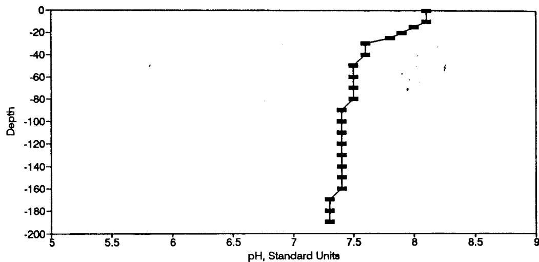
Figure BP17. pH Profile for the Eureka Springs Site-May 14, 1975.
