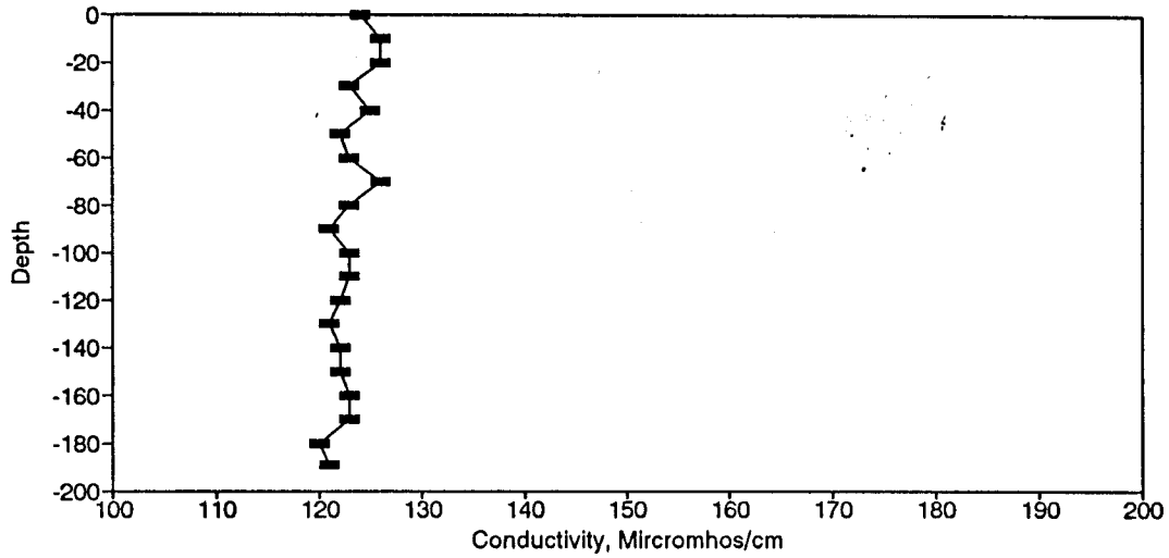
Figure BC146. Conductivity Profile for the Eureka Springs Site-March 6, 1986.
