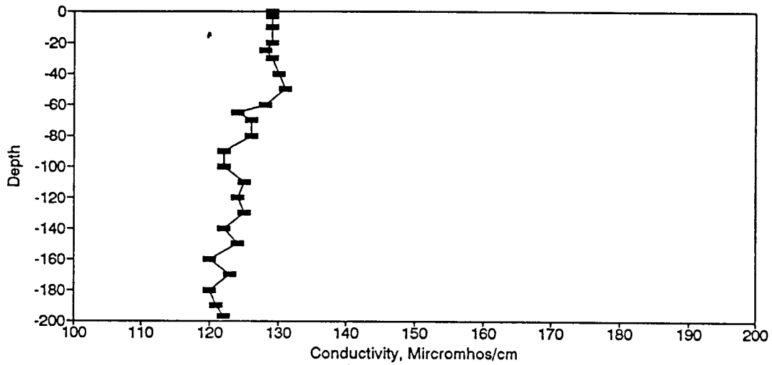
Figure BC148. Conductivity Profile for the Eureka Springs Site-May 6, 1986.
