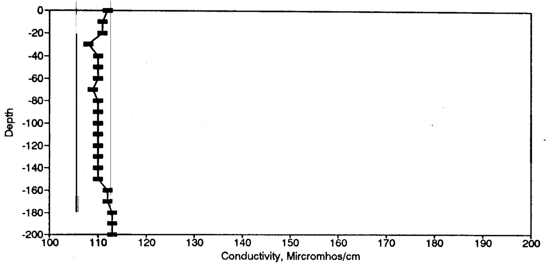
Figure BC3. Conductivity Profile for the Eureka Springs Site-February 20, 1974.
