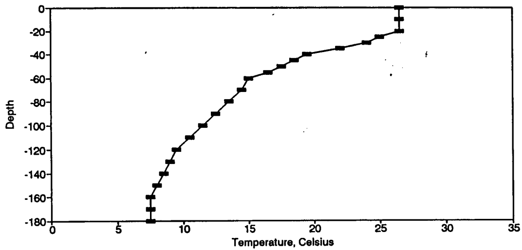
Figure BT32. Temperature Profile for the Eureka Springs Site-August 24, 1976.
