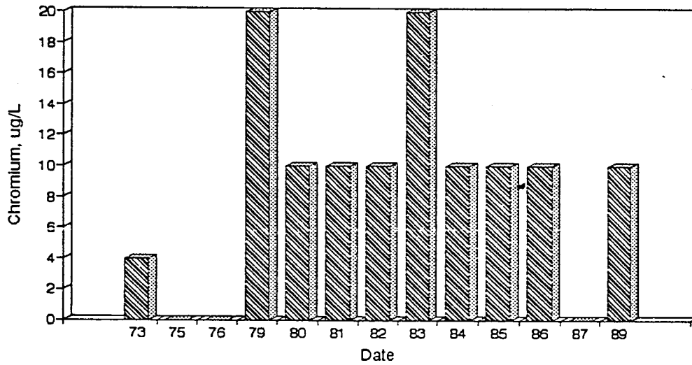
Figure A47. Graph of Chromium vs. Time for the White River Site-Aug.
