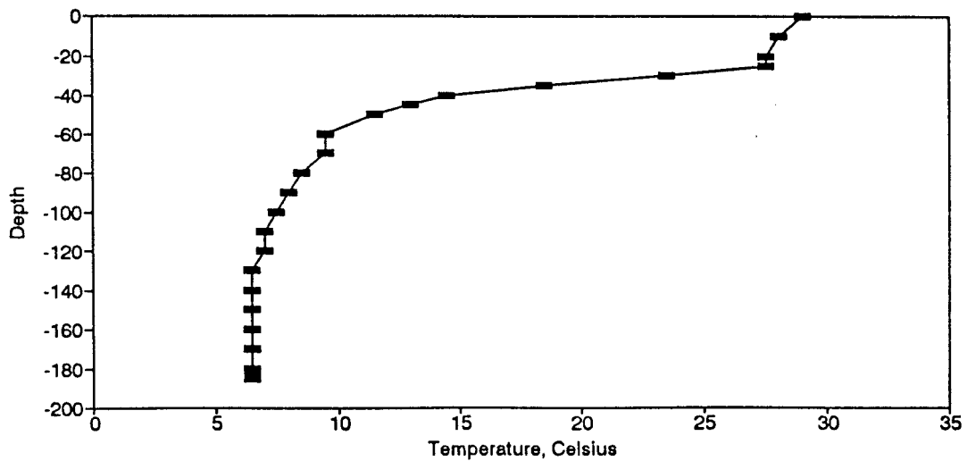
Figure BT45. Temperature Profile for the Eureka Springs Site-August 22, 1977.
