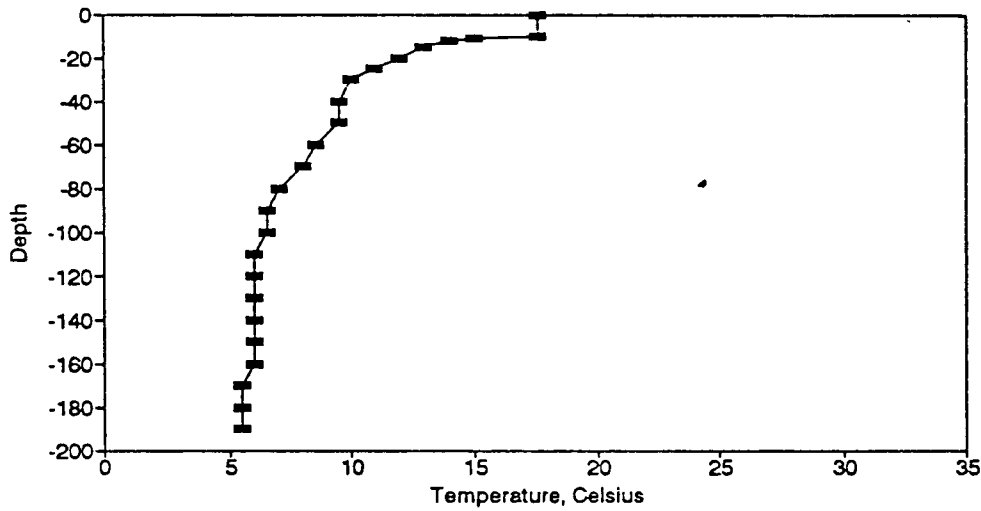
Figure BT77. Temperature Profile for the Eureka Springs Site-May 7, 1980.
