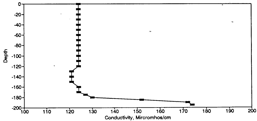
Figure BC12. Conductivity Profile for the Eureka Springs Site-December 16, 1974.
