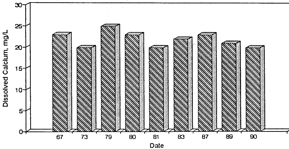
Figure A33. Graph of Dissolved Calcium vs. Time for the White River Site-Dec.
