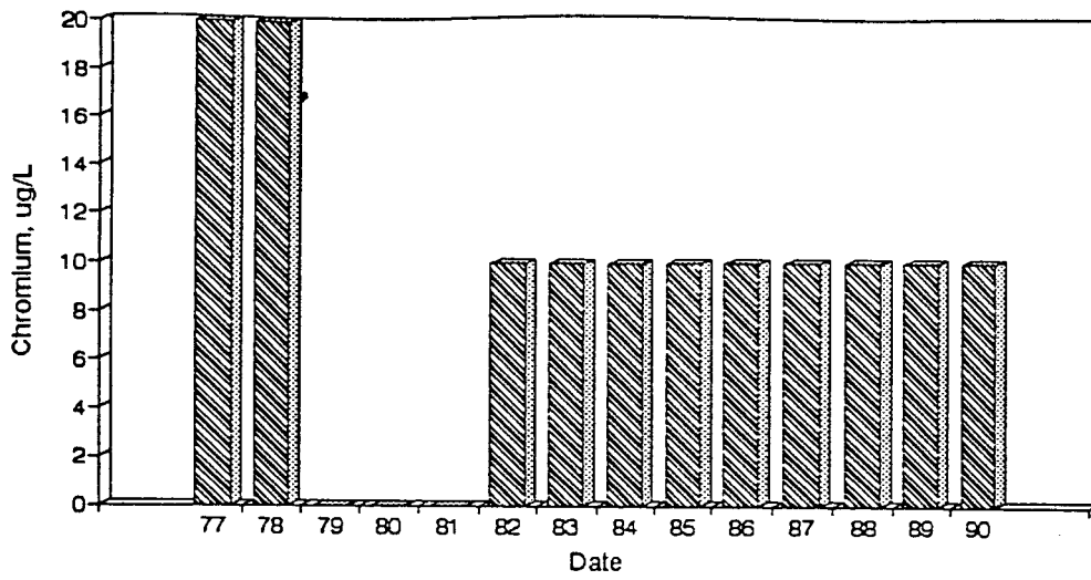
Figure A46. Graph of Chromium vs. Time for the White River Site-May.
