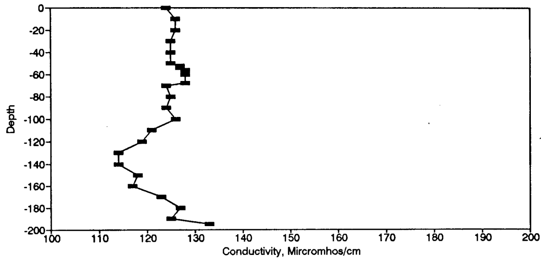
Figure BC141. Conductivity Profile for the Eureka Springs Site-October 10, 1985.
