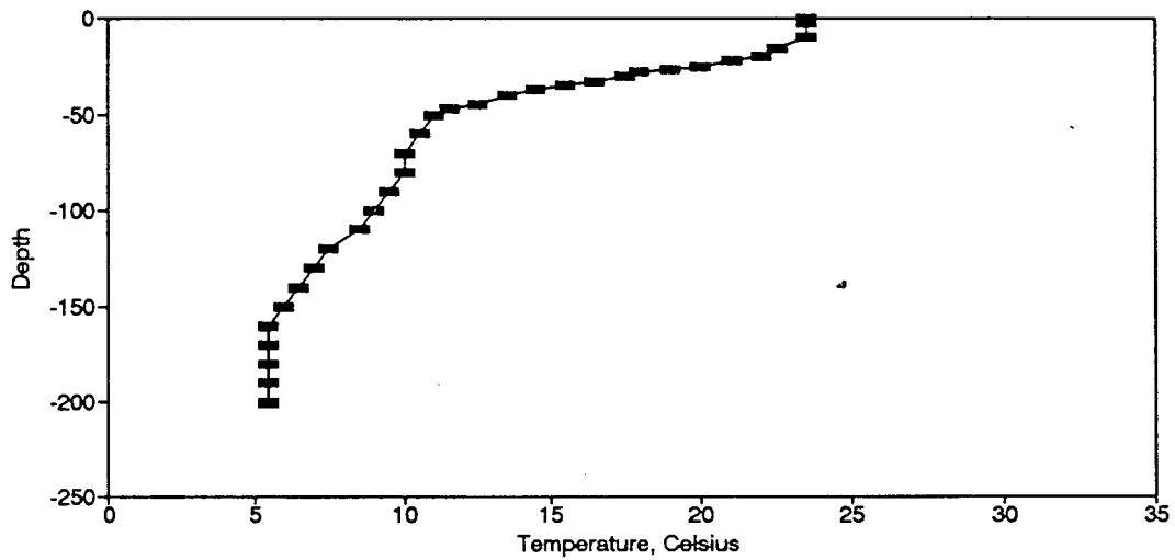
Figure BT137. Temperature Profile for the Eureka Springs Site-June 5, 1985.
