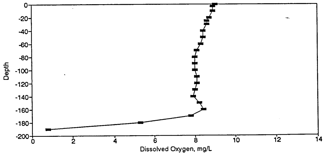
Figure BD156. Dissolved Oxygen Profile for the Eureka Springs Site-January 13, 1987.
