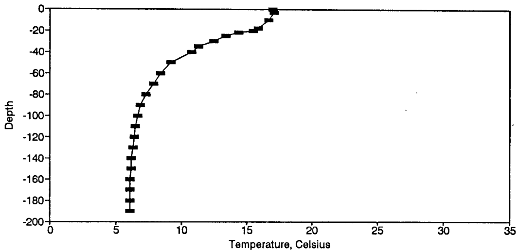
Figure BT183. Temperature Profile for the Eureka Springs Site-May 2, 1989.
