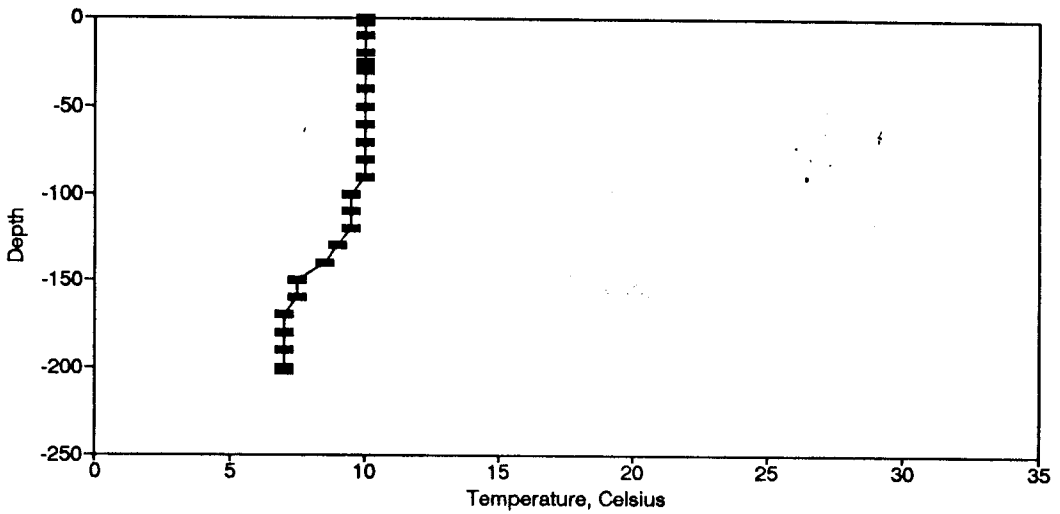
Figure BT131. Temperature Profile for the Eureka Springs Site-December 13, 1984.
