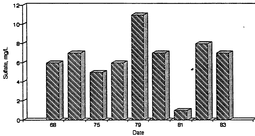
Figure A101. Graph of Sulfate vs. Time for the White River Site-Aug.
