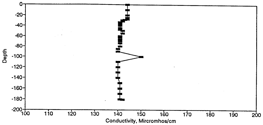
Figure BC91. Conductivity Profile for the Eureka Springs Site-August 12, 1981.
