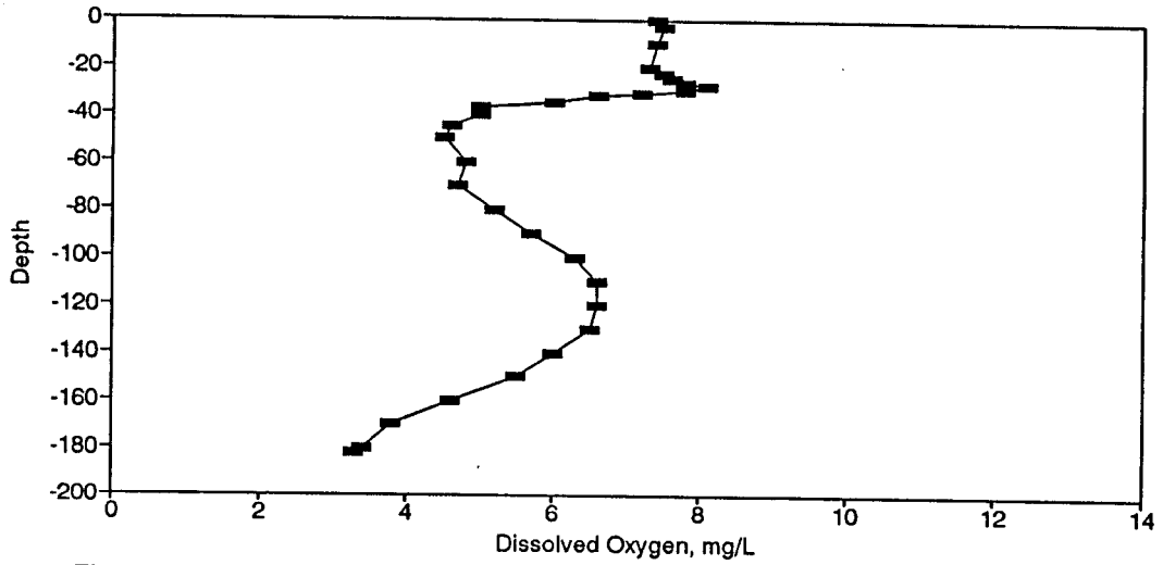
Figure BD151. Dissolved Oxygen Profile for the Eureka Springs Site-August 4, 1986.
