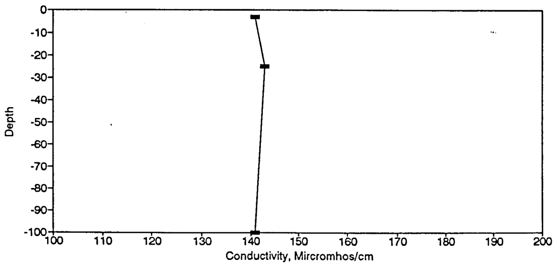
Figure BC186. Conductivity Profile for the Eureka Springs Site-August 8, 1989.
