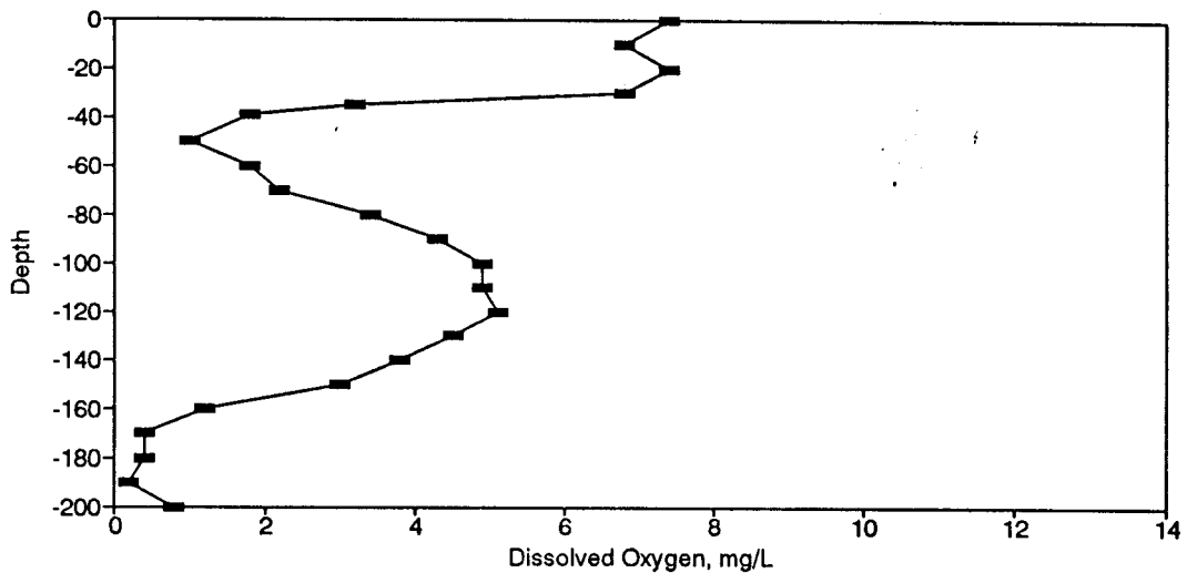
Figure BD8. Dissolved Oxygen Profile for the Eureka Springs Site-August 13, 1974.
