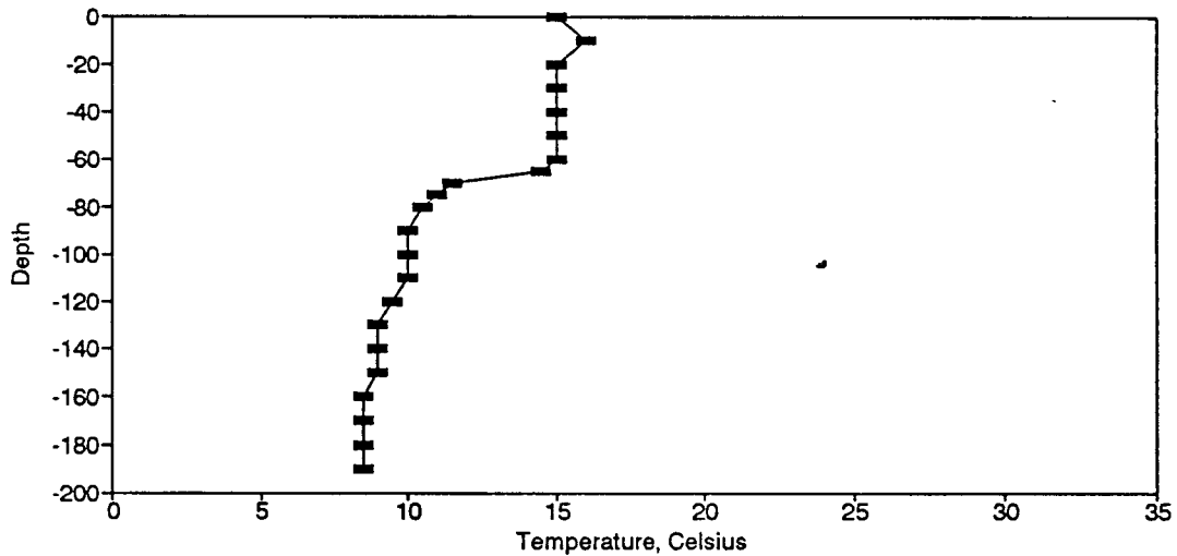
Figure BT23. Temperature Profile for the Eureka Springs Site-November 18, 1975.
