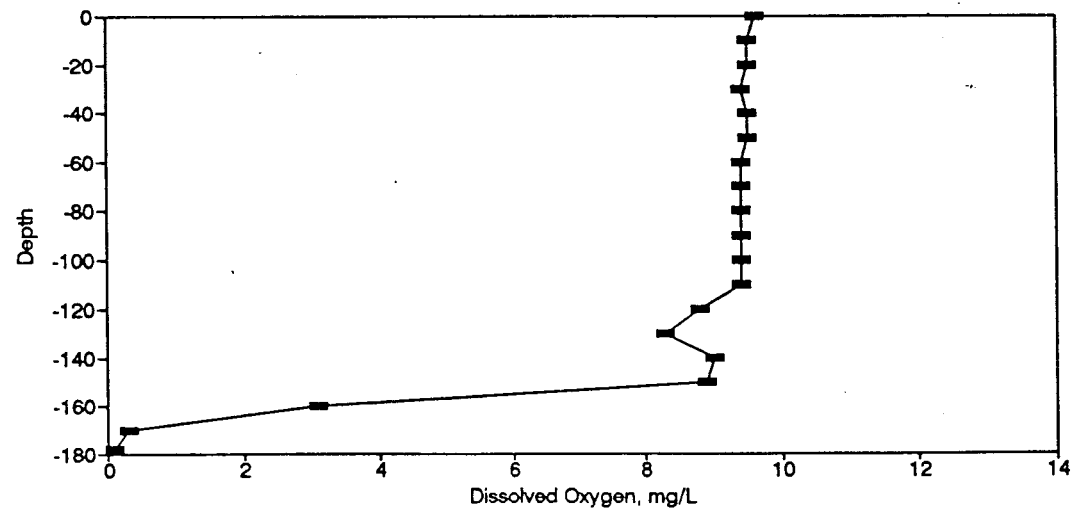
Figure BD36. Dissolved Oxygen Profile for the Eureka Springs Site-December 14, 1976.
