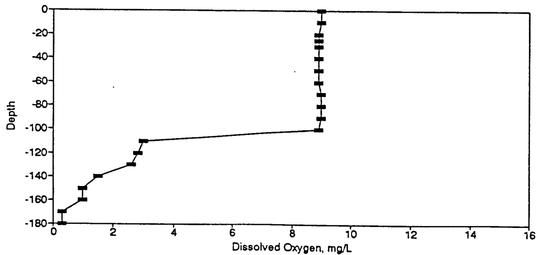
Figure BD72. Dissolved Oxygen Profile for the Eureka Springs Site-December 5, 1979.
