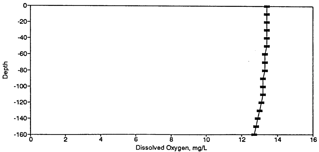
Figure BD39. Dissolved Oxygen Profile for the Eureka Springs Site-March 8, 1977.
