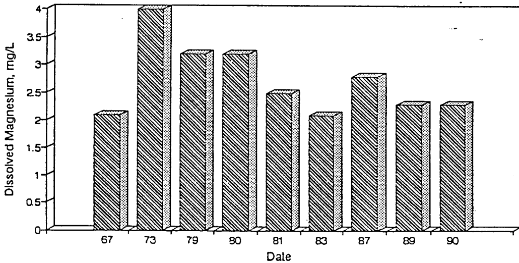
Figure A36. Graph of Dissolved Magnesium vs. Time for the White River Site-Dec.
