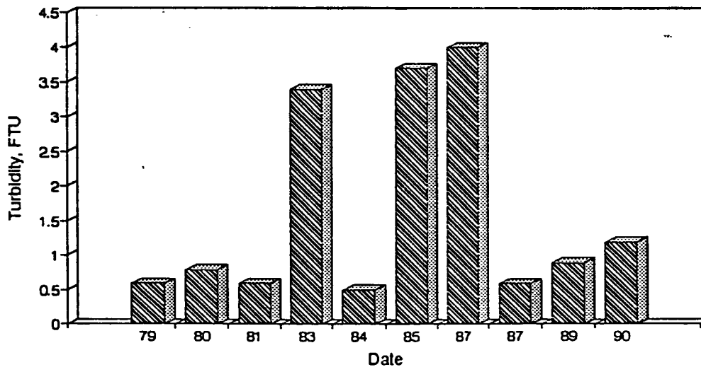
Figure A108. Graph of Turbidity vs. Time for the White River Site-Dec.
