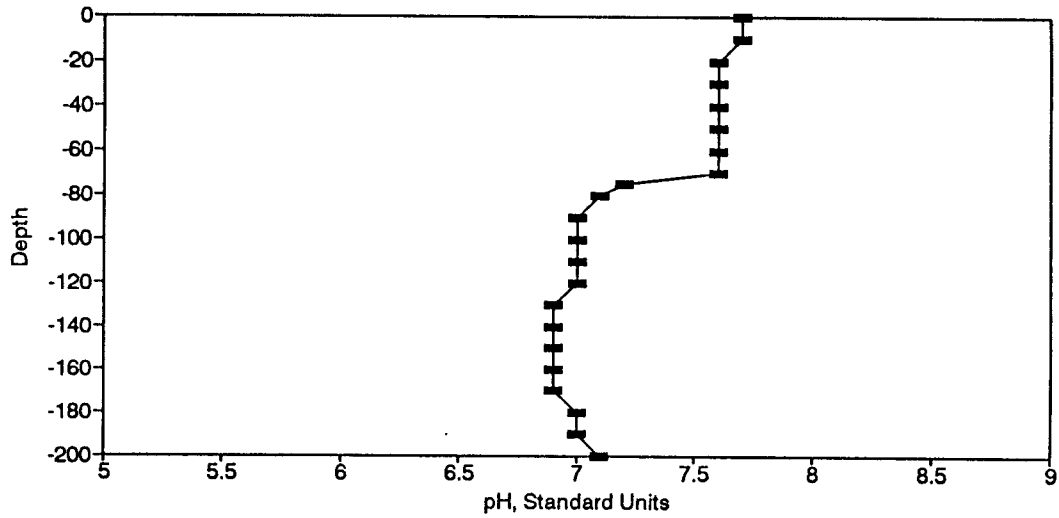
Figure BP10. pH Profile for the Eureka Springs Site-October, 22, 1974.
