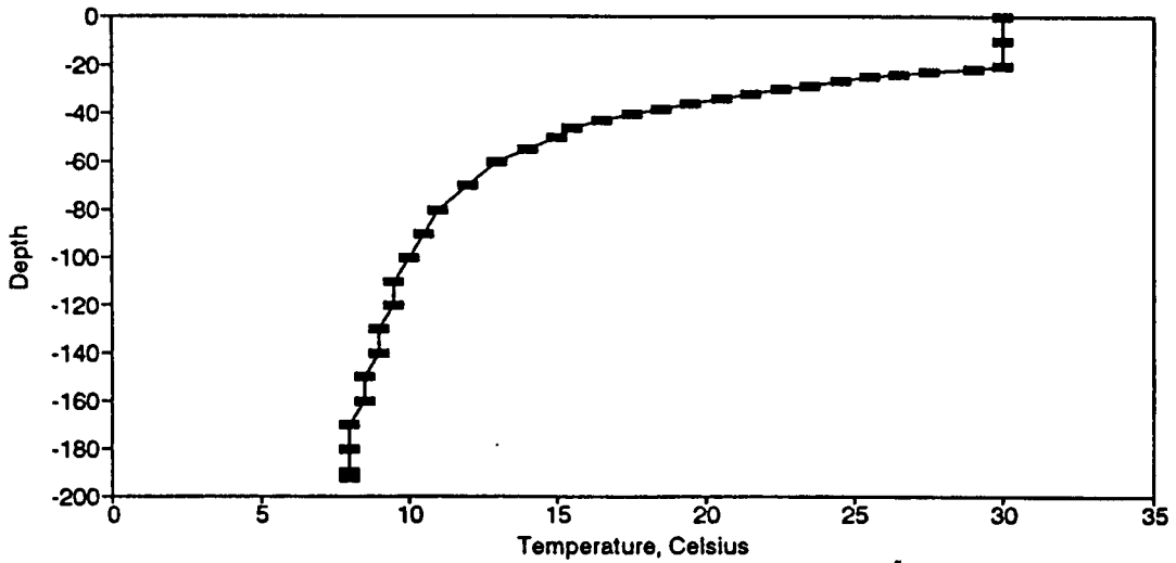
Figure BT115. Temperature Profile for the Eureka Springs Site-August 17, 1983.
