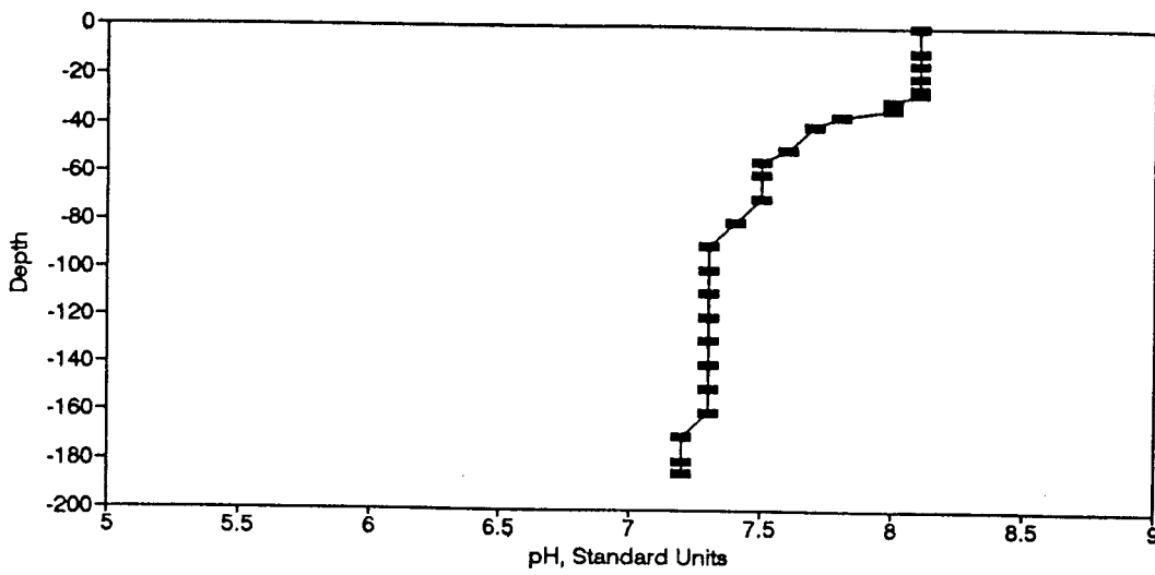
Figure BP100. pH Profile for the Eureka Springs Site-May 19, 1982.
