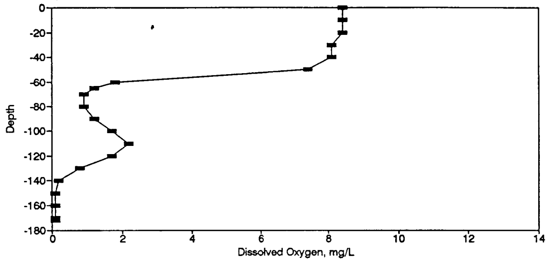
Figure BD34. Dissolved Oxygen Profile for the Eureka Springs Site-October 18, 1976.
