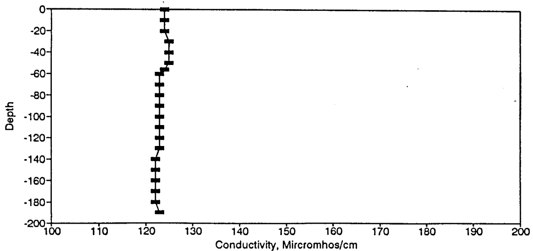
Figure BC123. Conductivity Profile for the Eureka Springs Site-April 24, 1984.
