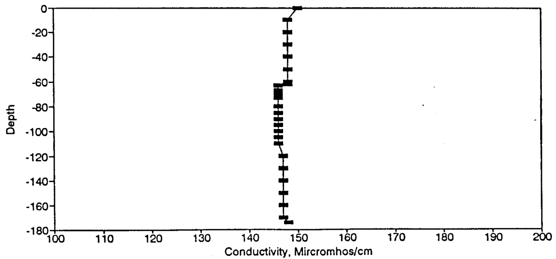
Figure BC93. Conductivity Profile for the Eureka Springs Site-October 20, 1981.
