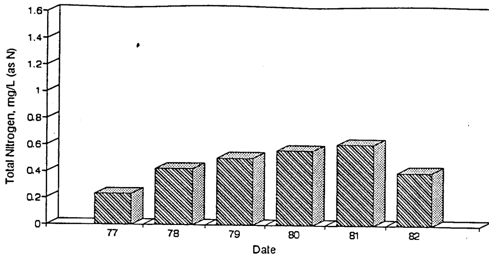
Figure A88. Graph of Total Nitrogen vs. Time for the White River Site-May.
