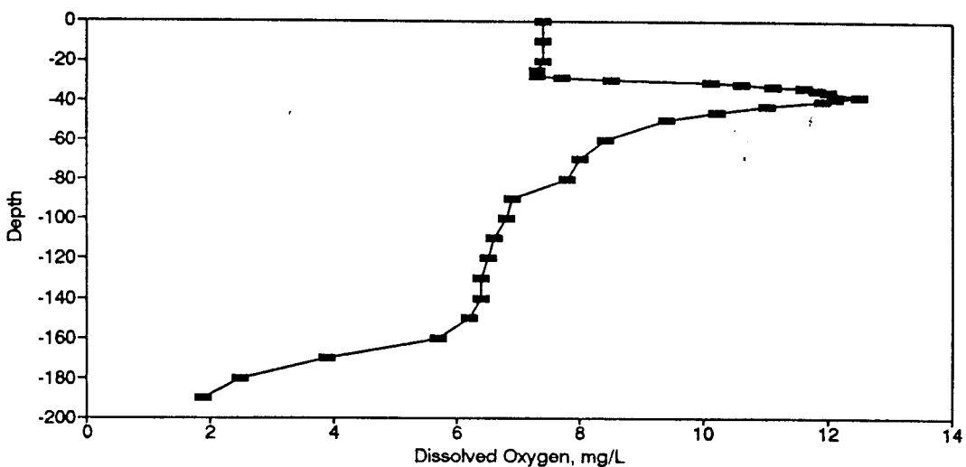
Figure BD80. Dissolved Oxygen Profile for the Eureka Springs Site-August 13, 1980.
