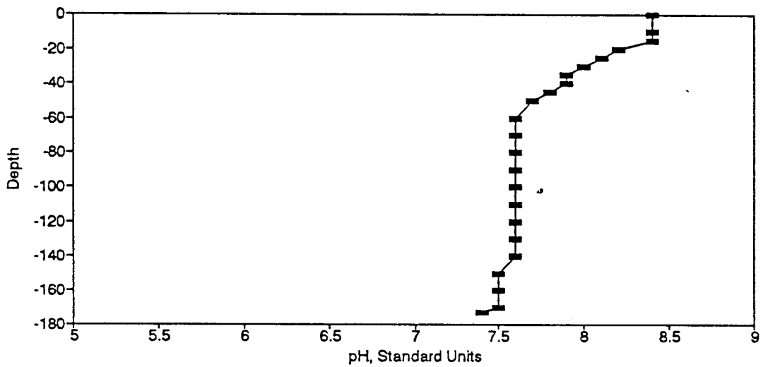
Figure BP44. pH Profile for the Eureka Springs Site-July 26, 1977.
