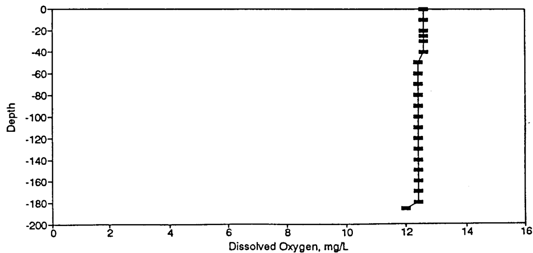
Figure BD51. Dissolved Oxygen Profile for the Eureka Springs Site-March 2, 1978.
