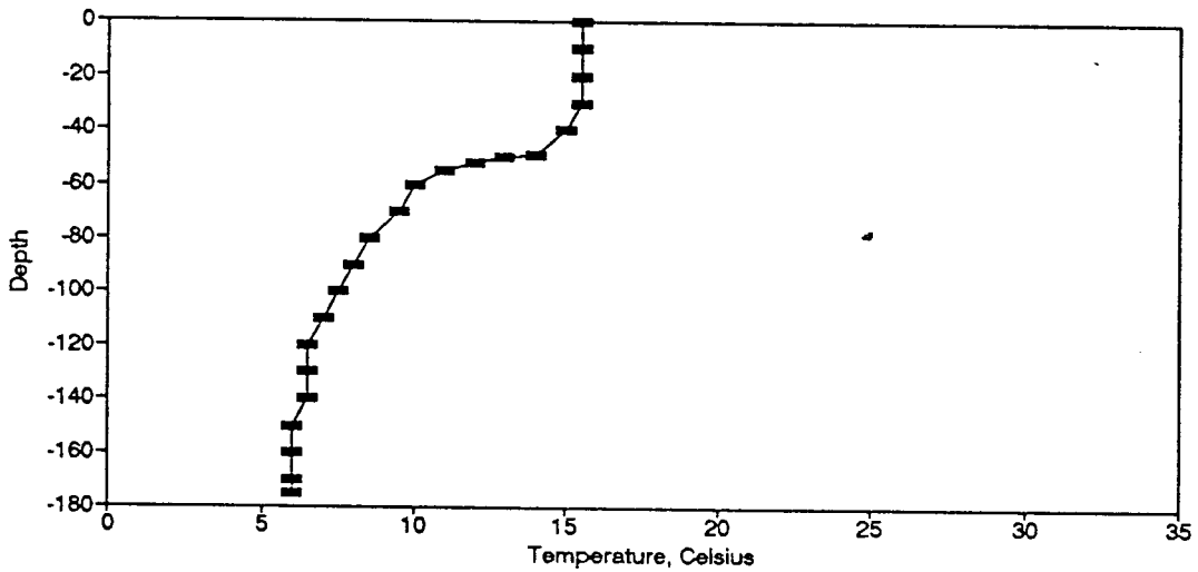
Figure BT83. Temperature Profile for the Eureka Springs Site-November 5, 1980.
