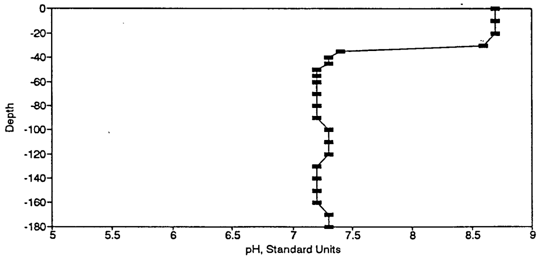
Figure BP33. pH Profile for the Eureka Springs Site-September 22, 1976.
