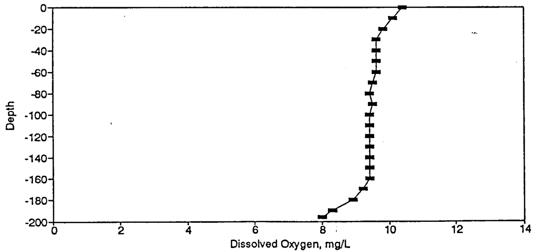
Figure BD144. Dissolved Oxygen Profile for the Eureka Springs Site-Januray 8, 1986.
