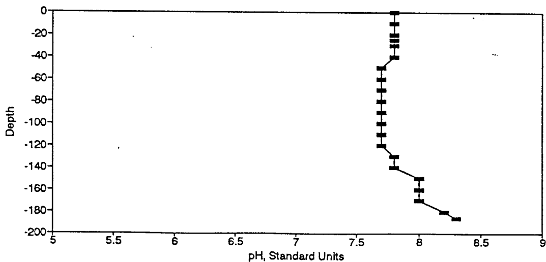
Figure BP51. pH Profile for the Eureka Springs Site-March 2, 1978.
