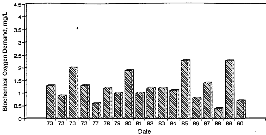
Figure A4. Graph of Biochemical Oxygen Demand vs. Time for the White River Site-May.
