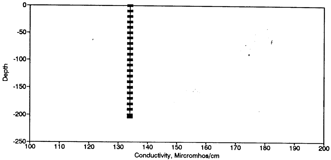
Figure BC134. Conductivity Profile for the Eureka Springs Site-March 7, 1985.
