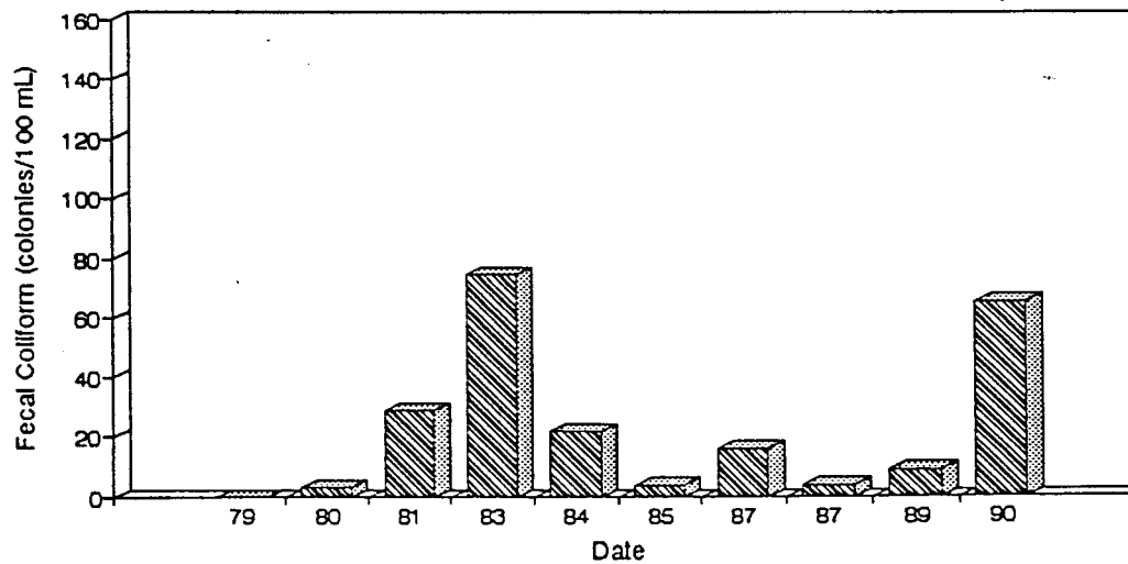
Figure A24. Graph of Fecal Coliform vs. Time for the White River Site-Dec.
