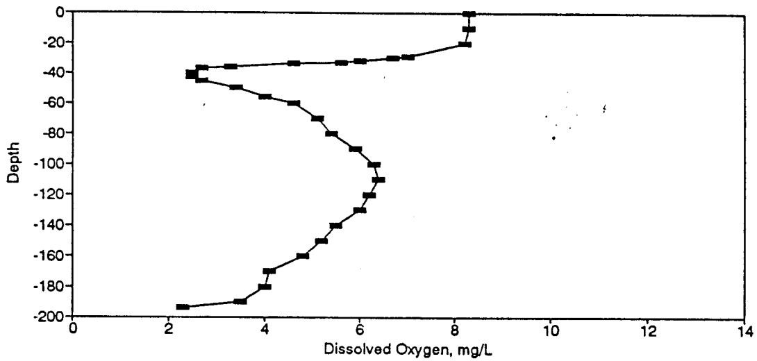
Figure BD176. Dissolved Oxygen Profile for the Eureka Springs Site-September 21, 1988.
