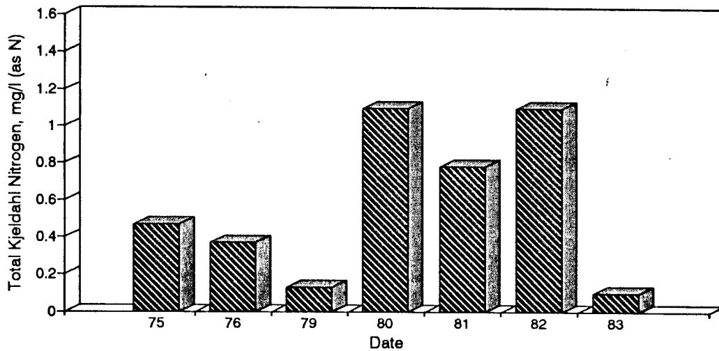
Figure A86. Graph of Total Kjeldahl Nitrogen vs. Time for the White River Site-Aug.
