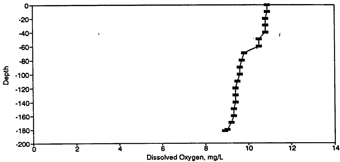
Figure BD110. Dissolved Oxygen Profile for the Eureka Springs Site-March 23, 1983.
