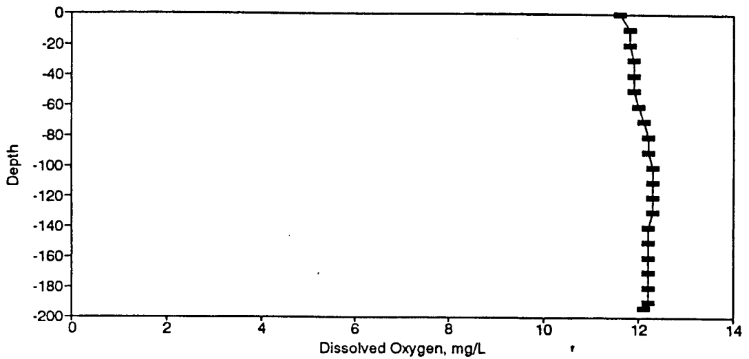
Figure BD97. Dissolved Oxygen Profile for the Eureka Springs Site-February 16, 1982.
