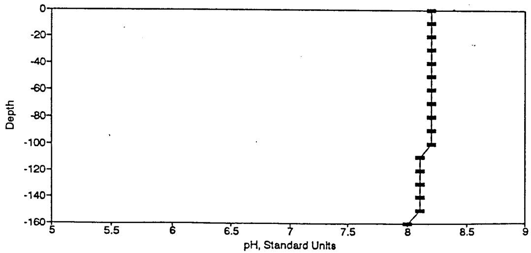
Figure BP39. pH Profile for the Eureka Springs Site-March 8, 1977.
