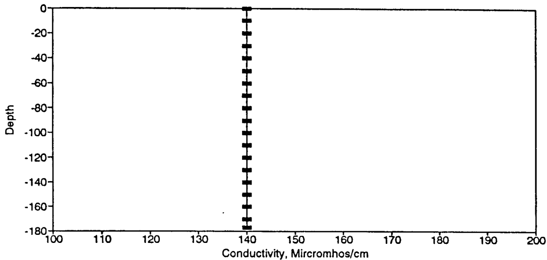
Figure BC61. Conductivity Profile for the Eureka Springs Site-January 9, 1979.
