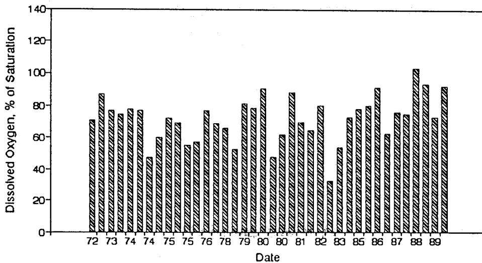
Figure A21. Graph of Dissolved Oxygen vs. Time for the White River Site-Dec.
