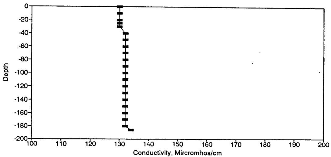
Figure BC51. Conductivity Profile for the Eureka Springs Site-March 2, 1978.
