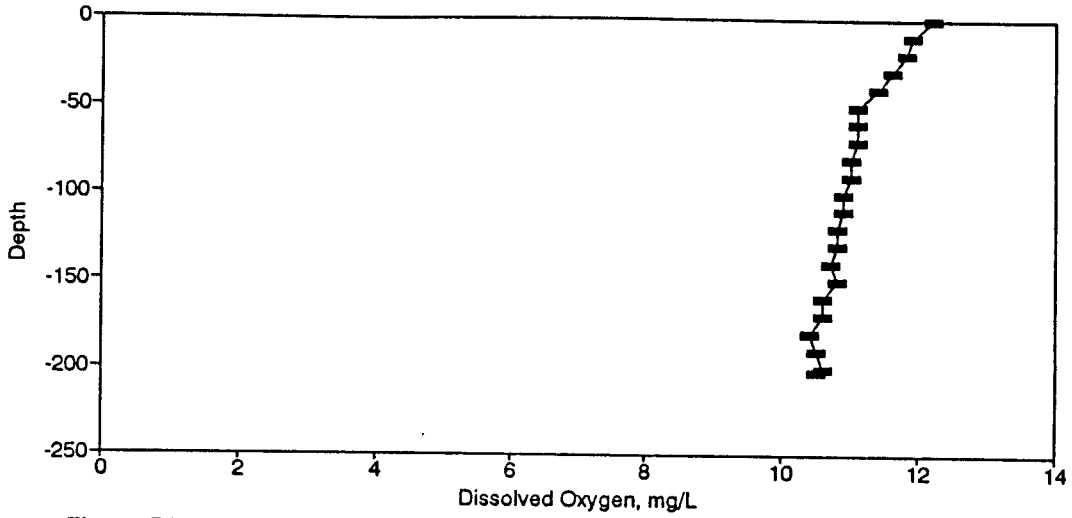
Figure BD181. Dissolved Oxygen Profile for the Eureka Springs Site-March 15, 1989.
