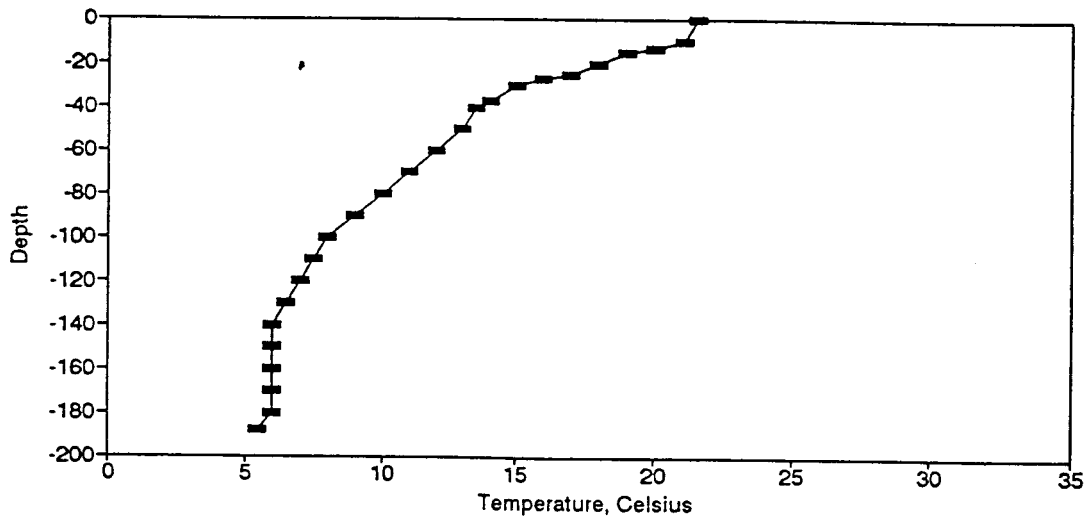
Figure BT124. Temperature Profile for the Eureka Springs Site-May 21, 1984.
