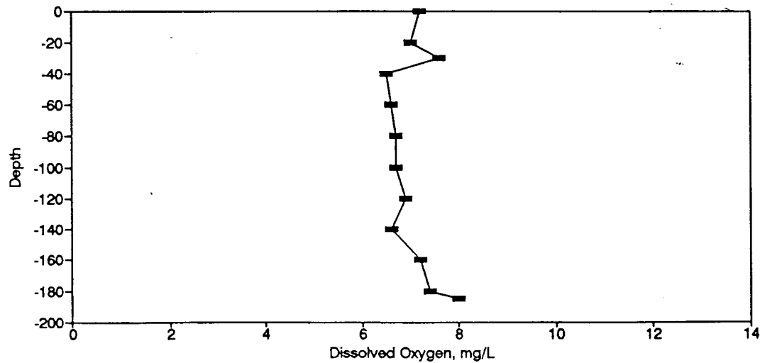
Figure BD18. Dissolved Oxygen Profile for the Eureka Springs Site-June 11, 1975.
