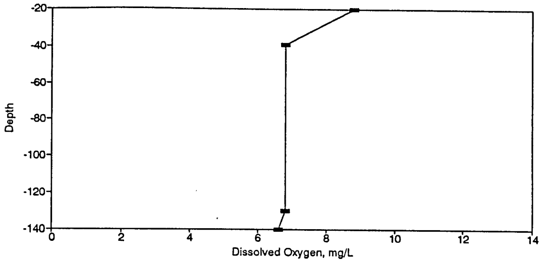
Figure BD187. Dissolved Oxygen Profile for the Eureka Springs Site-September 11, 1989.
