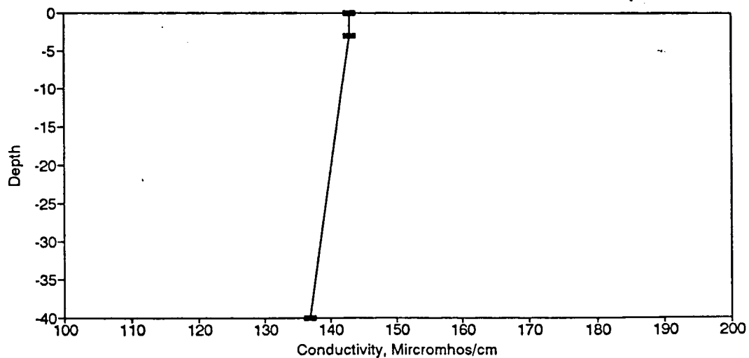
Figure BC162. Conductivity Profile for the Eureka Springs Site-July 15, 1987.
