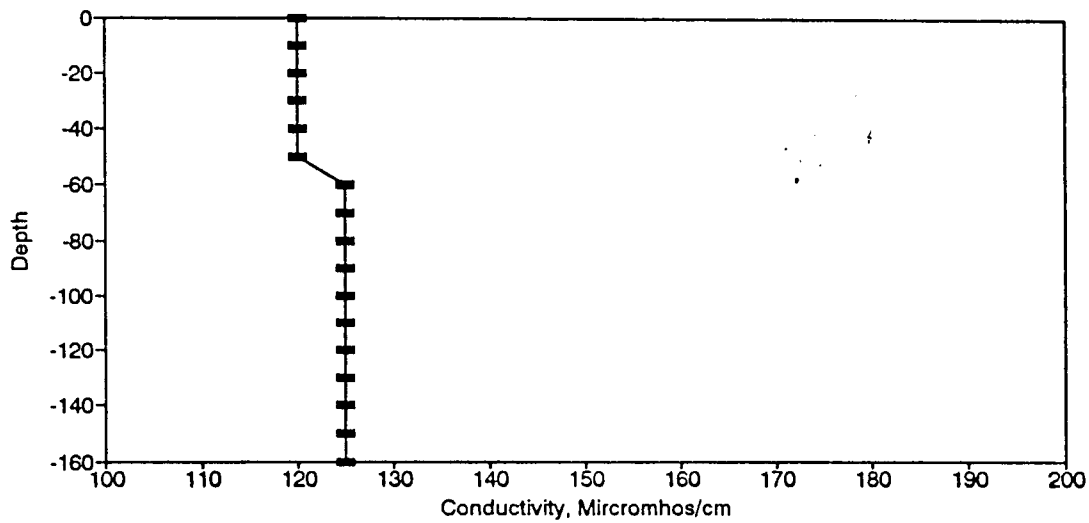
Figure BC38. Conductivity Profile for the Eureka Springs Site-February 7, 1977.
