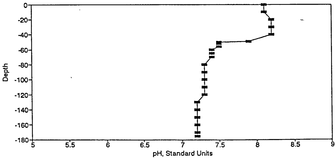
Figure BP105. pH Profile for the Eureka Springs Site-October 22, 1982.
