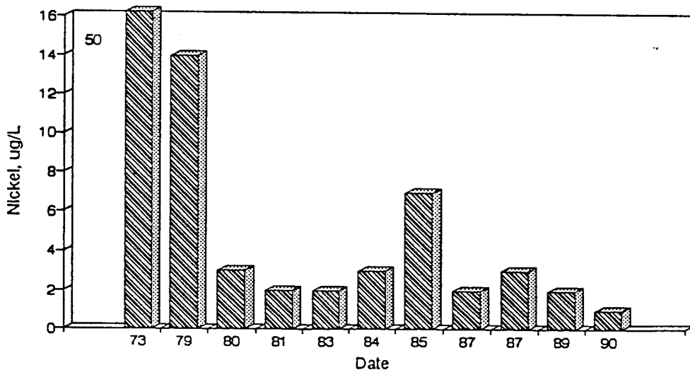
Figure A66. Graph of Nickel vs. Time for the White River Site-Dec.
