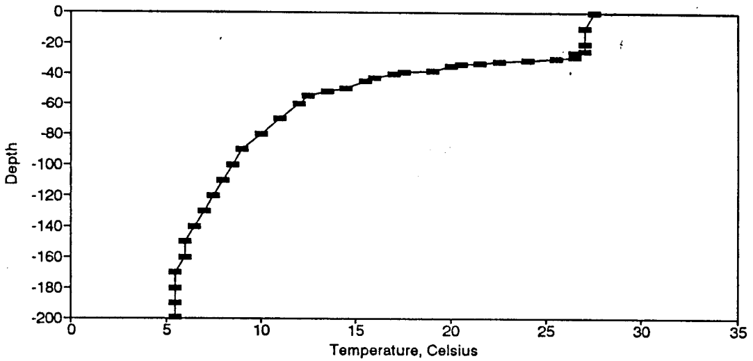
Figure BT68. Temperature Profile for the Eureka Springs Site-August 22, 1979.
