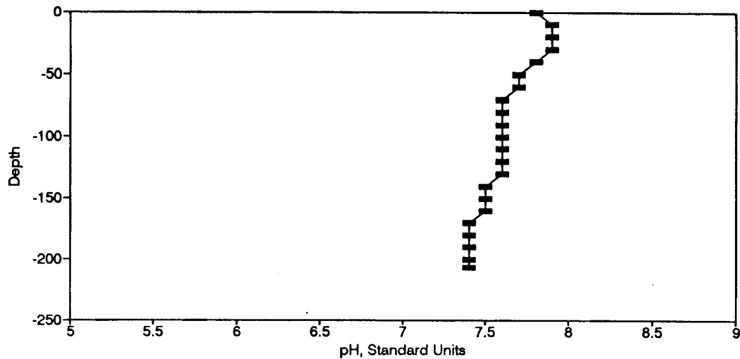
Figure BP16. pH Profile for the Eureka Springs Site-April 15, 1975.
