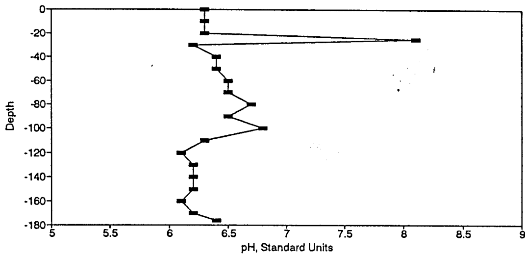
Figure BP119. pH Profile for the Eureka Springs Site-December 7, 1983.
