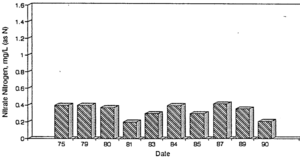
Figure A84. Graph of Nitrate Nitrogen vs. Time for the White River Site-Dec.
