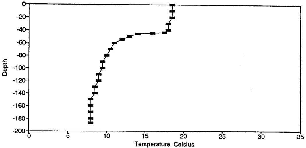
Figure BT165. Temperature Profile for the Eureka Springs Site-October 15, 1987.
