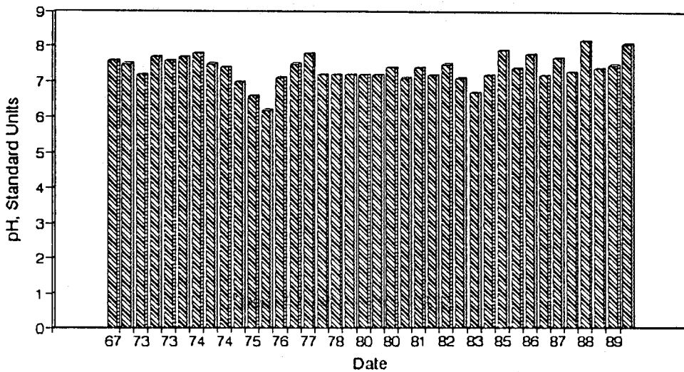
Figure A93. Graph of pH vs. Time for the White River Site-Dec.
