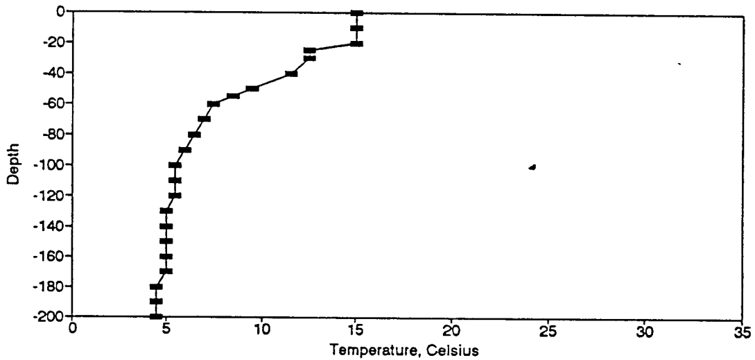
Figure BT53. Temperature Profile for the Eureka Springs Site-May 9, 1978.
