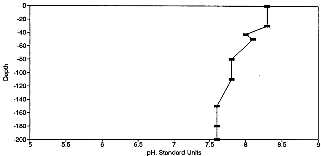
Figure BP6. pH Profile for the Eureka Springs Site-May 14, 1974.
