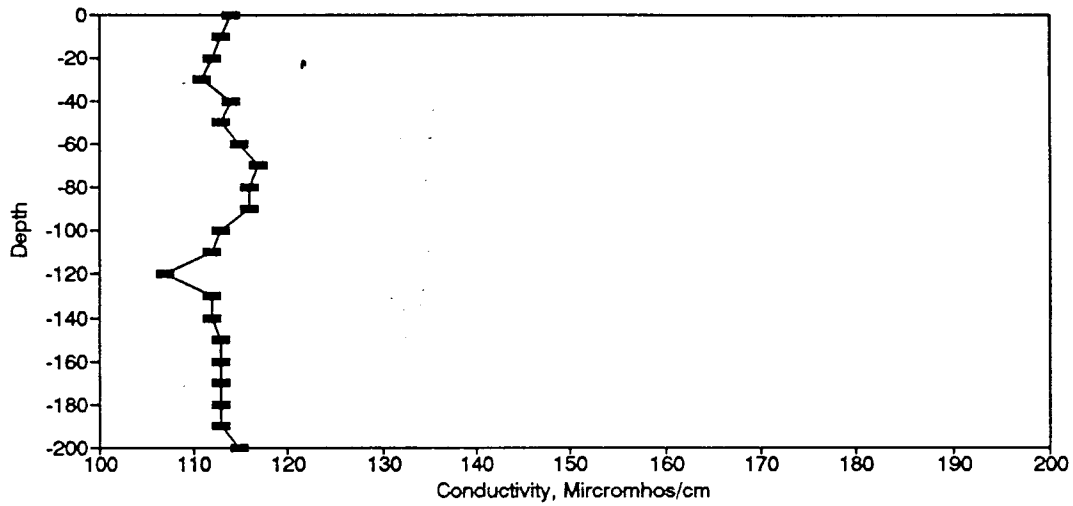
Figure BC4. Conductivity Profile for the Eureka Springs Site-March 19, 1974.
