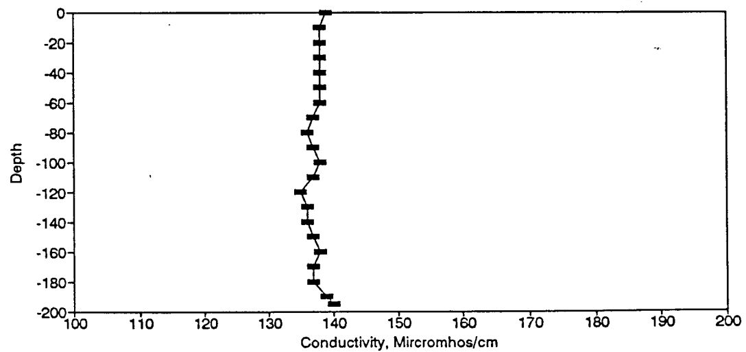
Figure BC168. Conductivity Profile for the Eureka Springs Site-January 20, 1988.
