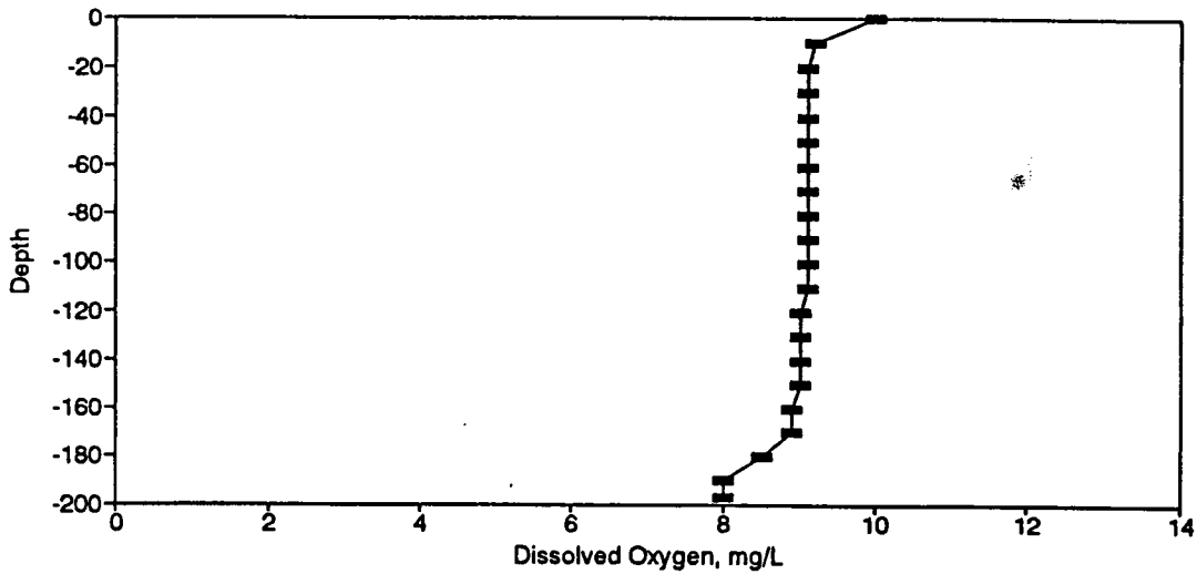
Figure BD109. Dissolved Oxygen Profile for the Eureka Springs Site-February 11, 1983.
