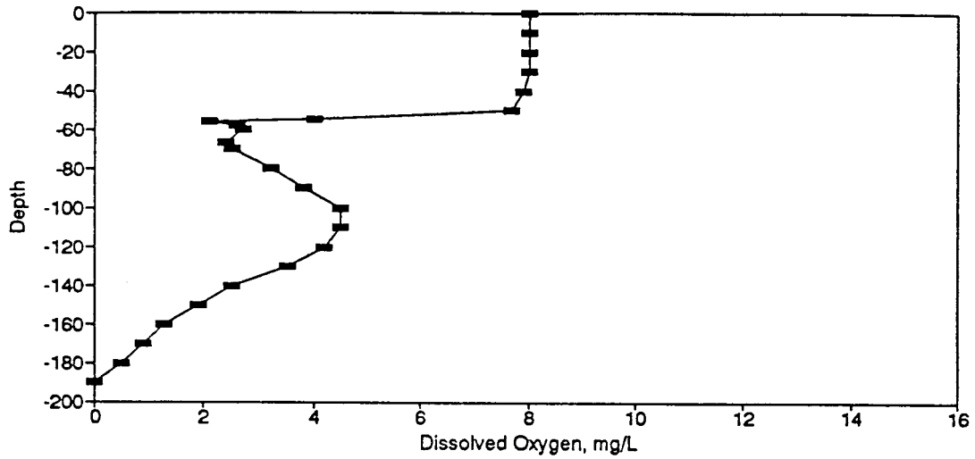
Figure BD70. Dissolved Oxygen Profile for the Eureka Springs Site-October 16, 1979.
