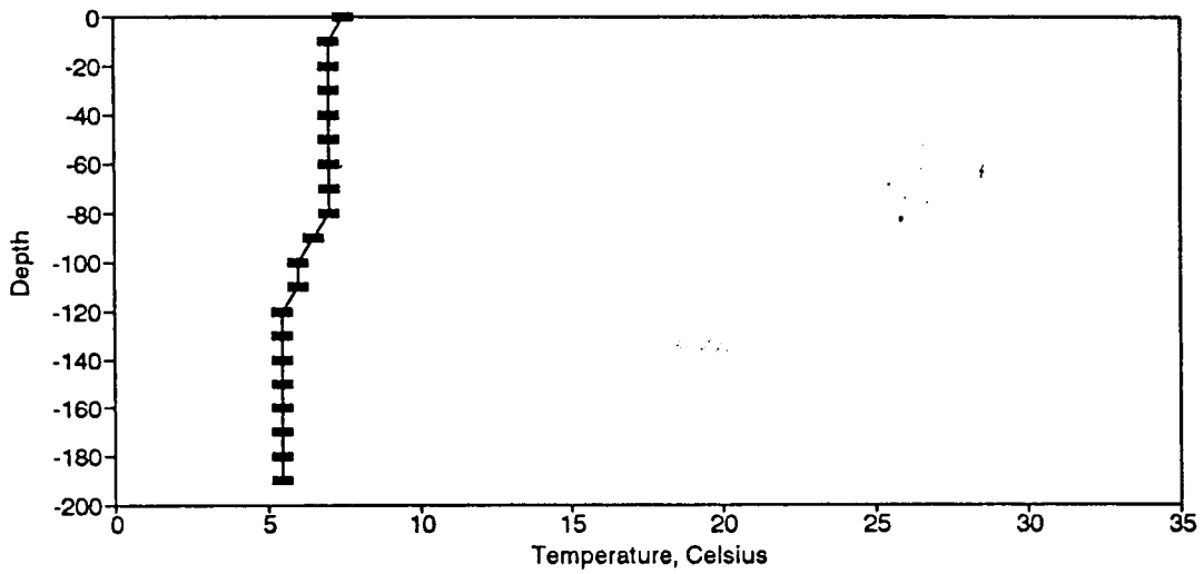
Figure BT170. Temperature Profile for the Eureka Springs Site-March 16, 1988.
