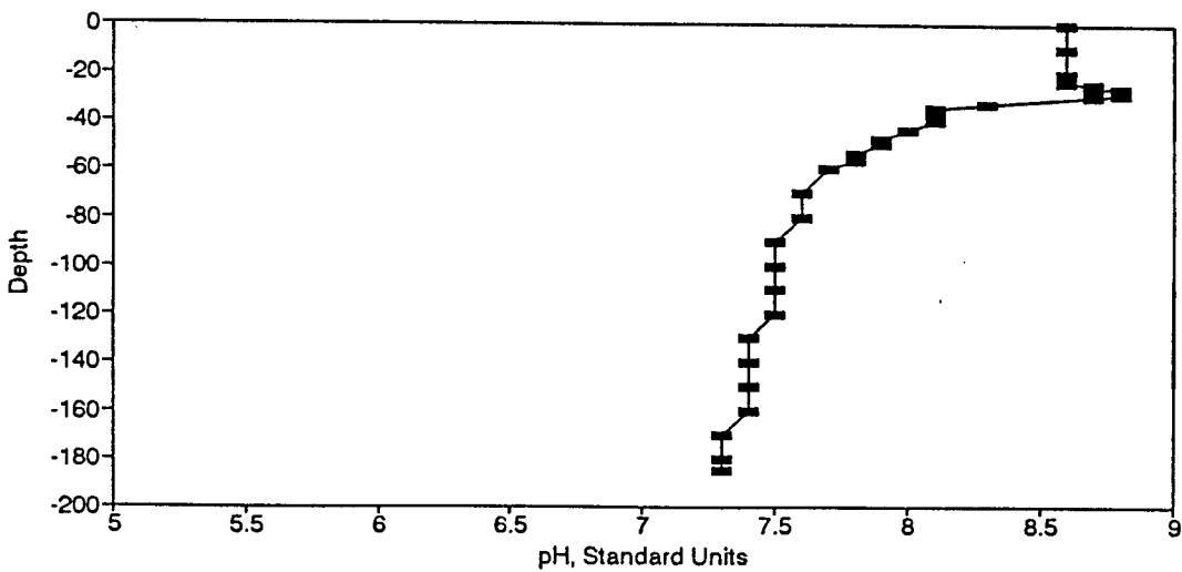
Figure BP102. pH Profile for the Eureka Springs Site-July 20, 1982.
