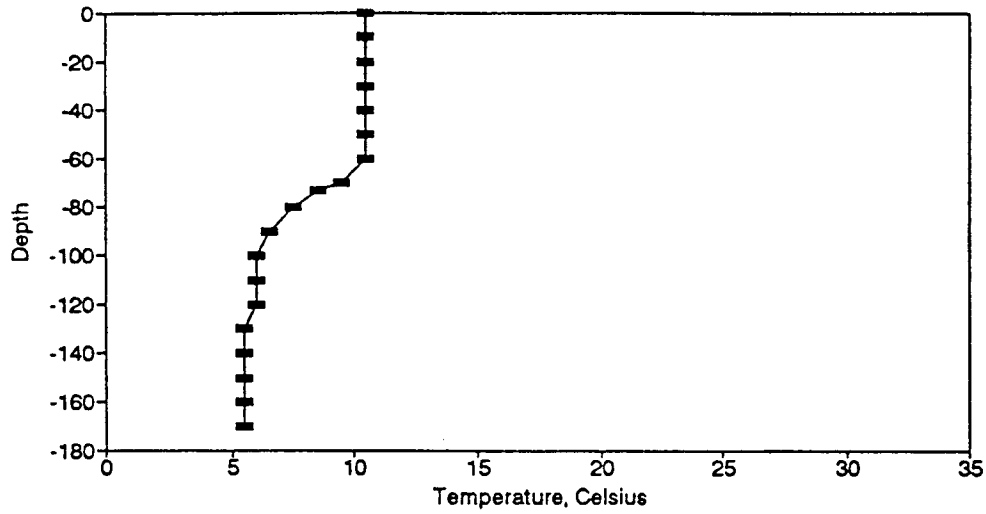
Figure BT76. Temperature Profile for the Eureka Springs Site-April 8, 1980.
