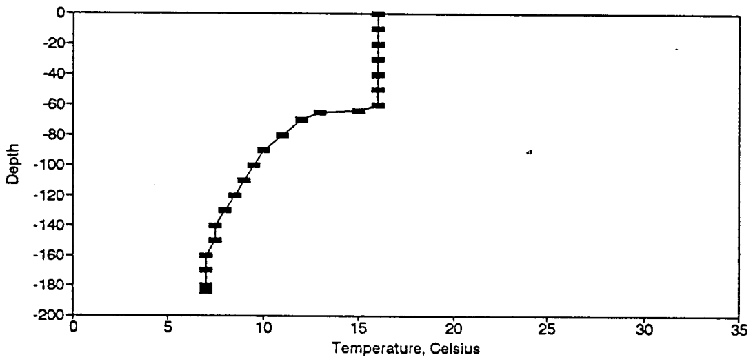
Figure BT71. Temperature Profile for the Eureka Springs Site-November 6, 1979.
