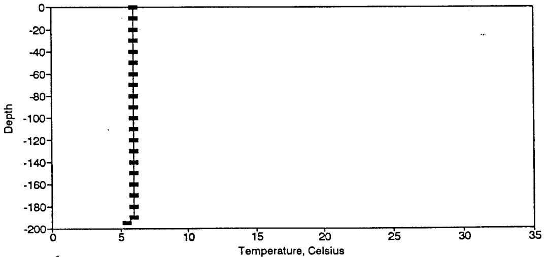
Figure BT168. Temperature Profile for the Eureka Springs Site-January 20, 1988.
