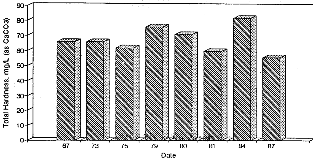
Figure A27. Graph of Total Hardness vs. Time for the White River Site-Dec.
