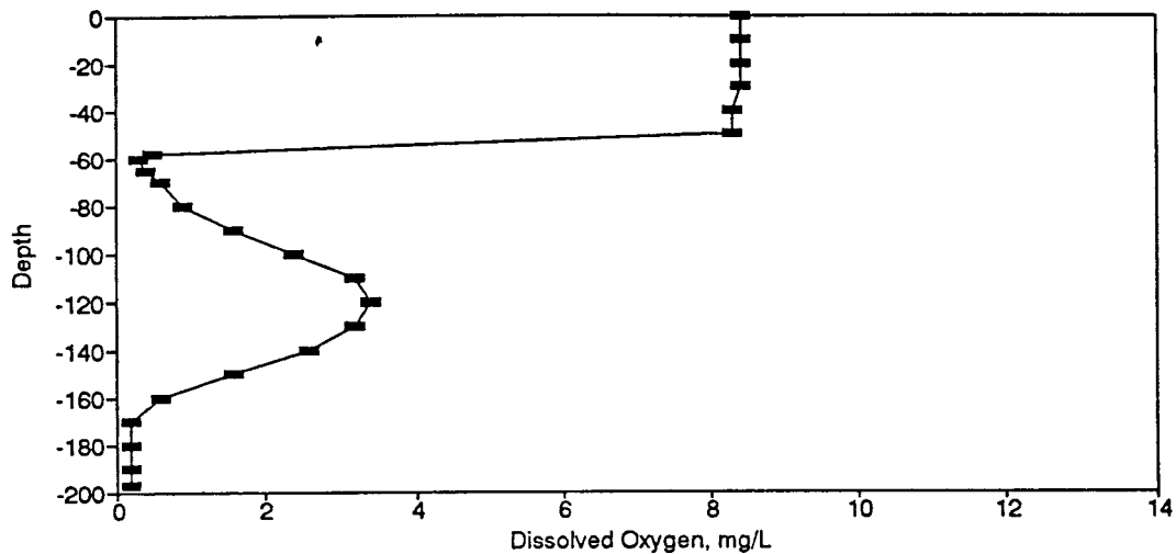
Figure BD154. Dissolved Oxygen Profile for the Eureka Springs Site-November 5, 1986.
