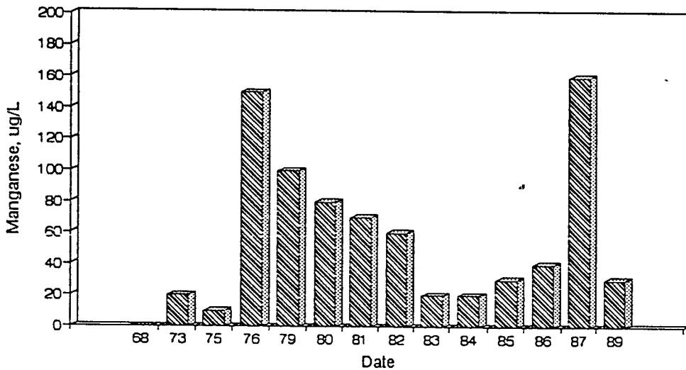
Figure A59. Graph of Manganese vs. Time for the White River Site-Aug.
