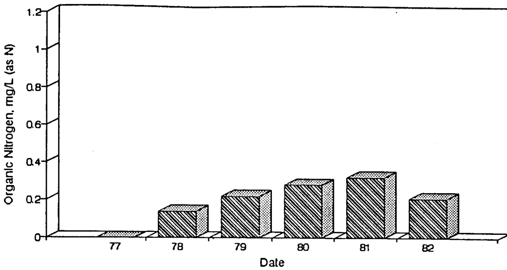
Figure A79. Graph of Organic Nitrogen vs. Time for the White River Site-May.
