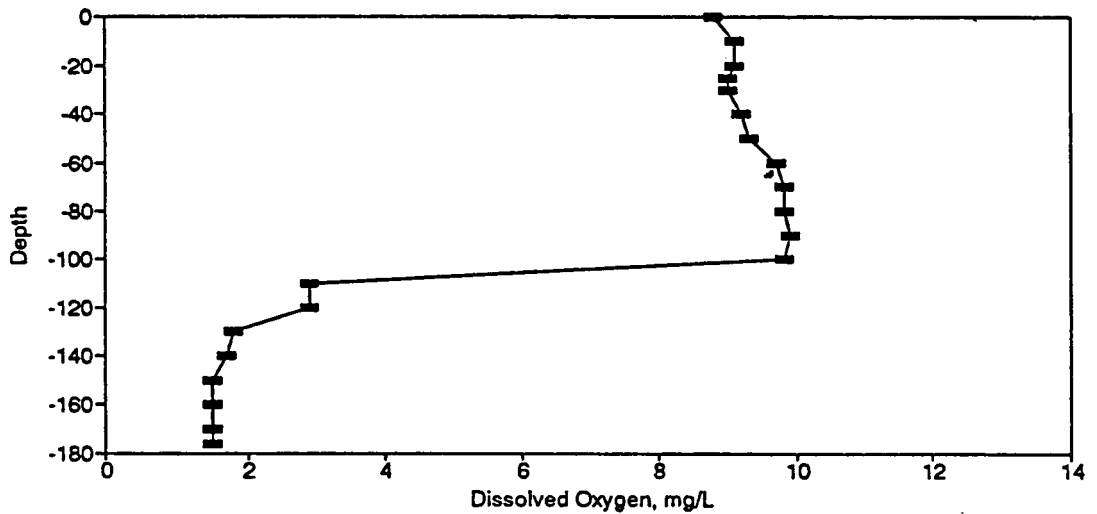
Figure BD119. Dissolved Oxygen Profile for the Eureka Springs Site-December 7, 1983.
