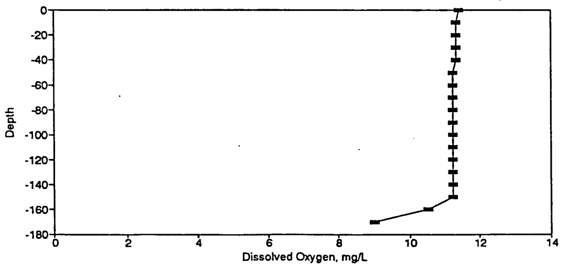
Figure BD120. Dissolved Oxygen Profile for the Eureka Springs Site-January 25, 1984.
