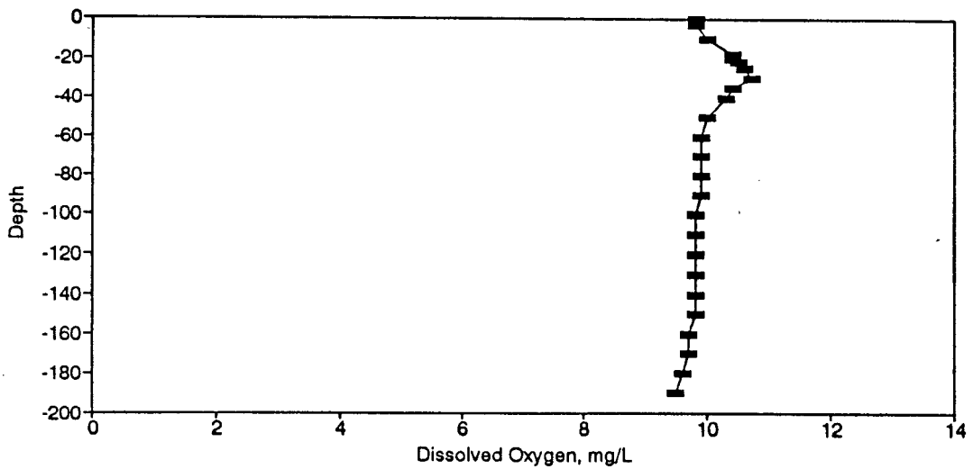
Figure BD183. Dissolved Oxygen Profile for the Eureka Springs Site-May 2, 1989.
