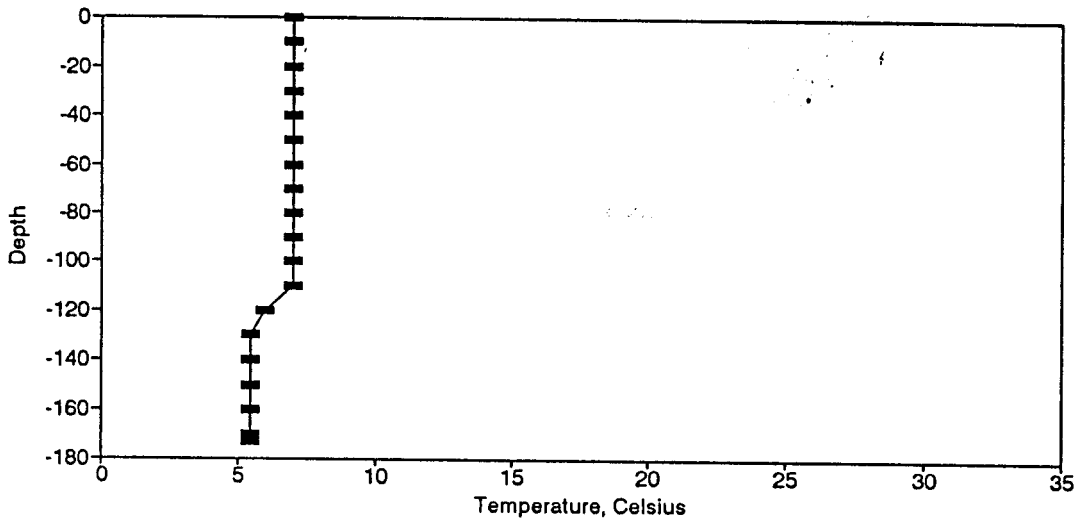
Figure BT122. Temperature Profile for the Eureka Springs Site-March 28, 1984.
