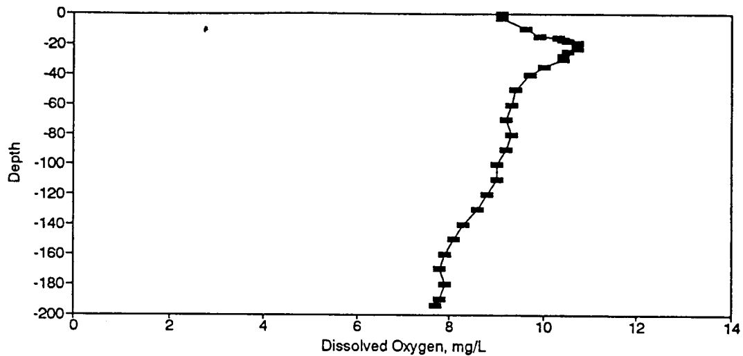
Figure BD160. Dissolved Oxygen Profile for the Eureka Springs Site-May 13, 1987.
