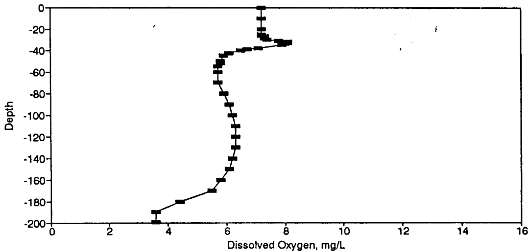
Figure BD68. Dissolved Oxygen Profile for the Eureka Springs Site-August 22, 1979.
