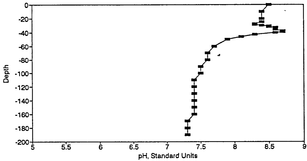
Figure BP80. pH Profile for the Eureka Springs Site-August 13, 1980.
