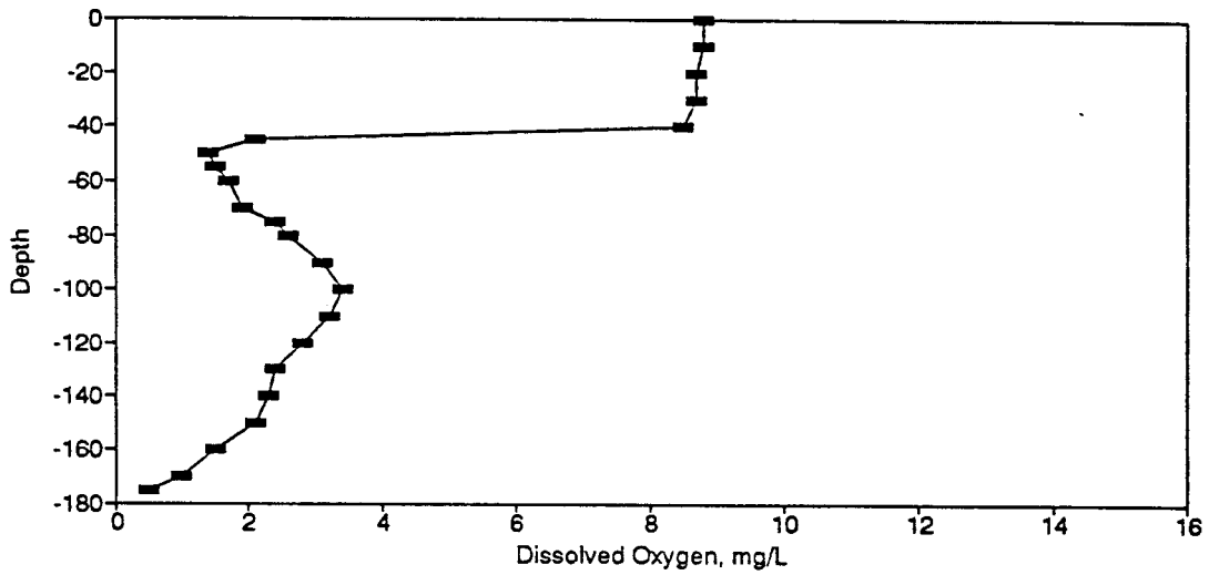
Figure BD59. Dissolved Oxygen Profile for the Eureka Springs Site-November 7, 1978.
