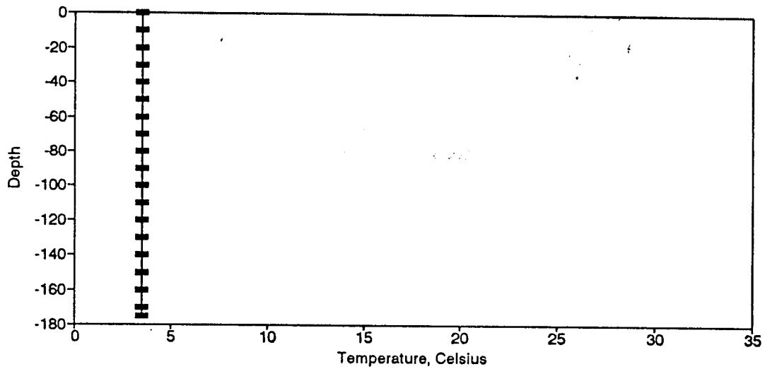
Figure BT62. Temperature Profile for the Eureka Springs Site-February 14, 1979.
