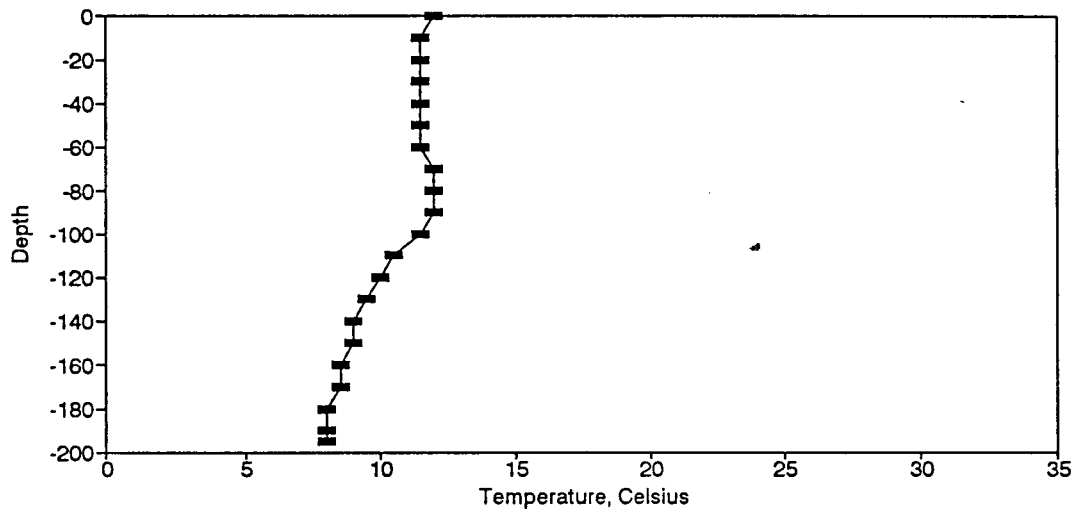
Figure BT155. Temperature Profile for the Eureka Springs Site-December 4, 1986.
