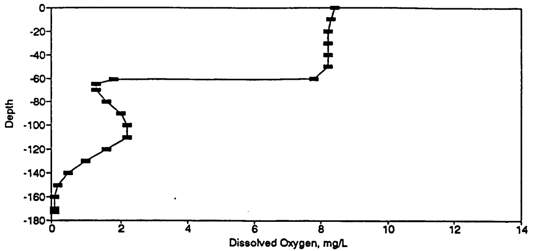
Figure BD118. Dissolved Oxygen Profile for the Eureka Springs Site-November 14, 1983.
