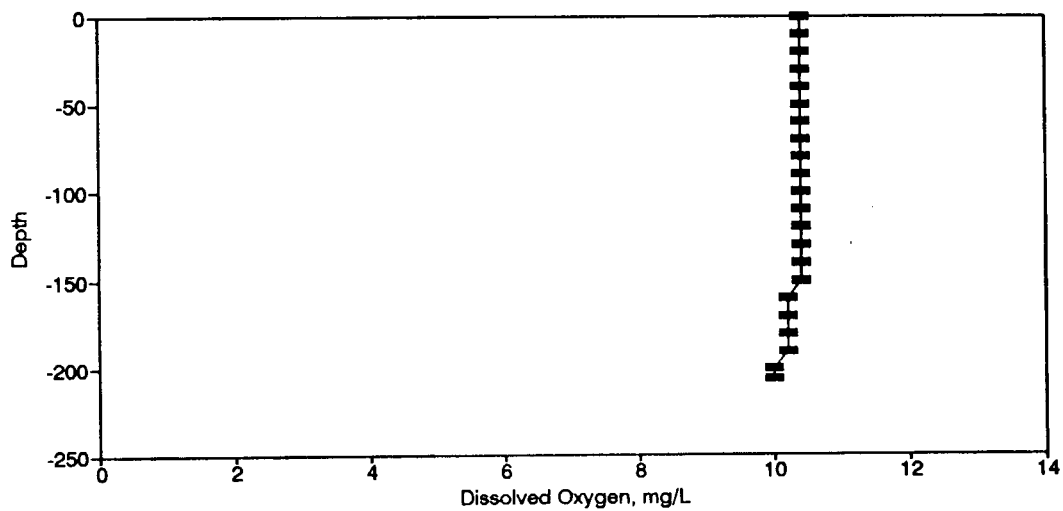
Figure BD135. Dissolved Oxygen Profile for the Eureka Springs Site-April 3, 1985.
