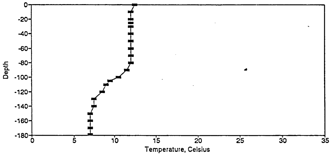
Figure BT95. Temperature Profile for the Eureka Springs Site-December 9, 1981.
