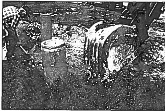
A poultry disposal pit near Lincoln, Ark., served as the test site for water quality research by University of Arkansas scientists. Shutting down the pit was the final stage in the field work portion of the study.
