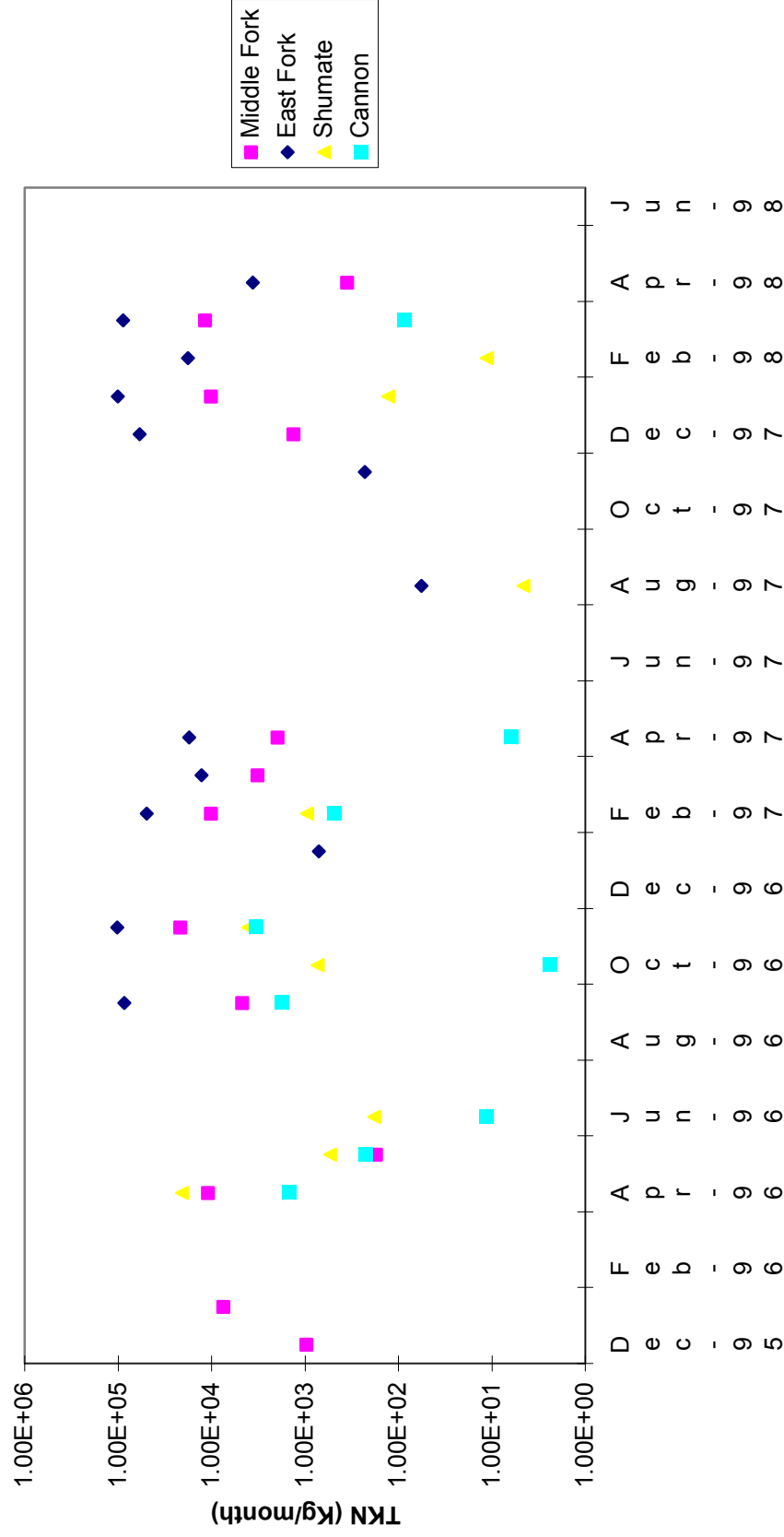
Figure 23. Monthly storm flow TKN loads for the East Fork, Middle Fork, Cannon Creek, and Shumate Creek.
