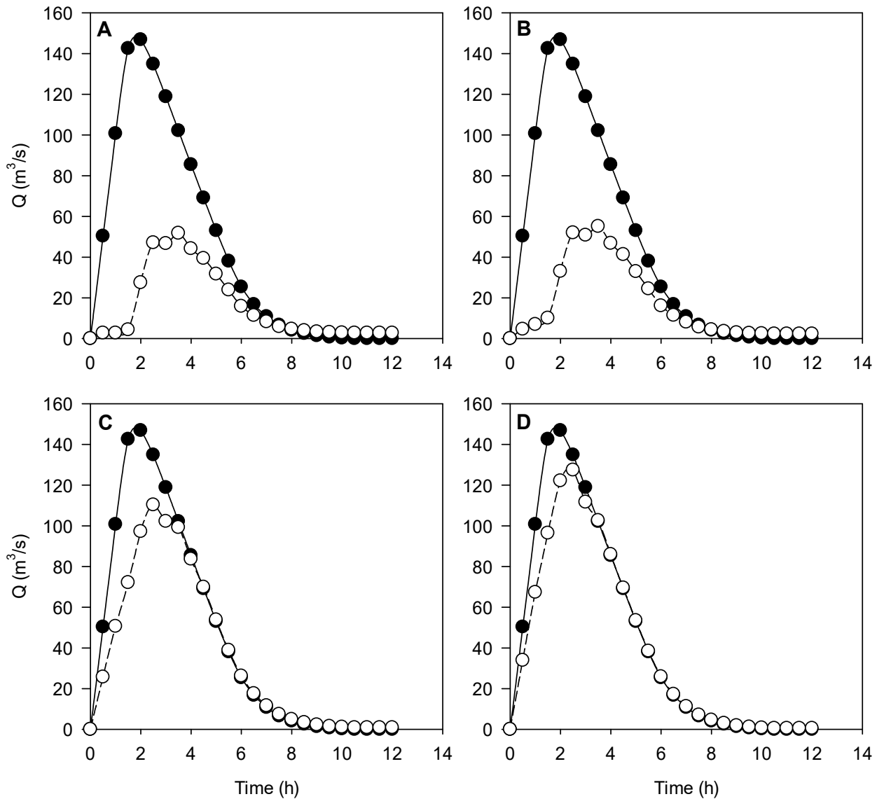
Figure 5. Simulated peakflow without (black circles and line) and with (white circles and line) ponds across A) all headwater sub-basins, B) moderate hydrologic risk sub-basins (CN \geq 70), C) elevated hydrologic risk sub-basins (CN \geq 75), or D) severe hydrologic risk sub-basins (CN \geq 80).
