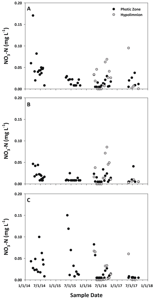
Figure 3. Measured nitrate-N ( NO_3-N ) concentrations for the Forest Service Lakes during the 2014-2017 growing seasons for (A) Cove, (B) Spring, and (C) Wedington. Black circles represent photic zone samples and gray circles represent hypolimnion samples.
