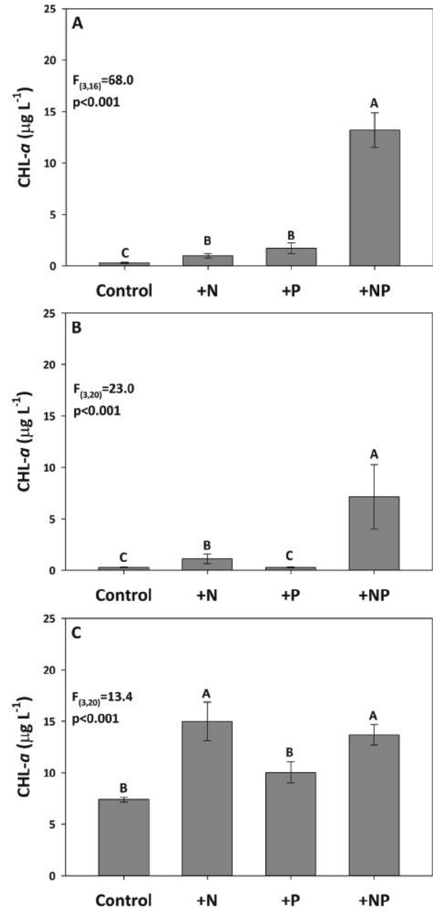
Figure 9. Mean (error bars=± 1 standard error) chlorophyll-a (CHL-a) concentrations across nutrient treatments, including: control, plus nitrogen (+N), plus phosphorus (+P), and plus nitrogen and phosphorus (+NP), for Spring Lake in 2017. Letters above error bars identify homogeneous groups. A: Pre-lake fertilization on May 23 2017. B: Pre-lake fertilization on June 25. C: Post-lake fertilization on July 14.
