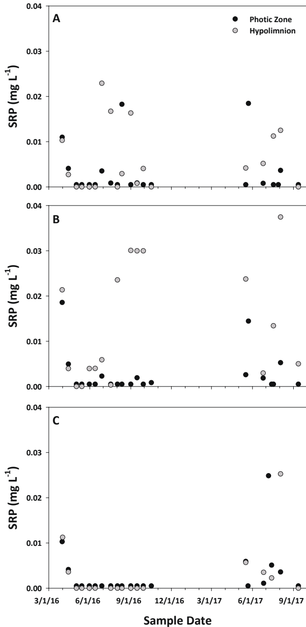
Figure 1. Measured soluble reactive phosphorus (SRP) concentrations for the Forest Service Lakes during the 2016-2017 growing seasons for (A) Cove, (B) Spring, and (C) Wedington. Black circles represent photic zone samples and gray circles represent hypolimnion samples.
