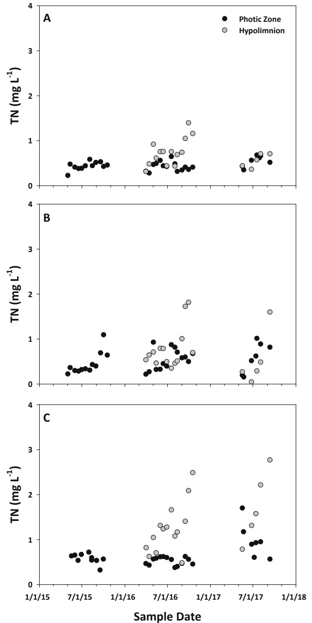
Figure 4. Measured total nitrogen (TN) concentrations for the Forest Service Lakes during the 2015-2017 growing seasons for (A) Cove, (B) Spring, and (C) Wedington. Black circles represent photic zone samples and gray circles represent hypolimnion samples.
