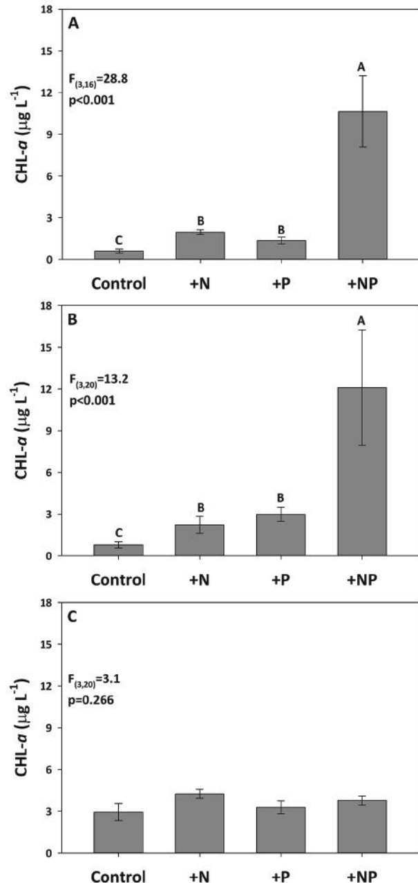
Figure 8. Mean (error bars=± 1 standard error) chlorophyll-a (CHL-a) concentrations across nutrient treatments, including: control, plus nitrogen (+N), plus phosphorus (+P), and plus nitrogen and phosphorus (+NP), for Cove Lake in 2017. Letters above error bars identify homogeneous groups. A: Pre-lake fertilization on May 23 2017. B: Pre-lake fertilization on June 25. C: Post-lake fertilization on July 27.
