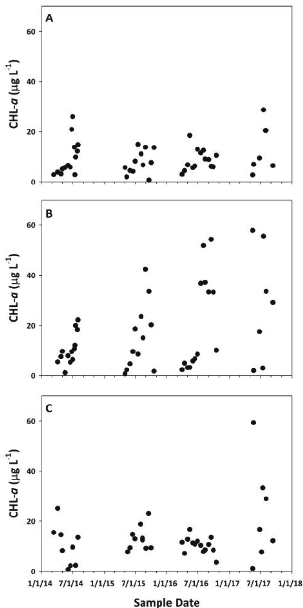
Figure 6. Measured chlorophyll-a (CHL-a) concentrations in the photic zone of the Forest Service Lakes during the 2014-2017 growing seasons for (A) Cove, (B) Spring, and (C) Wedington. Vertical bars represent when lakes were fertilized. Fertilization dates for Cove and Spring Lakes in 2016 were not available.
