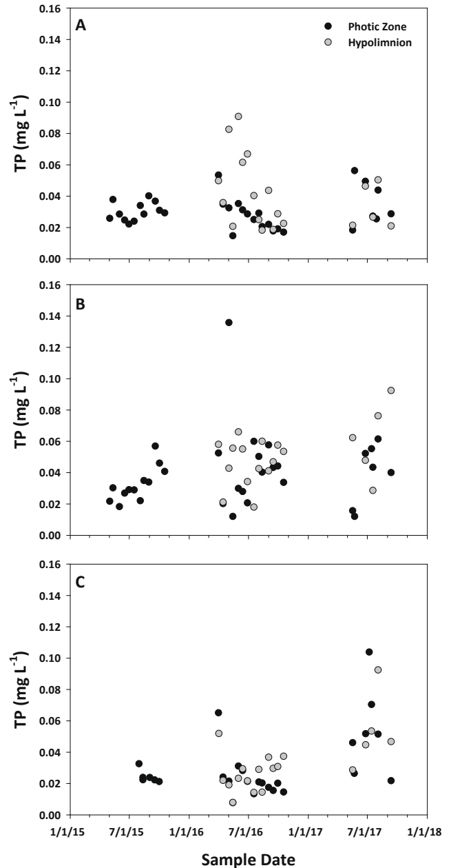
Figure 2. Measured total phosphorus (TP) concentrations for the Forest Service Lakes during the 2015-2017 growing seasons for (A) Cove, (B) Spring, and (C) Wedington. Black circles represent photic zone samples and gray circles represent hypolimnion samples.
