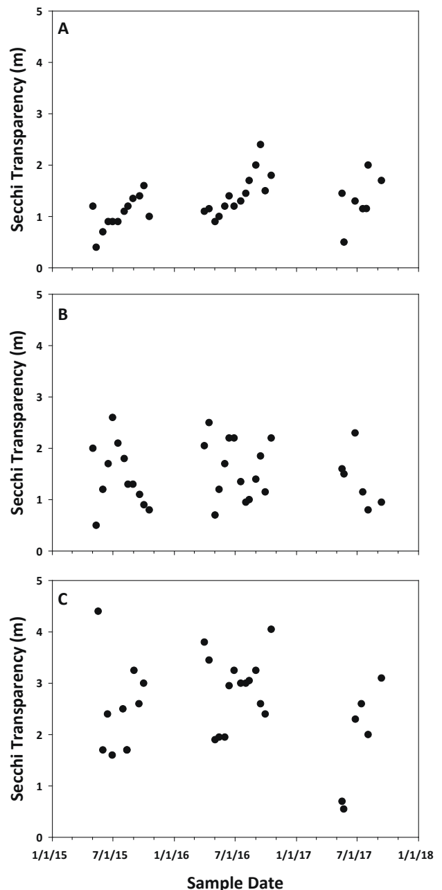
Figure 5. Measured secchi transparency for the Forest Service Lakes during the 2015-2017 growing seasons for (A) Cove, (B) Spring, and (C) Wedington.
